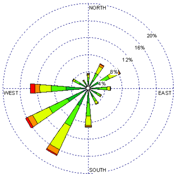
Tucumcari (23048) 1985-2005 Annual Average - all hours Average Speed = 9.29 kts
