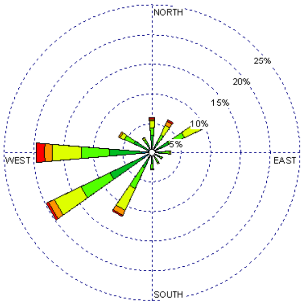
Tucumcari (23048) 1985-2005 April - 10-15z Average Speed - 9.12 kt
