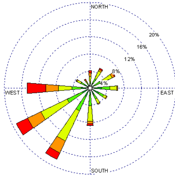
Tucumcari (23048) 1985-2005 April - 19-23z Average Speed - 12.97 kt
