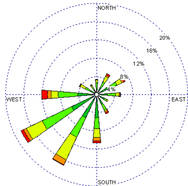
Tucumcari (23048) 1985-2005 April - 03-09z Average Speed - 9.25 kt
