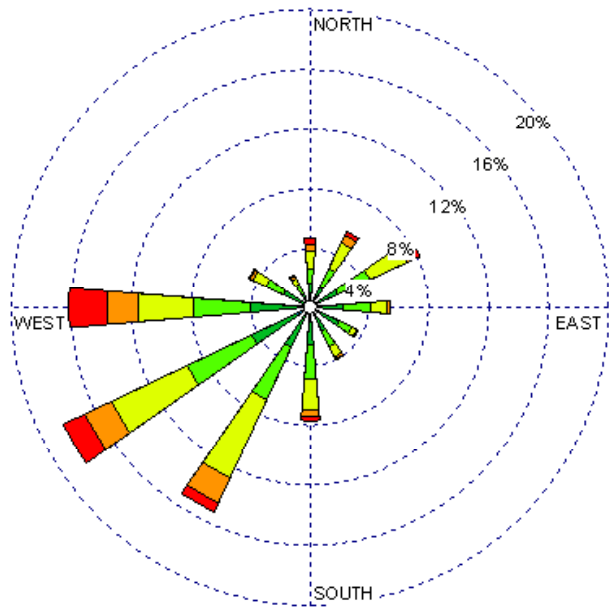
Tucumcari (23048) 1985-2005 April - All hours Average Speed - 10.95 kt
