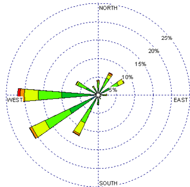
Tucumcari (23048) 1985-2005 December - 03-09z Average Speed -7.82 kt
