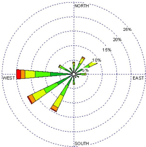
Tucumcari (23048) 1985-2005 December - All hours Average Speed -8.80 kt
