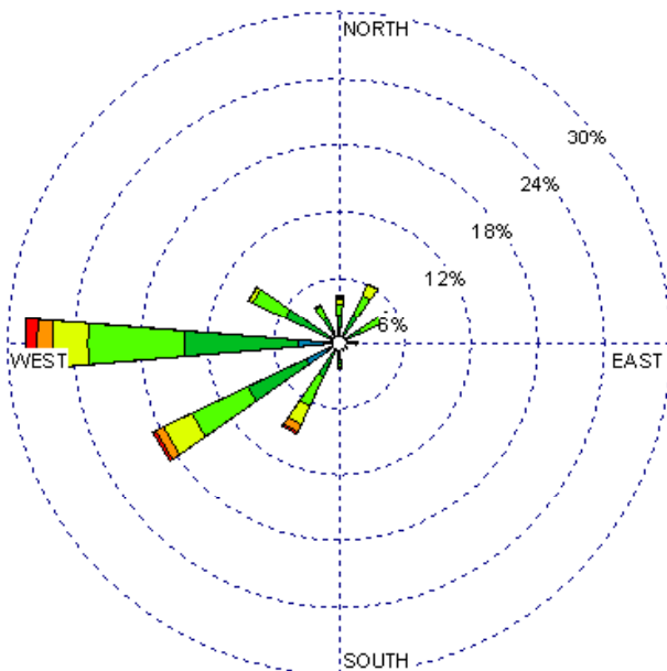
Tucumcari (23048) 1985-2005 December - 10-15z Average Speed -7.55 kt
