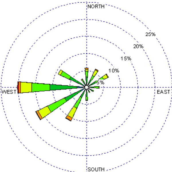
Tucumcari (23048) 1985-2005 February - 10-15z Average Speed -7.54 kt
