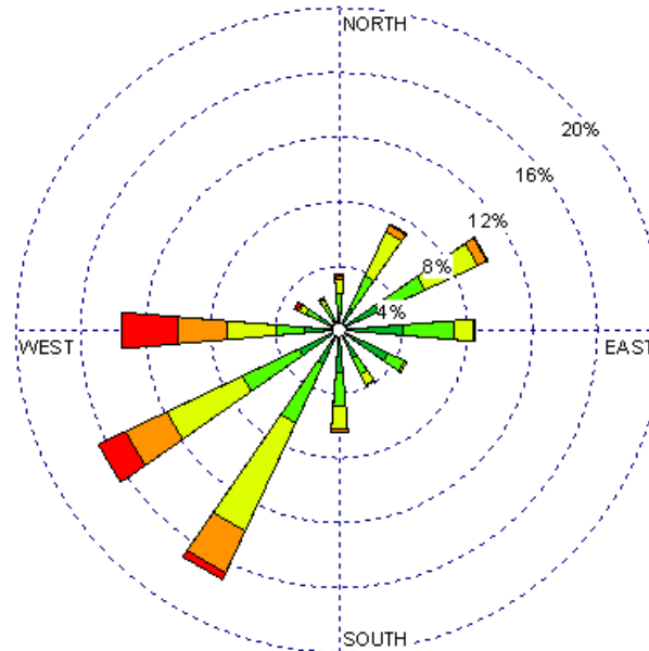
Tucumcari (23048) 1985-2005 February - 19-23z Average Speed -11.30 kt
