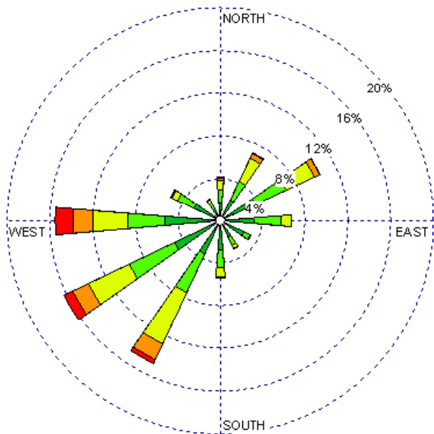
Tucumcari (23048) 1985-2005 February - All hours Average Speed -9.50 kt
