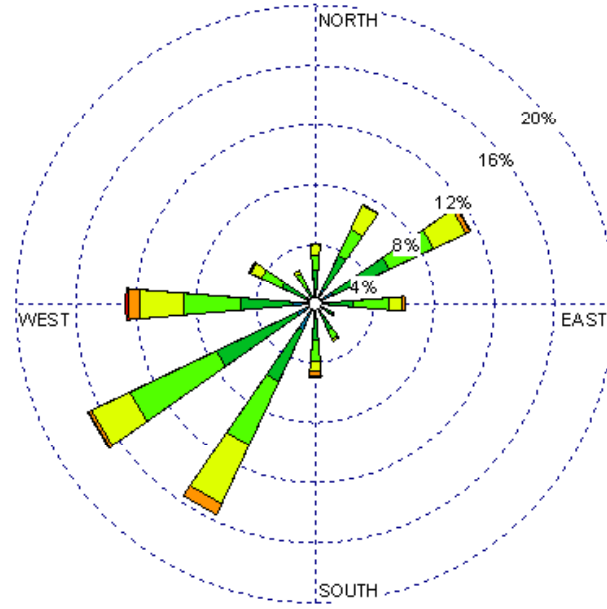
Tucumcari (23048) 1985-2005 February - 03-09z Average Speed -7.89 kt
