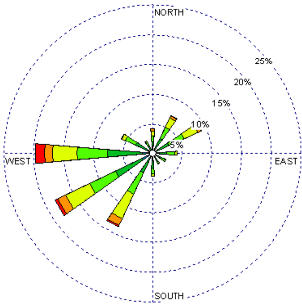
Tucumcari (23048) 1985-2005 January - All hours Average Speed -8.90 kt
