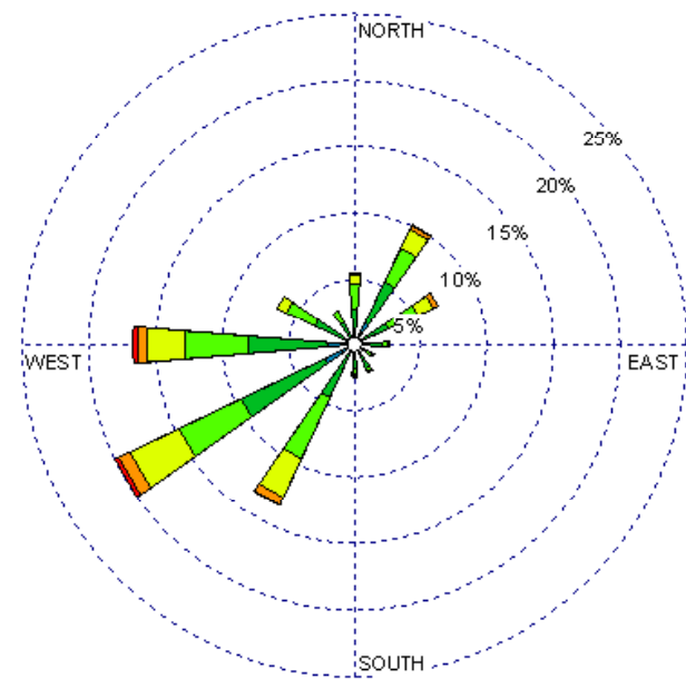
Tucumcari (23048) 1985-2005 January - 03-09z Average Speed -7.70 kt
