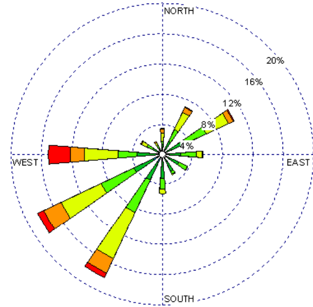
Tucumcari (23048) 1985-2005 January - 19-23z Average Speed -10.39 kt
