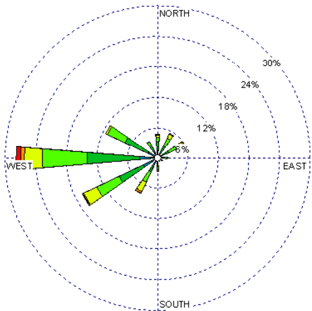
Tucumcari (23048) 1985-2005 January - 10-15z Average Speed -7.19 kt
