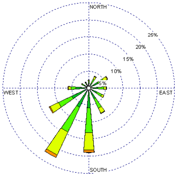
Tucumcari (23048) 1985-2005 July - All hours Average Speed -8.64 kt
