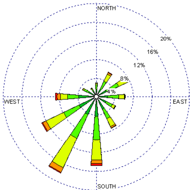
Tucumcari (23048) 1985-2005 June - All hours Average Speed -9.45 kt
