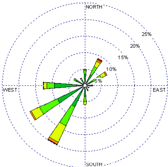
Tucumcari (23048) 1985-2005 September - 10-15z Average Speed= 7.26 kt
