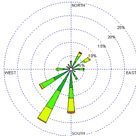
Tucumcari (23048) 1985-2005 September - 03-09z Average Speed= 7.53 kt
