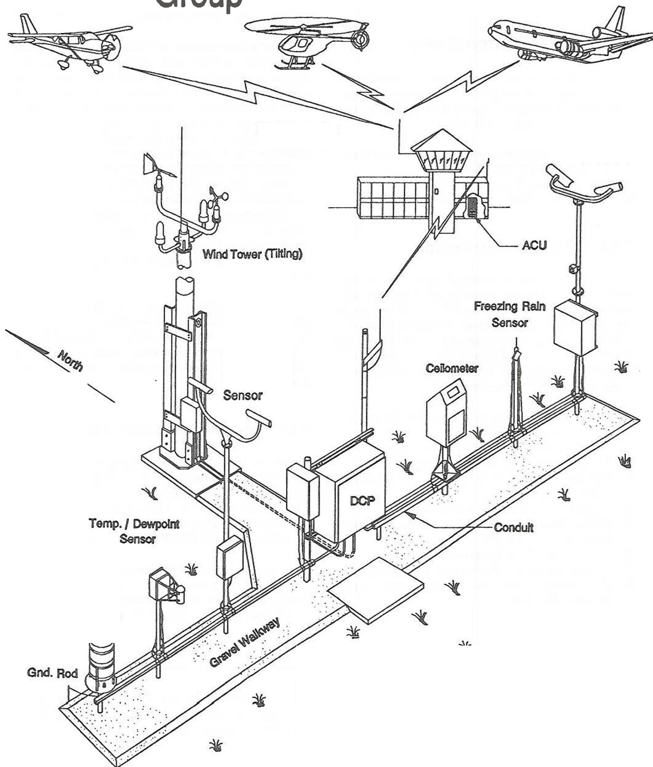
Figure 2. ASOS Combined Sensor Group
