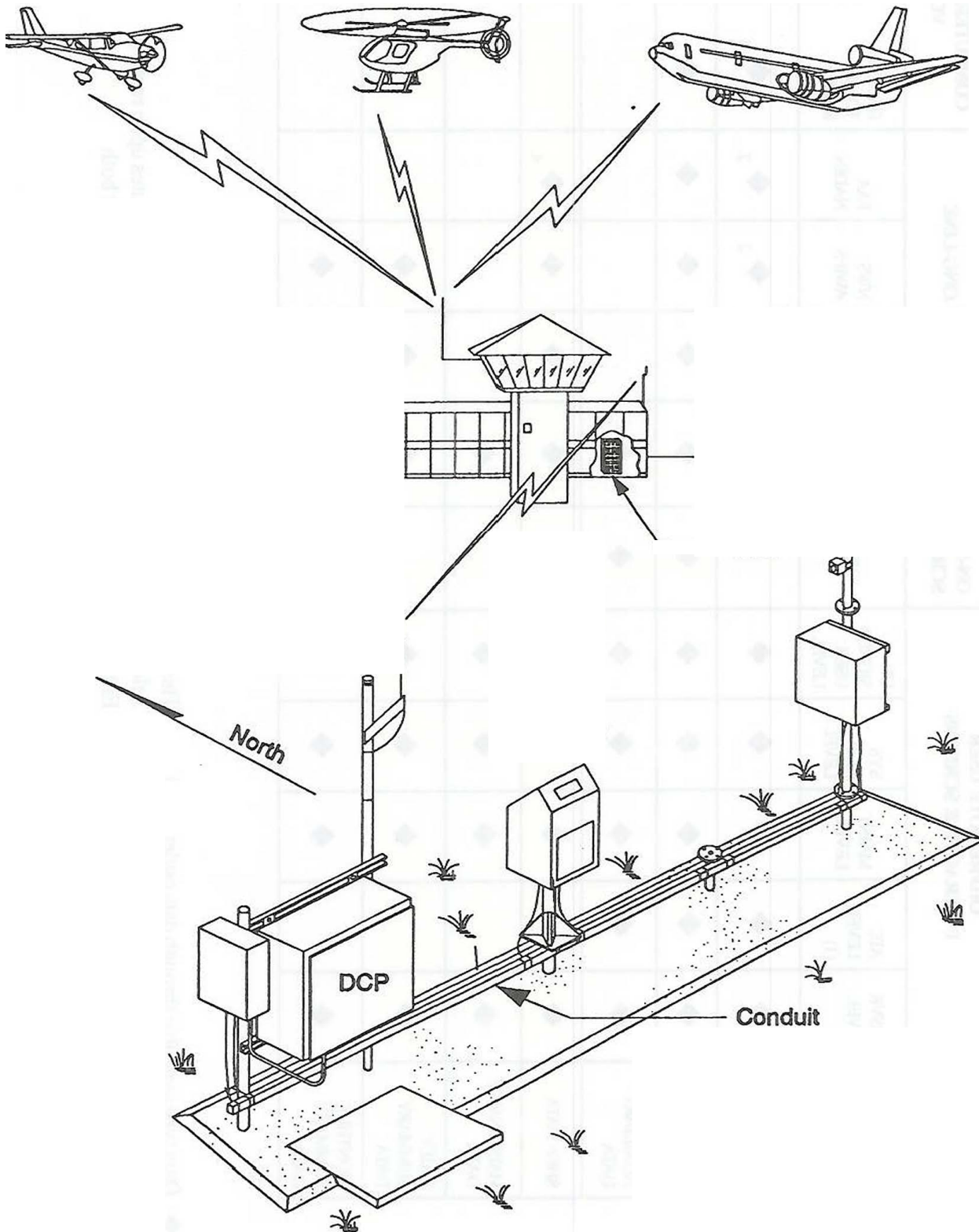
Figure 3. Additional Sensor Group
