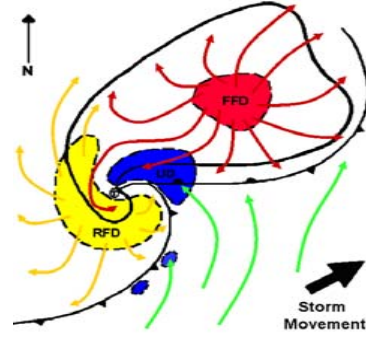
Tornado on backside of the storm relative to storm motion. Surface wind flow near tornado. RFD flow on left. Inflow on right. Tornado/wall cloud in middle.
