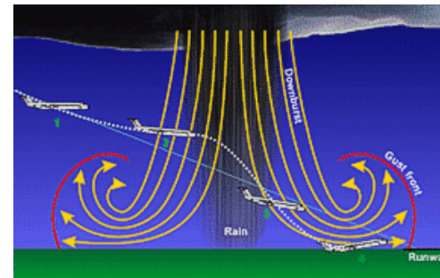
Microburst. Plane: headwind/lift, then downward tailwind.
