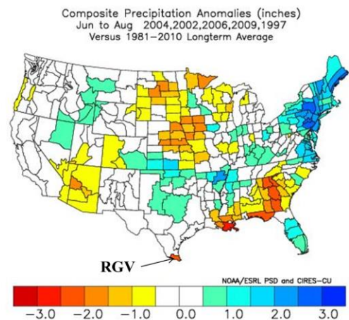
The NOAA/NCDC Climate Division Dataset has been updated to a newer version
