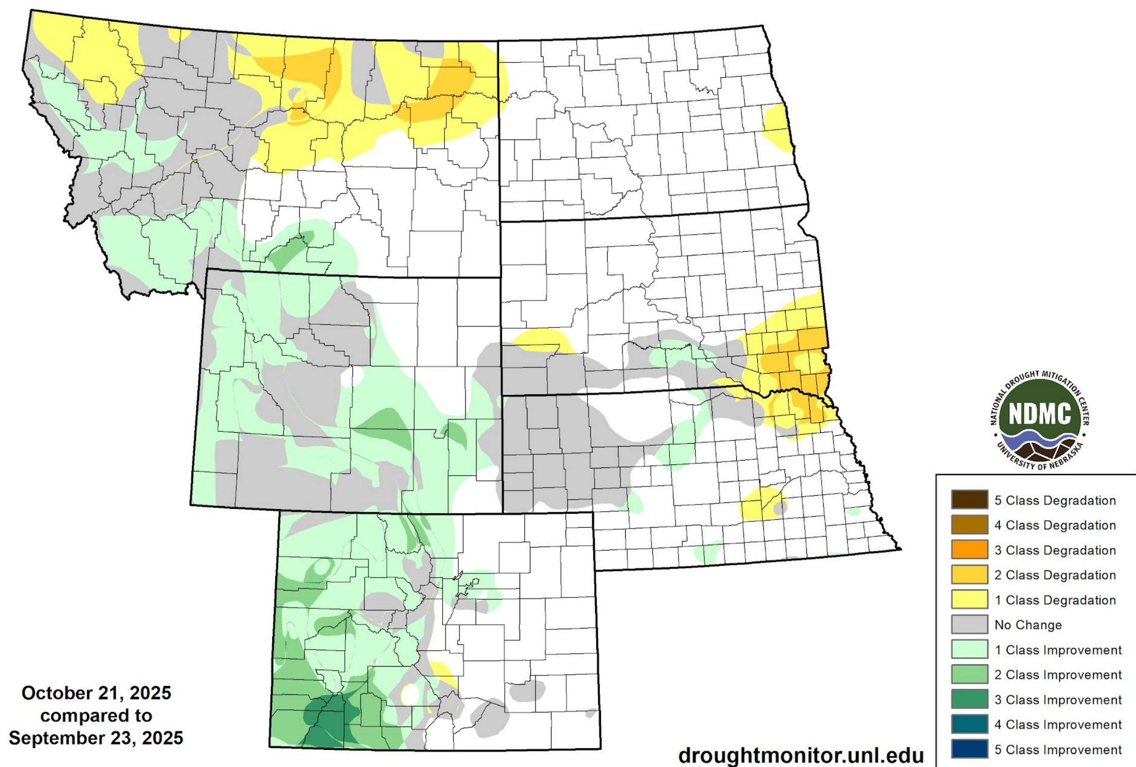
U.S. Drought Monitor Class Change - USDA Northern Plains Climate Hub 4 Week
