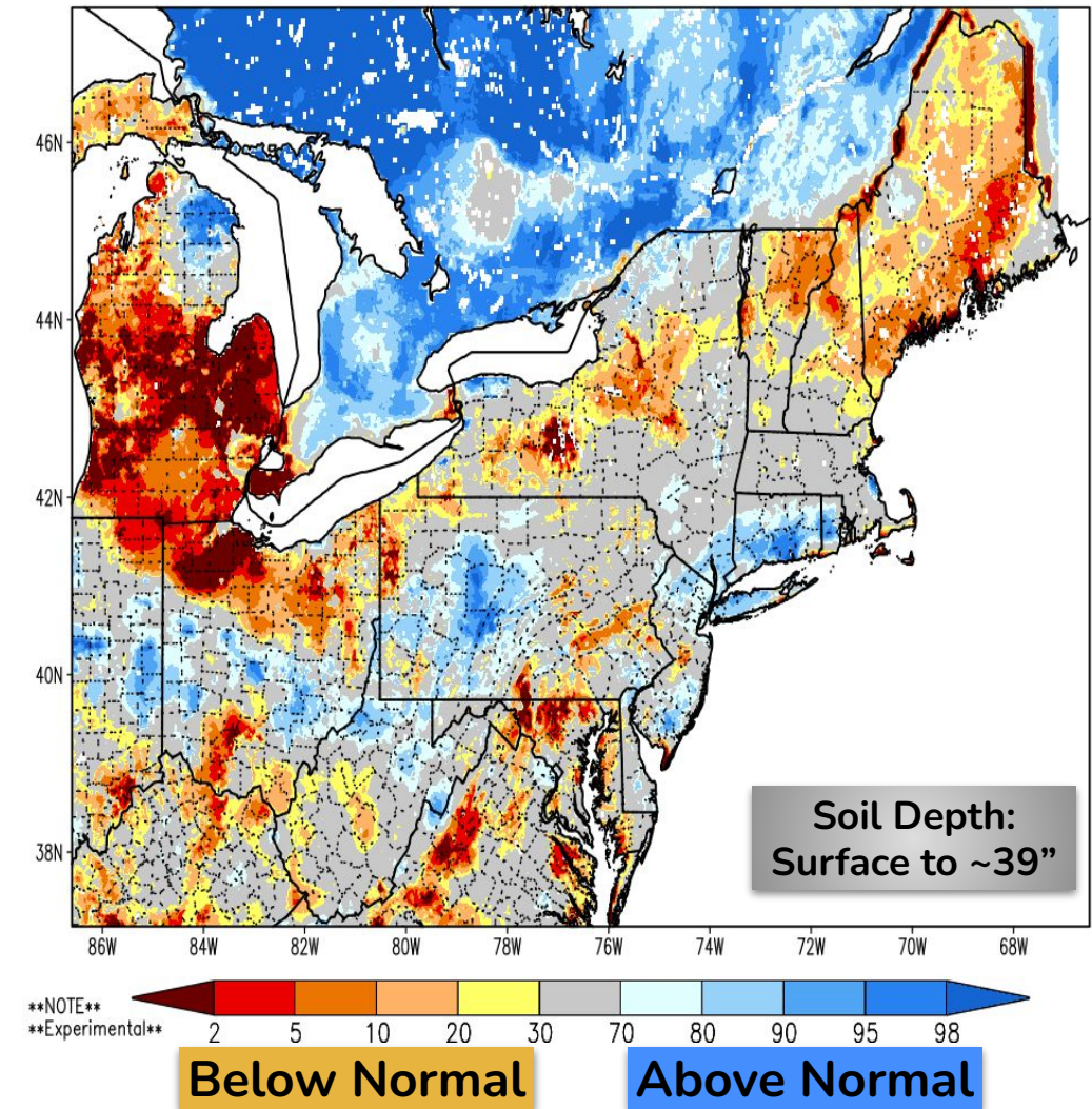
SPoRT-LIS 0-100 cm Soil Moisture percentile valid 27 Aug 2026
