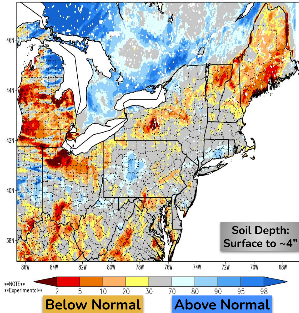
SPoRT-LIS 0-10 cm Soil Moisture percentile valid 27 Aug 2026
