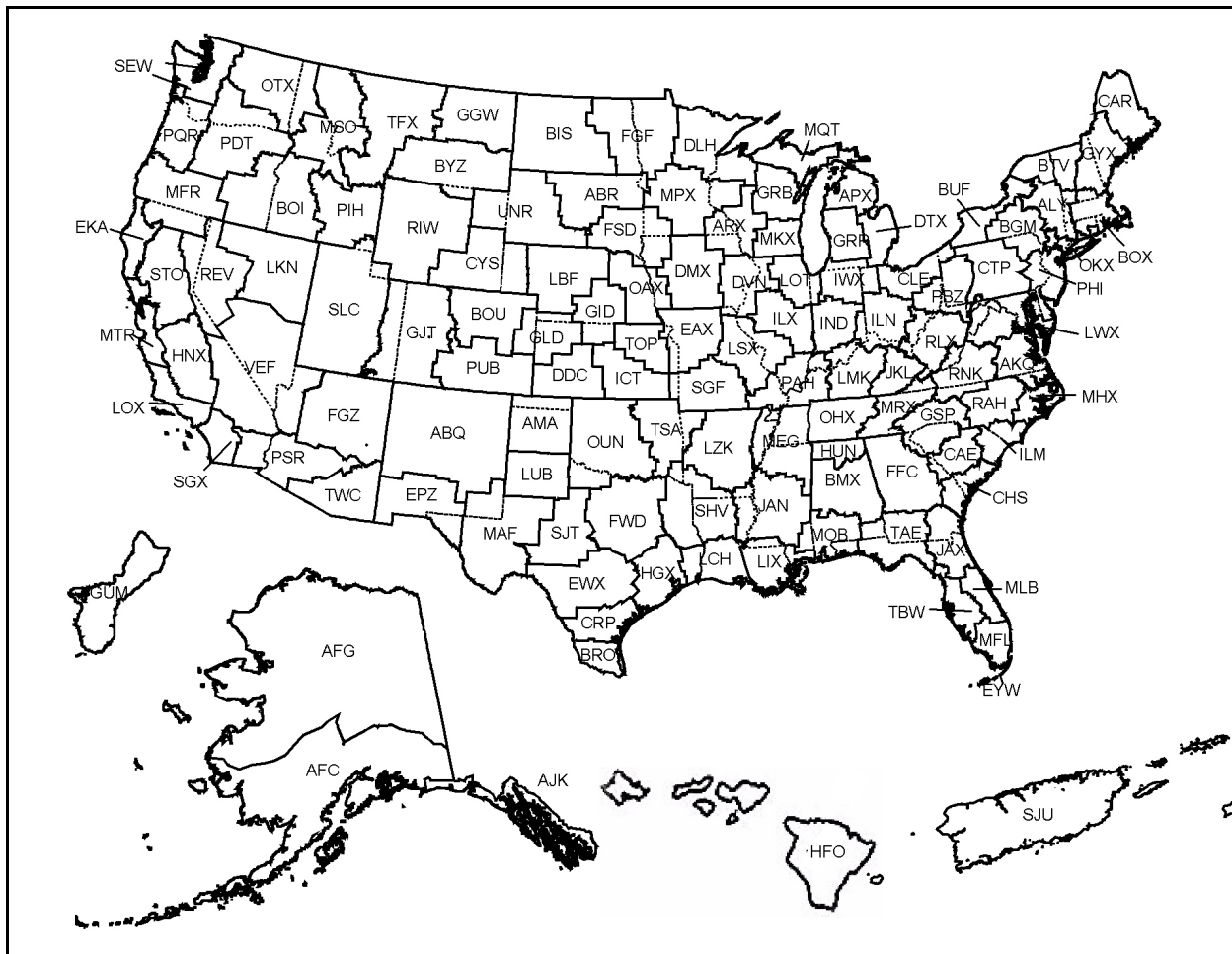
Figure 2: WFO hydrologic service areas (HSA).
