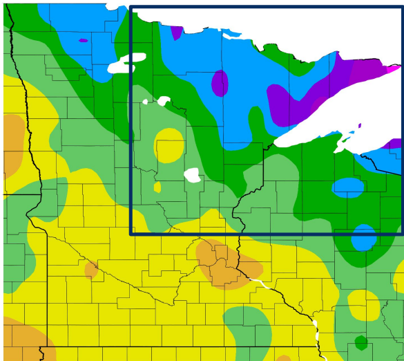
Temperature (F) 7/28/2026 – 8/26/2026
