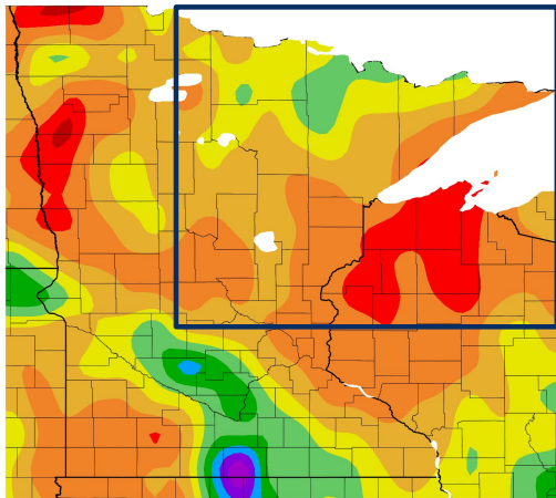
Precipitation (in) 7/28/2026 - 8/26/2026
