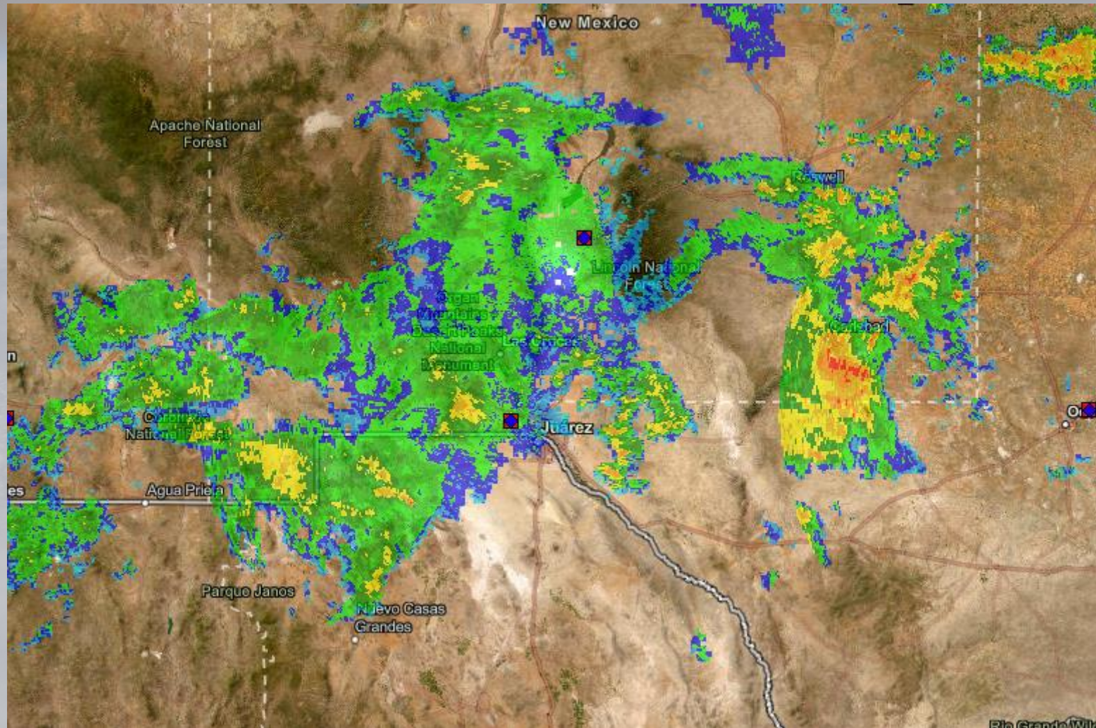
Radar imagery of Odile's remnants passing through the El Paso and Southern New Mexico regions on September 18, 2014
