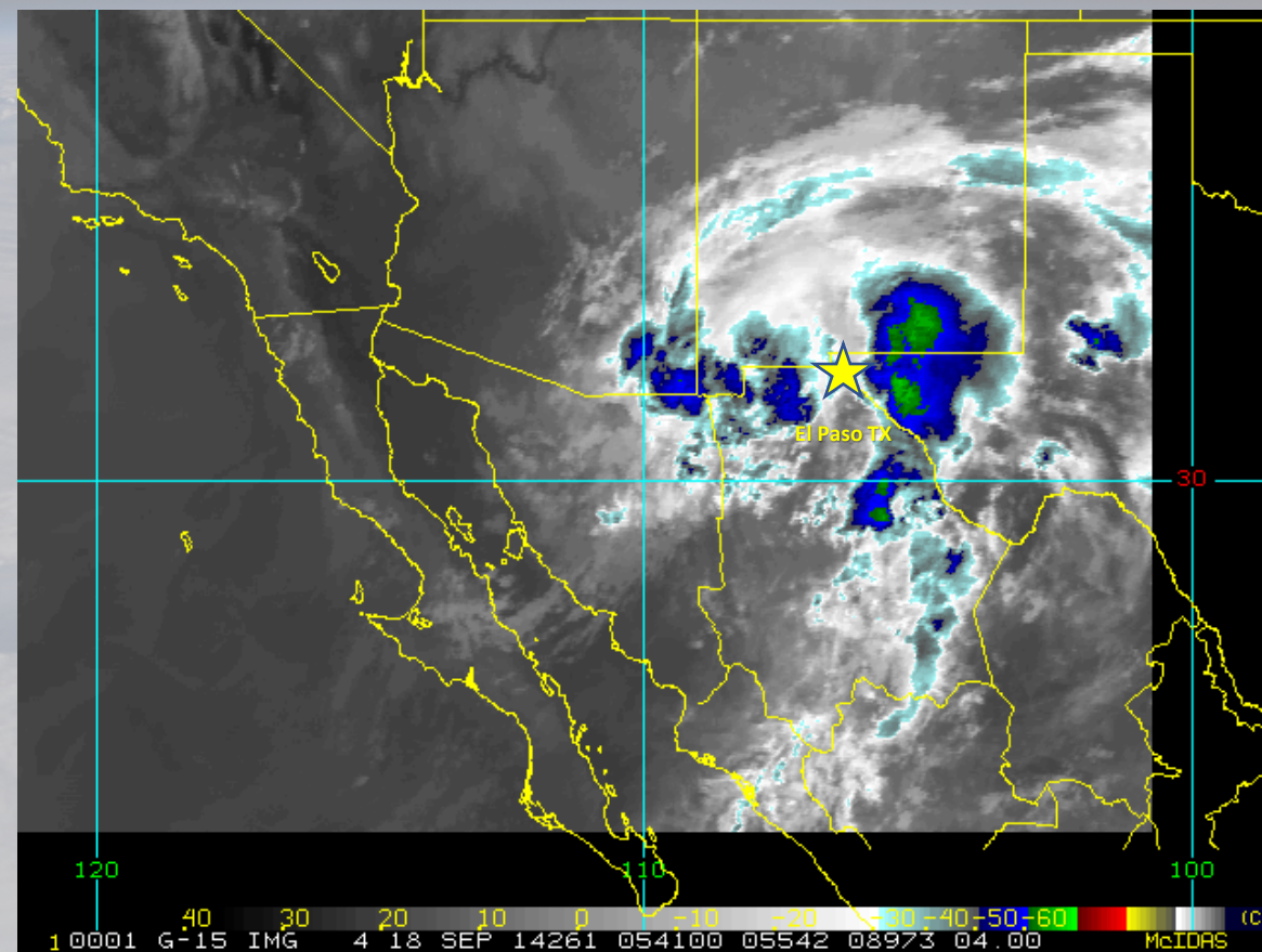
Odile Remnants over El Paso Region Sep 18
