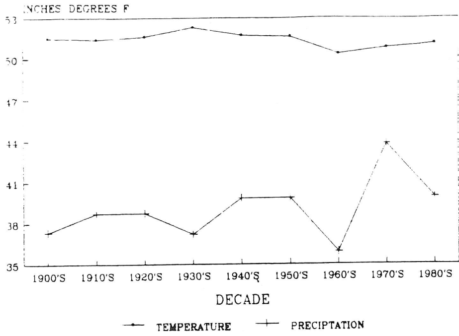
Figure 3. Pennsylvania average (based on seven stations) temperatures ( ^{\circ} F) and precipitation (inches) from 1900 to 1990.
