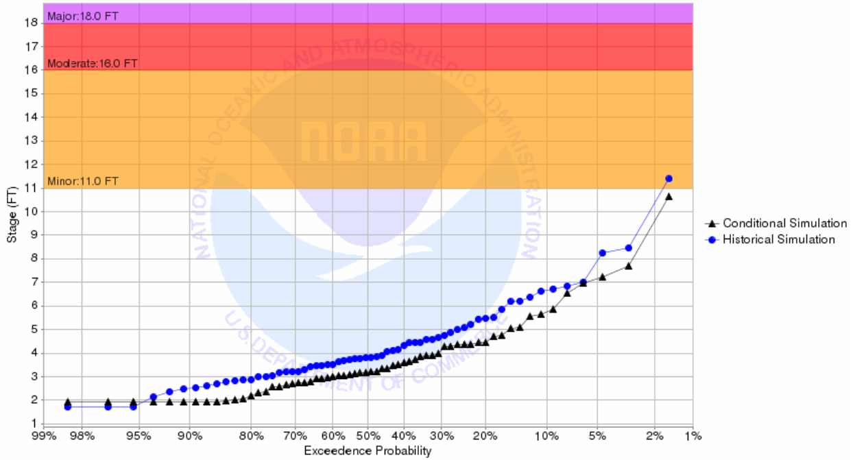
Chance of Exceeding River Stage at Pembina River at Walhalla (WLHN8) Forecast for the period 07/01/2018 - 09/29/2018 This is a conditional simulation based on the conditions as of 06/24/2018
