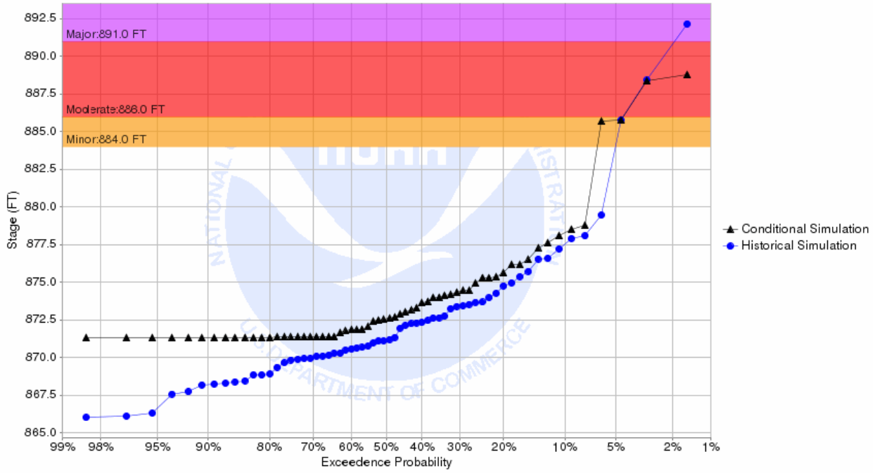
Chance of Exceeding River Stage at Sheyenne River at Harwood (HWDN8) Forecast for the period 07/01/2018 - 09/29/2018 This is a conditional simulation based on the conditions as of 06/24/2018
