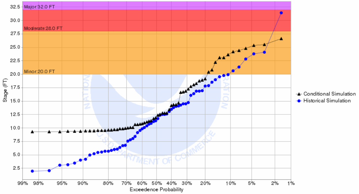
Chance of Exceeding River Stage at Wild Rice River at Hendrum (HNDM5) Forecast for the period 07/01/2018 - 09/29/2018 This is a conditional simulation based on the conditions as of 06/24/2018
