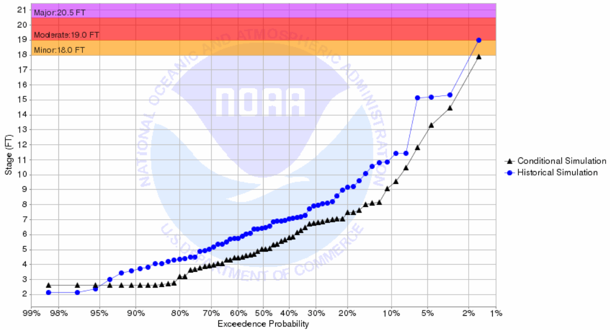
Chance of Exceeding River Stage at Pembina River at Necho (NCEN8) Forecast for the period 07/01/2018 - 09/29/2018 This is a conditional simulation based on the conditions as of 06/24/2018
