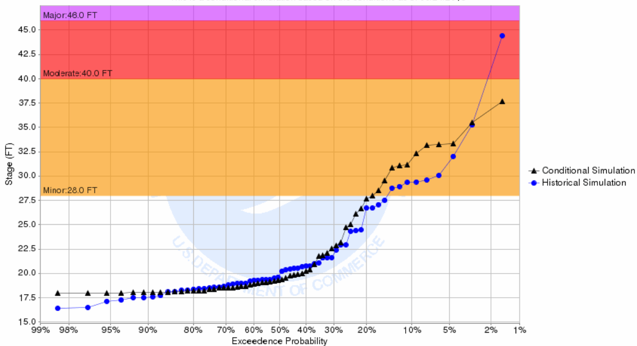
Chance of Exceeding River Stage at Red River at East Grand Forks (EGFM5) Forecast for the period 07/01/2018 - 09/29/2018 This is a conditional simulation based on the conditions as of 06/24/2018
