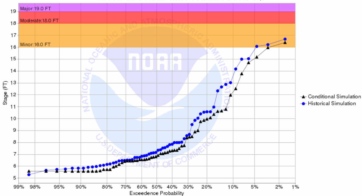
Chance of Exceeding River Stage at Roseau River at Roseau - Center St Brdg (ROSM5) Forecast for the period 07/01/2018 - 09/29/2018 This is a conditional simulation based on the conditions as of 06/24/2018
