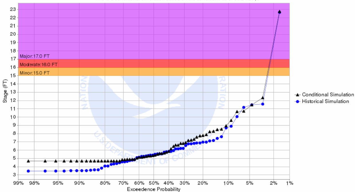
Chance of Exceeding River Stage at Sheyenne River at Valley City (VCRN8) Forecast for the period 07/01/2018 - 09/29/2018 This is a conditional simulation based on the conditions as of 06/24/2018
