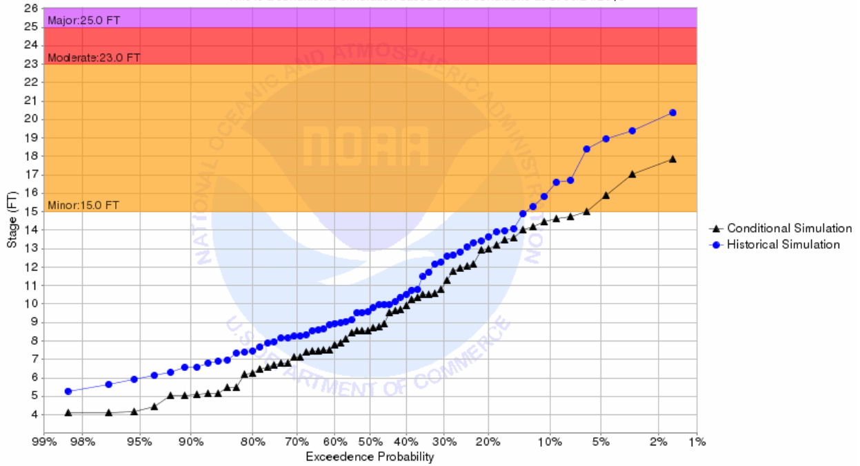
Chance of Exceeding River Stage at Red Lake River at Crookston (CRKM5) Forecast for the period 07/01/2018 - 09/29/2018 This is a conditional simulation based on the conditions as of 06/24/2018
