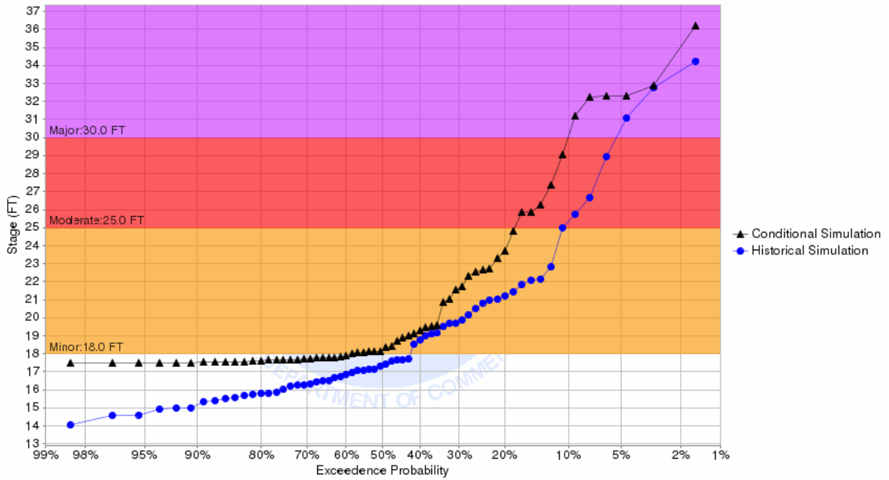
Chance of Exceeding River Stage at Red River at Fargo WTP (FGON8) Forecast for the period 07/01/2018 - 09/29/2018 This is a conditional simulation based on the conditions as of 06/24/2018
