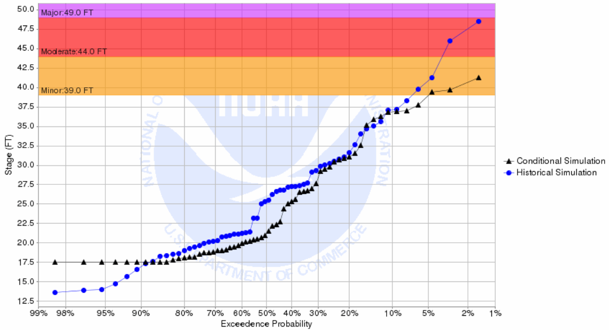
Chance of Exceeding River Stage at Red River at Pembina (PBNN8) Forecast for the period 07/01/2018 - 09/29/2018 This is a conditional simulation based on the conditions as of 06/24/2018
