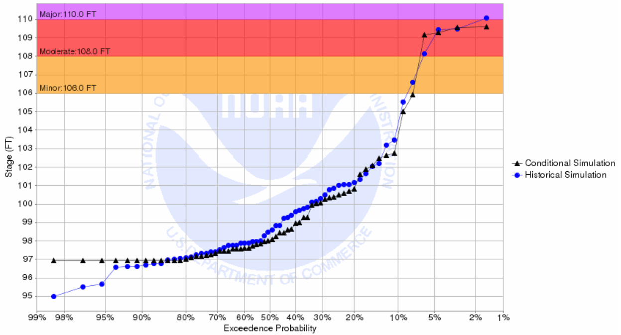
Chance of Exceeding River Stage at Snake River at Alvarado (ALVM5) Forecast for the period 07/01/2018 - 09/29/2018 This is a conditional simulation based on the conditions as of 06/24/2018
