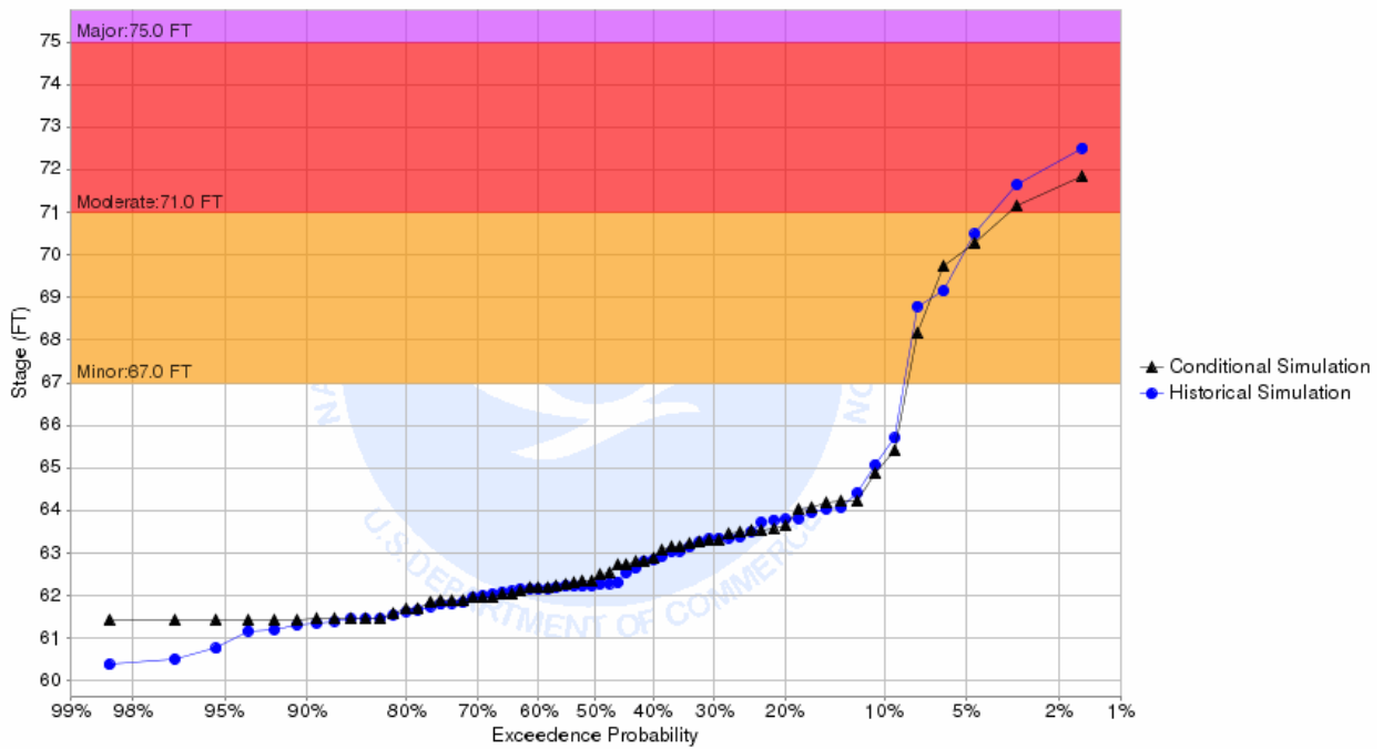
Chance of Exceeding River Stage at Snake River at Warren 3ENE-Morkassel Brdg (MKLM5) Forecast for the period 07/01/2018 - 09/29/2018 This is a conditional simulation based on the conditions as of 06/24/2018
