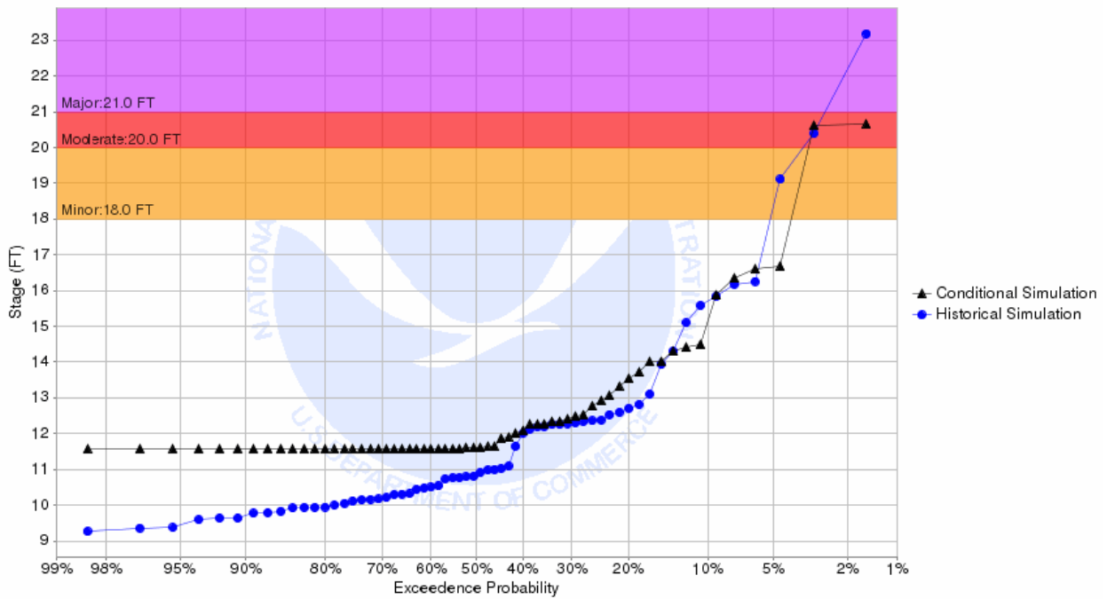
Chance of Exceeding River Stage at Sheyenne River Diversion at West Fargo (WFON8) Forecast for the period 07/01/2018 - 09/29/2018 This is a conditional simulation based on the conditions as of 06/24/2018
