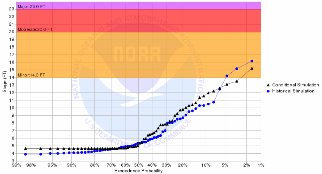
Chance of Exceeding River Stage at Marsh River at Shelly 4SE (SHYM5) Forecast for the period 07/01/2018 - 09/29/2018 This is a conditional simulation based on the conditions as of 06/24/2018
