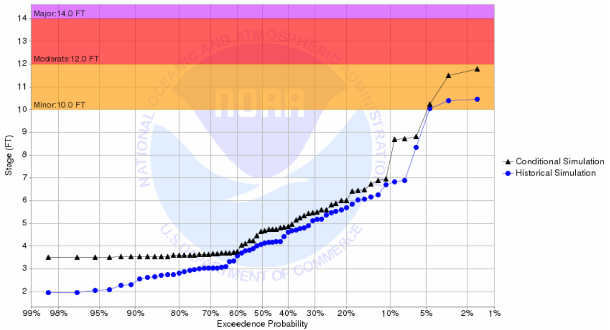
Chance of Exceeding River Stage at Wild Rice River at Twin Valley 1NE (TWVM5) Forecast for the period 07/01/2018 - 09/29/2018 This is a conditional simulation based on the conditions as of 06/24/2018
