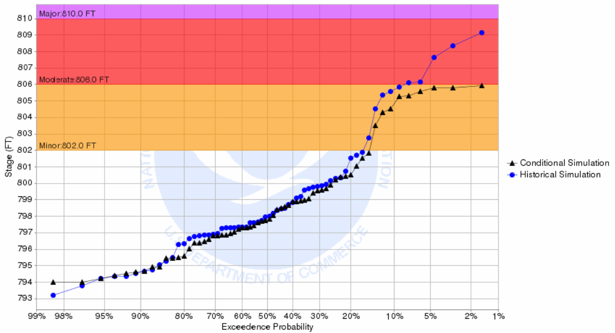
Chance of Exceeding River Stage at Two Rivers River at Hallock (HLLM5) Forecast for the period 07/01/2018 - 09/29/2018 This is a conditional simulation based on the conditions as of 06/24/2018
