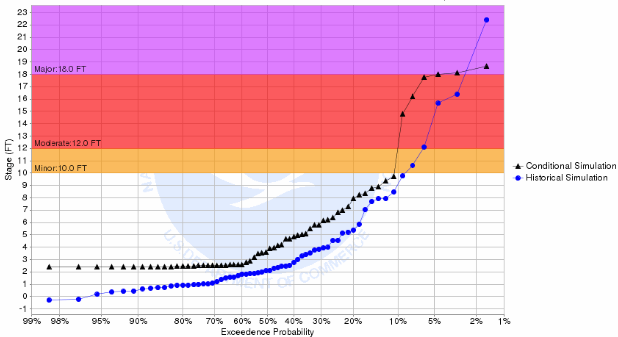
Chance of Exceeding River Stage at Wild Rice River at Abercrombie 3NW (ABRN8) Forecast for the period 07/01/2018 - 09/29/2018 This is a conditional simulation based on the conditions as of 06/24/2018
