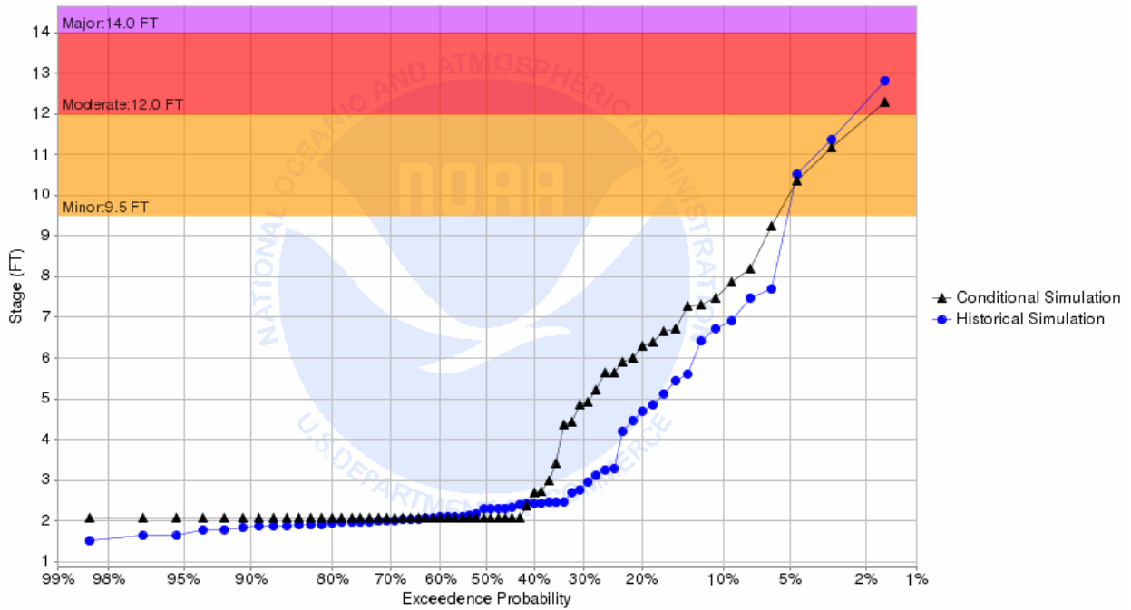
Chance of Exceeding River Stage at Maple River at Enderlin 1E (ENDN8) Forecast for the period 07/01/2018 - 09/29/2018 This is a conditional simulation based on the conditions as of 06/24/2018
