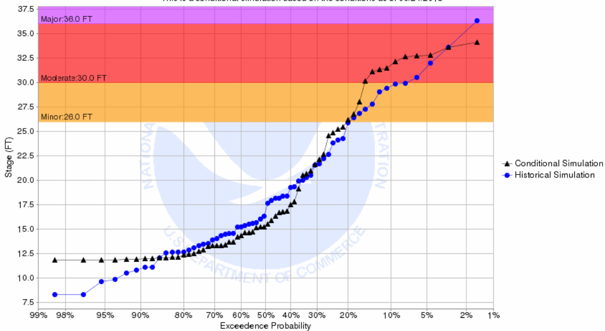
Chance of Exceeding River Stage at Red River at Oslo (OSLM5) Forecast for the period 07/01/2018 - 09/29/2018 This is a conditional simulation based on the conditions as of 06/24/2018
