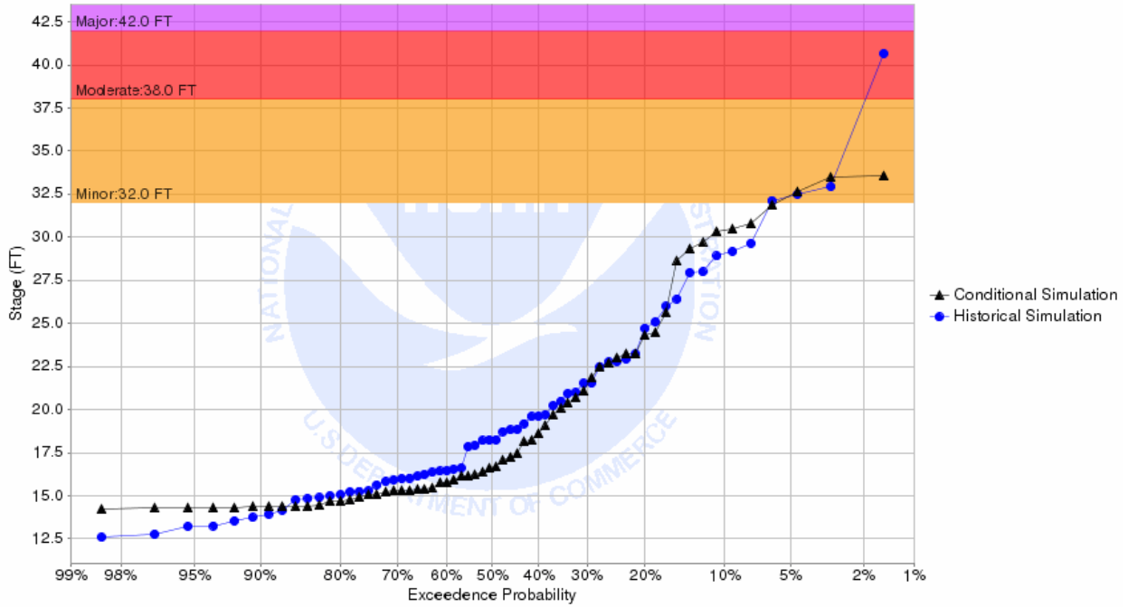
Chance of Exceeding River Stage at Red River at Drayton 2NE - Hwy 66 Brdg (DRTN8) Forecast for the period 07/01/2018 - 09/29/2018 This is a conditional simulation based on the conditions as of 06/24/2018
