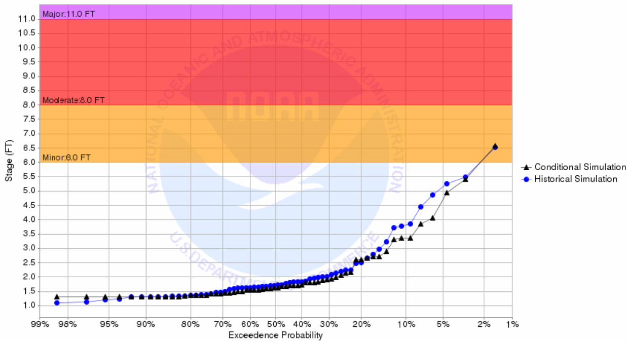
Chance of Exceeding River Stage at Forest River at Minto (MTON8) Forecast for the period 07/01/2018 - 09/29/2018 This is a conditional simulation based on the conditions as of 06/24/2018
