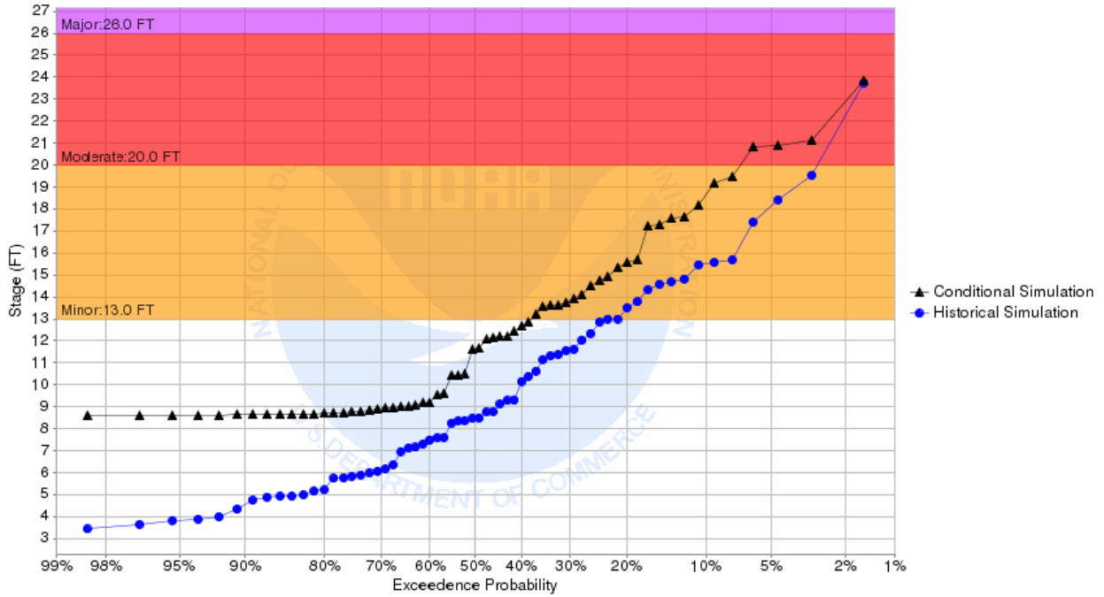
Chance of Exceeding River Stage at Buffalo River at Dilworth 7NNE (DILM5) Forecast for the period 07/01/2018 - 09/29/2018 This is a conditional simulation based on the conditions as of 06/24/2018
