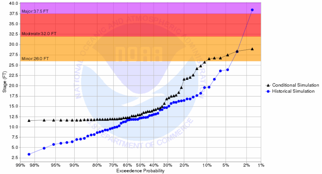
Chance of Exceeding River Stage at Red River at Hillsboro 11ESE (Halstad MN) (HILN8) Forecast for the period 07/01/2018 - 09/29/2018 This is a conditional simulation based on the conditions as of 06/24/2018
