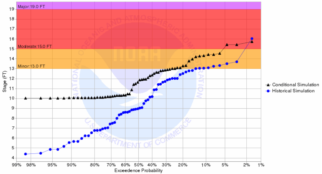
Chance of Exceeding River Stage at South Branch Buffalo River at Sabin 1ESE (SABM5) Forecast for the period 07/01/2018 - 09/29/2018 This is a conditional simulation based on the conditions as of 06/24/2018
