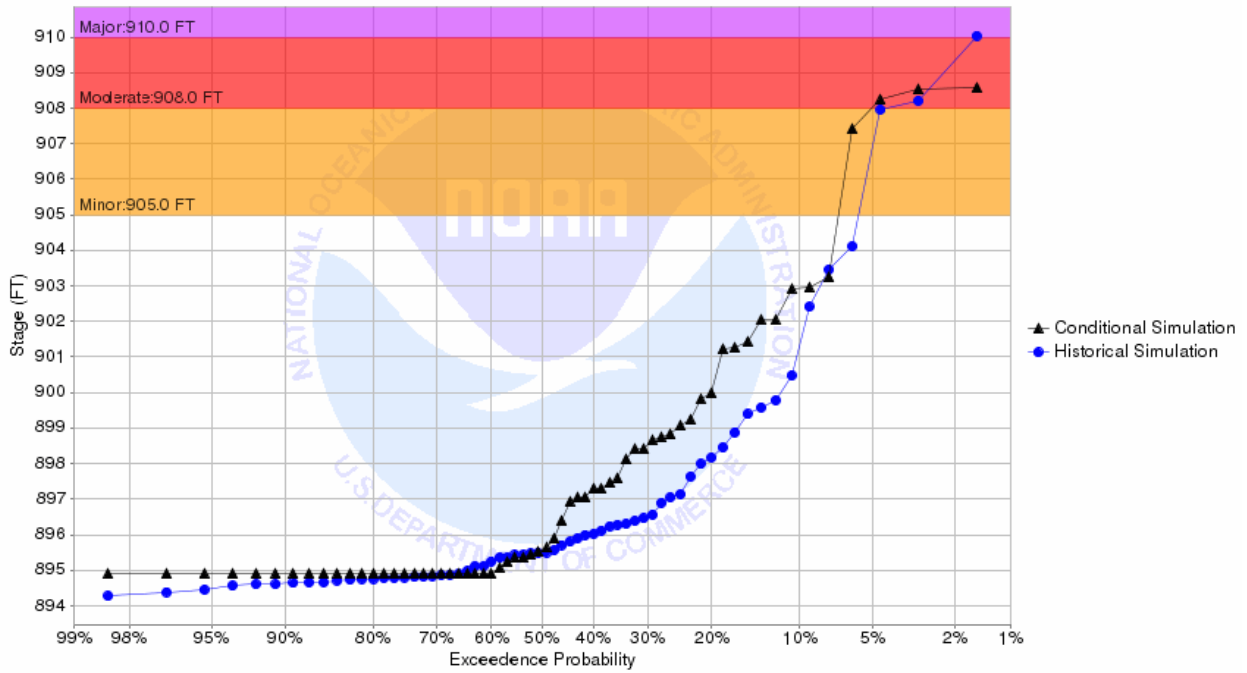
Chance of Exceeding River Stage at Maple River at Mapleton 3SW (MPLN8) Forecast for the period 07/01/2018 - 09/29/2018 This is a conditional simulation based on the conditions as of 06/24/2018
