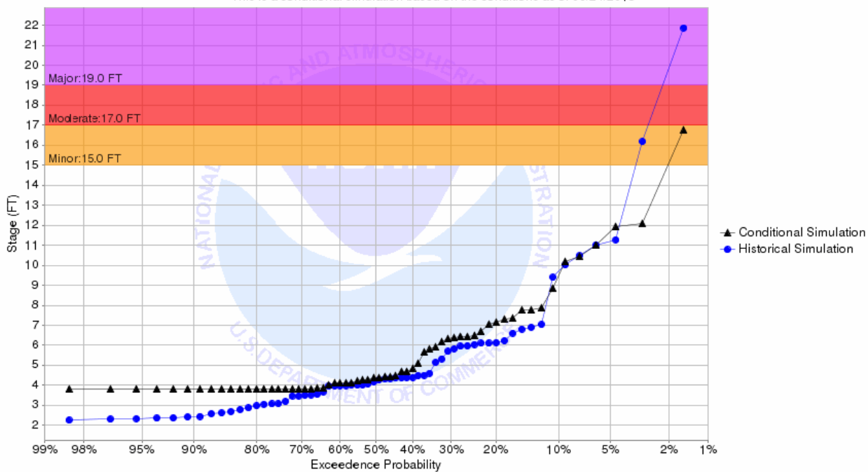
Chance of Exceeding River Stage at Sheyenne River at Lisbon (LBNN8) Forecast for the period 07/01/2018 - 09/29/2018 This is a conditional simulation based on the conditions as of 06/24/2018
