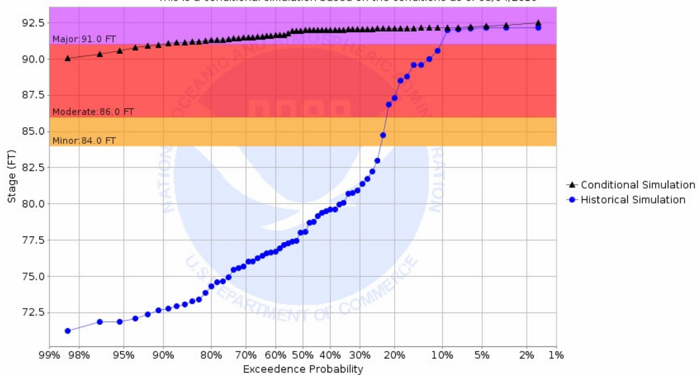
Chance of Exceeding River Stage at Sheyenne River at Harwood (HWDN8) Forecast for the period 03/11/2019 - 06/09/2019 This is a conditional simulation based on the conditions as of 03/04/2019
