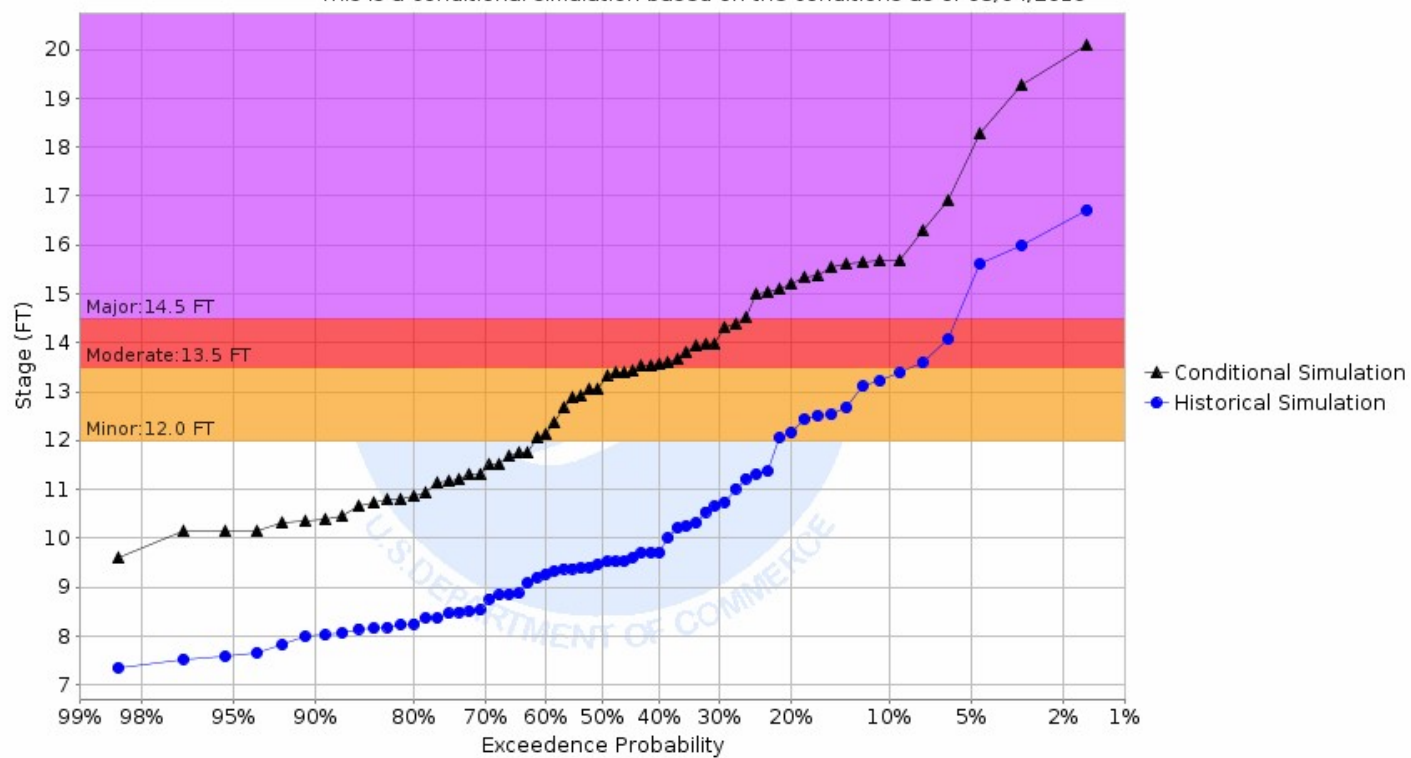
Chance of Exceeding River Stage at Park River at Grafton (GRNN8) Forecast for the period 03/11/2019 - 06/09/2019 This is a conditional simulation based on the conditions as of 03/04/2019
