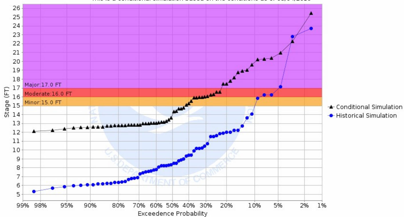
Chance of Exceeding River Stage at Sheyenne River at Valley City (VCRN8) Forecast for the period 03/11/2019 - 06/09/2019 This is a conditional simulation based on the conditions as of 03/04/2019
