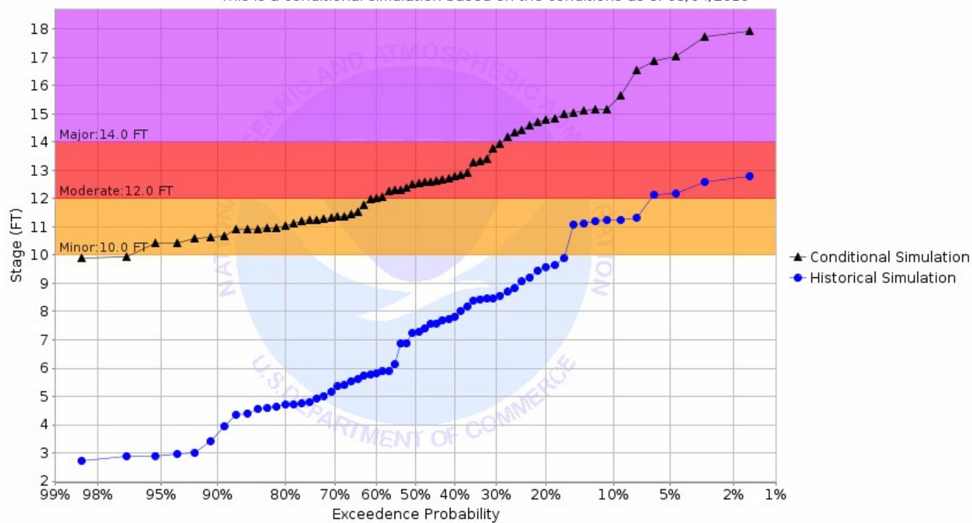
Chance of Exceeding River Stage at Wild Rice River at Twin Valley 1NE (TWVM5) Forecast for the period 03/11/2019 - 06/09/2019 This is a conditional simulation based on the conditions as of 03/04/2019
