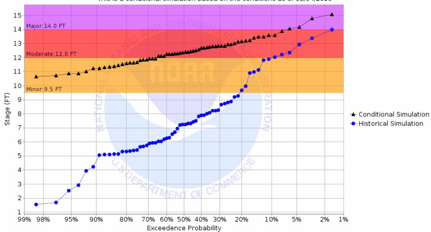
Chance of Exceeding River Stage at Maple River at Enderlin 1E (ENDN8) Forecast for the period 03/11/2019 - 06/09/2019 This is a conditional simulation based on the conditions as of 03/04/2019
