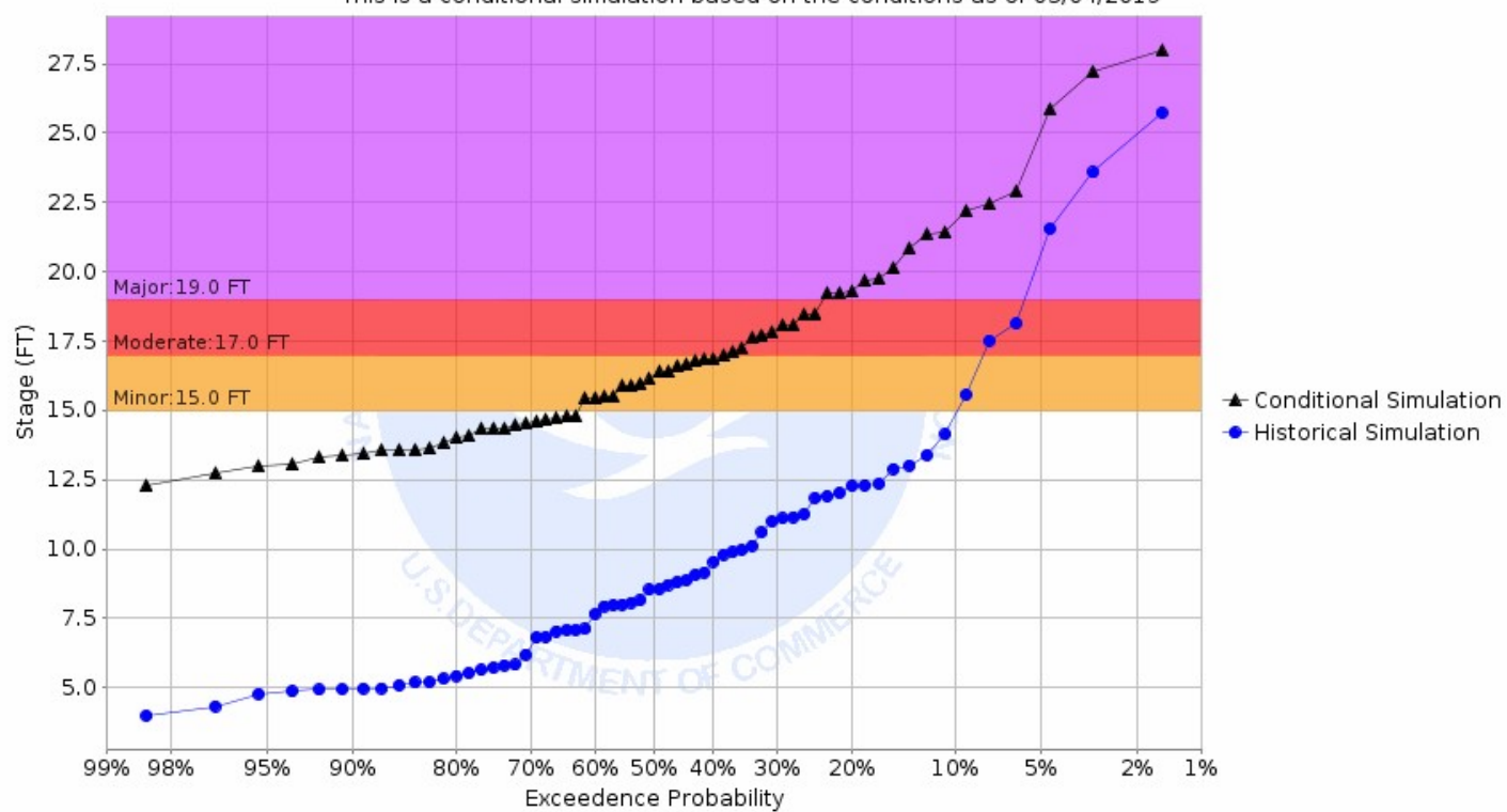
Chance of Exceeding River Stage at Sheyenne River at Lisbon (LBNN8) Forecast for the period 03/11/2019 - 06/09/2019 This is a conditional simulation based on the conditions as of 03/04/2019
