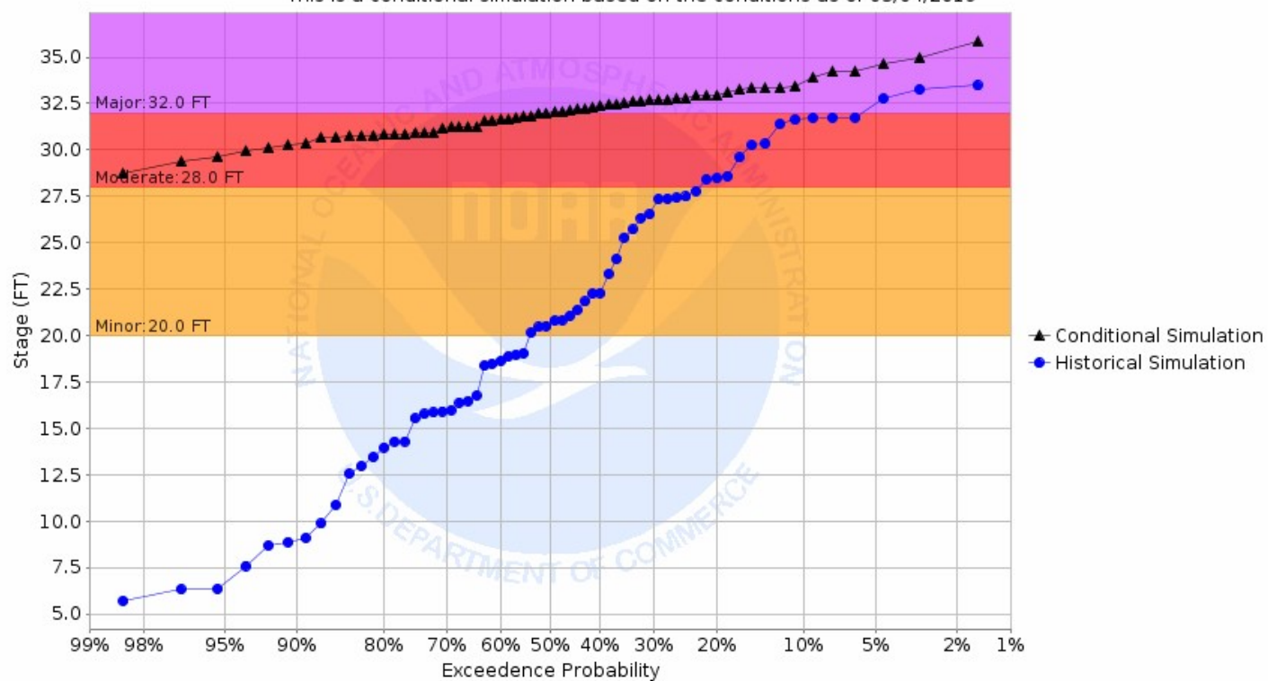
Chance of Exceeding River Stage at Wild Rice River at Hendrum (HNDM5) Forecast for the period 03/11/2019 - 06/09/2019 This is a conditional simulation based on the conditions as of 03/04/2019
