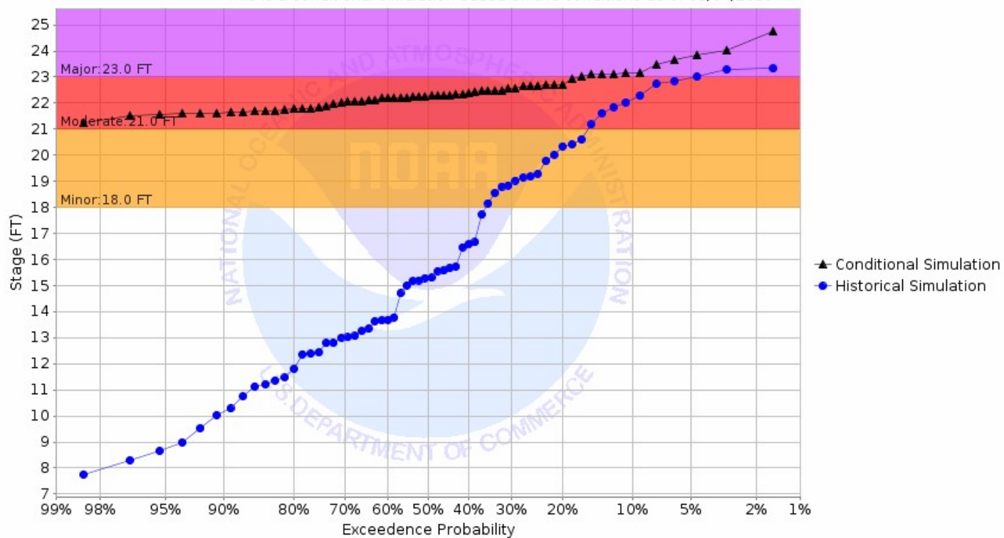
Chance of Exceeding River Stage at Maple River at Mapleton 3SW (MPLN8) Forecast for the period 03/11/2019 - 06/09/2019 This is a conditional simulation based on the conditions as of 03/04/2019
