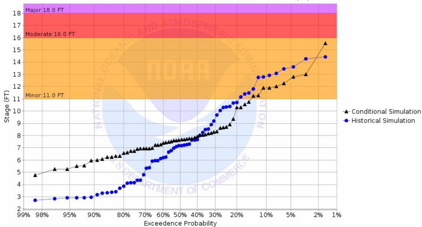
Chance of Exceeding River Stage at Pembina River at Walhalla (WLHN8) Forecast for the period 03/11/2019 - 06/09/2019 This is a conditional simulation based on the conditions as of 03/04/2019
