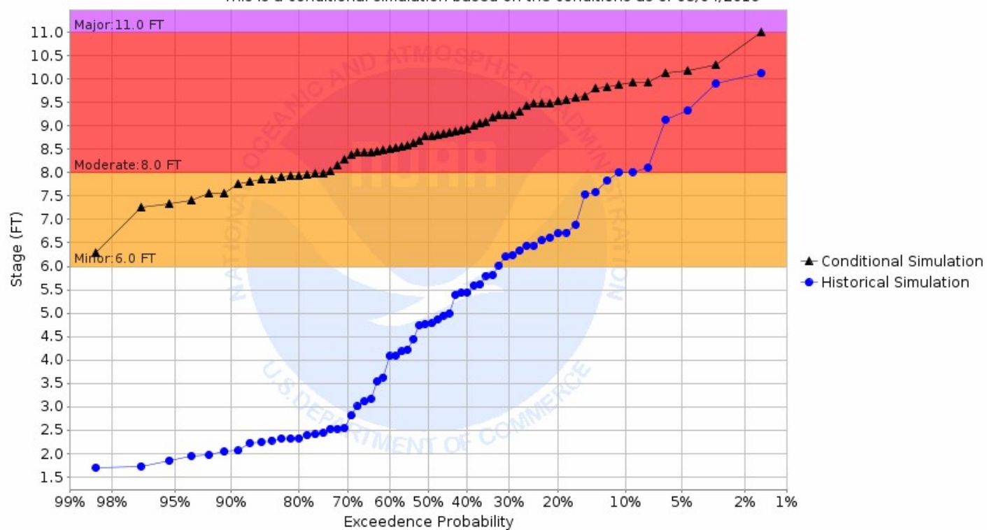
Chance of Exceeding River Stage at Forest River at Minto (MTON8) Forecast for the period 03/11/2019 - 06/09/2019 This is a conditional simulation based on the conditions as of 03/04/2019
