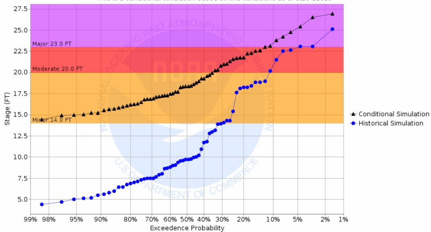
Chance of Exceeding River Stage at Marsh River at Shelly 4SE (SHYM5) Forecast for the period 03/11/2019 - 06/09/2019 This is a conditional simulation based on the conditions as of 03/04/2019
