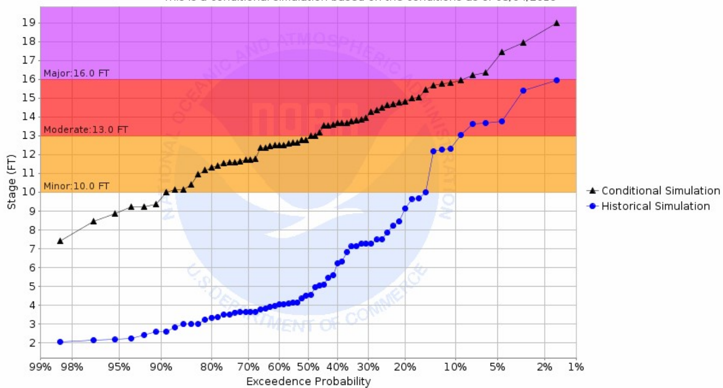
Chance of Exceeding River Stage at Goose River at Hillsboro (HGRN8) Forecast for the period 03/11/2019 - 06/09/2019 This is a conditional simulation based on the conditions as of 03/04/2019
