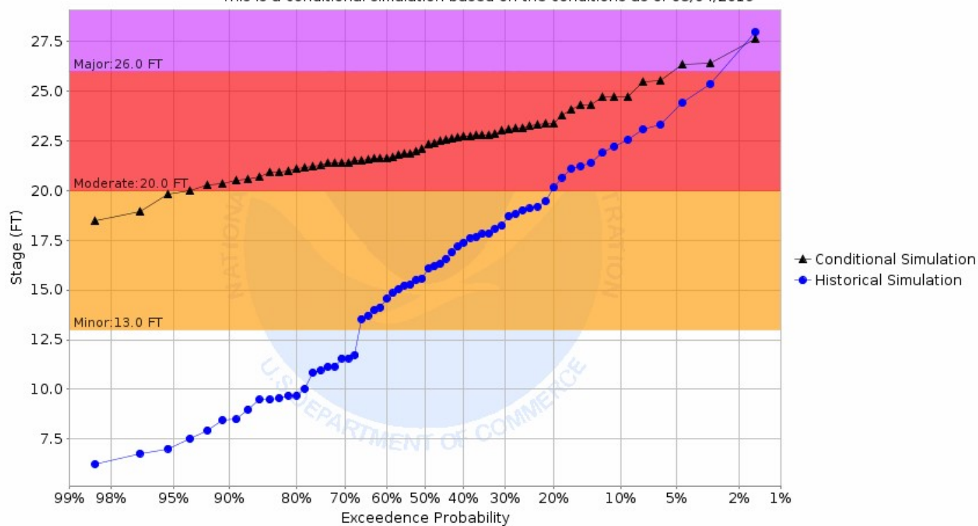
Chance of Exceeding River Stage at Buffalo River at Dilworth 7NE (DILM5) Forecast for the period 03/11/2019 - 06/09/2019 This is a conditional simulation based on the conditions as of 03/04/2019
