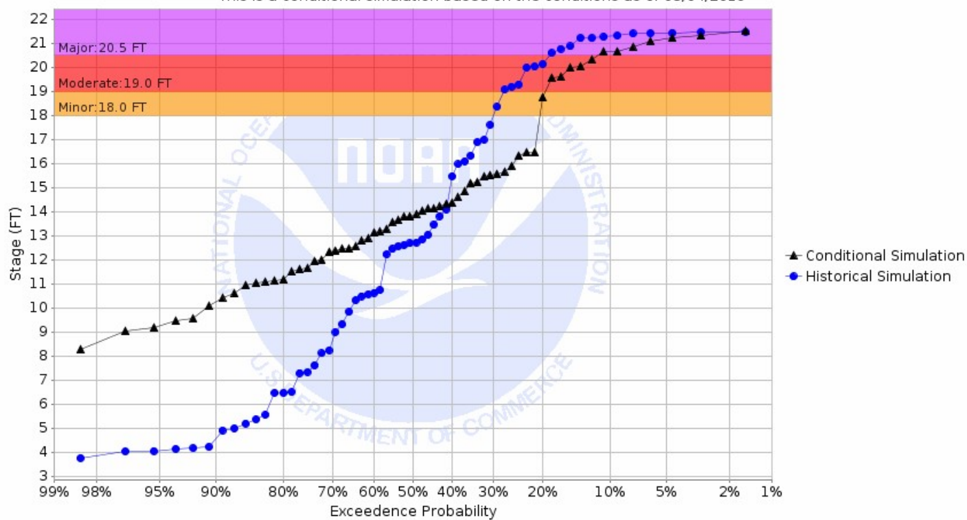
Chance of Exceeding River Stage at Pembina River at Necho (NCEN8) Forecast for the period 03/11/2019 - 06/09/2019 This is a conditional simulation based on the conditions as of 03/04/2019
