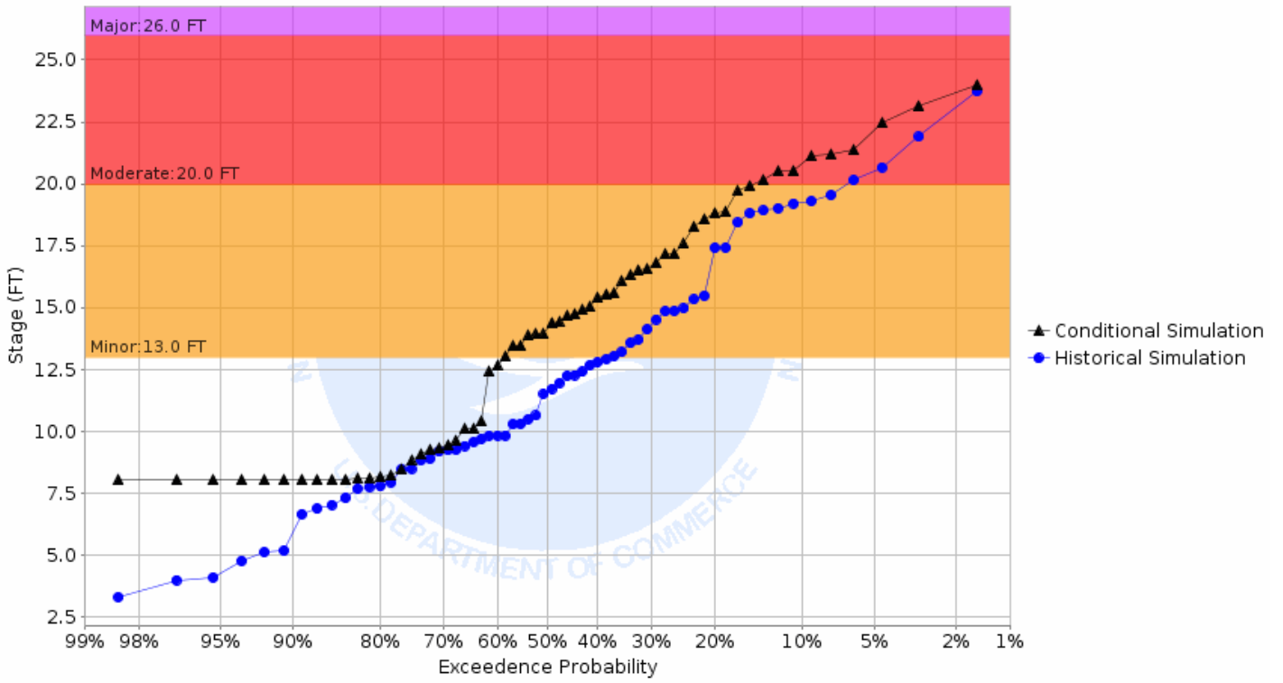
Chance of Exceeding River Stage at Buffalo River at Dilworth 7NE (DILM5) Forecast for the period 05/06/2019 - 07/28/2019 This is a conditional simulation based on the conditions as of 04/22/2019
