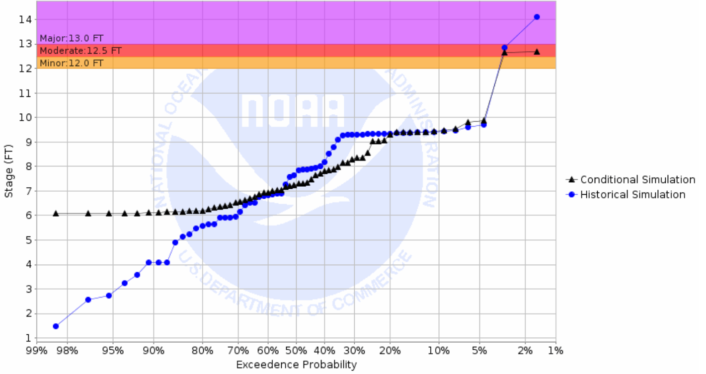
Chance of Exceeding River Stage at Red Lake River at High Landing (HIGM5) Forecast for the period 05/06/2019 - 07/28/2019 This is a conditional simulation based on the conditions as of 04/22/2019
