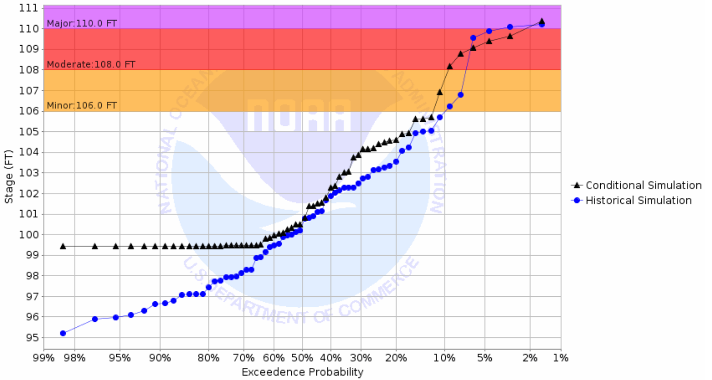
Chance of Exceeding River Stage at Snake River at Alvarado (ALVM5) Forecast for the period 05/06/2019 - 07/28/2019 This is a conditional simulation based on the conditions as of 04/22/2019
