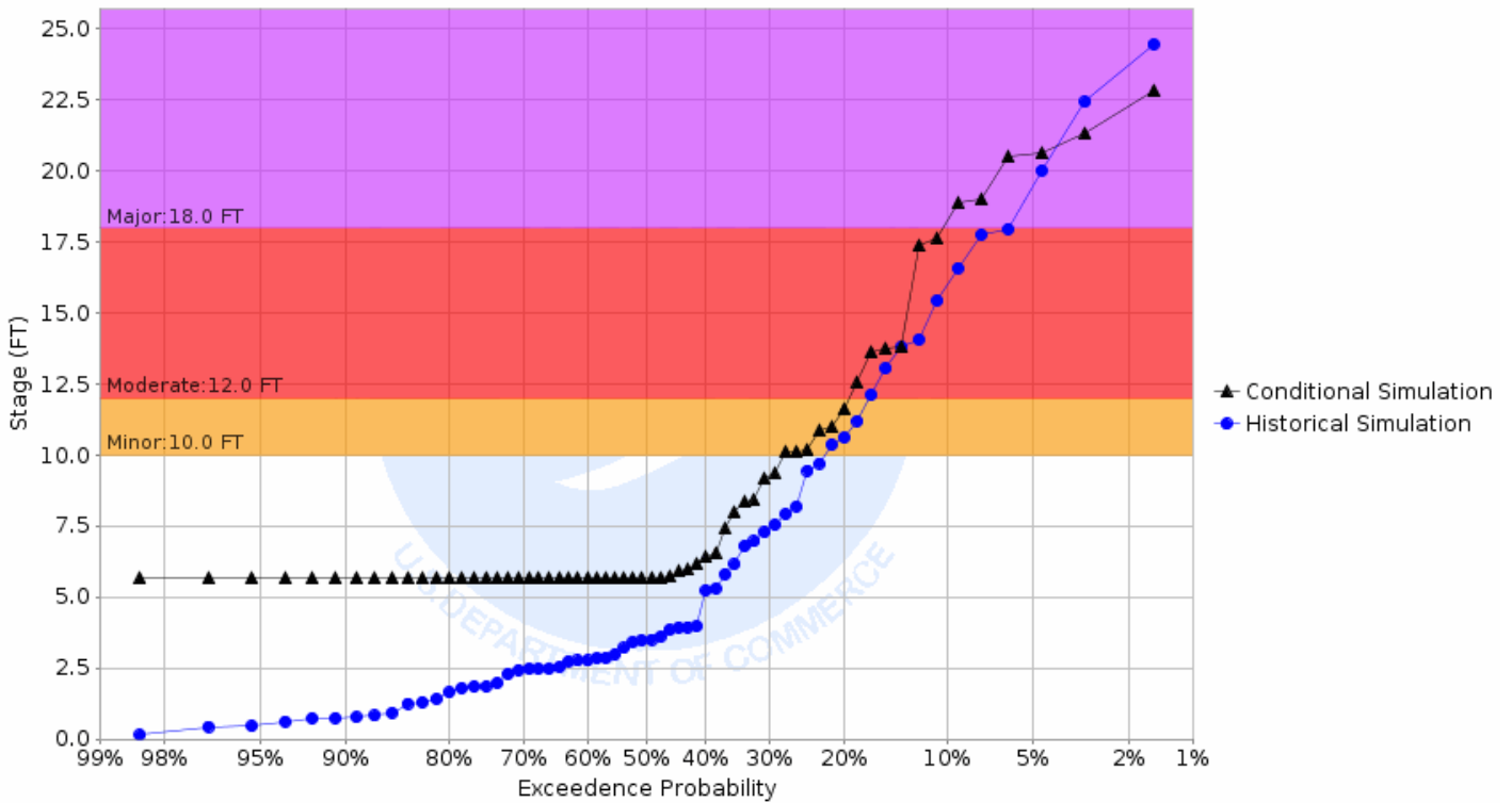
Chance of Exceeding River Stage at Wild Rice River at Abercrombie 2WNW (ABRN8) Forecast for the period 05/06/2019 - 07/28/2019 This is a conditional simulation based on the conditions as of 04/22/2019
