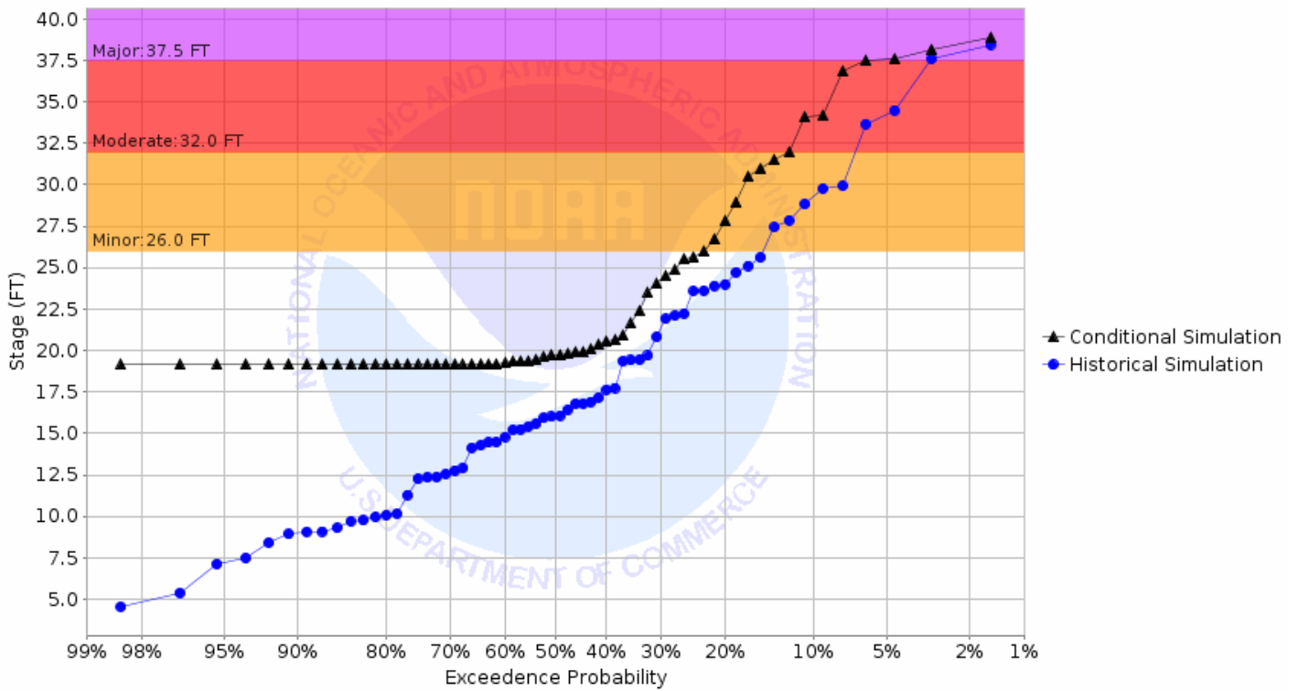
Chance of Exceeding River Stage at Red River of the North at Hillsboro 11ESE (Halstad MN) (HILN8) Forecast for the period 05/06/2019 - 07/28/2019 This is a conditional simulation based on the conditions as of 04/22/2019
