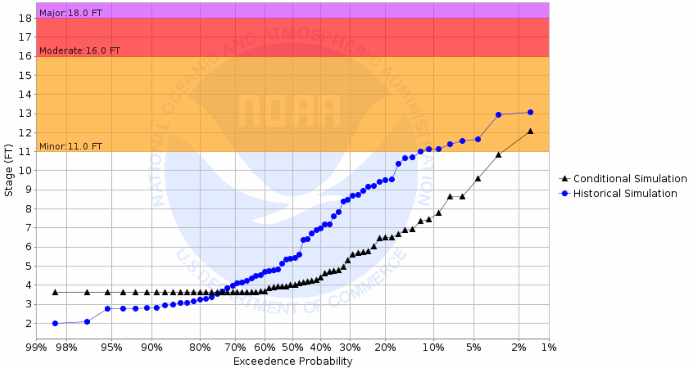
Chance of Exceeding River Stage at Pembina River at Walhalla (WLHN8) Forecast for the period 05/06/2019 - 07/28/2019 This is a conditional simulation based on the conditions as of 04/22/2019
