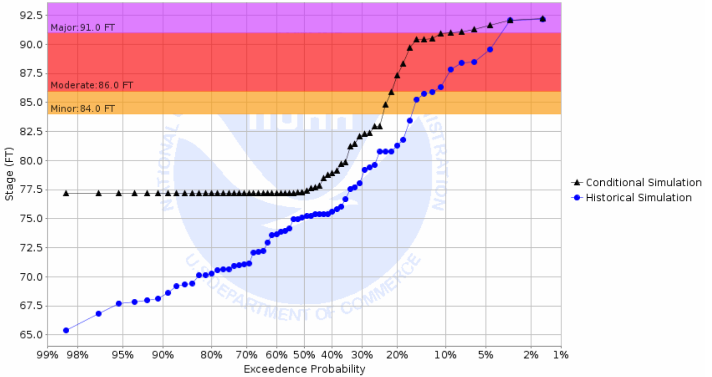
Chance of Exceeding River Stage at Sheyenne River at Harwood (HWDN8) Forecast for the period 05/06/2019 - 07/28/2019 This is a conditional simulation based on the conditions as of 04/22/2019
