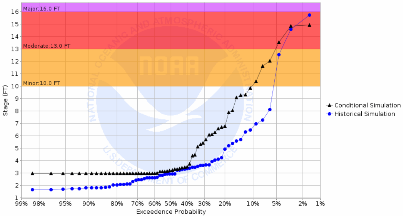
Chance of Exceeding River Stage at Goose River at Hillsboro (HGRN8) Forecast for the period 05/06/2019 - 07/28/2019 This is a conditional simulation based on the conditions as of 04/22/2019
