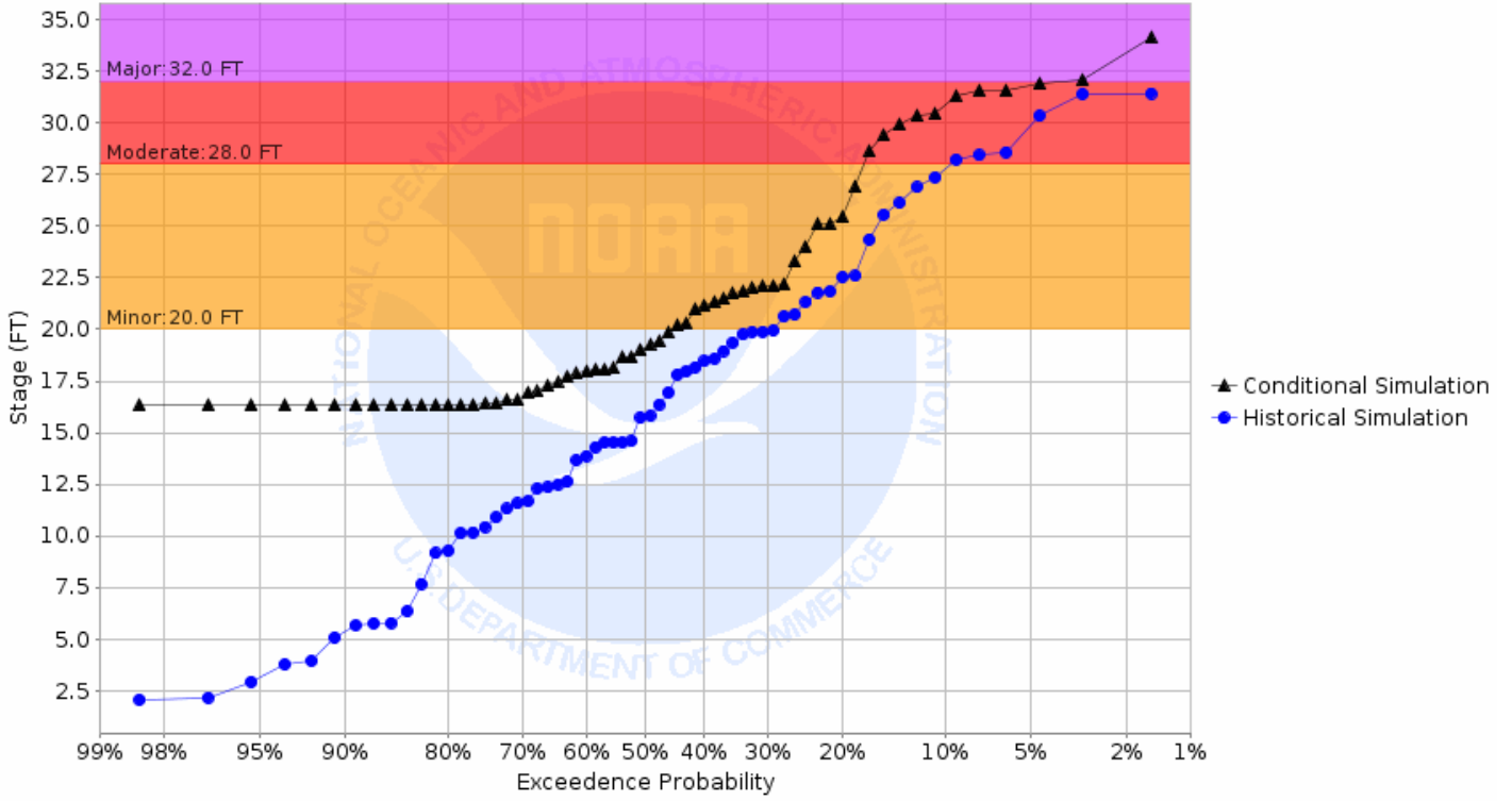
Chance of Exceeding River Stage at Wild Rice River at Hendrum (HNDM5) Forecast for the period 05/06/2019 - 07/28/2019 This is a conditional simulation based on the conditions as of 04/22/2019
