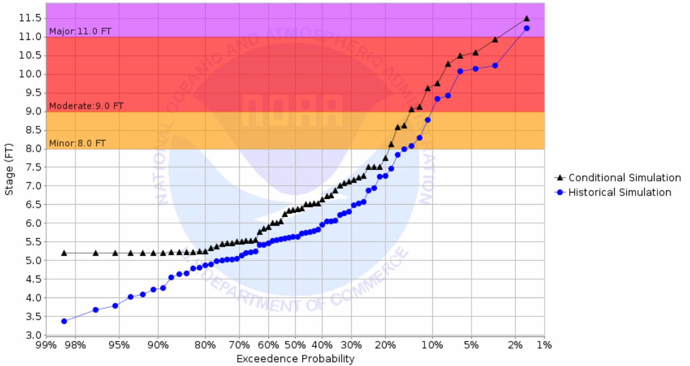
Chance of Exceeding River Stage at Buffalo River at Hawley 2SW (HWYM5) Forecast for the period 05/06/2019 - 07/28/2019 This is a conditional simulation based on the conditions as of 04/22/2019
