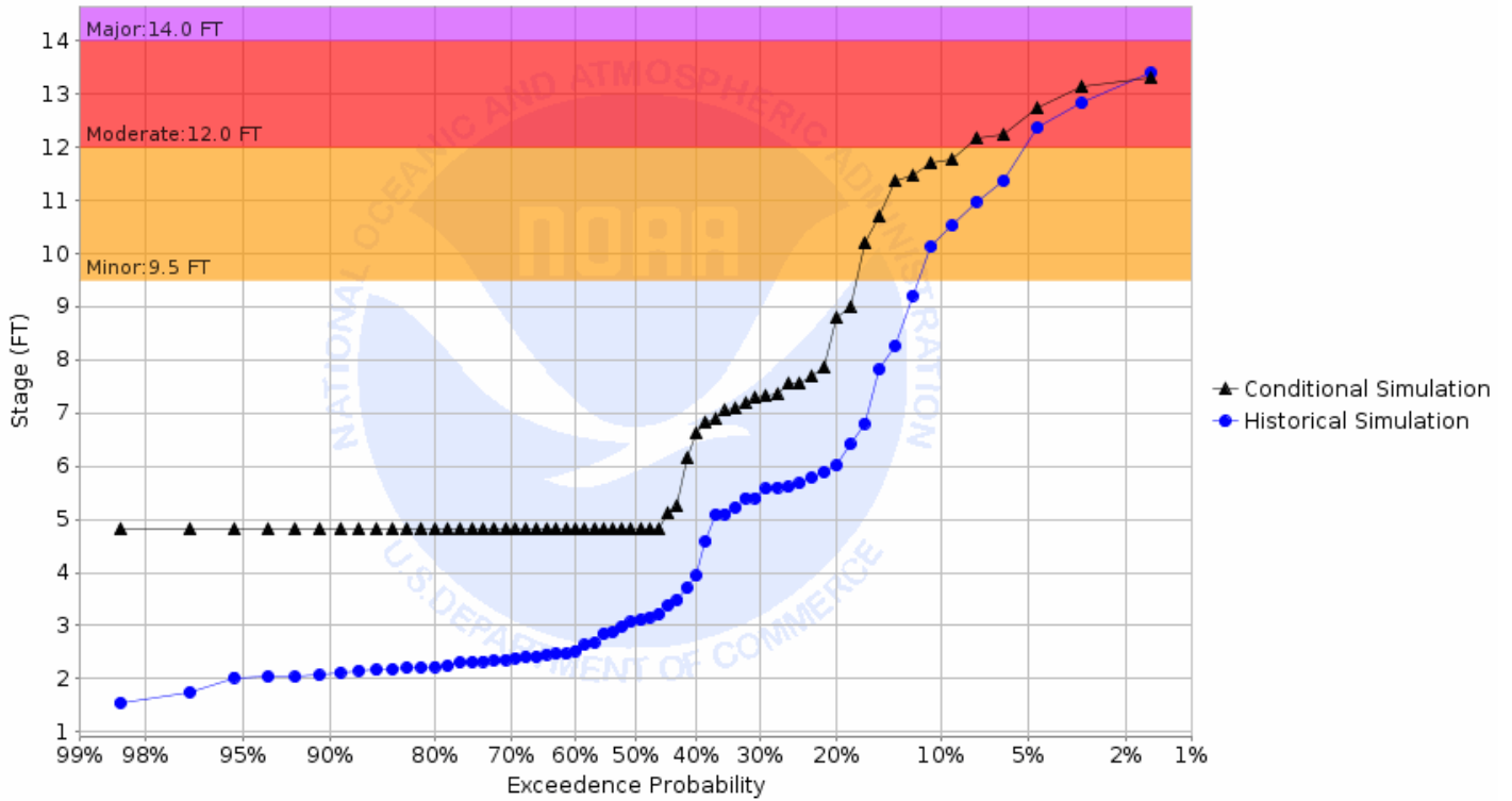
Chance of Exceeding River Stage at Maple River at Enderlin 1E (ENDN8) Forecast for the period 05/06/2019 - 07/28/2019 This is a conditional simulation based on the conditions as of 04/22/2019
