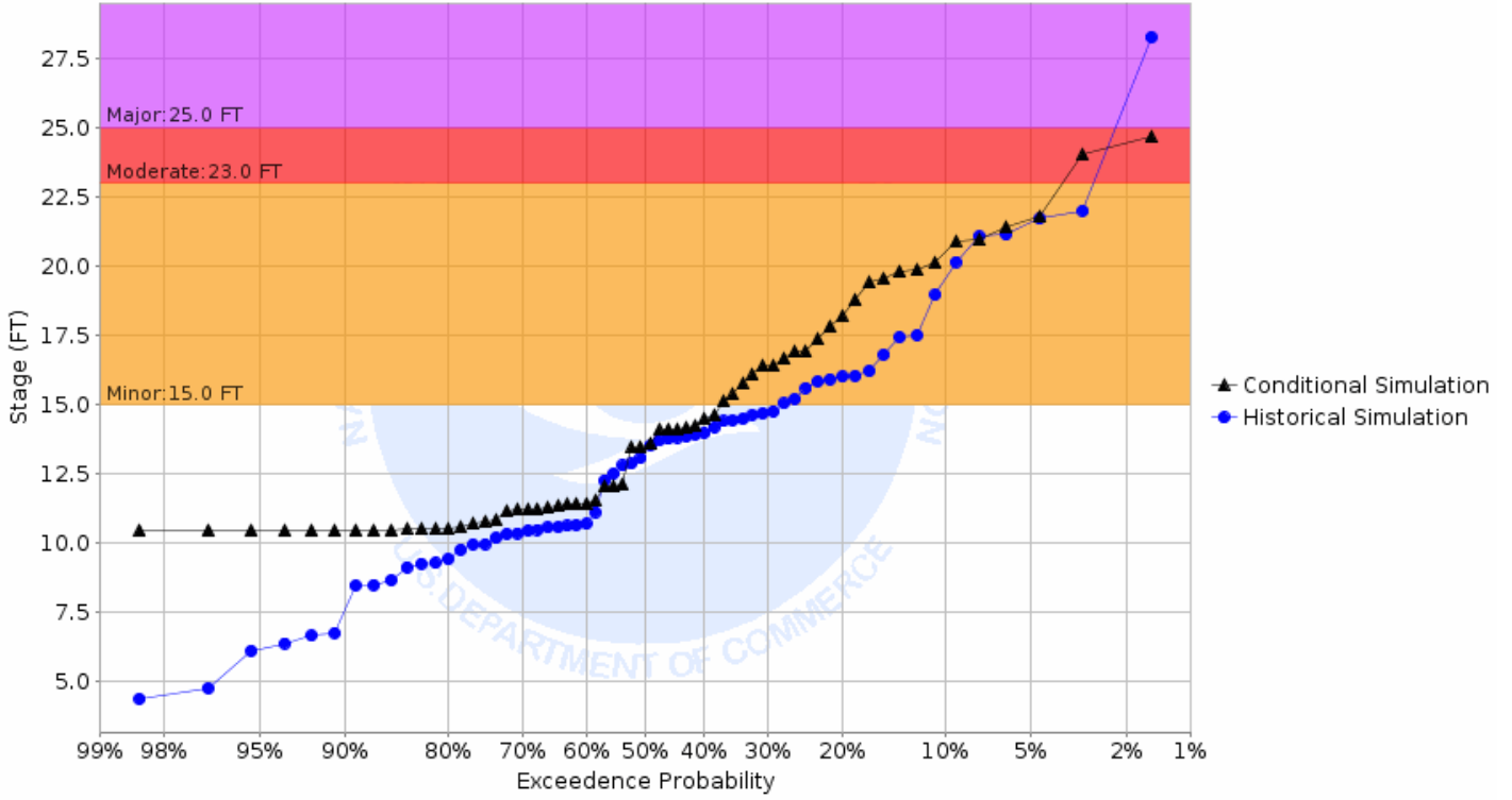
Chance of Exceeding River Stage at Red Lake River at Crookston (CRKM5) Forecast for the period 05/06/2019 - 07/28/2019 This is a conditional simulation based on the conditions as of 04/22/2019
