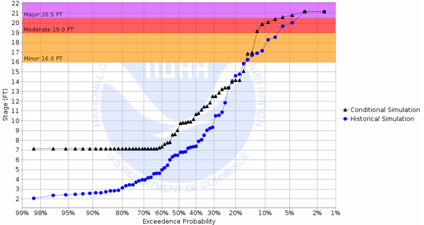
Chance of Exceeding River Stage at Sheyenne River at Kindred 2SE (KNDN8) Forecast for the period 05/06/2019 - 07/28/2019 This is a conditional simulation based on the conditions as of 04/22/2019
