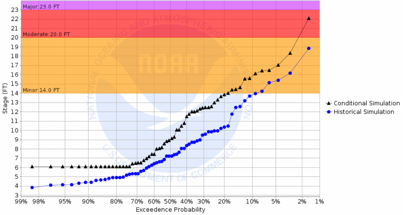
Chance of Exceeding River Stage at Marsh River at Shelly 4SE (SHYM5) Forecast for the period 05/06/2019 - 07/28/2019 This is a conditional simulation based on the conditions as of 04/22/2019
