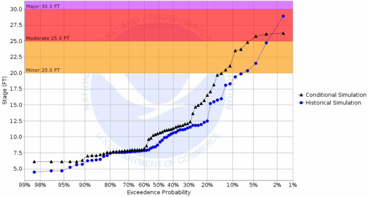
Chance of Exceeding River Stage at Sand Hill River at Climax (CLXM5) Forecast for the period 05/06/2019 - 07/28/2019 This is a conditional simulation based on the conditions as of 04/22/2019
