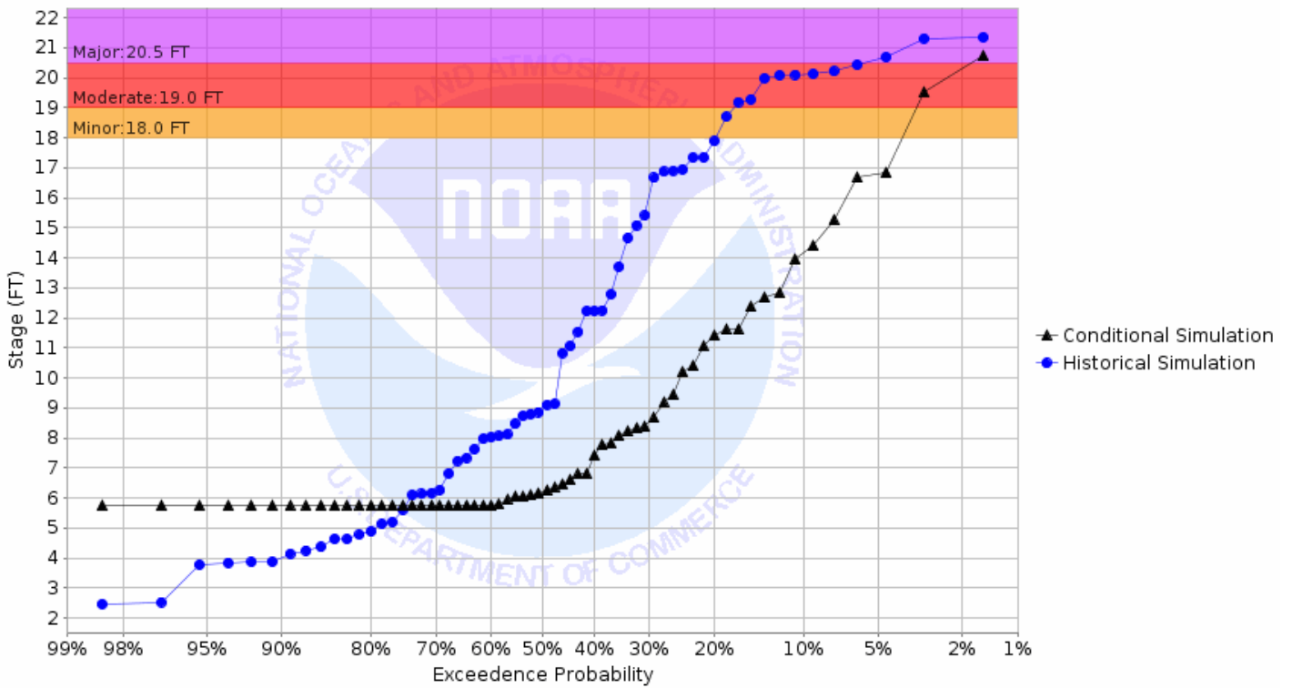
Chance of Exceeding River Stage at Pembina River at Neche (NCEN8) Forecast for the period 05/06/2019 - 07/28/2019 This is a conditional simulation based on the conditions as of 04/22/2019
