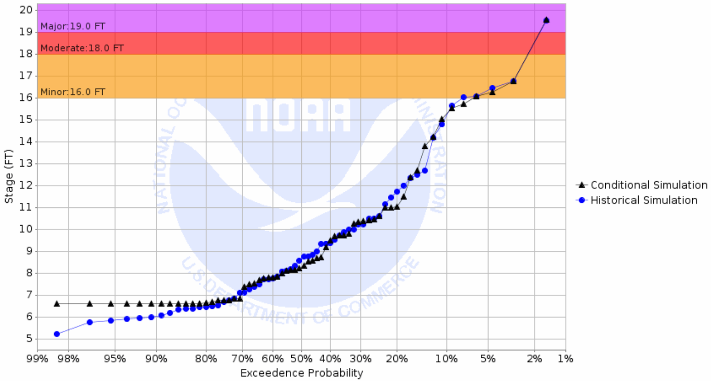
Chance of Exceeding River Stage at Roseau River at Roseau - Center St Brdg (ROSM5) Forecast for the period 05/06/2019 - 07/28/2019 This is a conditional simulation based on the conditions as of 04/22/2019
