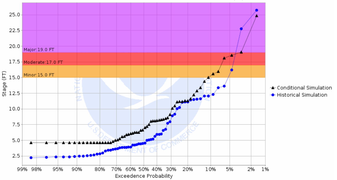
Chance of Exceeding River Stage at Sheyenne River at Lisbon (LBNN8) Forecast for the period 05/06/2019 - 07/28/2019 This is a conditional simulation based on the conditions as of 04/22/2019
