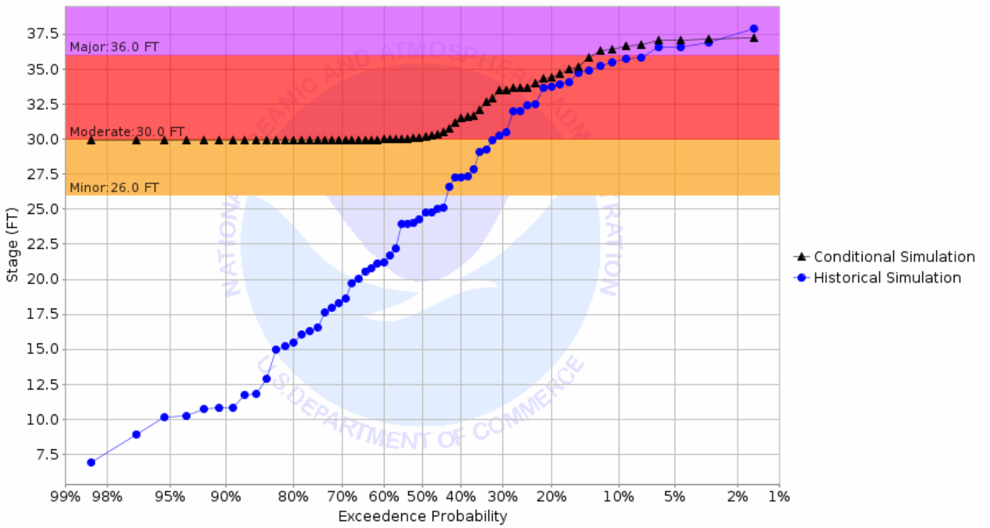
Chance of Exceeding River Stage at Red River of the North at Oslo (OSLM5) Forecast for the period 05/06/2019 - 07/28/2019 This is a conditional simulation based on the conditions as of 04/22/2019
