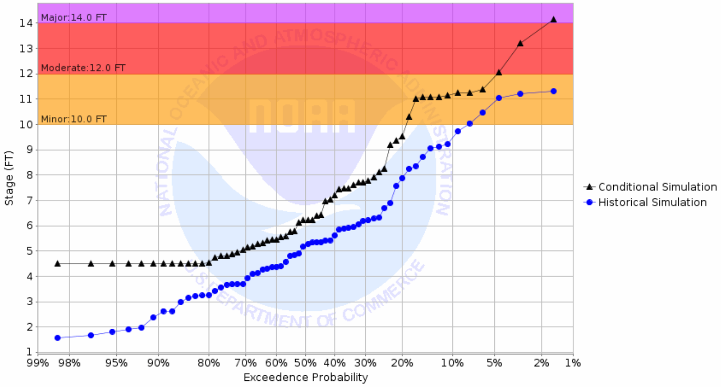
Chance of Exceeding River Stage at Wild Rice River at Twin Valley 1NE (TWVM5) Forecast for the period 05/06/2019 - 07/28/2019 This is a conditional simulation based on the conditions as of 04/22/2019
