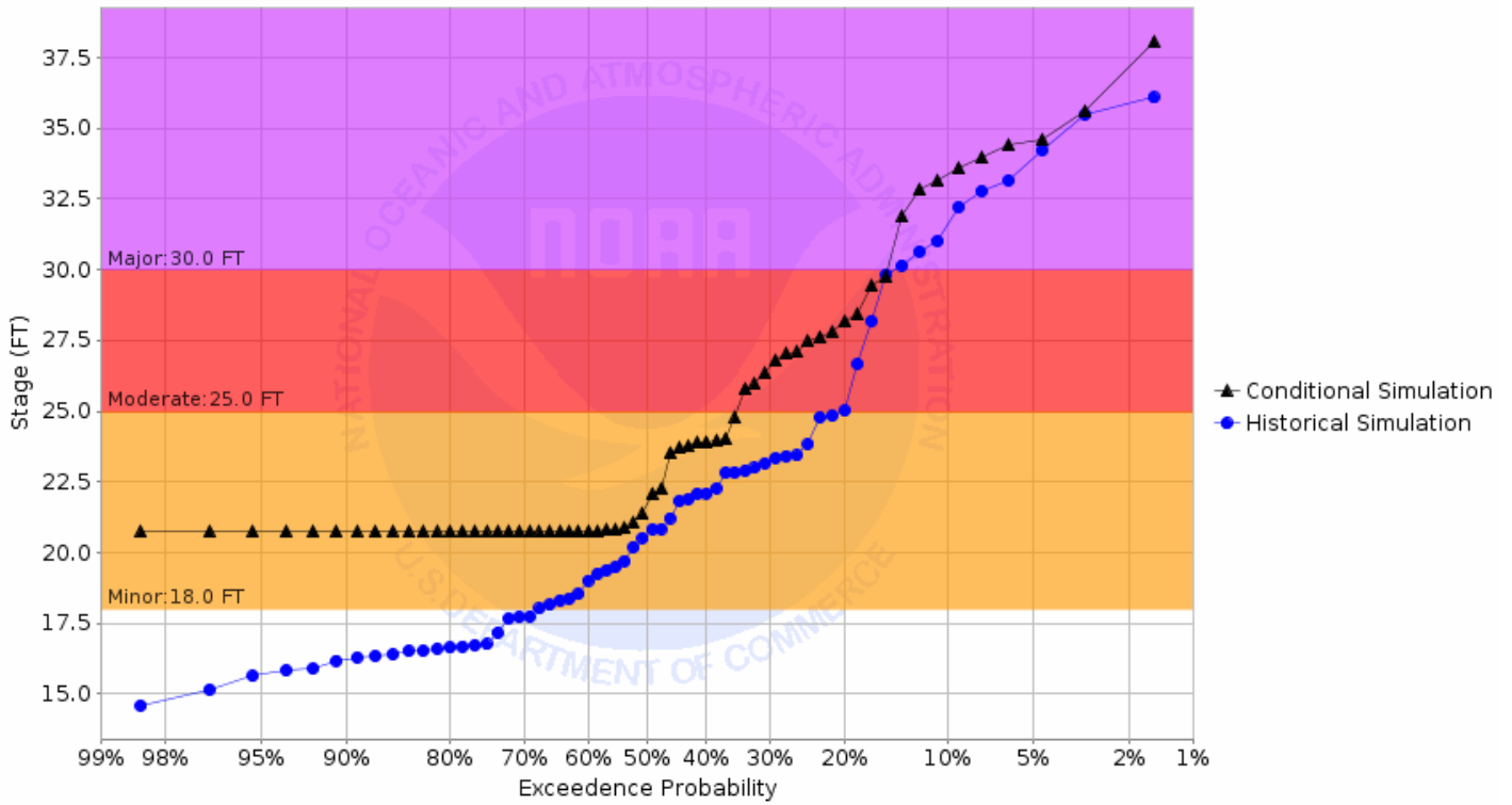
Chance of Exceeding River Stage at Red River of the North at Fargo WTP (FGON8) Forecast for the period 05/06/2019 - 07/28/2019 This is a conditional simulation based on the conditions as of 04/22/2019
