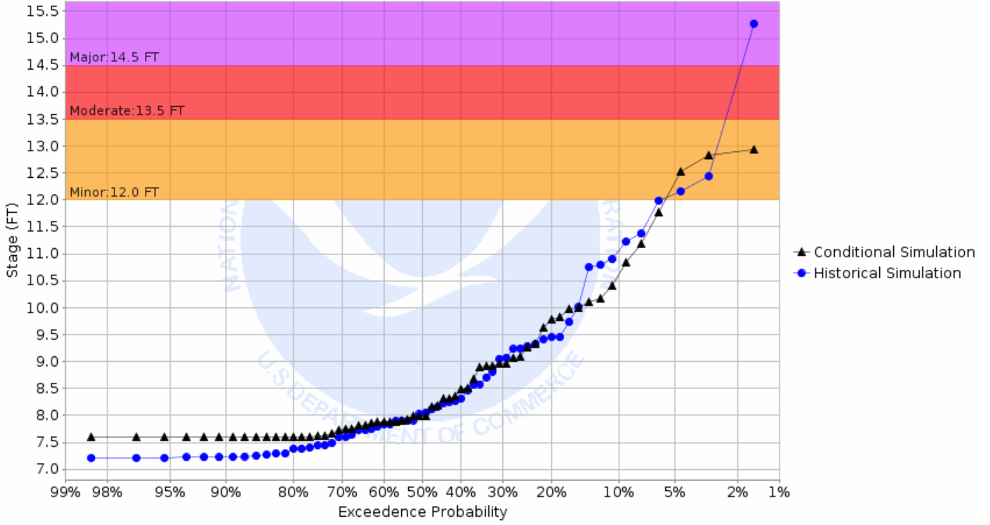
Chance of Exceeding River Stage at Park River at Grafton (GRNN8) Forecast for the period 05/06/2019 - 07/28/2019 This is a conditional simulation based on the conditions as of 04/22/2019
