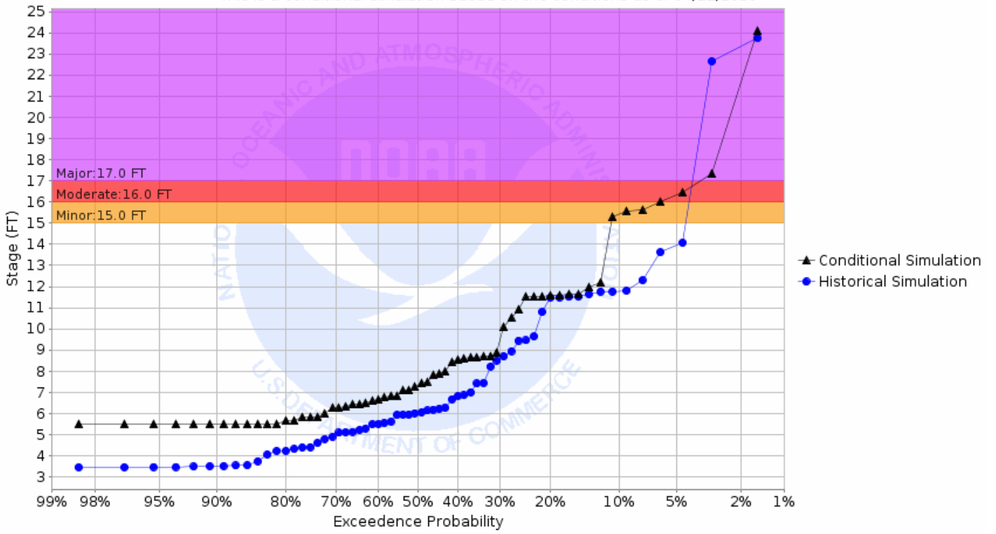
Chance of Exceeding River Stage at Sheyenne River at Valley City (VCRN8) Forecast for the period 05/06/2019 - 07/28/2019 This is a conditional simulation based on the conditions as of 04/22/2019
