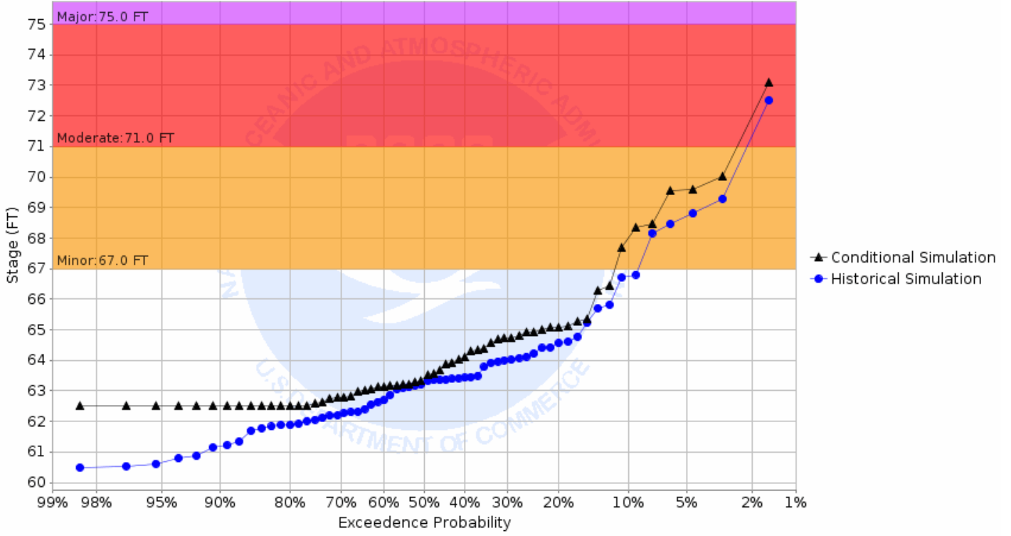
Chance of Exceeding River Stage at Snake River at Warren 3ENE-Morkassel Brdg (MKLM5) Forecast for the period 05/06/2019 - 07/28/2019 This is a conditional simulation based on the conditions as of 04/22/2019
