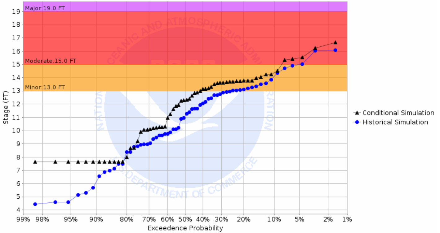
Chance of Exceeding River Stage at South Branch Buffalo River at Sabin 1E (SABM5) Forecast for the period 05/06/2019 - 07/28/2019 This is a conditional simulation based on the conditions as of 04/22/2019
