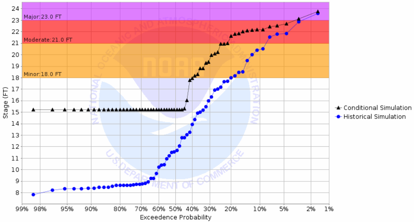
Chance of Exceeding River Stage at Maple River at Mapleton 3SW (MPLN8) Forecast for the period 05/06/2019 - 07/28/2019 This is a conditional simulation based on the conditions as of 04/22/2019
