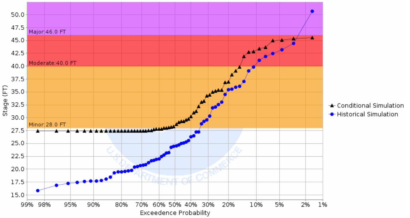
Chance of Exceeding River Stage at Red River of the North at East Grand Forks (EGFM5) Forecast for the period 05/06/2019 - 07/28/2019 This is a conditional simulation based on the conditions as of 04/22/2019
