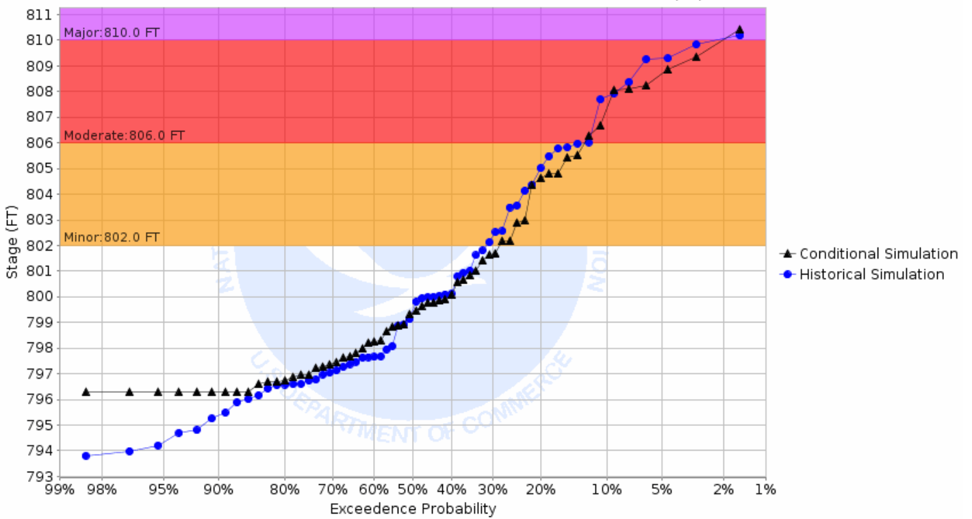
Chance of Exceeding River Stage at Two Rivers River at Hallock (HLLM5) Forecast for the period 05/06/2019 - 07/28/2019 This is a conditional simulation based on the conditions as of 04/22/2019
