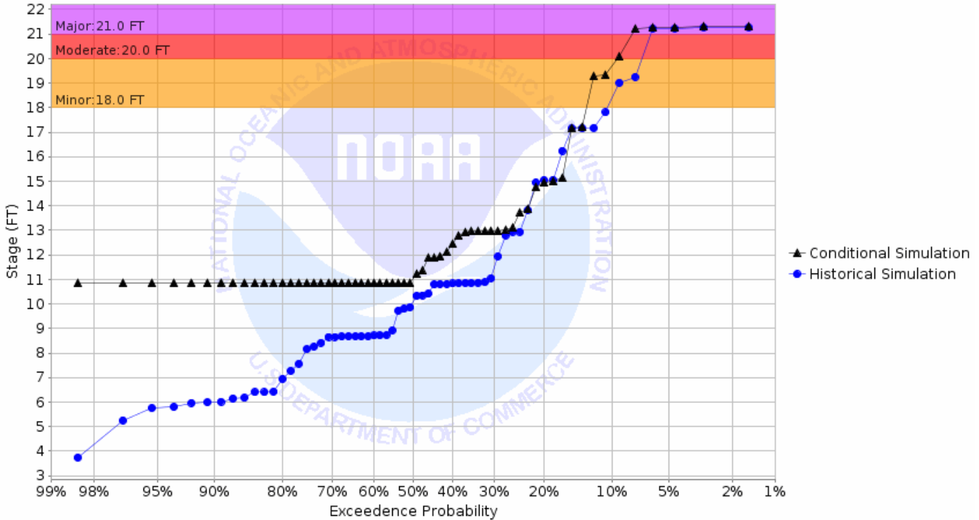
Chance of Exceeding River Stage at Sheyenne River Diversion at West Fargo (WFON8) Forecast for the period 05/06/2019 - 07/28/2019 This is a conditional simulation based on the conditions as of 04/22/2019
