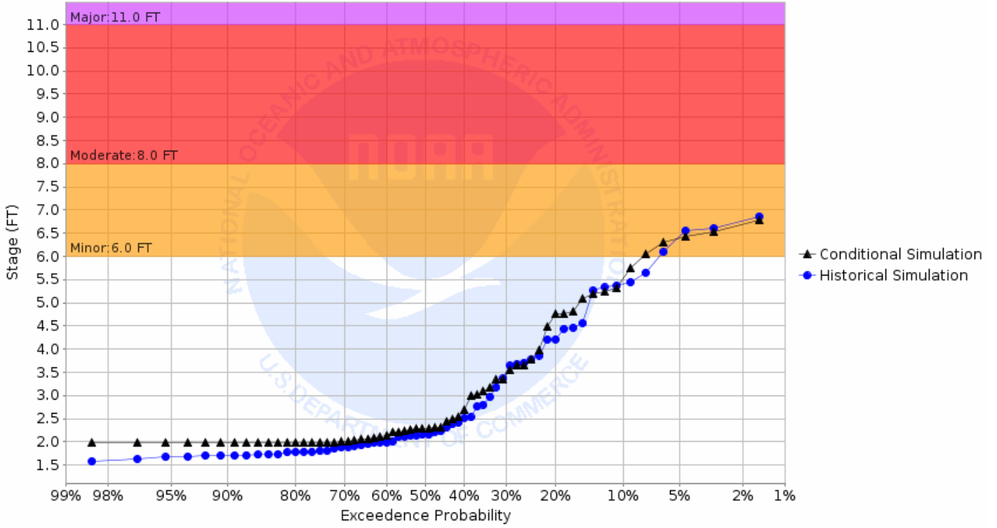
Chance of Exceeding River Stage at Forest River at Minto (MTON8) Forecast for the period 05/06/2019 - 07/28/2019 This is a conditional simulation based on the conditions as of 04/22/2019
