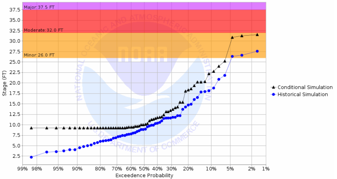
Chance of Exceeding River Stage at Red River of the North at Hillsboro 11ESE (Halstad MN) (HILN8) Forecast for the period 08/26/2019 - 11/24/2019 This is a conditional simulation based on the conditions as of 08/19/2019
