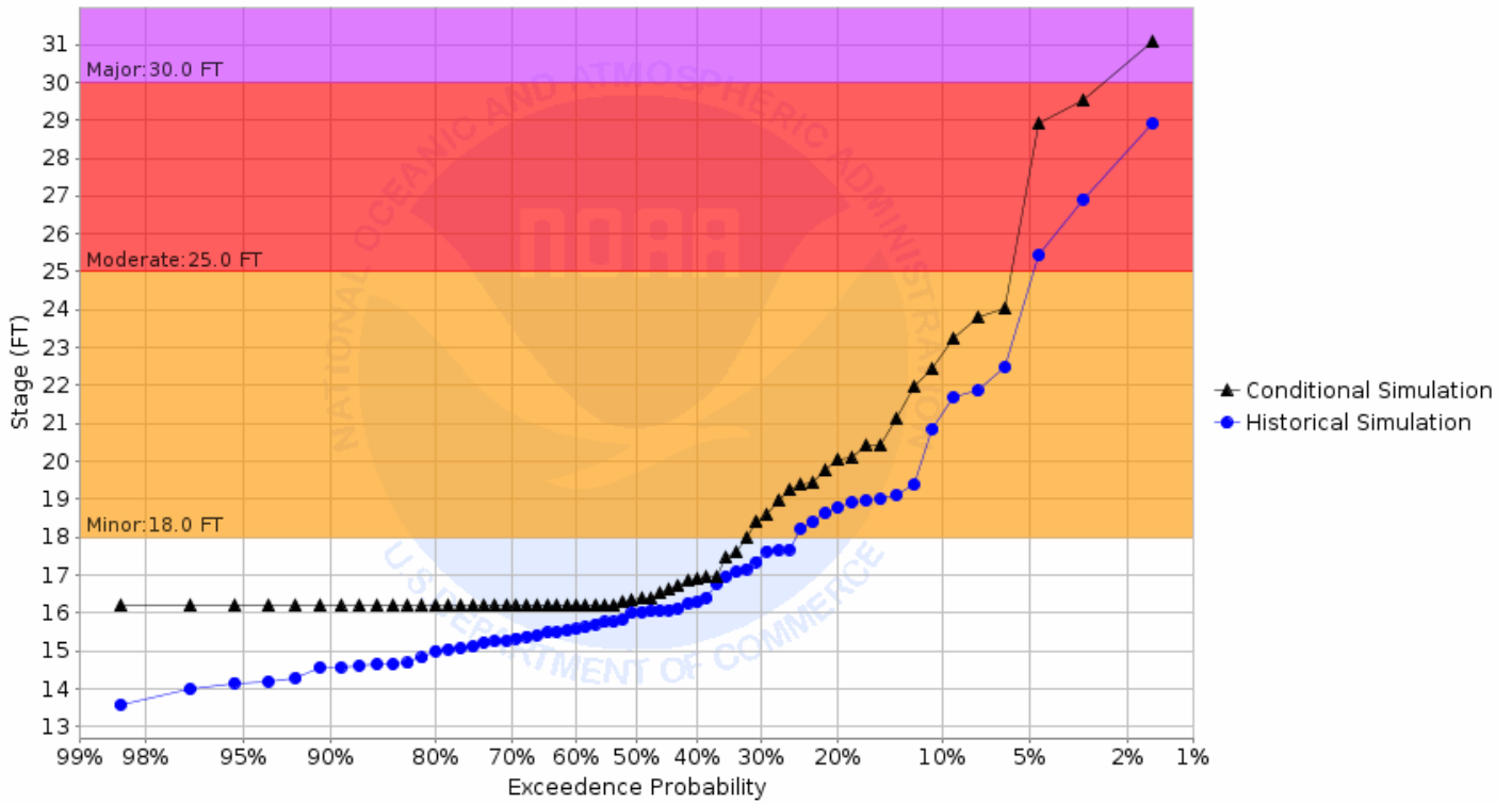
Chance of Exceeding River Stage at Red River of the North at Fargo WTP (FGON8) Forecast for the period 08/26/2019 - 11/24/2019 This is a conditional simulation based on the conditions as of 08/19/2019
