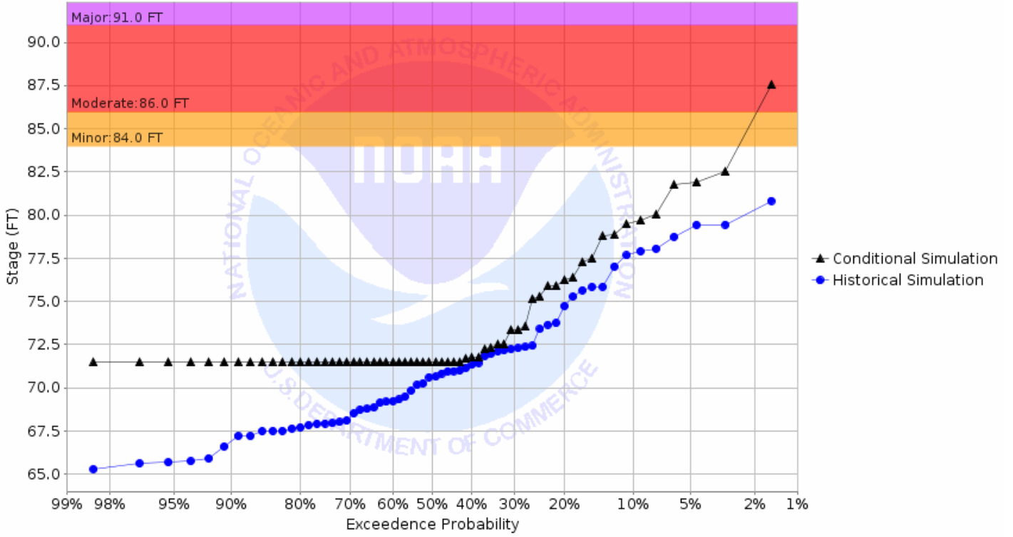
Chance of Exceeding River Stage at Sheyenne River at Harwood (HWDN8) Forecast for the period 08/26/2019 - 11/24/2019 This is a conditional simulation based on the conditions as of 08/19/2019
