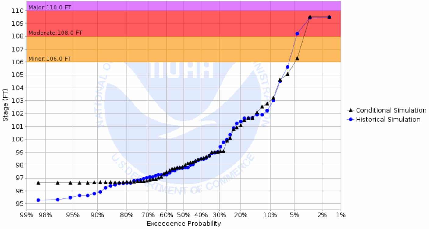
Chance of Exceeding River Stage at Snake River at Alvarado (ALVM5) Forecast for the period 08/26/2019 - 11/24/2019 This is a conditional simulation based on the conditions as of 08/19/2019
