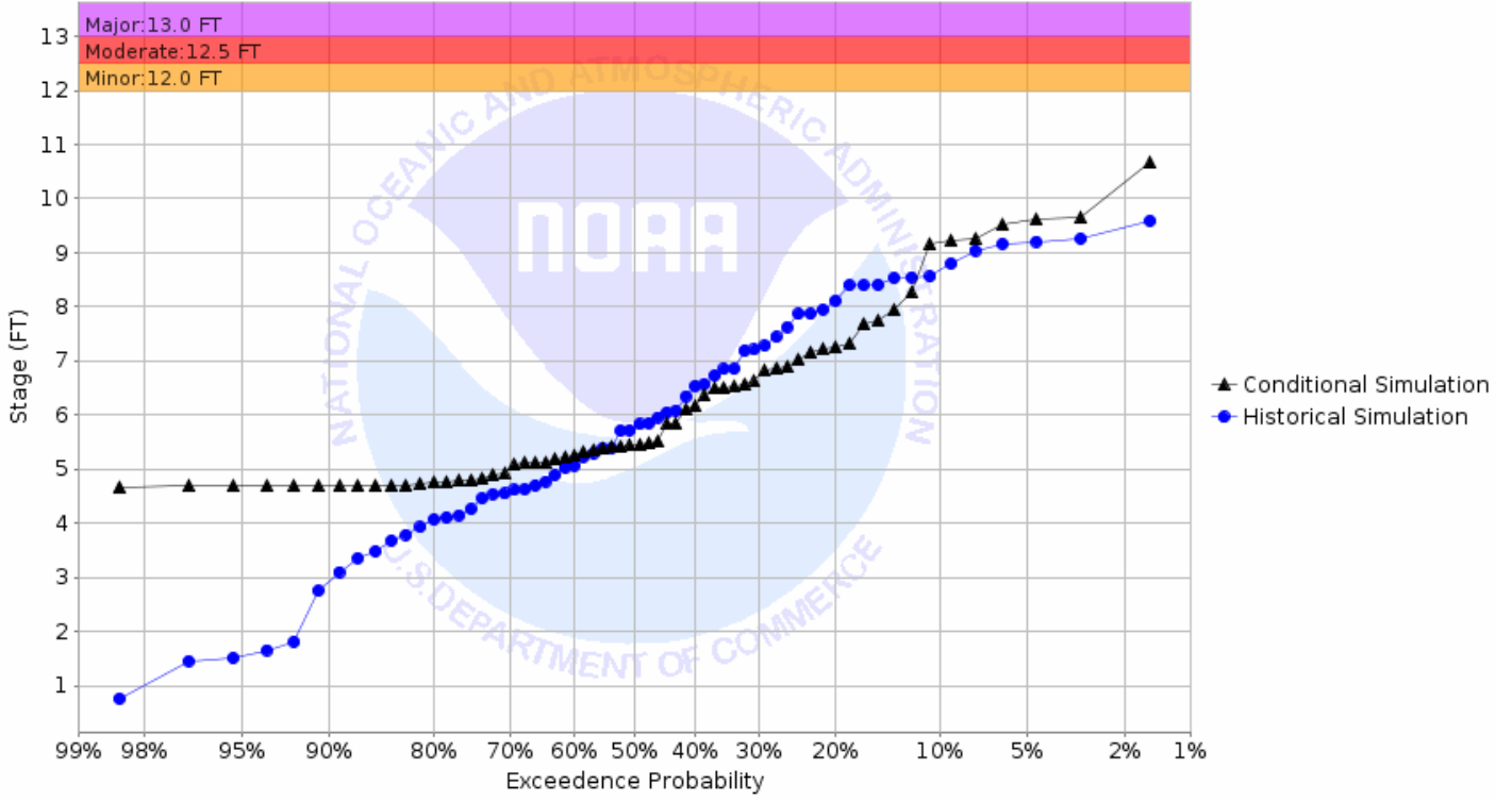
Chance of Exceeding River Stage at Red Lake River at High Landing (HIGM5) Forecast for the period 08/26/2019 - 11/24/2019 This is a conditional simulation based on the conditions as of 08/19/2019
