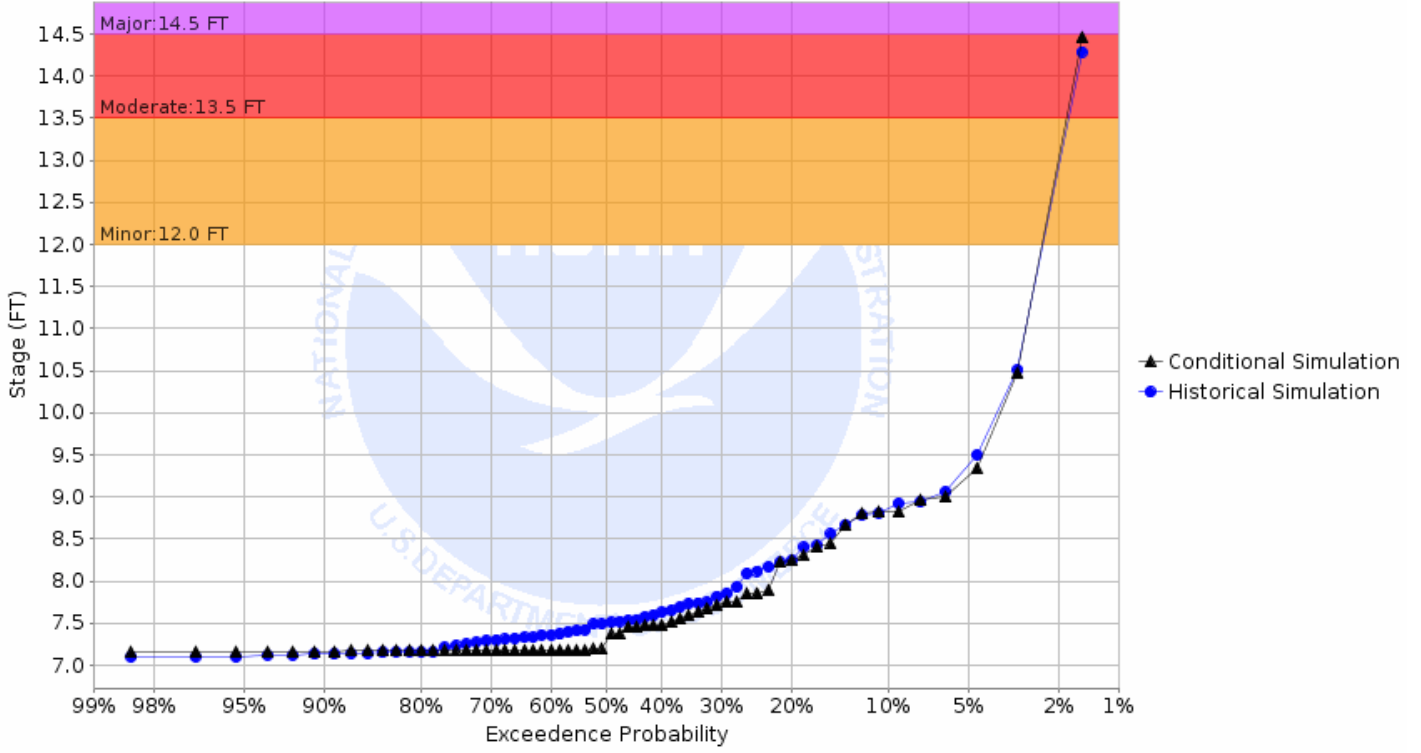
Chance of Exceeding River Stage at Park River at Grafton (GRNN8) Forecast for the period 08/26/2019 - 11/24/2019 This is a conditional simulation based on the conditions as of 08/19/2019
