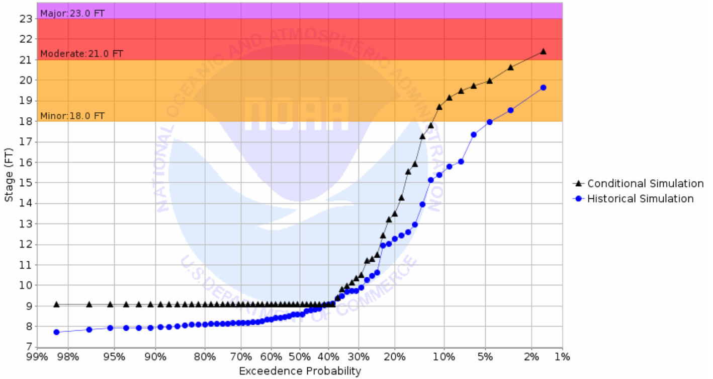
Chance of Exceeding River Stage at Maple River at Mapleton 3SW (MPLN8) Forecast for the period 08/26/2019 - 11/24/2019 This is a conditional simulation based on the conditions as of 08/19/2019
