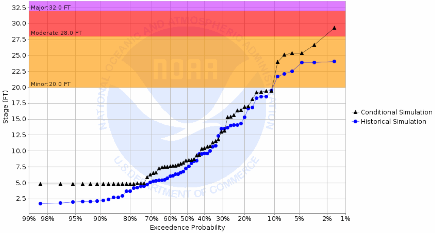
Chance of Exceeding River Stage at Wild Rice River at Hendrum (HNDM5) Forecast for the period 08/26/2019 - 11/24/2019 This is a conditional simulation based on the conditions as of 08/19/2019
