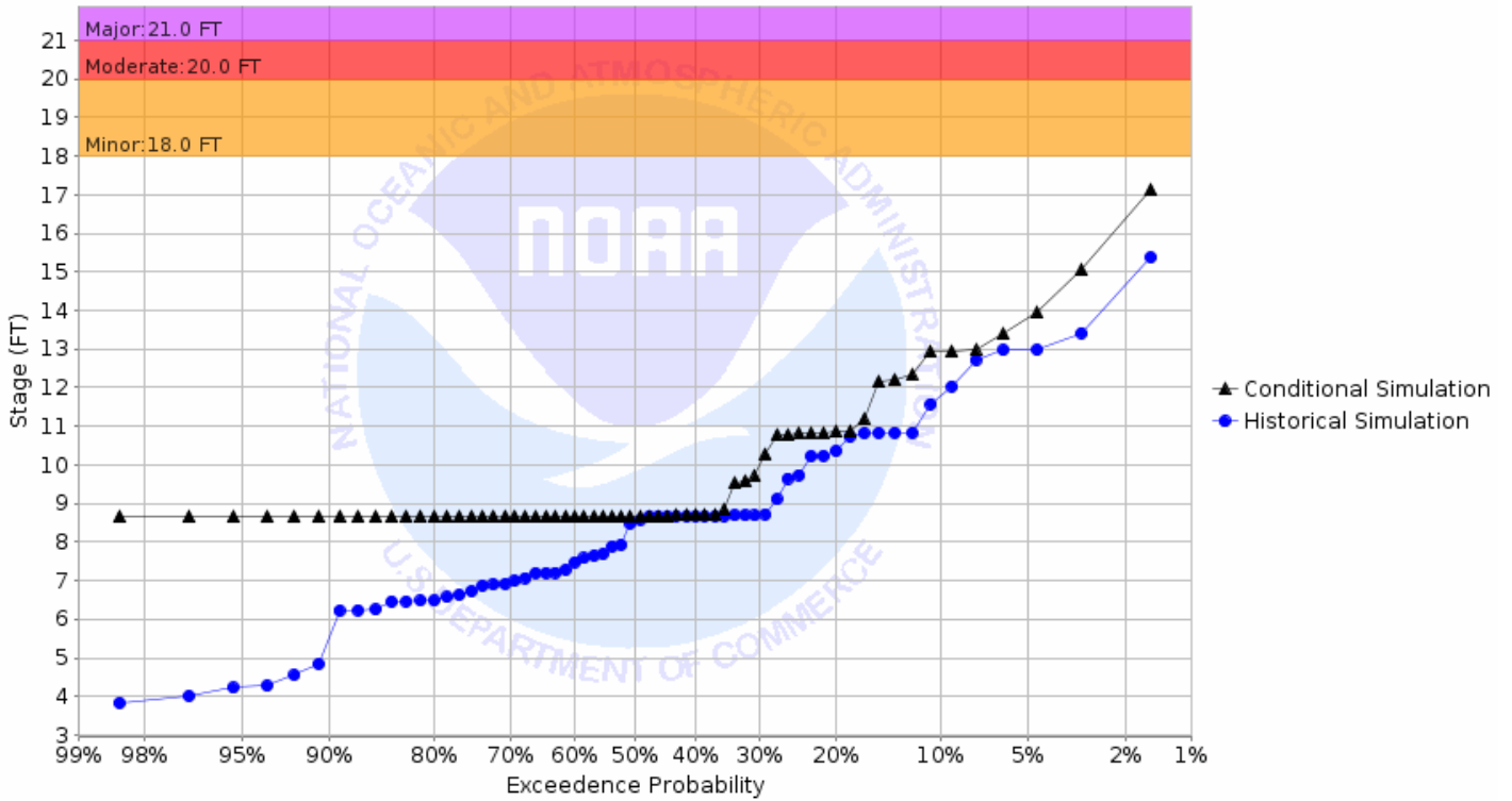
Chance of Exceeding River Stage at Sheyenne River Diversion at West Fargo (WFON8) Forecast for the period 08/26/2019 - 11/24/2019 This is a conditional simulation based on the conditions as of 08/19/2019
