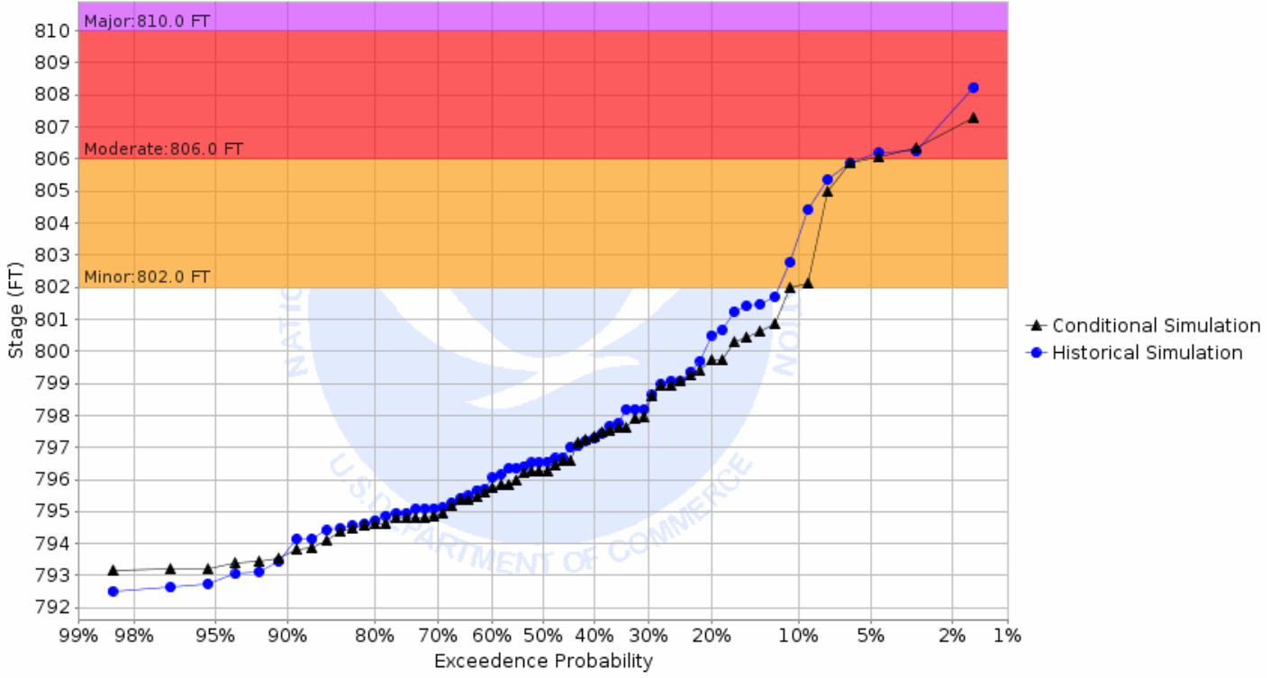
Chance of Exceeding River Stage at Two Rivers River at Hallock (HLLM5) Forecast for the period 08/26/2019 - 11/24/2019 This is a conditional simulation based on the conditions as of 08/19/2019
