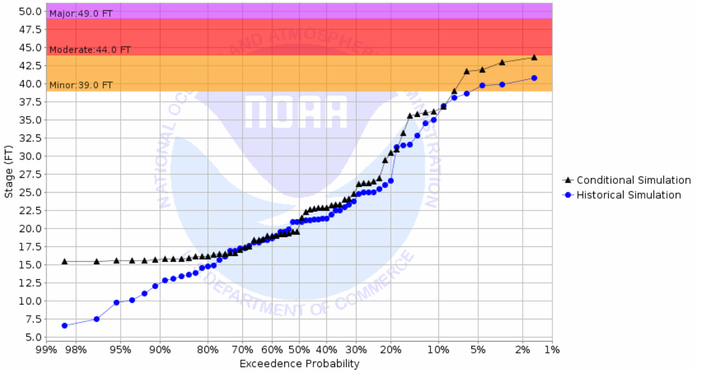
Chance of Exceeding River Stage at Red River of the North at Pembina (PBNN8) Forecast for the period 08/26/2019 - 11/24/2019 This is a conditional simulation based on the conditions as of 08/19/2019
