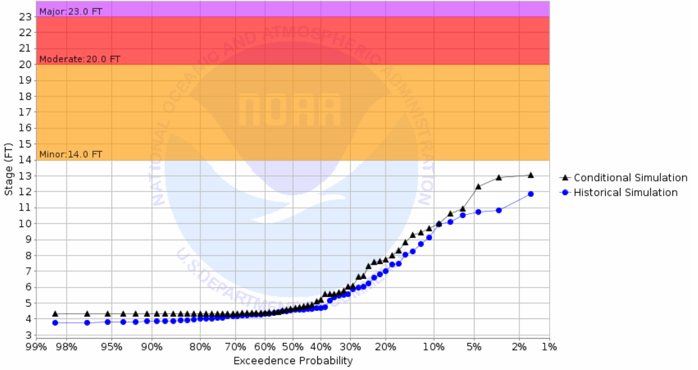
Chance of Exceeding River Stage at Marsh River at Shelly 4SE (SHYM5) Forecast for the period 08/26/2019 - 11/24/2019 This is a conditional simulation based on the conditions as of 08/19/2019
