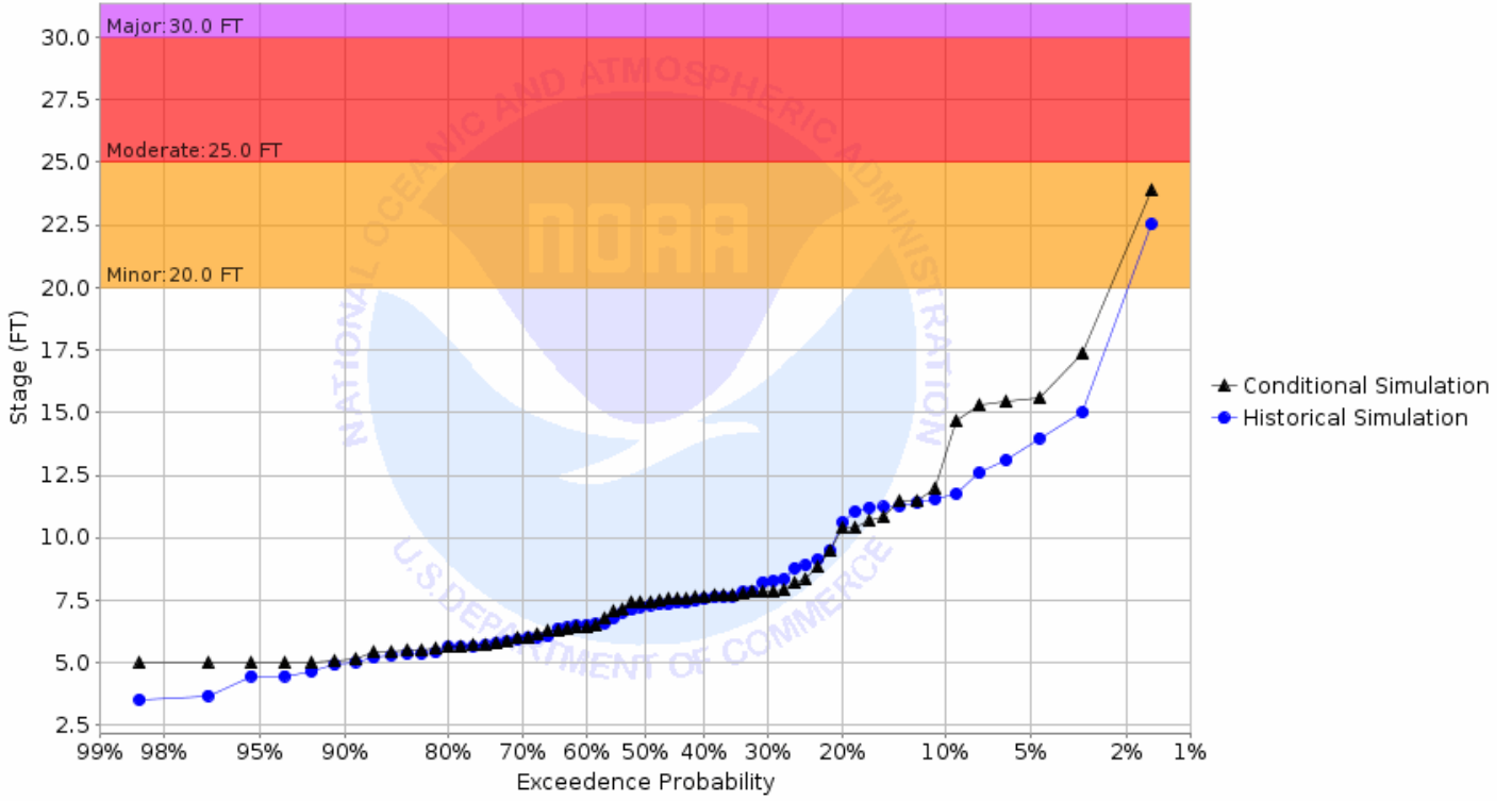
Chance of Exceeding River Stage at Sand Hill River at Climax (CLXM5) Forecast for the period 08/26/2019 - 11/24/2019 This is a conditional simulation based on the conditions as of 08/19/2019
