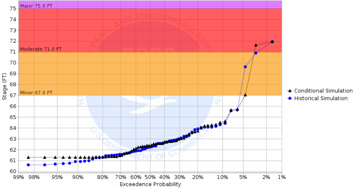
Chance of Exceeding River Stage at Snake River at Warren 3ENE-Morkassel Brdg (MKLM5) Forecast for the period 08/26/2019 - 11/24/2019 This is a conditional simulation based on the conditions as of 08/19/2019
