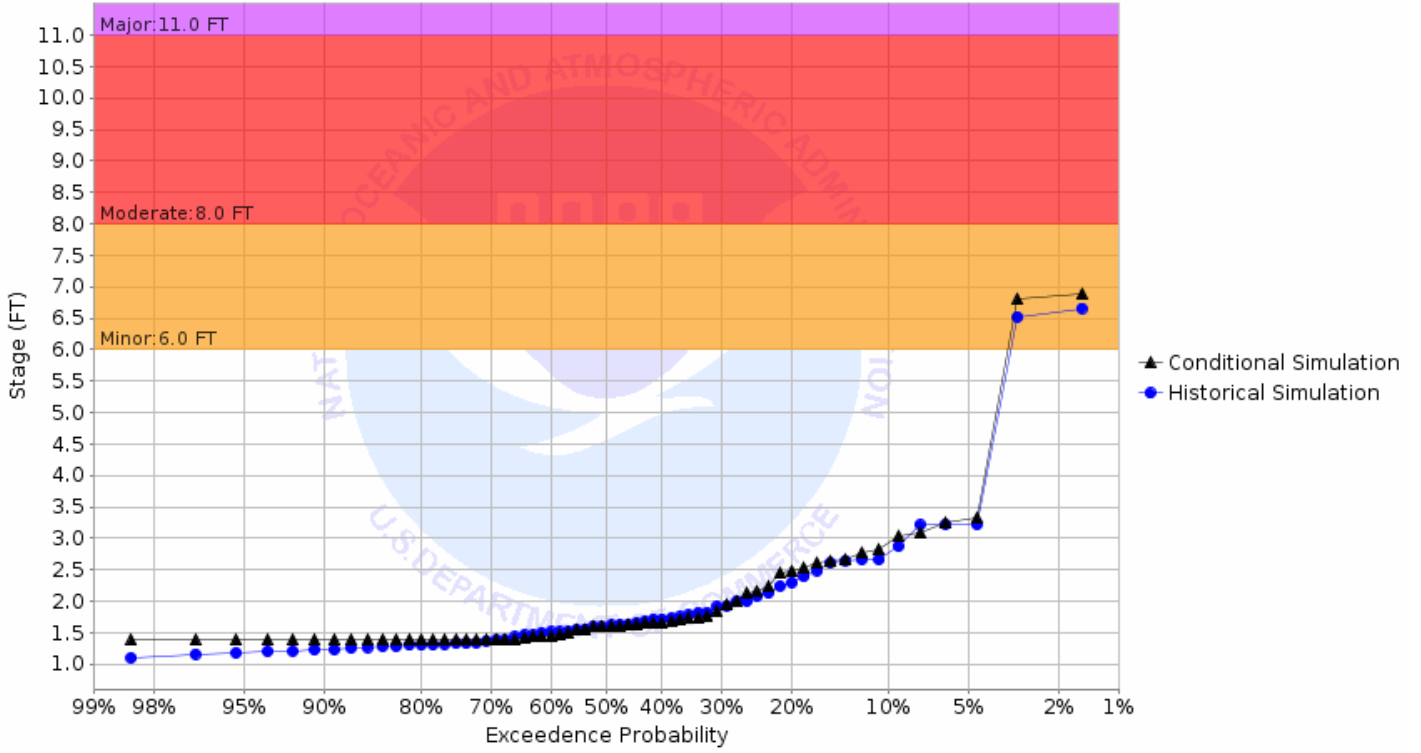
Chance of Exceeding River Stage at Forest River at Minto (MTON8) Forecast for the period 08/26/2019 - 11/24/2019 This is a conditional simulation based on the conditions as of 08/19/2019
