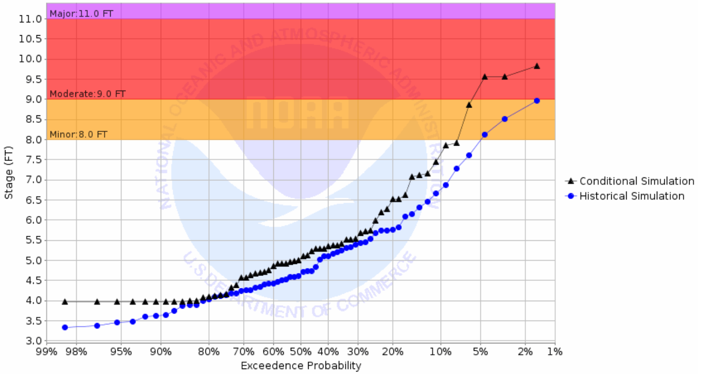
Chance of Exceeding River Stage at Buffalo River at Hawley 2SW (HWYM5) Forecast for the period 08/26/2019 - 11/24/2019 This is a conditional simulation based on the conditions as of 08/19/2019
