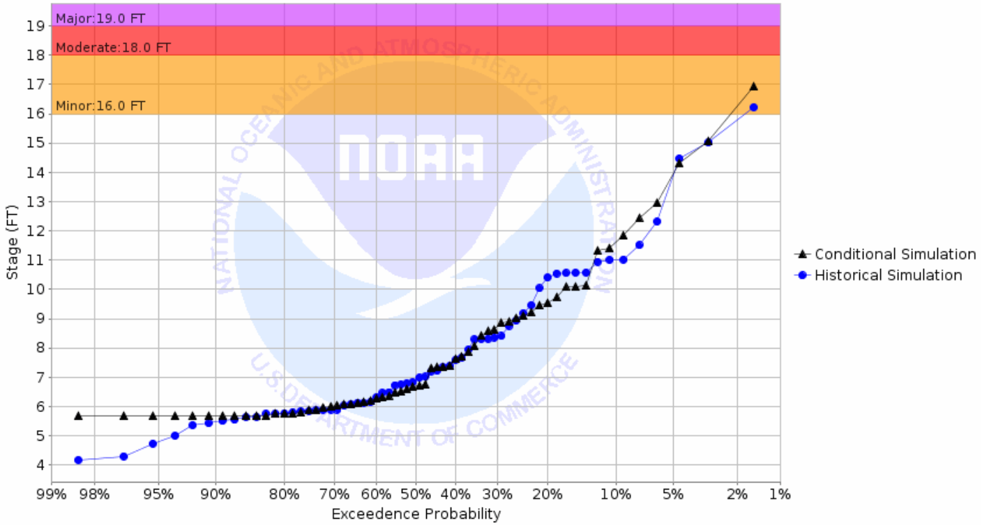
Chance of Exceeding River Stage at Roseau River at Roseau - Center St Brdg (ROSM5) Forecast for the period 08/26/2019 - 11/24/2019 This is a conditional simulation based on the conditions as of 08/19/2019
