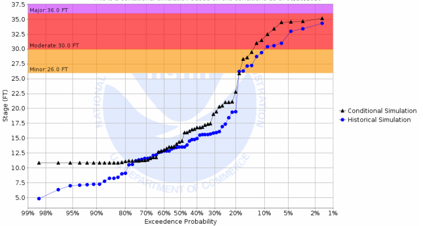
Chance of Exceeding River Stage at Red River of the North at Oslo (OSLM5) Forecast for the period 08/26/2019 - 11/24/2019 This is a conditional simulation based on the conditions as of 08/19/2019
