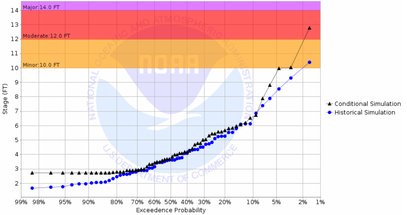
Chance of Exceeding River Stage at Wild Rice River at Twin Valley 1NE (TWVM5) Forecast for the period 08/26/2019 - 11/24/2019 This is a conditional simulation based on the conditions as of 08/19/2019
