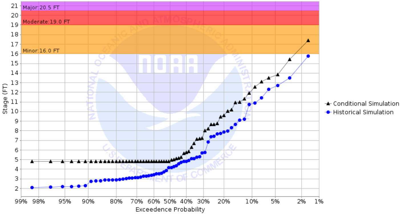
Chance of Exceeding River Stage at Sheyenne River at Kindred 2SE (KNDN8) Forecast for the period 08/26/2019 - 11/24/2019 This is a conditional simulation based on the conditions as of 08/19/2019
