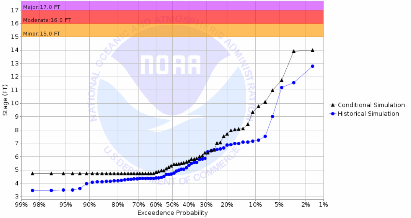
Chance of Exceeding River Stage at Sheyenne River at Valley City (VCRN8) Forecast for the period 08/26/2019 - 11/24/2019 This is a conditional simulation based on the conditions as of 08/19/2019
