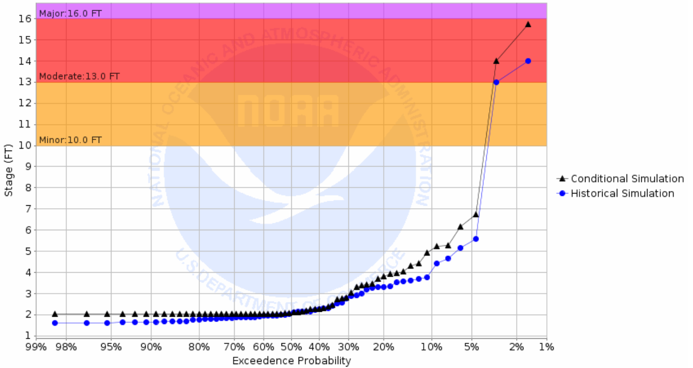
Chance of Exceeding River Stage at Goose River at Hillsboro (HGRN8) Forecast for the period 08/26/2019 - 11/24/2019 This is a conditional simulation based on the conditions as of 08/19/2019
