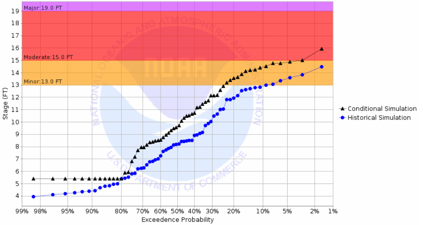
Chance of Exceeding River Stage at South Branch Buffalo River at Sabin 1E (SABM5) Forecast for the period 08/26/2019 - 11/24/2019 This is a conditional simulation based on the conditions as of 08/19/2019
