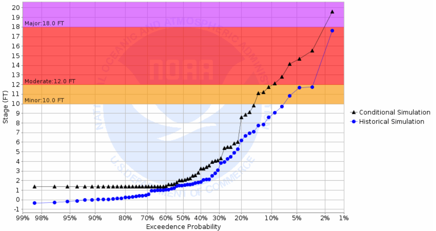
Chance of Exceeding River Stage at Wild Rice River at Abercrombie 2WNW (ABRN8) Forecast for the period 08/26/2019 - 11/24/2019 This is a conditional simulation based on the conditions as of 08/19/2019
