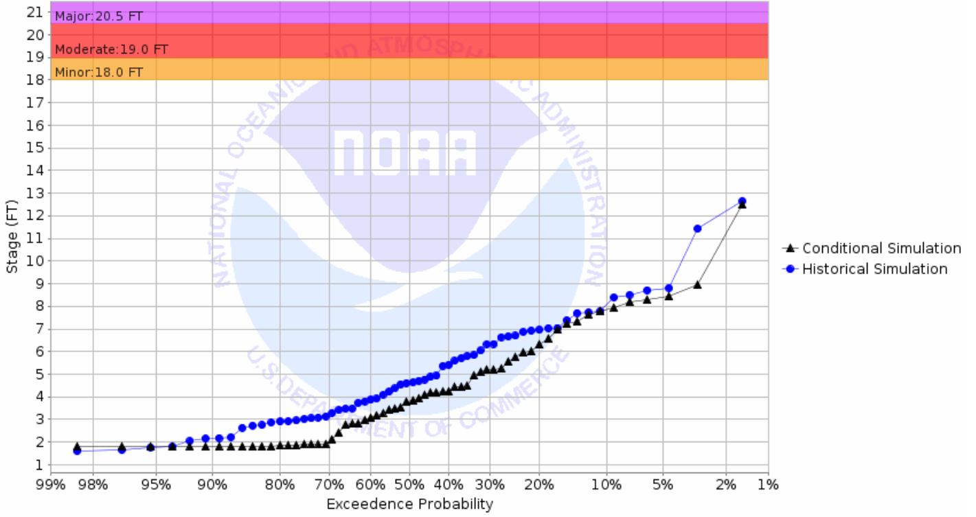
Chance of Exceeding River Stage at Pembina River at Neche (NCEN8) Forecast for the period 08/26/2019 - 11/24/2019 This is a conditional simulation based on the conditions as of 08/19/2019
