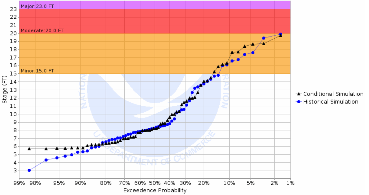
Chance of Exceeding River Stage at Red Lake River at Crookston (CRKM5) Forecast for the period 08/26/2019 - 11/24/2019 This is a conditional simulation based on the conditions as of 08/19/2019
