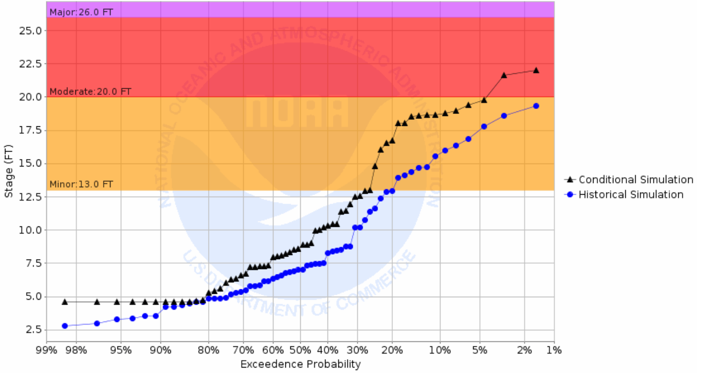
Chance of Exceeding River Stage at Buffalo River at Dilworth 7NE (DILM5) Forecast for the period 08/26/2019 - 11/24/2019 This is a conditional simulation based on the conditions as of 08/19/2019
