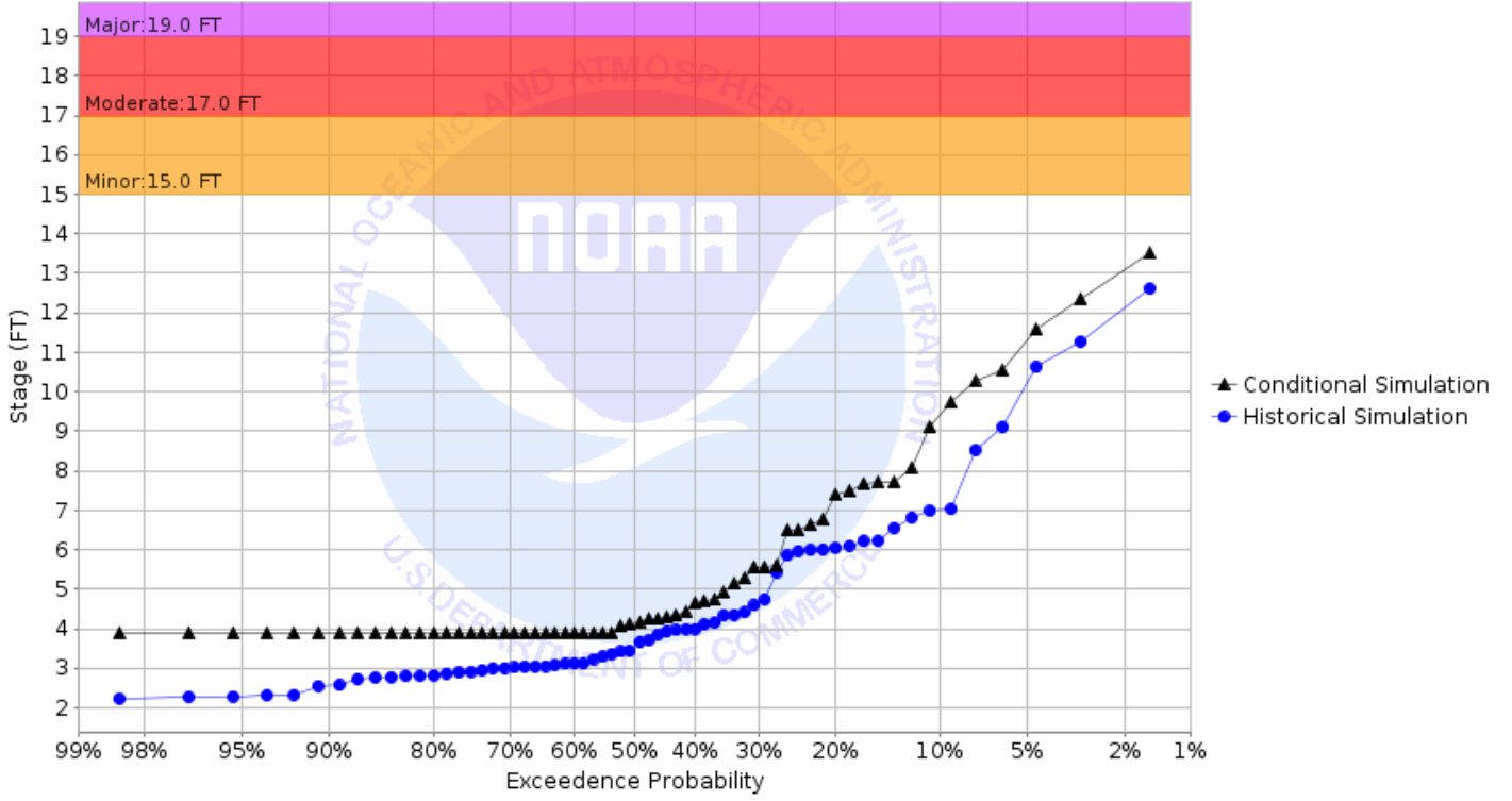
Chance of Exceeding River Stage at Sheyenne River at Lisbon (LBNN8) Forecast for the period 08/26/2019 - 11/24/2019 This is a conditional simulation based on the conditions as of 08/19/2019
