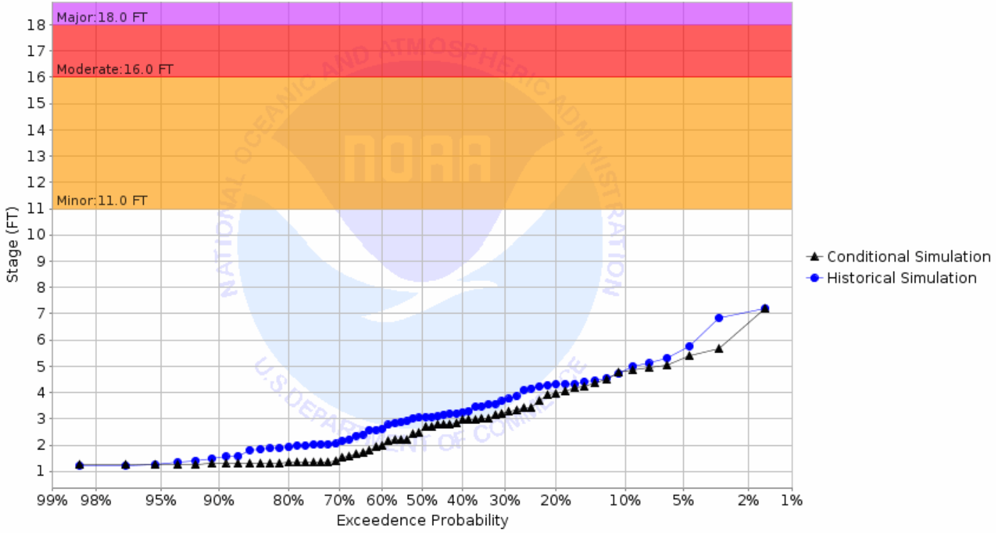
Chance of Exceeding River Stage at Pembina River at Walhalla (WLHN8) Forecast for the period 08/26/2019 - 11/24/2019 This is a conditional simulation based on the conditions as of 08/19/2019
