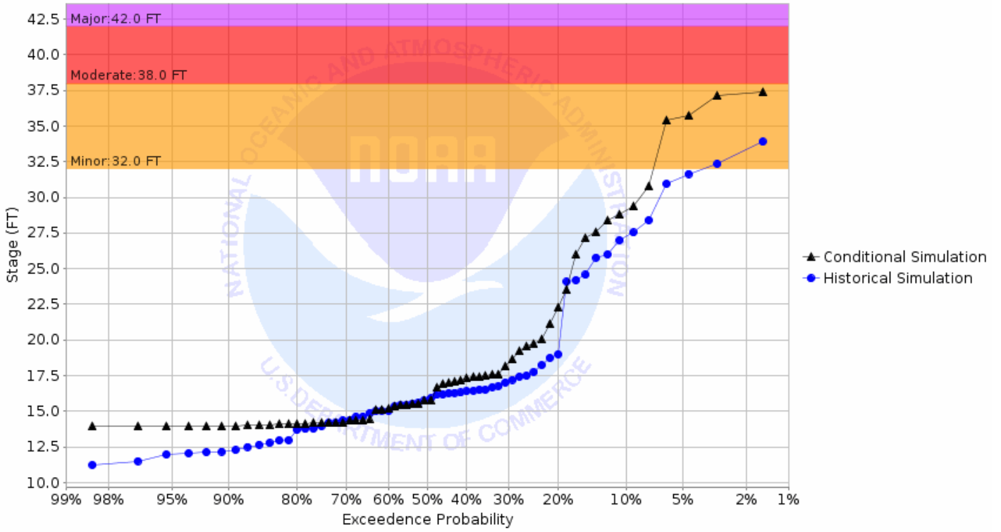
Chance of Exceeding River Stage at Red River of the North at Drayton 2NE - Hwy 66 Brdg (DRTN8) Forecast for the period 08/26/2019 - 11/24/2019 This is a conditional simulation based on the conditions as of 08/19/2019
