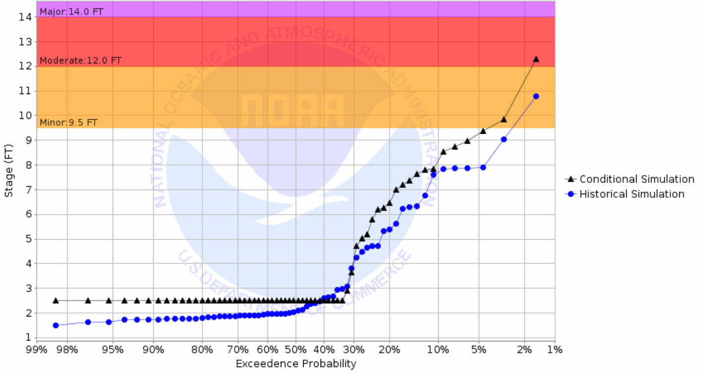
Chance of Exceeding River Stage at Maple River at Enderlin 1E (ENDN8) Forecast for the period 08/26/2019 - 11/24/2019 This is a conditional simulation based on the conditions as of 08/19/2019
