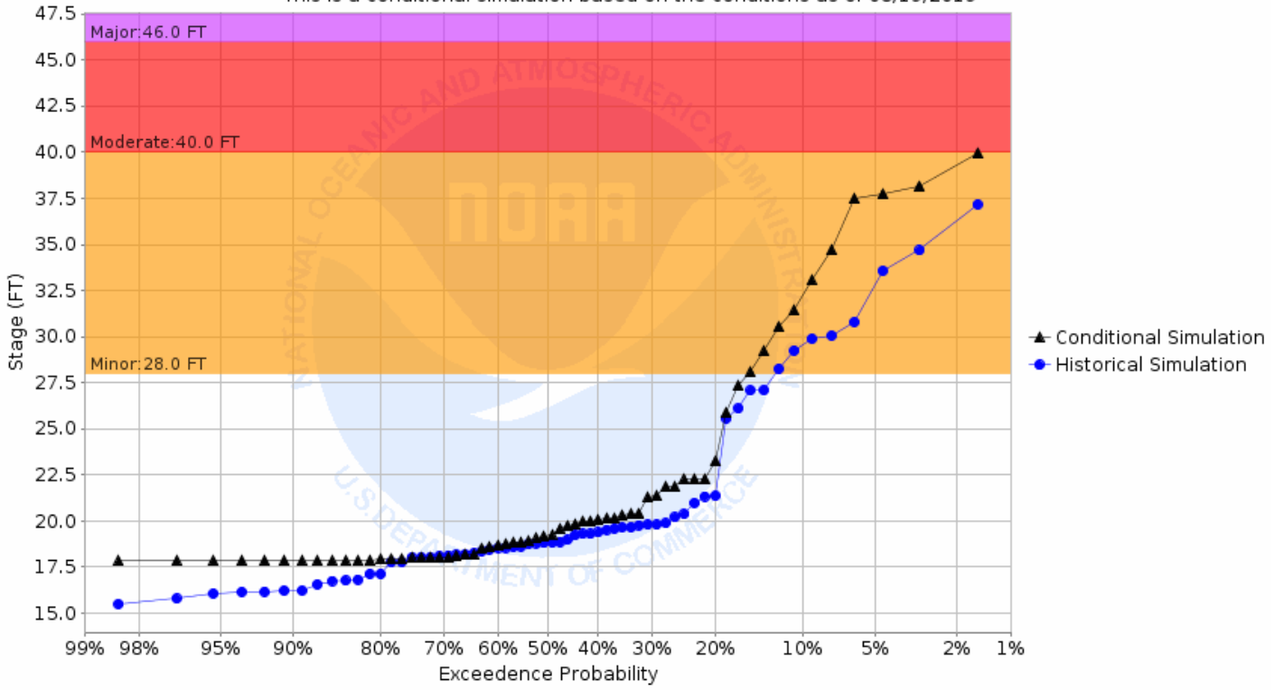
Chance of Exceeding River Stage at Red River of the North at Oslo (OSLM5) Forecast for the period 08/26/2019 - 11/24/2019 This is a conditional simulation based on the conditions as of 08/19/2019
