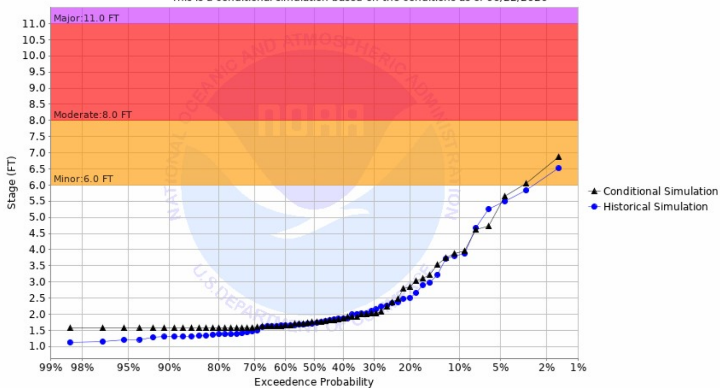
Chance of Exceeding River Stage at Forest River at Minto (MTON8) Forecast for the period 06/29/2020 - 09/27/2020 This is a conditional simulation based on the conditions as of 06/22/2020
