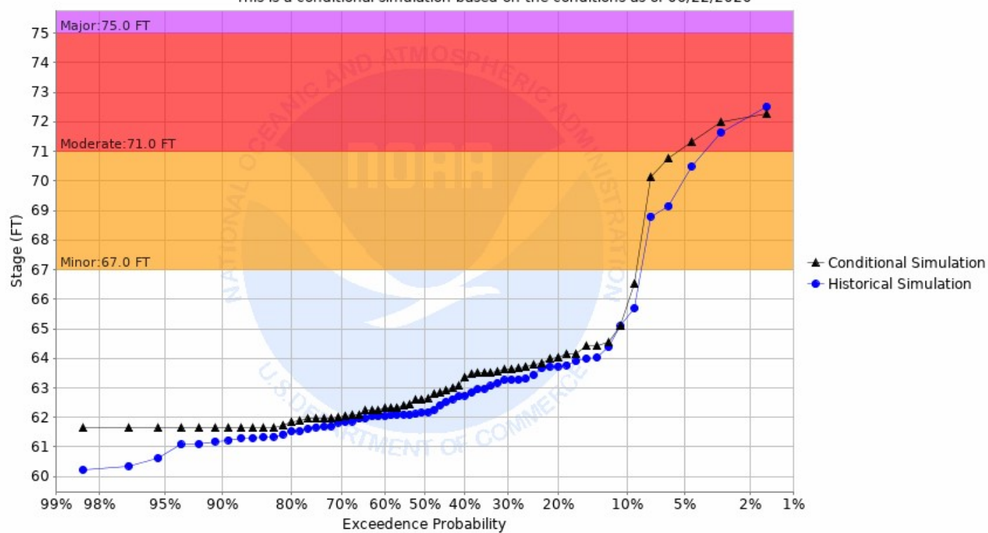
Chance of Exceeding River Stage at Snake River at Warren 3ENE-Morkassel Brdg (MKLM5) Forecast for the period 06/29/2020 - 09/27/2020 This is a conditional simulation based on the conditions as of 06/22/2020
