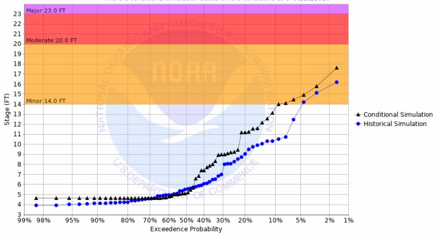
Chance of Exceeding River Stage at Marsh River at Shelly 4SE (SHYM5) Forecast for the period 06/29/2020 - 09/27/2020 This is a conditional simulation based on the conditions as of 06/22/2020
