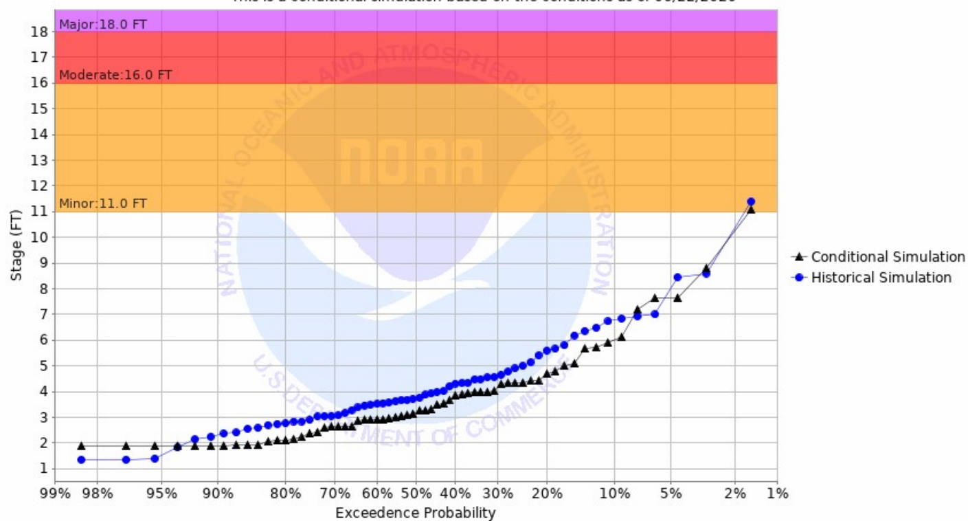
Chance of Exceeding River Stage at Pembina River at Walhalla (WLHN8) Forecast for the period 06/29/2020 - 09/27/2020 This is a conditional simulation based on the conditions as of 06/22/2020
