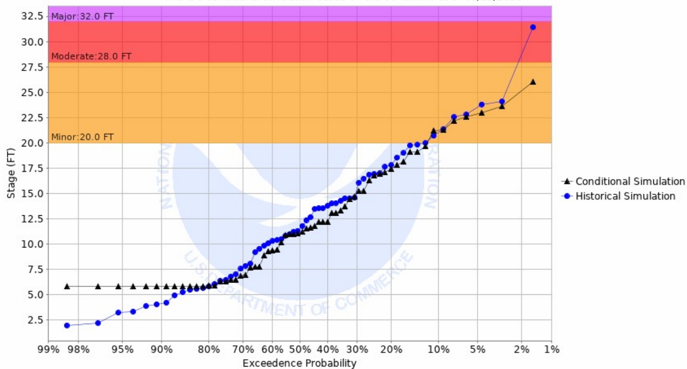
Chance of Exceeding River Stage at Wild Rice River at Hendrum (HNDM5) Forecast for the period 06/29/2020 - 09/27/2020 This is a conditional simulation based on the conditions as of 06/22/2020
