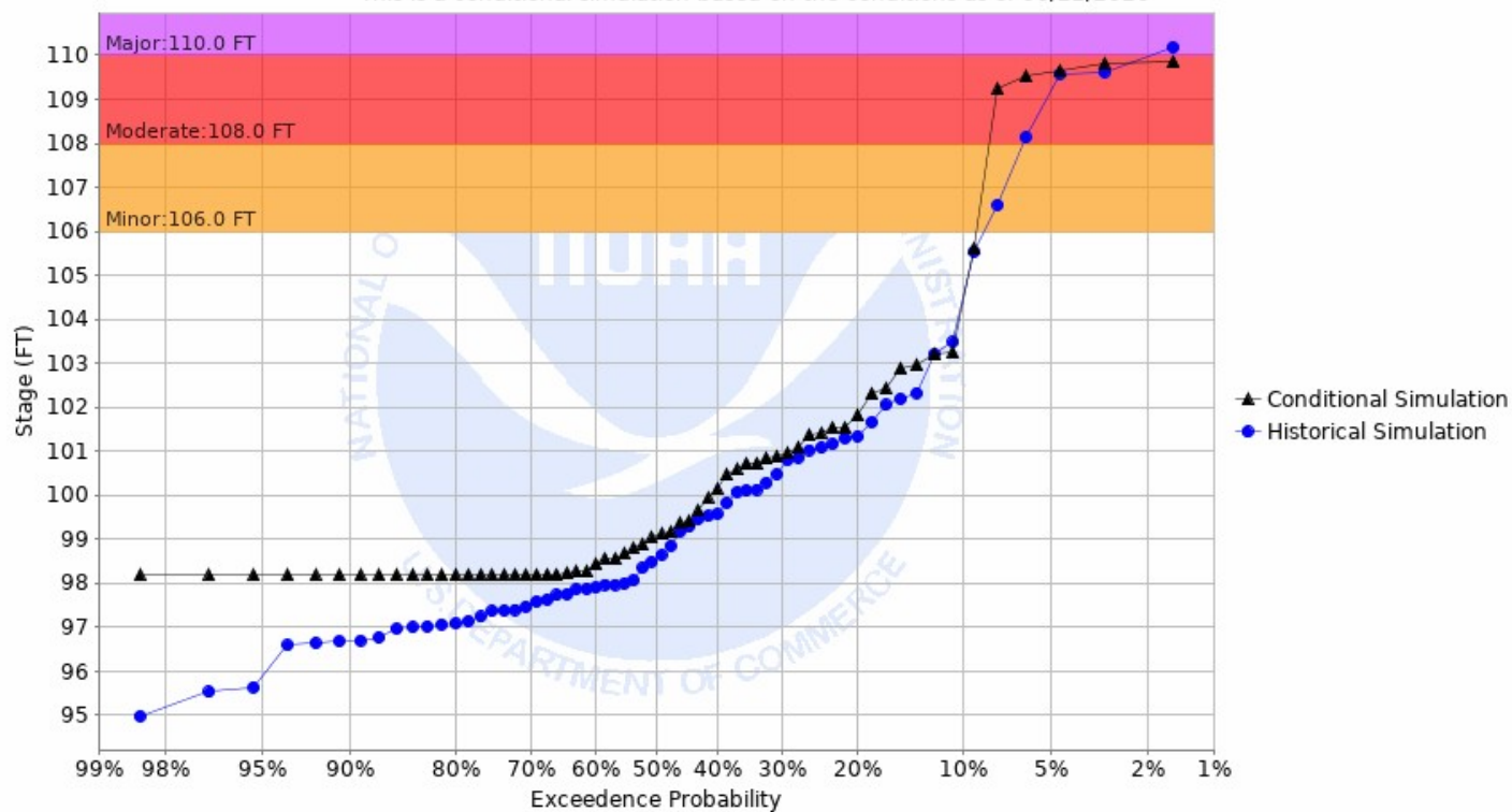
Chance of Exceeding River Stage at Snake River at Alvarado (ALVM5) Forecast for the period 06/29/2020 - 09/27/2020 This is a conditional simulation based on the conditions as of 06/22/2020
