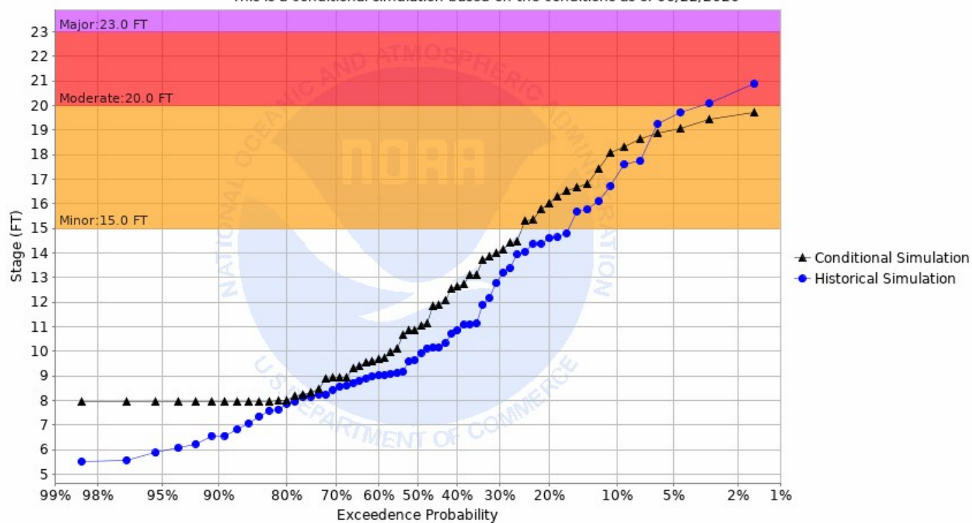
Chance of Exceeding River Stage at Red Lake River at Crookston (CRKM5) Forecast for the period 06/29/2020 - 09/27/2020 This is a conditional simulation based on the conditions as of 06/22/2020
