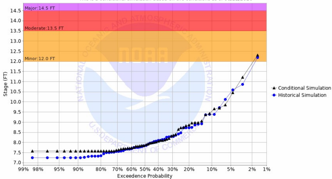
Chance of Exceeding River Stage at Park River at Grafton (GRNN8) Forecast for the period 06/29/2020 - 09/27/2020 This is a conditional simulation based on the conditions as of 06/22/2020
