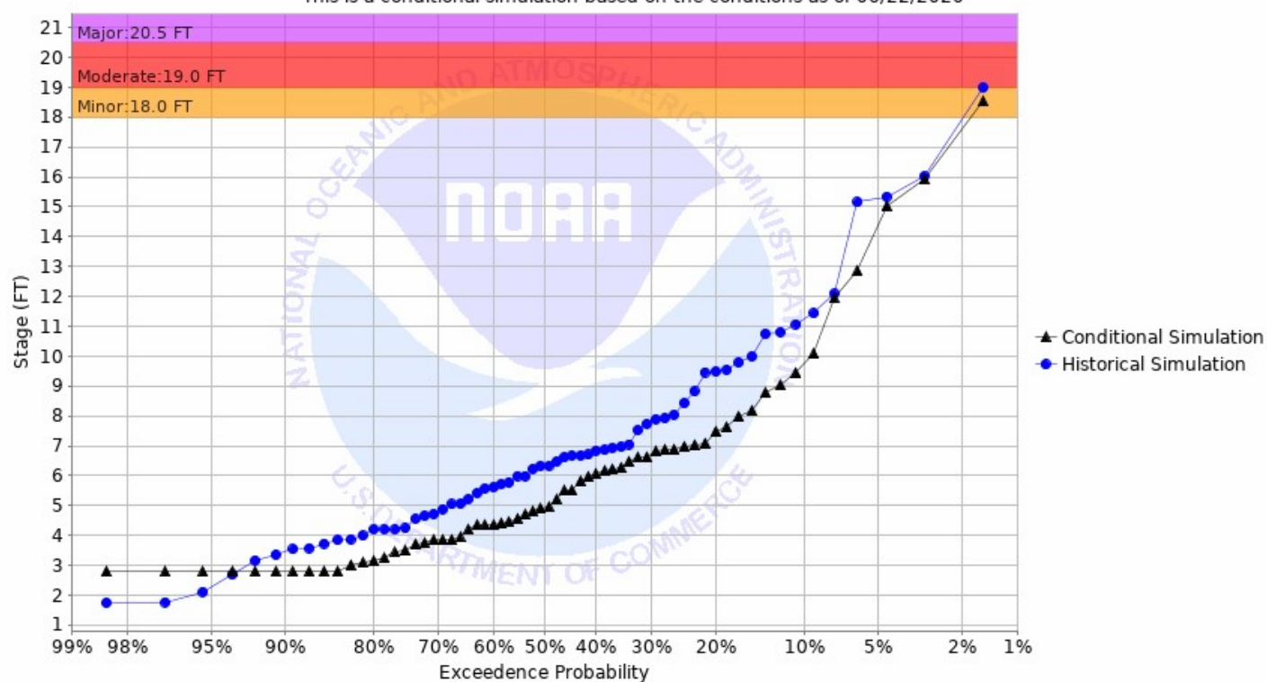
Chance of Exceeding River Stage at Pembina River at Natchez (NCEN8) Forecast for the period 06/29/2020 - 09/27/2020 This is a conditional simulation based on the conditions as of 06/22/2020
