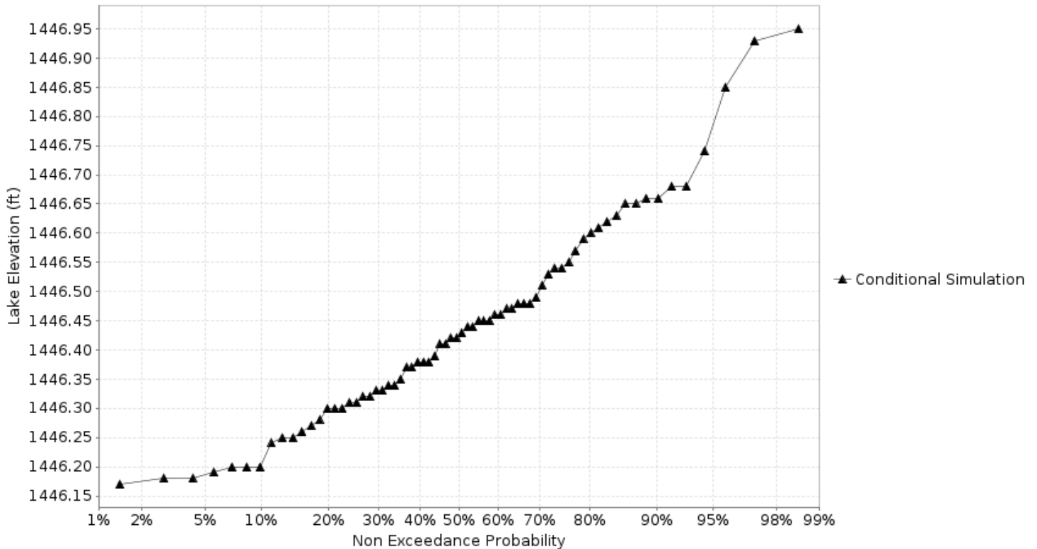
Probability of Falling to Low Lake Levels on the Devils Lake at Devils Lake 5SW-Creel Bay (DCBN8) Forecast for the period 09/01/2021 - 11/30/2021 This is a conditional simulation based on the conditions as of 08/23/2021
