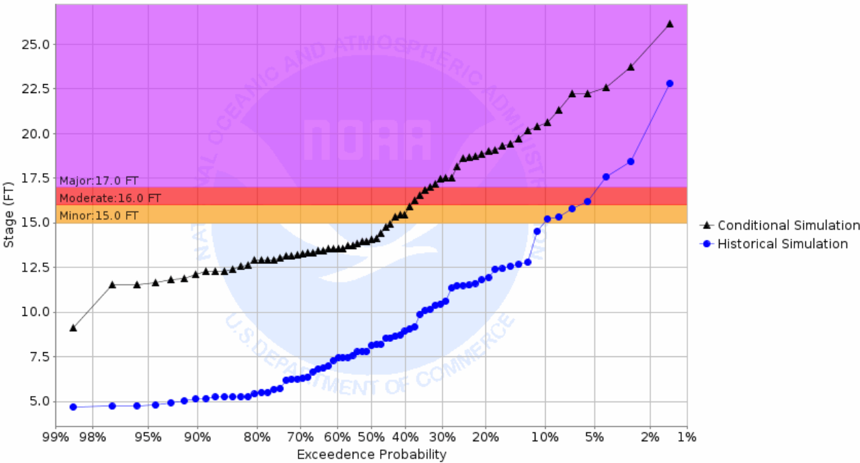
Chance of Exceeding River Stage at Sheyenne River at Valley City (VCRN8) Forecast for the period 01/31/2022 - 05/01/2022 This is a conditional simulation based on the conditions as of 01/24/2022
