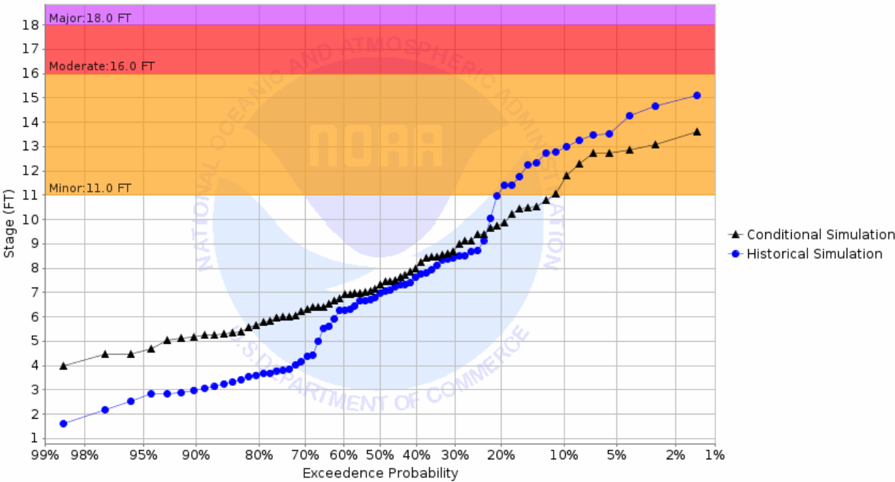
Chance of Exceeding River Stage at Pembina River at Walhalla (WLHN8) Forecast for the period 01/31/2022 - 05/01/2022 This is a conditional simulation based on the conditions as of 01/24/2022
