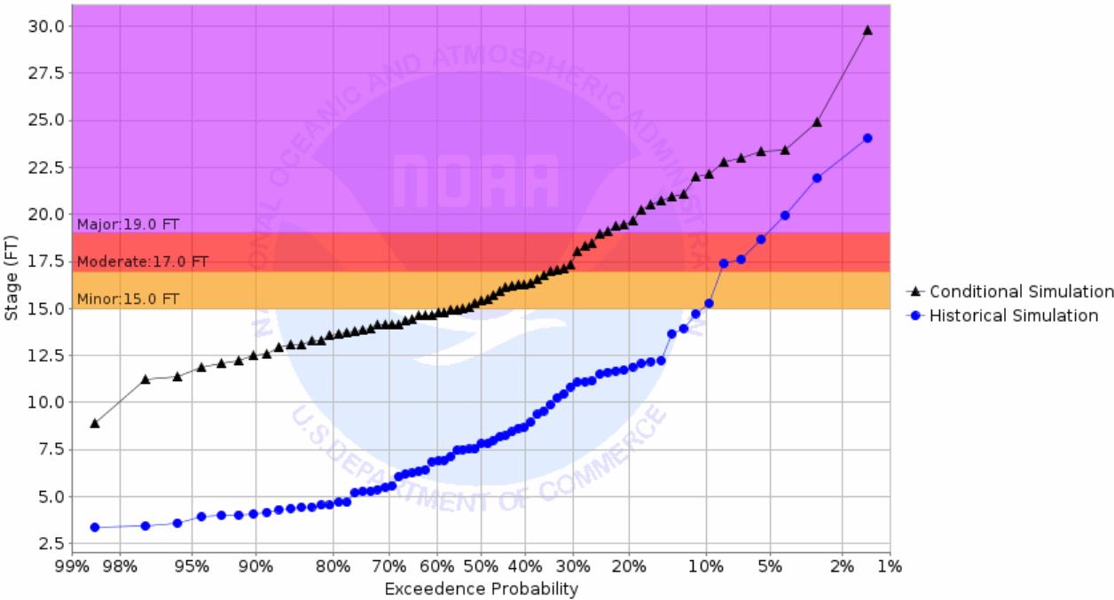
Chance of Exceeding River Stage at Sheyenne River at Lisbon (LBNN8) Forecast for the period 01/31/2022 - 05/01/2022 This is a conditional simulation based on the conditions as of 01/24/2022
