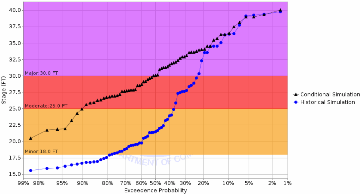
Chance of Exceeding River Stage at Red River of the North at Fargo WTP (FGON8) Forecast for the period 01/31/2022 - 05/01/2022 This is a conditional simulation based on the conditions as of 01/24/2022
