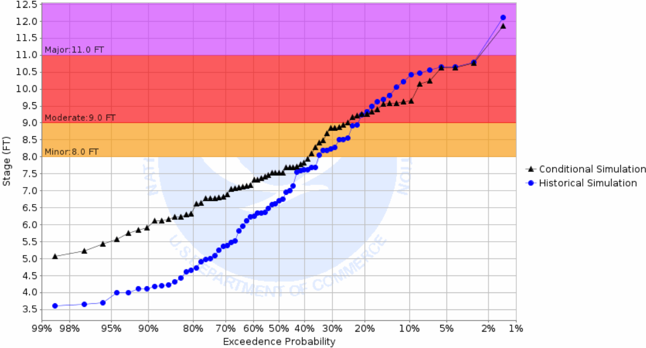
Chance of Exceeding River Stage at Buffalo River at Hawley 2SW (HWYM5) Forecast for the period 01/31/2022 - 05/01/2022 This is a conditional simulation based on the conditions as of 01/24/2022
