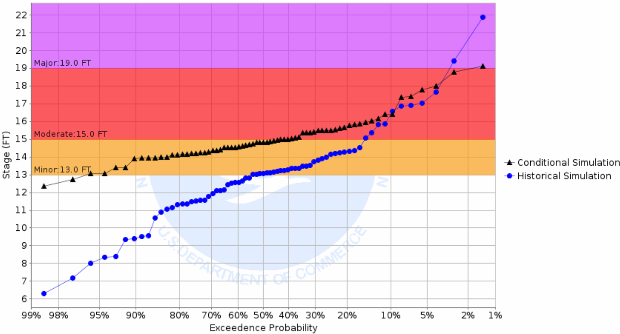
Chance of Exceeding River Stage at South Branch Buffalo River at Sabin 1E (SABM5) Forecast for the period 01/31/2022 - 05/01/2022 This is a conditional simulation based on the conditions as of 01/24/2022
