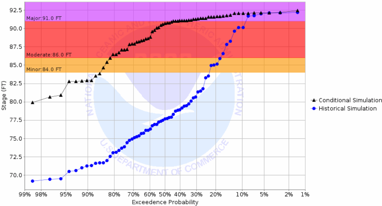
Chance of Exceeding River Stage at Sheyenne River at Harwood (HWDN8) Forecast for the period 01/31/2022 - 05/01/2022 This is a conditional simulation based on the conditions as of 01/24/2022
