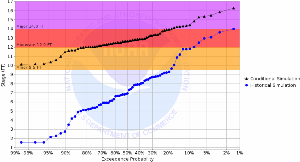
Chance of Exceeding River Stage at Maple River at Enderlin 1E (ENDN8) Forecast for the period 01/31/2022 - 05/01/2022 This is a conditional simulation based on the conditions as of 01/24/2022
