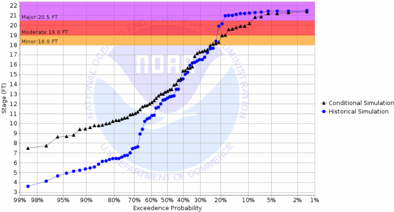
Chance of Exceeding River Stage at Pembina River at Neche (NCEN8) Forecast for the period 01/31/2022 - 05/01/2022 This is a conditional simulation based on the conditions as of 01/24/2022
