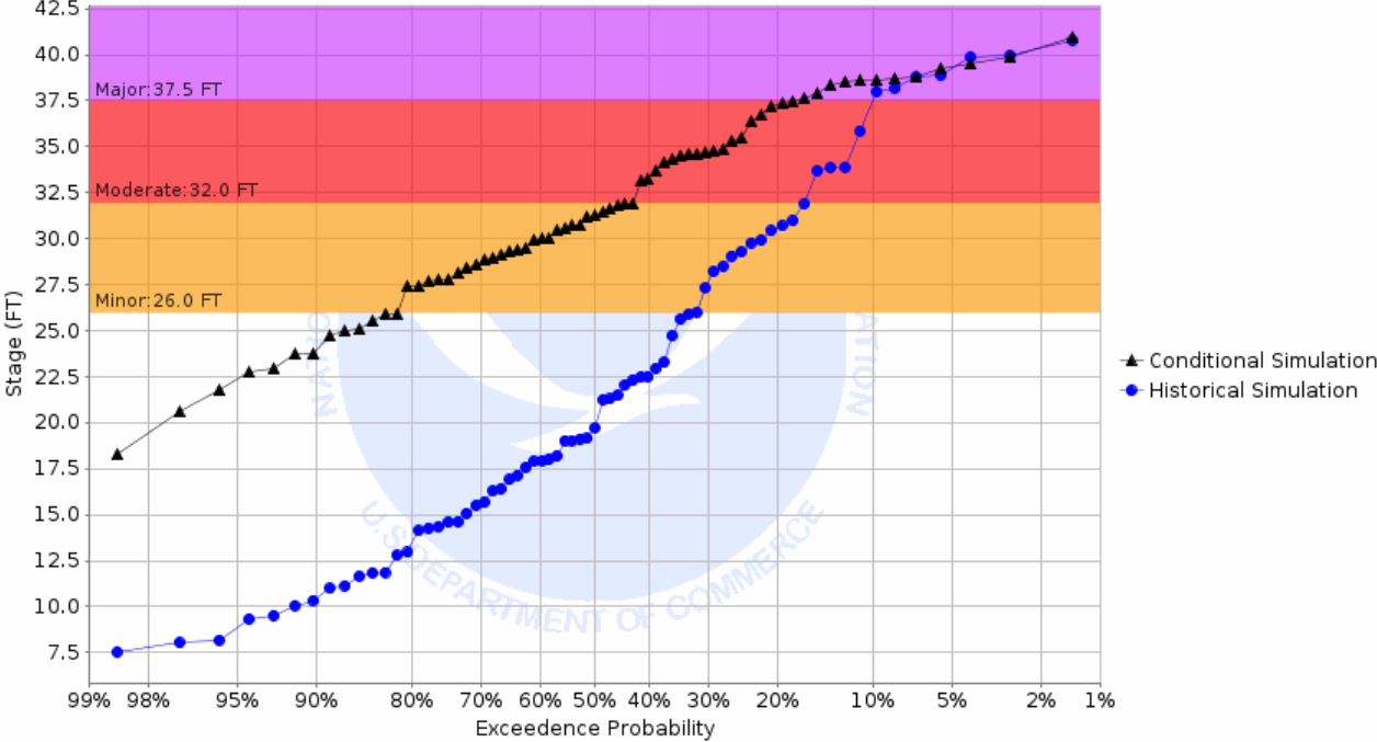
Chance of Exceeding River Stage at Red River of the North at Hillsboro 11ESE (Halstad MN) (HILN8) Forecast for the period 01/31/2022 - 05/01/2022 This is a conditional simulation based on the conditions as of 01/24/2022
