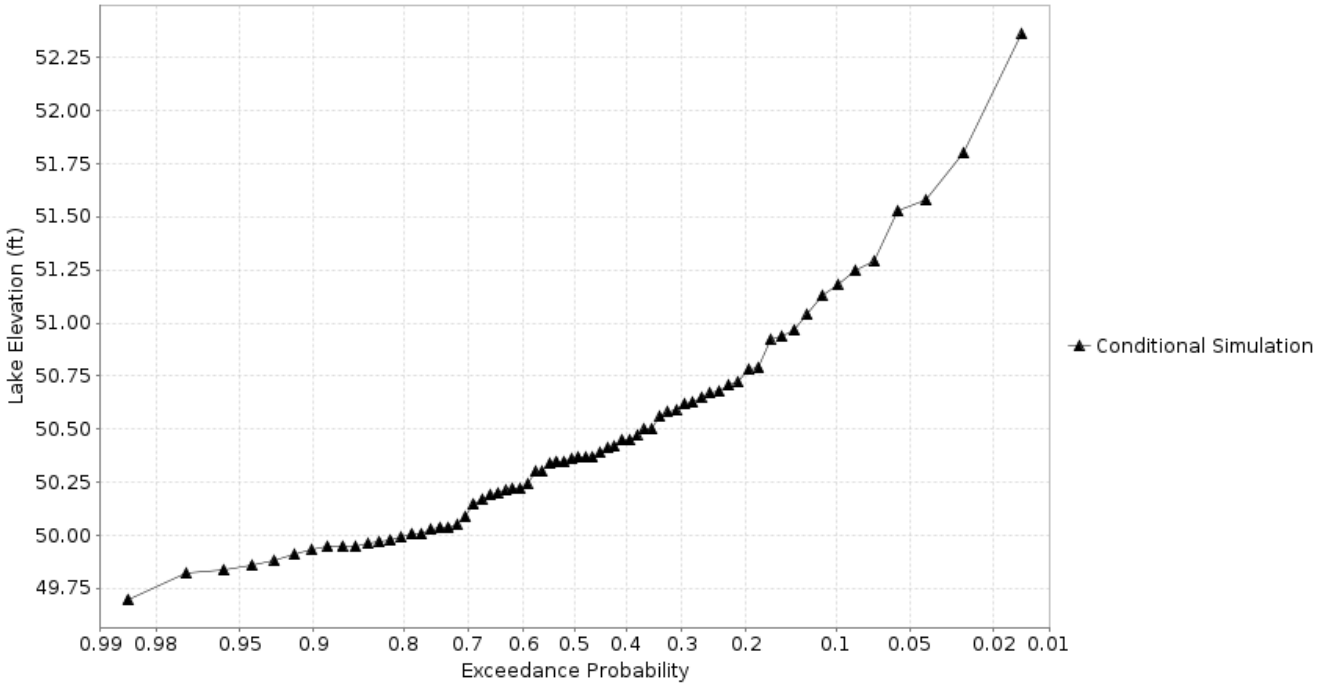
Probability of Rising to High Lake Levels on the Eastern Stump Lake at Lakota 11S (ESLN8) Forecast for the period 03/21/2022 - 09/30/2022 This is a conditional simulation based on the conditions as of 03/21/2022 Pumping schedule : 350cfs Jun 1 - Nov 10
