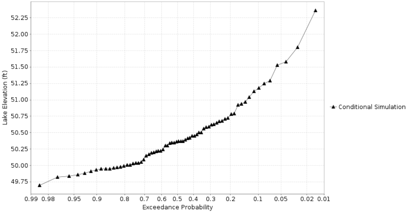
Probability of Rising to High Lake Levels on the Devils Lake at Devils Lake 5SW-Creel Bay (DCBN8) Forecast for the period 03/21/2022 - 09/30/2022 This is a conditional simulation based on the conditions as of 03/21/2022 Pumping schedule : 350cfs Jun 1 - Nov 10
