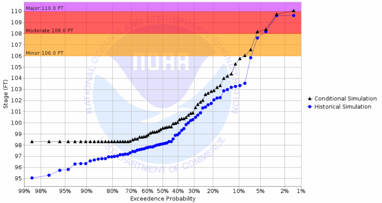
Chance of Exceeding River Stage at Snake River at Alvarado (ALVM5) Forecast for the period 08/01/2022 - 10/30/2022 This is a conditional simulation based on the conditions as of 07/25/2022
