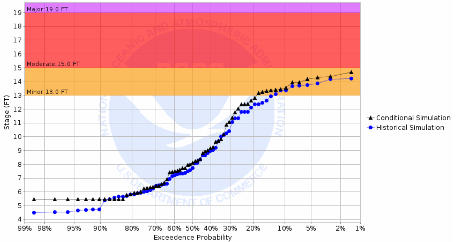
Chance of Exceeding River Stage at South Branch Buffalo River at Sabin 1E (SABM5) Forecast for the period 08/01/2022 - 10/30/2022 This is a conditional simulation based on the conditions as of 07/25/2022
