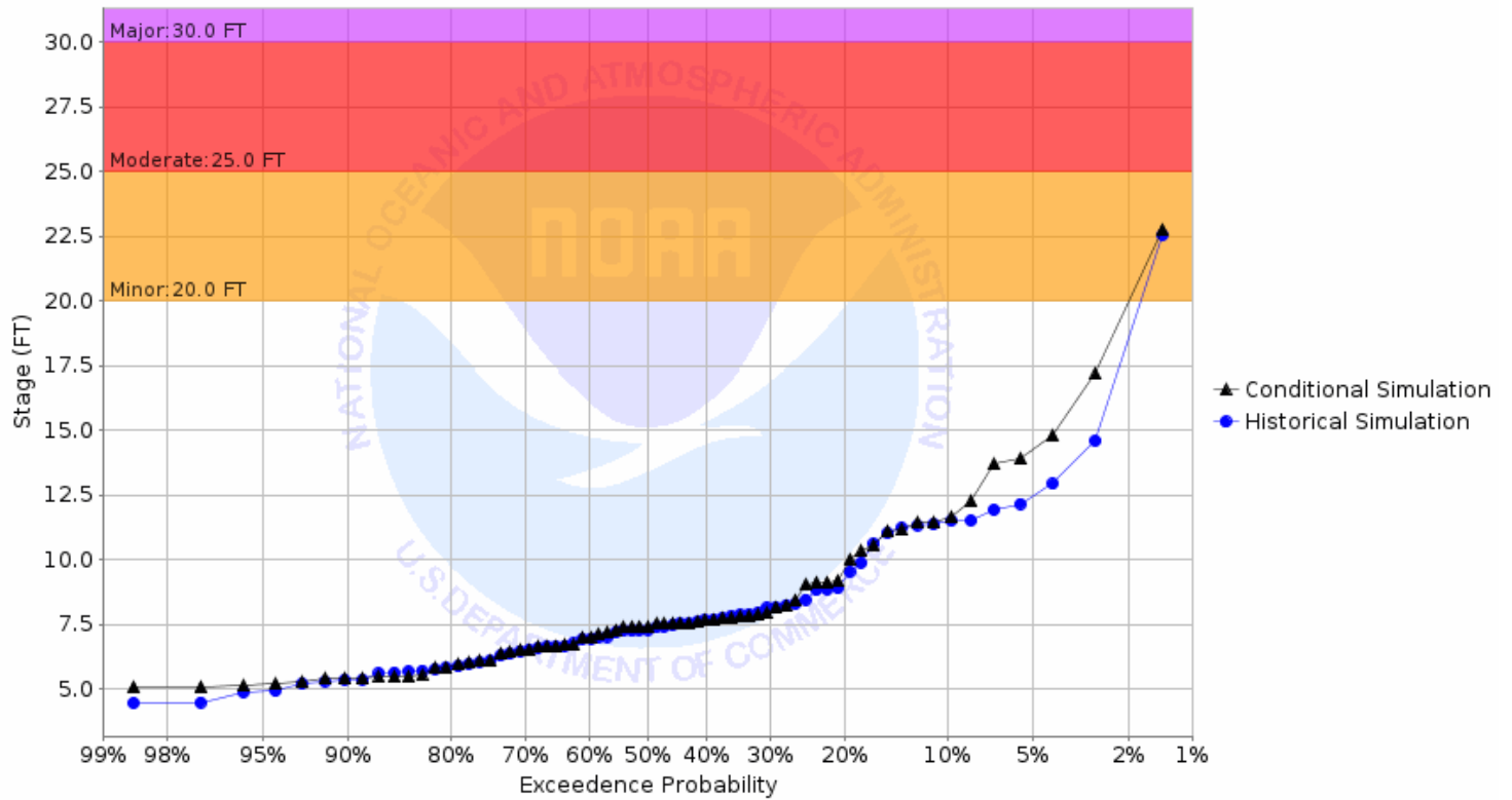
Chance of Exceeding River Stage at Sand Hill River at Climax (CLXM5) Forecast for the period 08/01/2022 - 10/30/2022 This is a conditional simulation based on the conditions as of 07/25/2022
