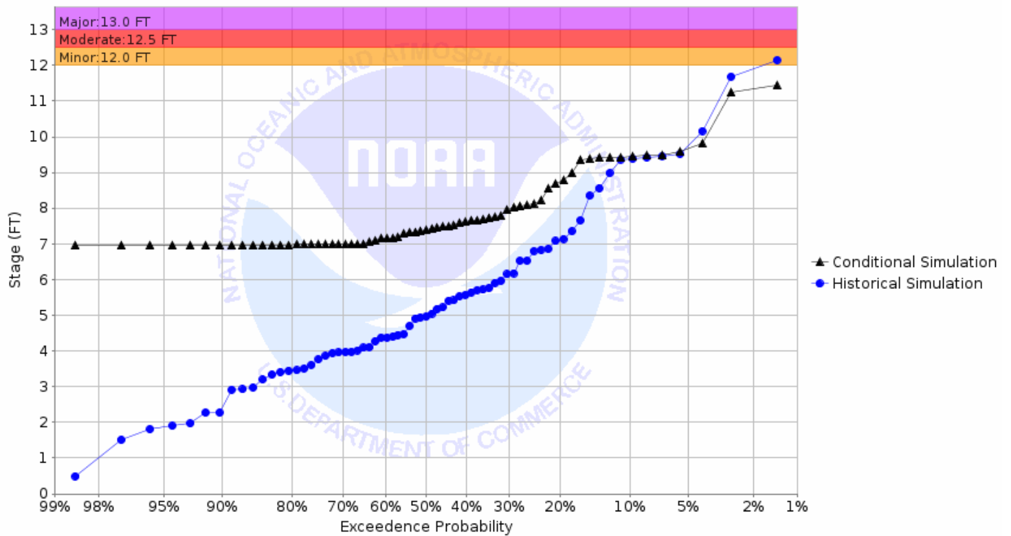
Chance of Exceeding River Stage at Red Lake River at High Landing (HIGM5) Forecast for the period 08/01/2022 - 10/30/2022 This is a conditional simulation based on the conditions as of 07/25/2022
