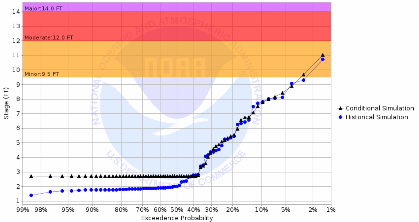
Chance of Exceeding River Stage at Maple River at Enderlin 1E (ENDN8) Forecast for the period 08/01/2022 - 10/30/2022 This is a conditional simulation based on the conditions as of 07/25/2022
