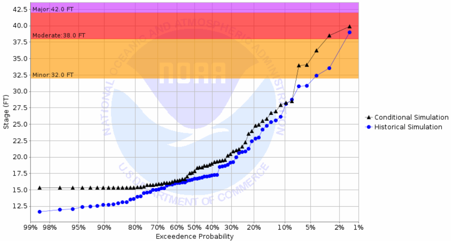
Chance of Exceeding River Stage at Red River of the North at Drayton 2NE - Hwy 66 Brdg (DRTN8) Forecast for the period 08/01/2022 - 10/30/2022 This is a conditional simulation based on the conditions as of 07/25/2022
