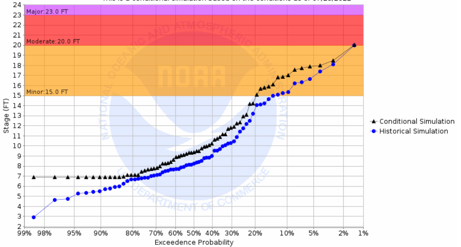
Chance of Exceeding River Stage at Red Lake River at Crookston (CRKM5) Forecast for the period 08/01/2022 - 10/30/2022 This is a conditional simulation based on the conditions as of 07/25/2022
