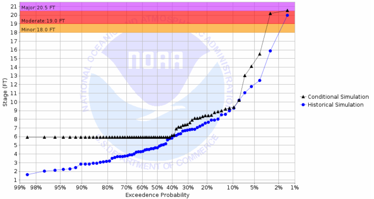
Chance of Exceeding River Stage at Pembina River at Neche (NCEN8) Forecast for the period 08/01/2022 - 10/30/2022 This is a conditional simulation based on the conditions as of 07/25/2022
