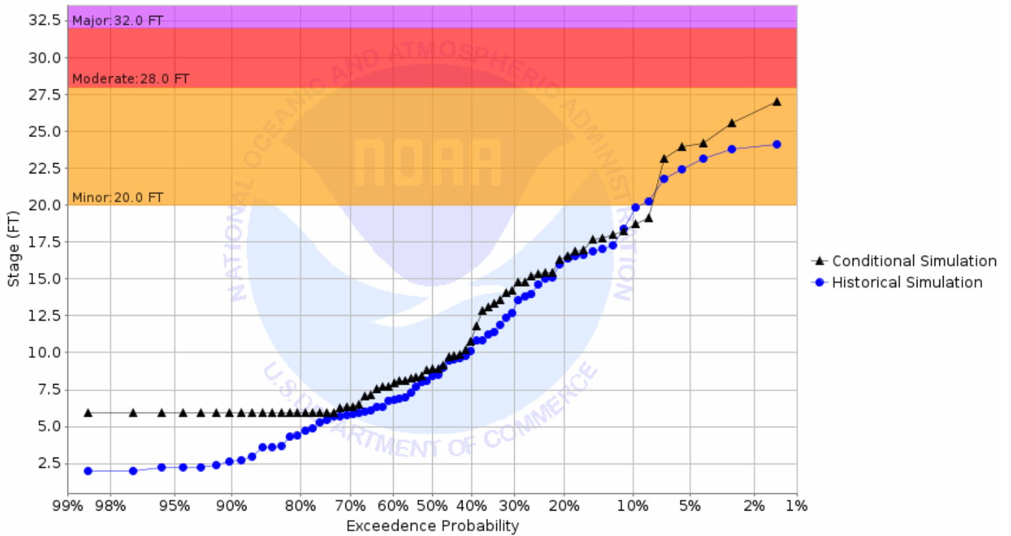
Chance of Exceeding River Stage at Wild Rice River at Hendrum (HNDM5) Forecast for the period 08/01/2022 - 10/30/2022 This is a conditional simulation based on the conditions as of 07/25/2022
