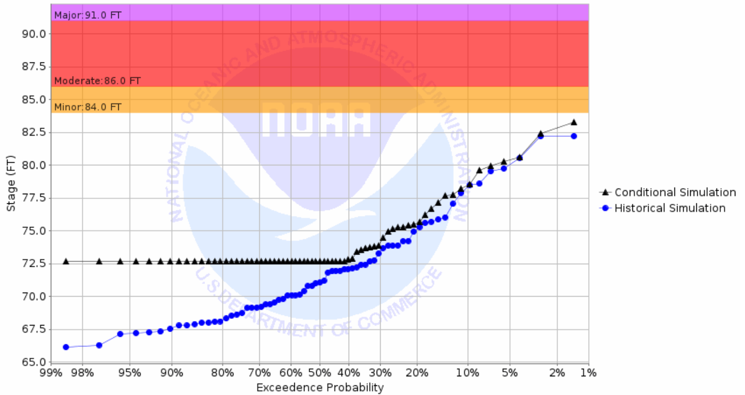
Chance of Exceeding River Stage at Sheyenne River at Harwood (HWDN8) Forecast for the period 08/01/2022 - 10/30/2022 This is a conditional simulation based on the conditions as of 07/25/2022
