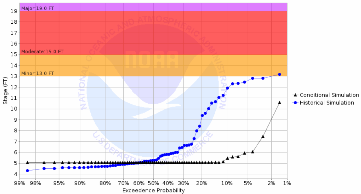
Chance of Exceeding River Stage at Buffalo River at Hawley 2SW (HWYM5) Forecast for the period 10/31/2022 - 01/29/2023 This is a conditional simulation based on the conditions as of 10/24/2022
