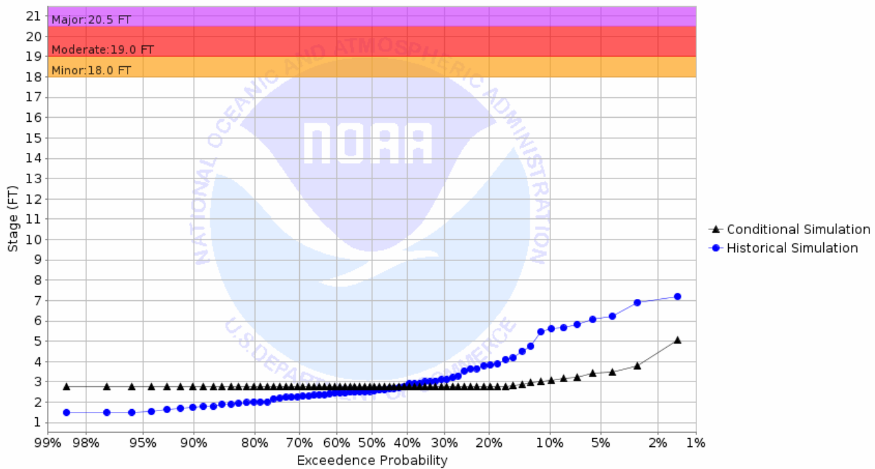
Chance of Exceeding River Stage at Pembina River at Neche (NCEN8) Forecast for the period 10/31/2022 - 01/29/2023 This is a conditional simulation based on the conditions as of 10/24/2022
