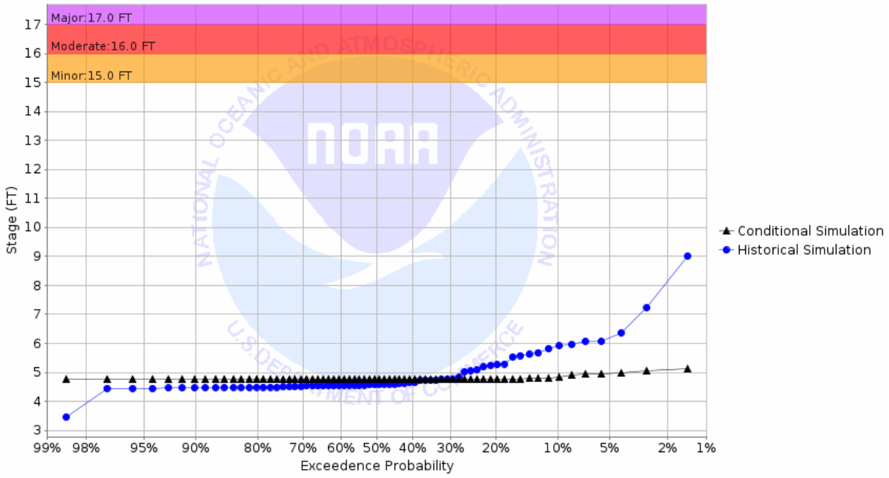
Chance of Exceeding River Stage at Sheyenne River at Valley City (VCRN8) Forecast for the period 10/31/2022 - 01/29/2023 This is a conditional simulation based on the conditions as of 10/24/2022
