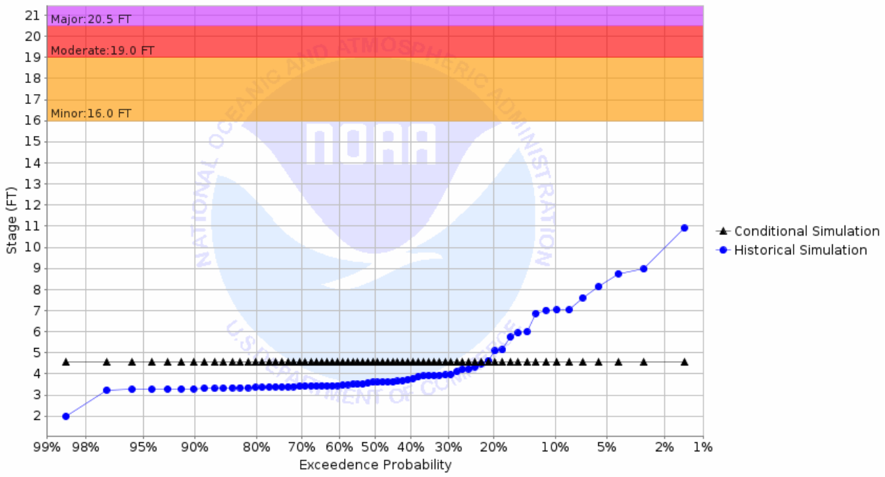
Chance of Exceeding River Stage at Sheyenne River Diversion at West Fargo (WF0N8) Forecast for the period 10/31/2022 - 01/29/2023 This is a conditional simulation based on the conditions as of 10/24/2022
