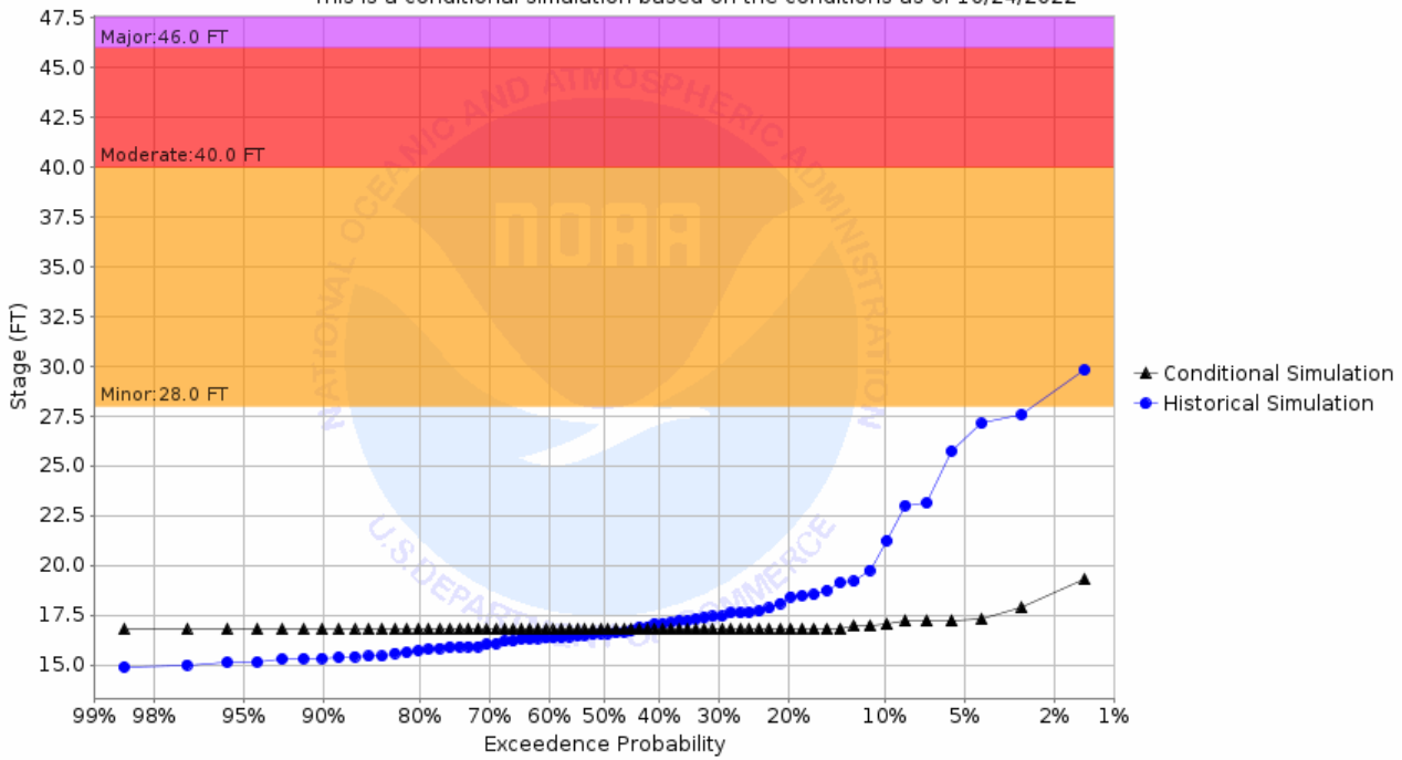
Chance of Exceeding River Stage at Red River of the North at Oslo (OSLM5) Forecast for the period 10/31/2022 - 01/29/2023 This is a conditional simulation based on the conditions as of 10/24/2022
