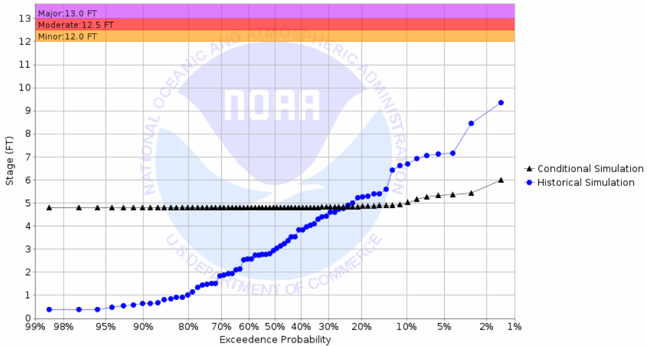
Chance of Exceeding River Stage at Red Lake River at High Landing (HIGM5) Forecast for the period 10/31/2022 - 01/29/2023 This is a conditional simulation based on the conditions as of 10/24/2022
