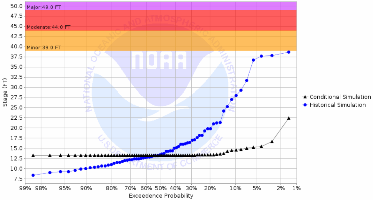
Chance of Exceeding River Stage at Red River of the North at Pembina (PBNN8) Forecast for the period 10/31/2022 - 01/29/2023 This is a conditional simulation based on the conditions as of 10/24/2022
