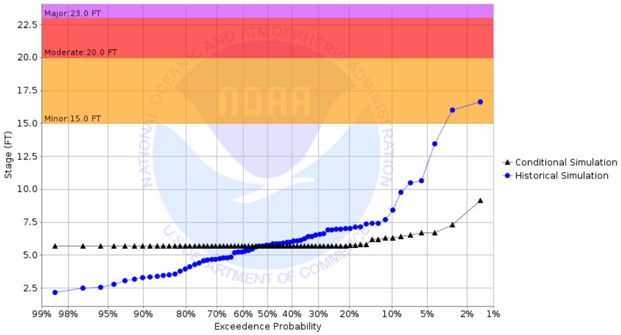
Chance of Exceeding River Stage at Snake River at Warren 3ENE-Morkassel Brdg (MKLM5) Forecast for the period 10/31/2022 - 01/29/2023 This is a conditional simulation based on the conditions as of 10/24/2022
