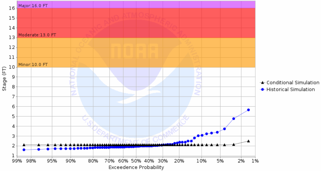
Chance of Exceeding River Stage at Goose River at Hillsboro (HGRN8) Forecast for the period 10/31/2022 - 01/29/2023 This is a conditional simulation based on the conditions as of 10/24/2022
