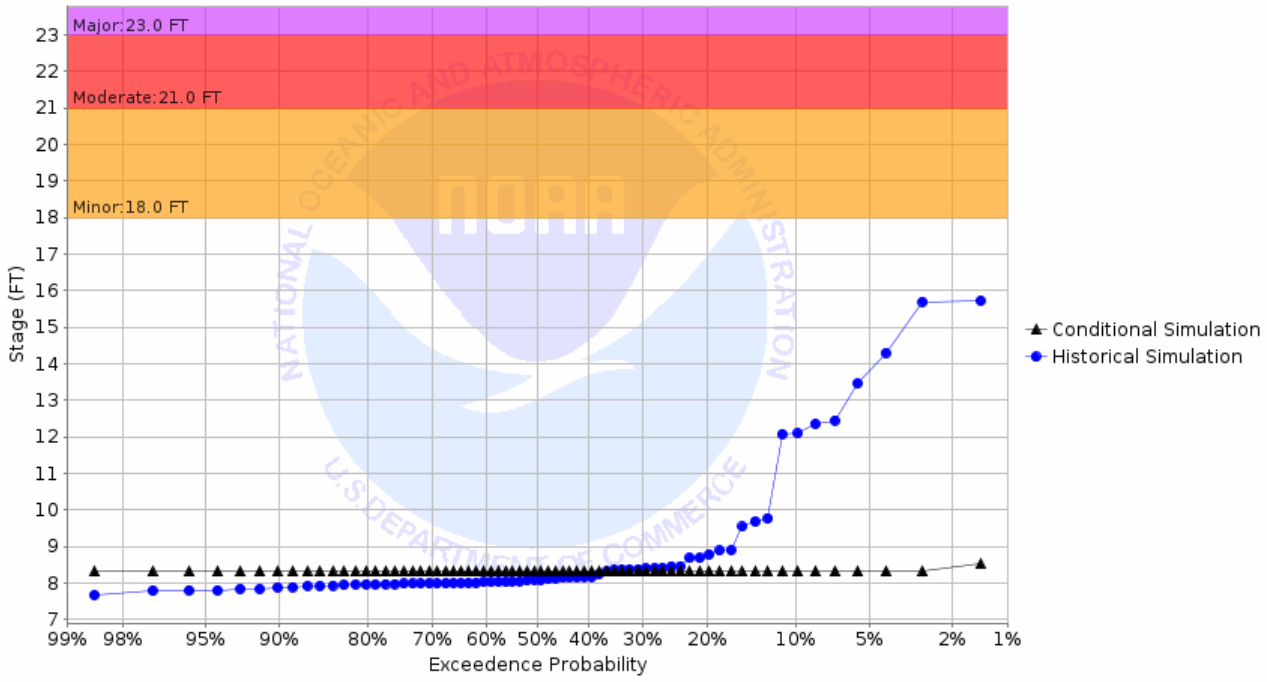
Chance of Exceeding River Stage at Maple River at Mapleton 3SW (MPLN8) Forecast for the period 10/31/2022 - 01/29/2023 This is a conditional simulation based on the conditions as of 10/24/2022
