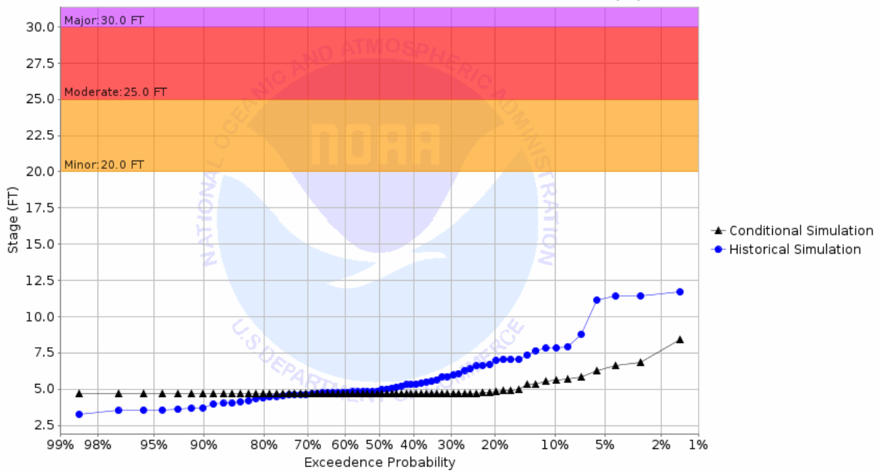
Chance of Exceeding River Stage at Red Lake River at High Landing (HIGM5) Forecast for the period 10/31/2022 - 01/29/2023 This is a conditional simulation based on the conditions as of 10/24/2022
