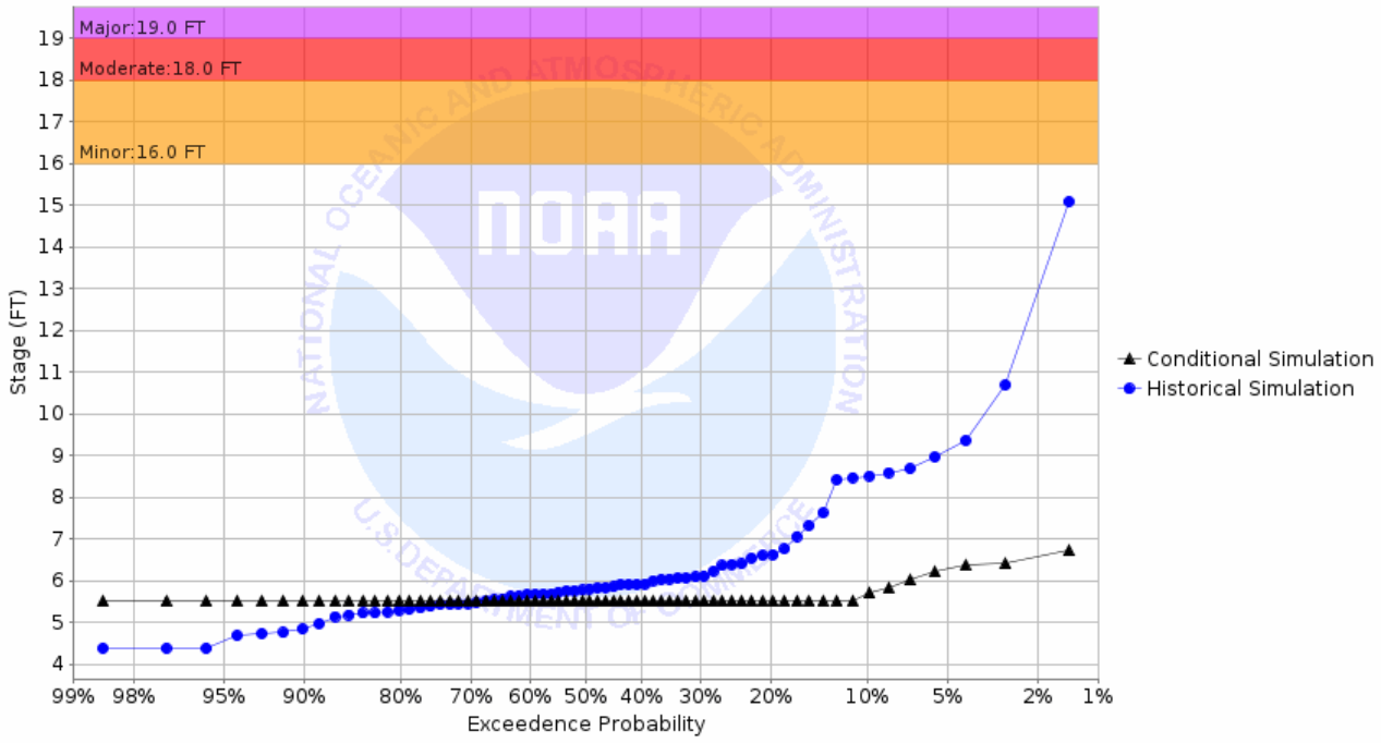
Chance of Exceeding River Stage at Roseau River at Roseau - Center St Brdg (ROSM5) Forecast for the period 10/31/2022 - 01/29/2023 This is a conditional simulation based on the conditions as of 10/24/2022
