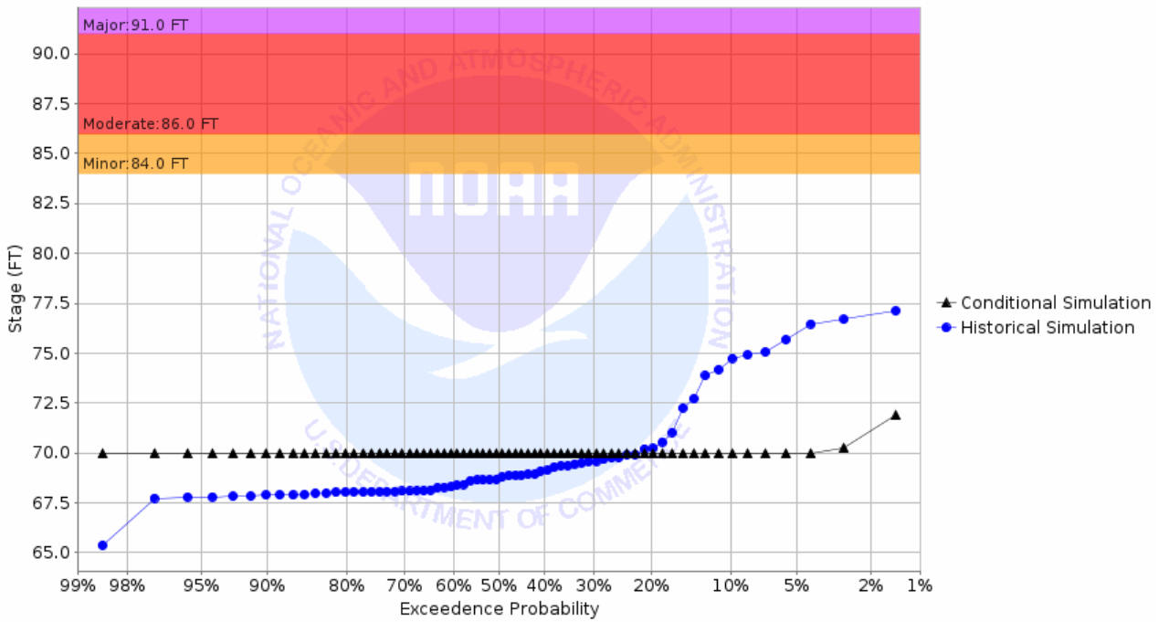
Chance of Exceeding River Stage at Sheyenne River at Harwood (HWDN8) Forecast for the period 10/31/2022 - 01/29/2023 This is a conditional simulation based on the conditions as of 10/24/2022
