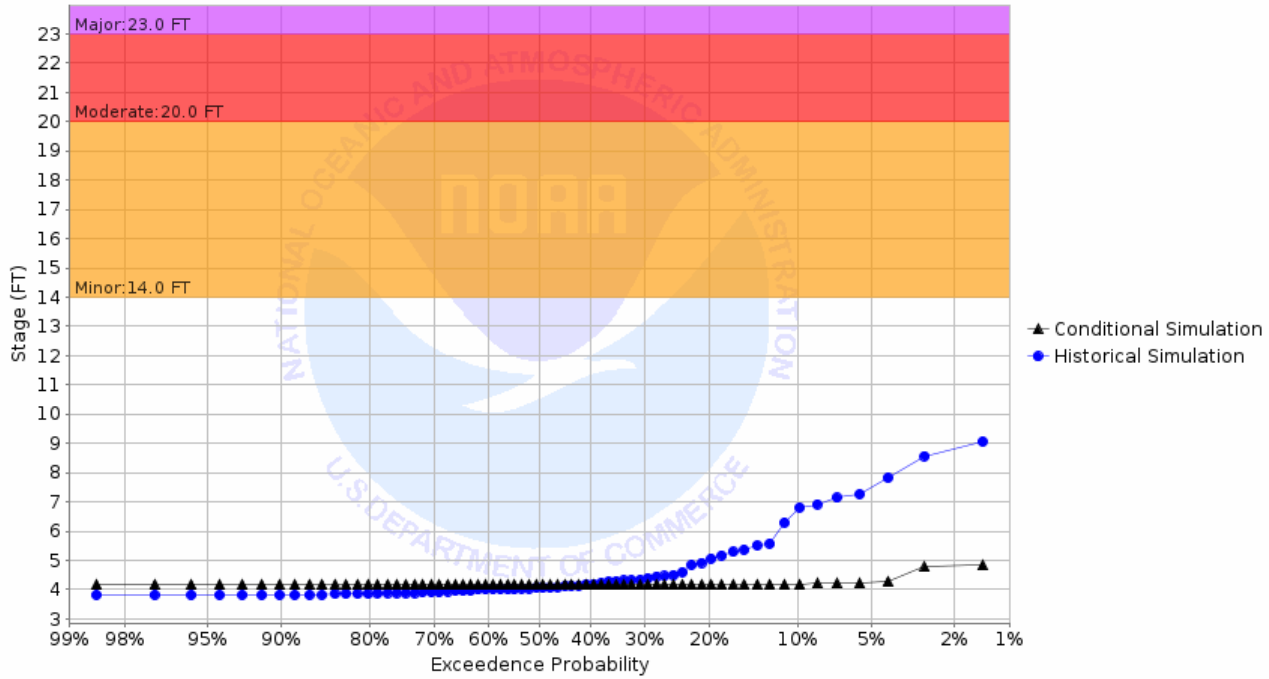
Chance of Exceeding River Stage at Marsh River at Shelly 4SE (SHYM5) Forecast for the period 10/31/2022 - 01/29/2023 This is a conditional simulation based on the conditions as of 10/24/2022
