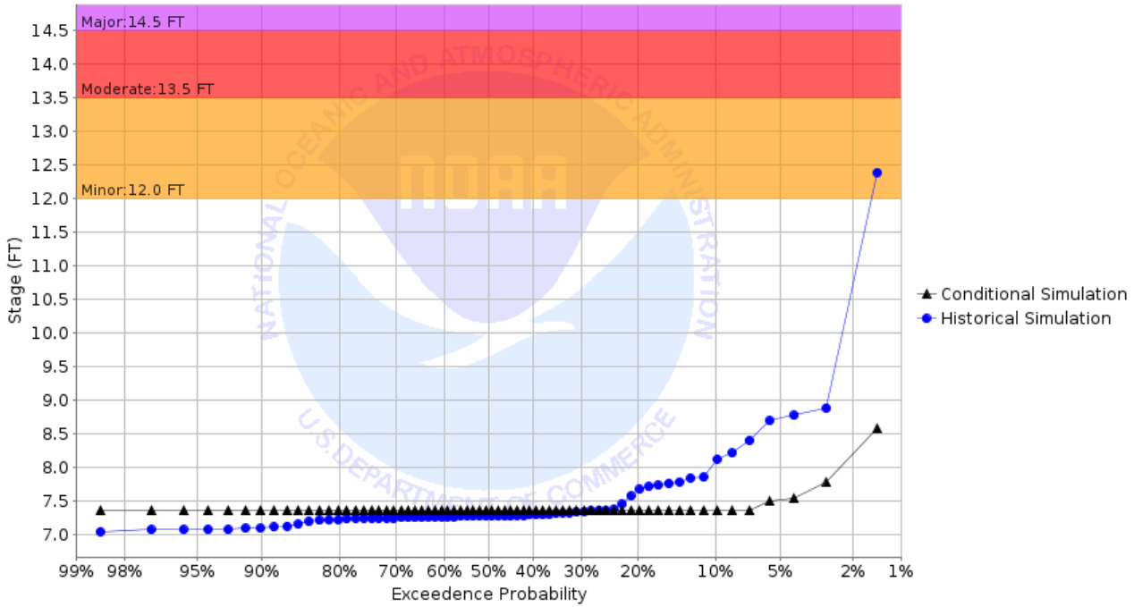
Chance of Exceeding River Stage at Park River at Grafton (GRNN8) Forecast for the period 10/31/2022 - 01/29/2023 This is a conditional simulation based on the conditions as of 10/24/2022
