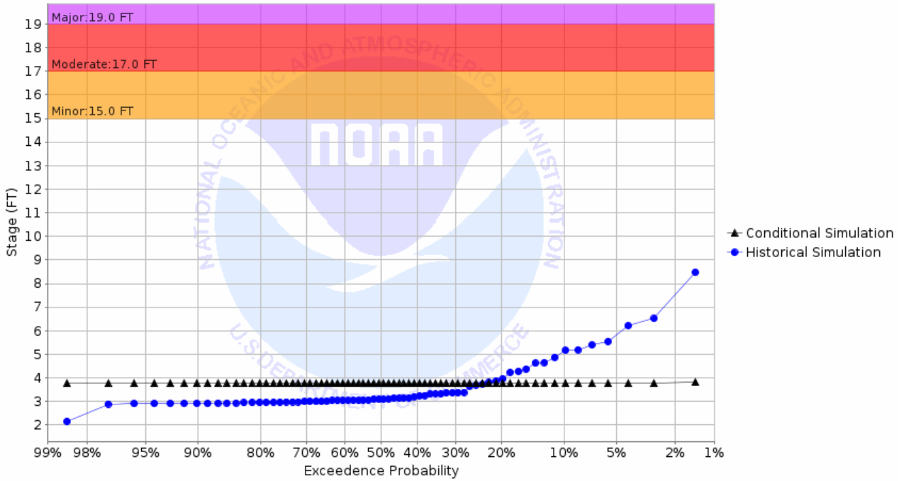
Chance of Exceeding River Stage at Sheyenne River at Lisbon (LBNN8) Forecast for the period 10/31/2022 - 01/29/2023 This is a conditional simulation based on the conditions as of 10/24/2022
