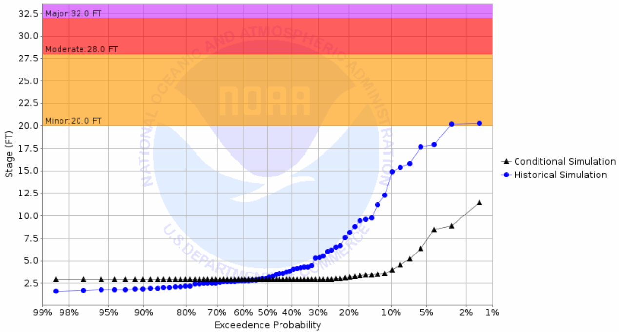
Chance of Exceeding River Stage at Wild Rice River at Hendrum (HNDM5) Forecast for the period 10/31/2022 - 01/29/2023 This is a conditional simulation based on the conditions as of 10/24/2022
