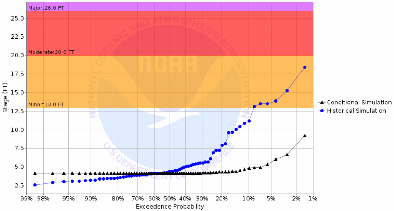
Chance of Exceeding River Stage at Buffalo River at Dilworth 7NE (DILM5) Forecast for the period 10/31/2022 - 01/29/2023 This is a conditional simulation based on the conditions as of 10/24/2022
