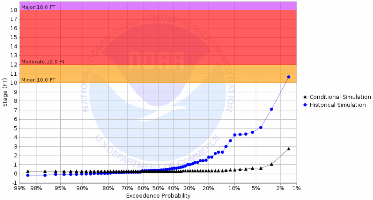
Chance of Exceeding River Stage at Wild Rice River at Abercrombie 2WNW (ABRN8) Forecast for the period 10/31/2022 - 01/29/2023 This is a conditional simulation based on the conditions as of 10/24/2022
