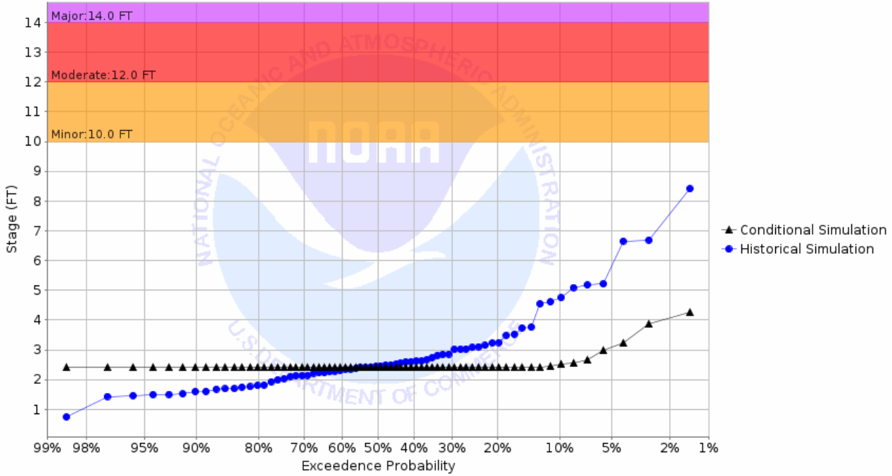
Chance of Exceeding River Stage at Wild Rice River at Twin Valley 1NE (TWVM5) Forecast for the period 10/31/2022 - 01/29/2023 This is a conditional simulation based on the conditions as of 10/24/2022
