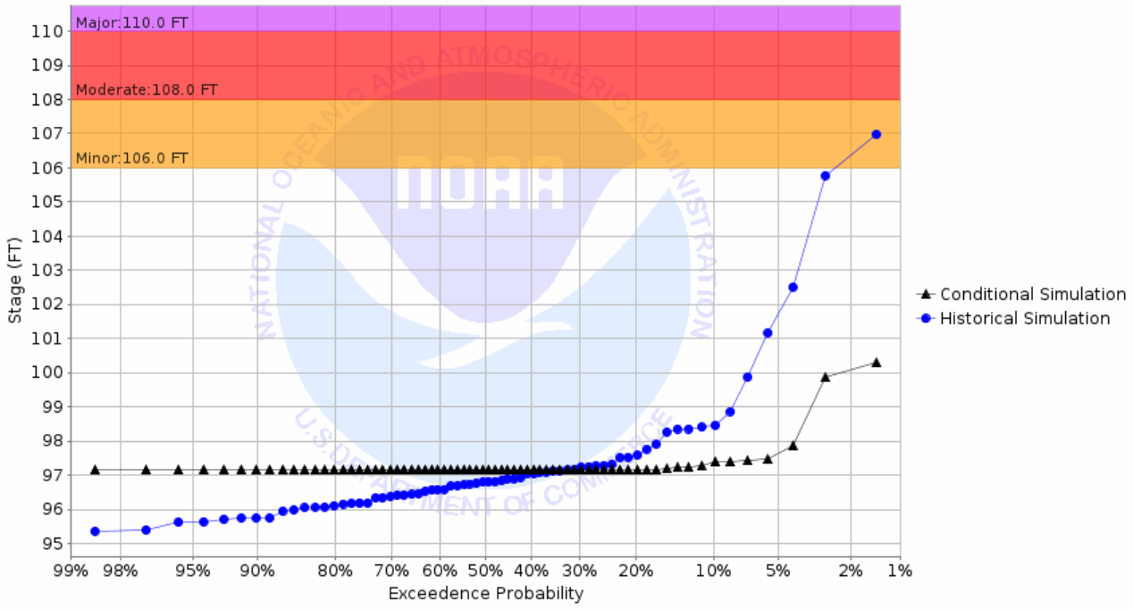
Chance of Exceeding River Stage at Snake River at Alvarado (ALVM5) Forecast for the period 10/31/2022 - 01/29/2023 This is a conditional simulation based on the conditions as of 10/24/2022
