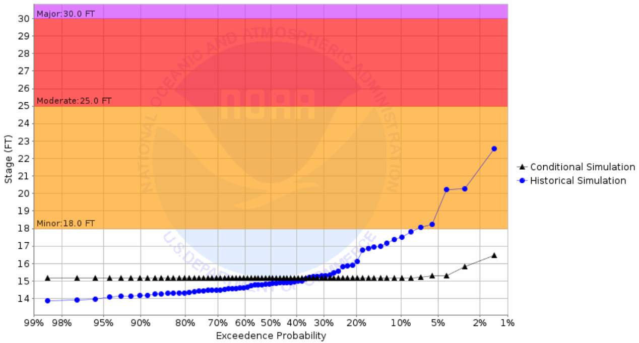
Chance of Exceeding River Stage at Red River of the North at Hillsboro 11ESE (Halstad MN) (HILN8) Forecast for the period 10/31/2022 - 01/29/2023 This is a conditional simulation based on the conditions as of 10/24/2022
