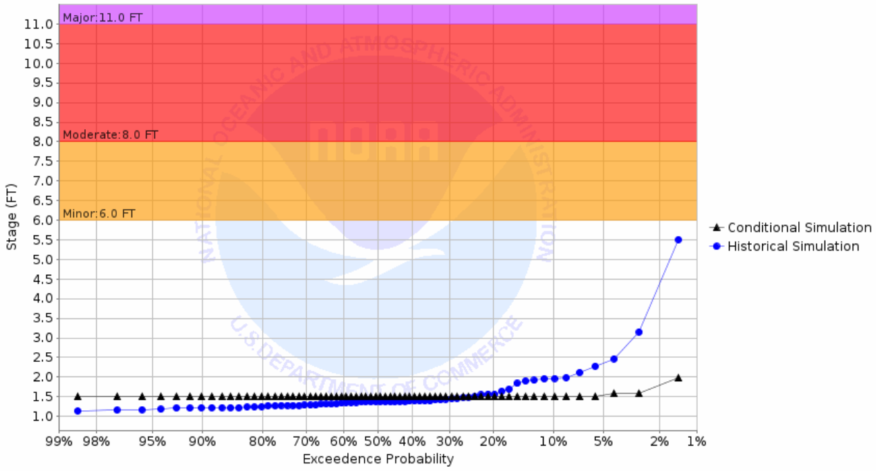
Chance of Exceeding River Stage at Forest River at Minto (MTON8) Forecast for the period 10/31/2022 - 01/29/2023 This is a conditional simulation based on the conditions as of 10/24/2022
