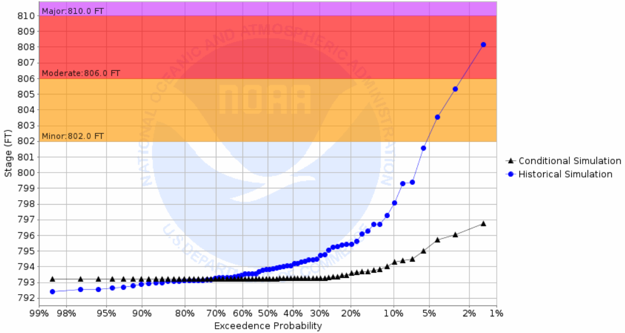
Chance of Exceeding River Stage at Two Rivers River at Hallock (HLLM5) Forecast for the period 10/31/2022 - 01/29/2023 This is a conditional simulation based on the conditions as of 10/24/2022
