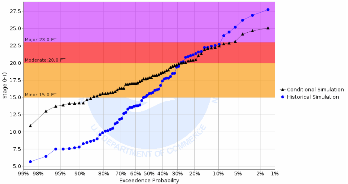
Chance of Exceeding River Stage at Red Lake River at Crookston (CRKM5) Forecast for the period 03/27/2023 - 06/25/2023 This is a conditional simulation based on the conditions as of 03/20/2023
