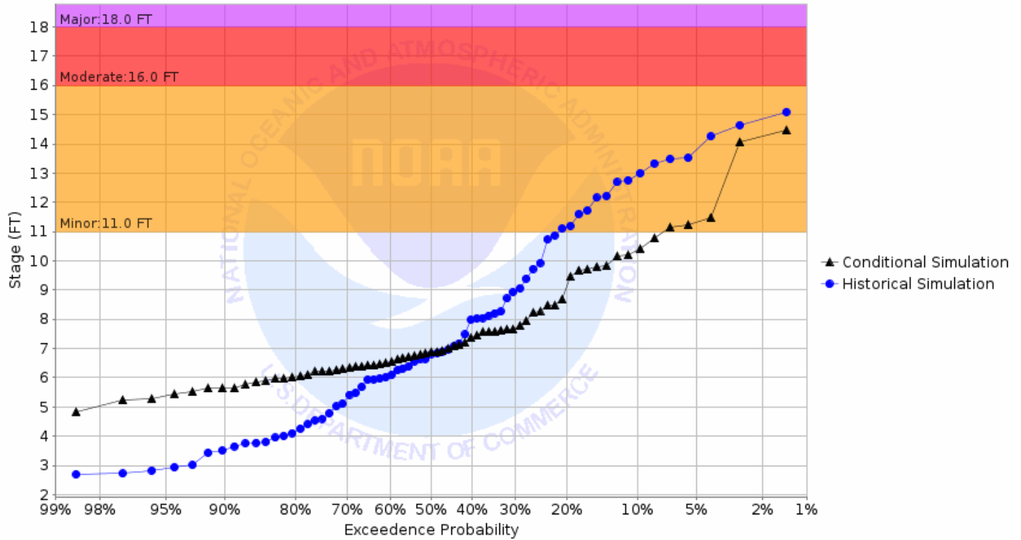
Chance of Exceeding River Stage at Pembina River at Walhalla (WLHN8) Forecast for the period 03/27/2023 - 06/25/2023 This is a conditional simulation based on the conditions as of 03/20/2023
