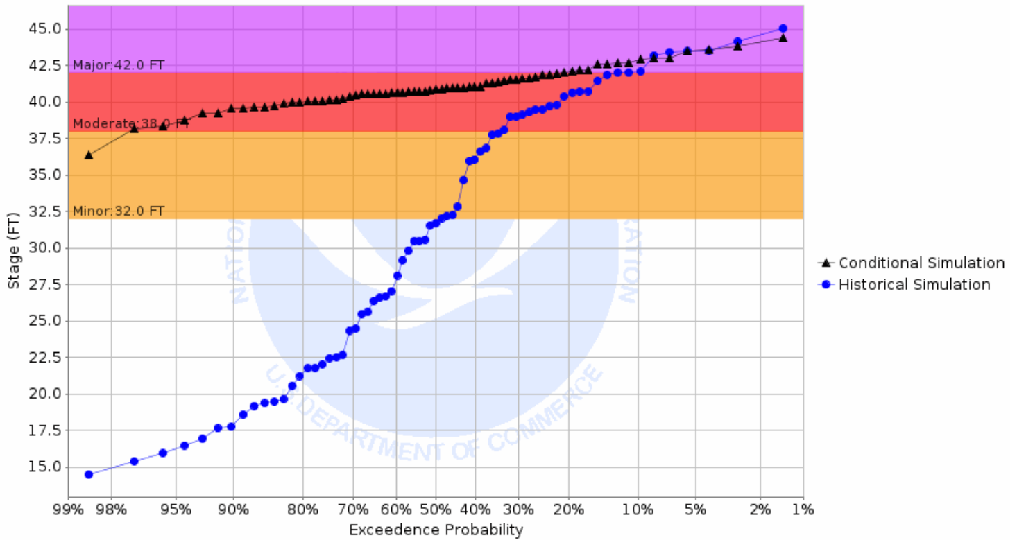
Chance of Exceeding River Stage at Red River of the North at Drayton 2NE - Hwy 66 Brdg (DRTN8) Forecast for the period 03/27/2023 - 06/25/2023 This is a conditional simulation based on the conditions as of 03/20/2023
