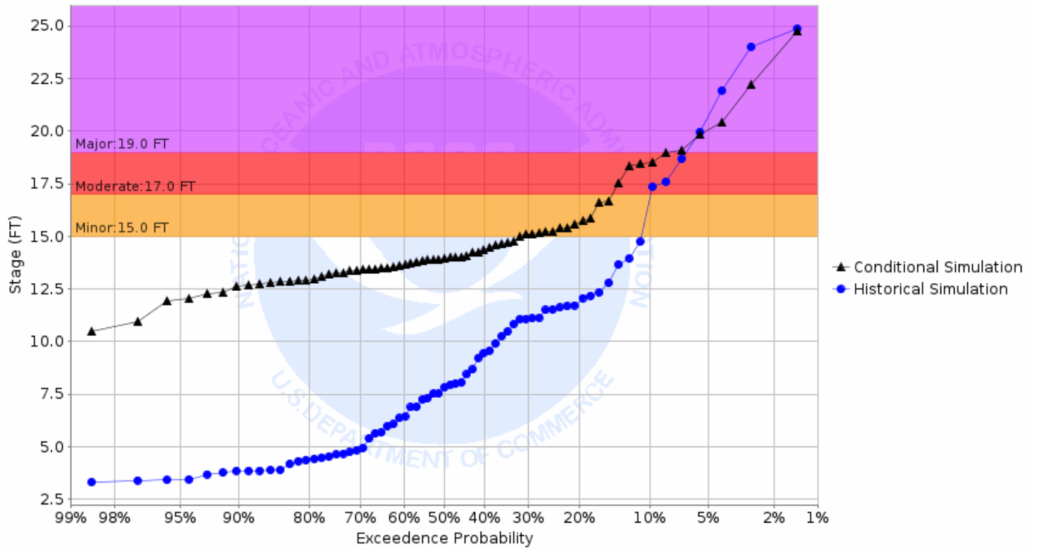
Chance of Exceeding River Stage at Sheyenne River at Lisbon (LBNN8) Forecast for the period 03/27/2023 - 06/25/2023 This is a conditional simulation based on the conditions as of 03/20/2023
