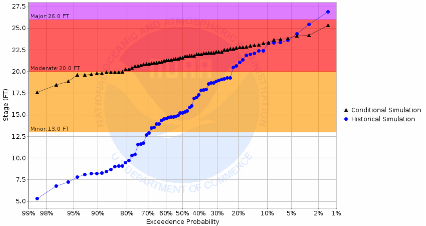
Chance of Exceeding River Stage at Buffalo River at Dilworth 7NE (DILM5) Forecast for the period 03/27/2023 - 06/25/2023 This is a conditional simulation based on the conditions as of 03/20/2023
