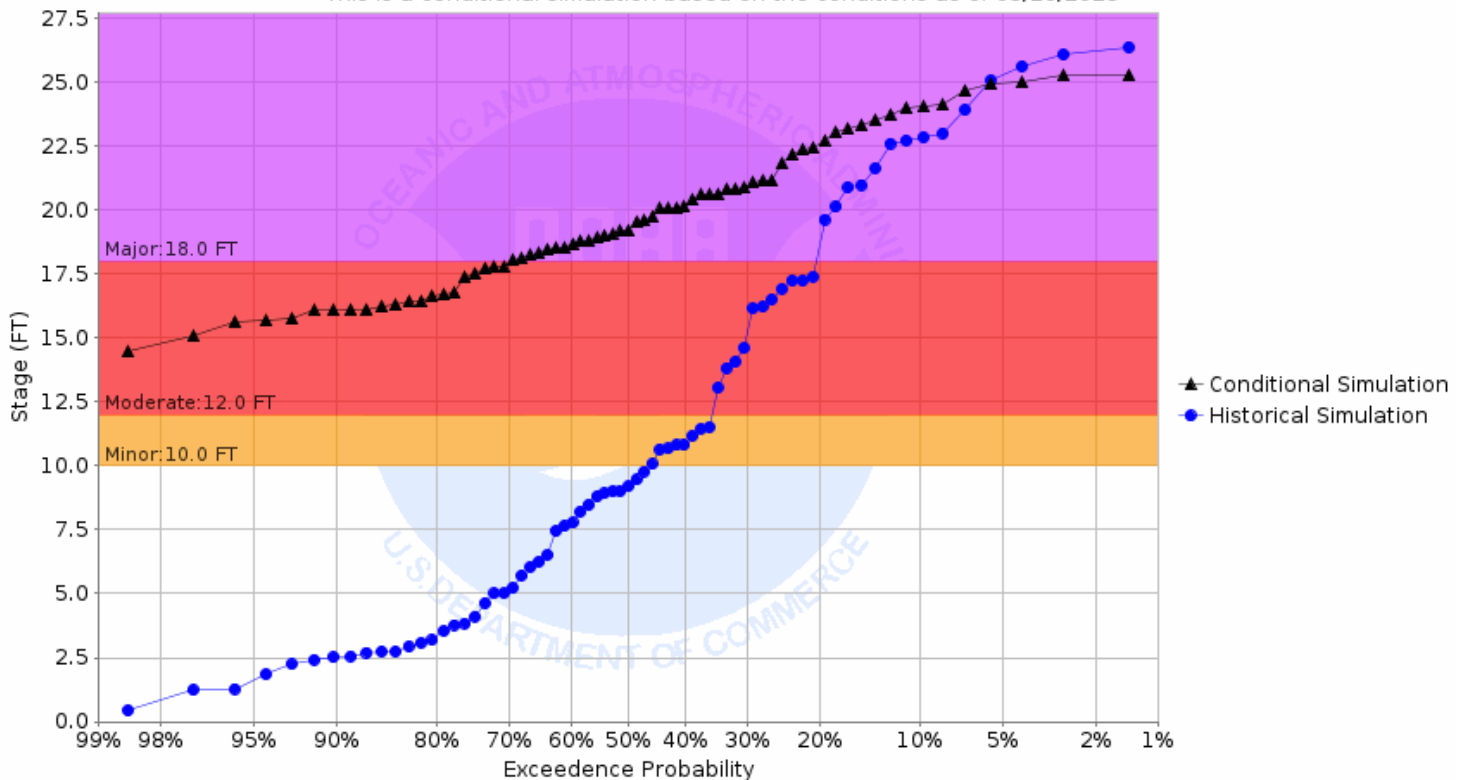
Chance of Exceeding River Stage at Wild Rice River at Abercrombie 2WNW (ABRN8) Forecast for the period 03/27/2023 - 06/25/2023 This is a conditional simulation based on the conditions as of 03/20/2023
