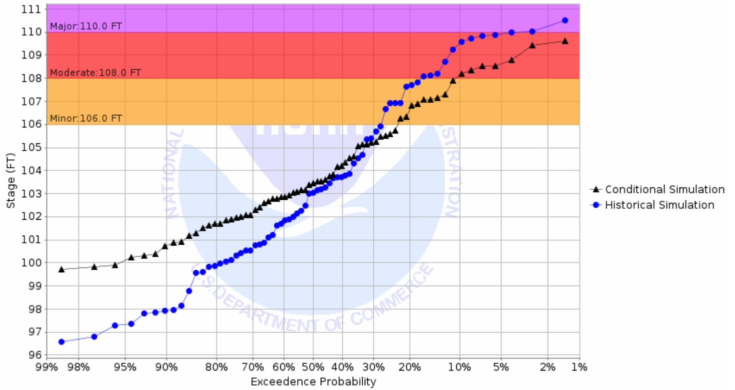
Chance of Exceeding River Stage at Snake River at Alvarado (ALVM5) Forecast for the period 03/27/2023 - 06/25/2023 This is a conditional simulation based on the conditions as of 03/20/2023
