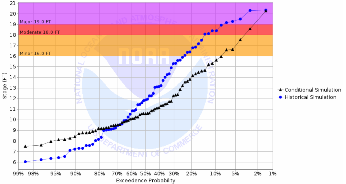
Chance of Exceeding River Stage at Roseau River at Roseau - Center St Brdg (ROSM5) Forecast for the period 03/27/2023 - 06/25/2023 This is a conditional simulation based on the conditions as of 03/20/2023
