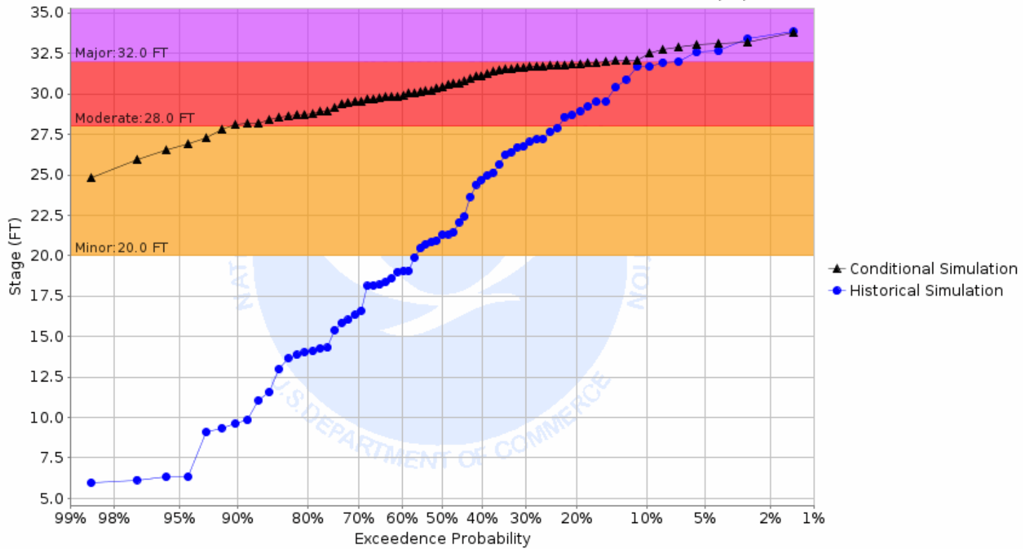
Chance of Exceeding River Stage at Wild Rice River at Hendrum (HNDM5) Forecast for the period 03/27/2023 - 06/25/2023 This is a conditional simulation based on the conditions as of 03/20/2023
