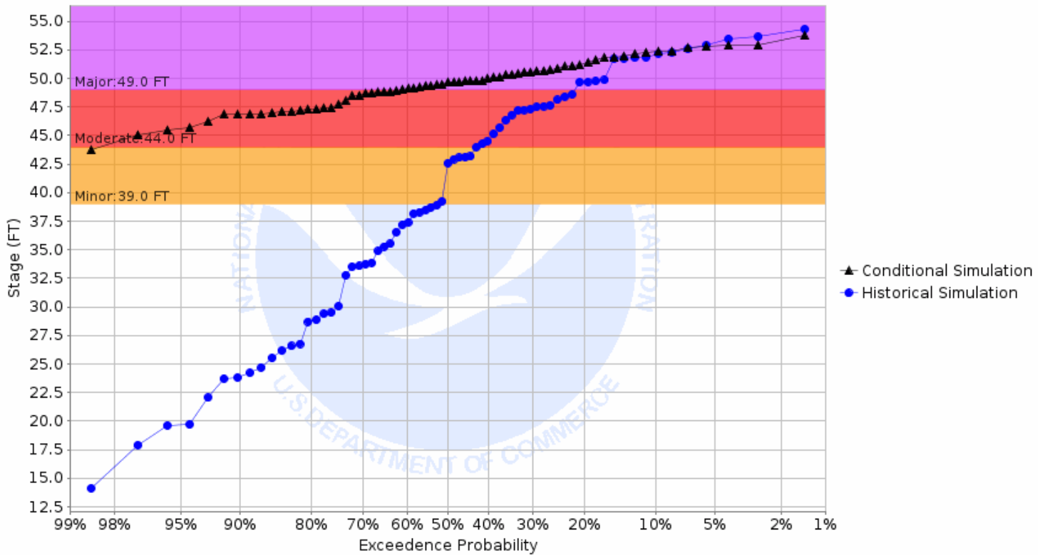
Chance of Exceeding River Stage at Red River of the North at Pembina (PBNN8) Forecast for the period 03/27/2023 - 06/25/2023 This is a conditional simulation based on the conditions as of 03/20/2023
