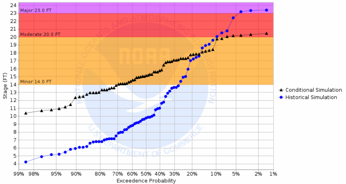
Chance of Exceeding River Stage at Marsh River at Shelly 4SE (SHYM5) Forecast for the period 03/27/2023 - 06/25/2023 This is a conditional simulation based on the conditions as of 03/20/2023
