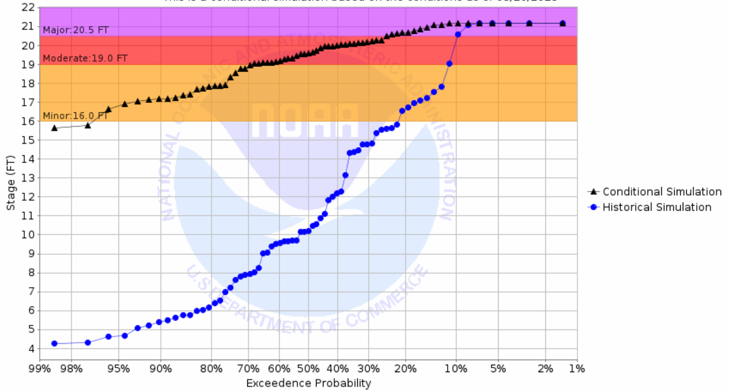
Chance of Exceeding River Stage at Sheyenne River at Kindred 2SE (KNDN8) Forecast for the period 03/27/2023 - 06/25/2023 This is a conditional simulation based on the conditions as of 03/20/2023
