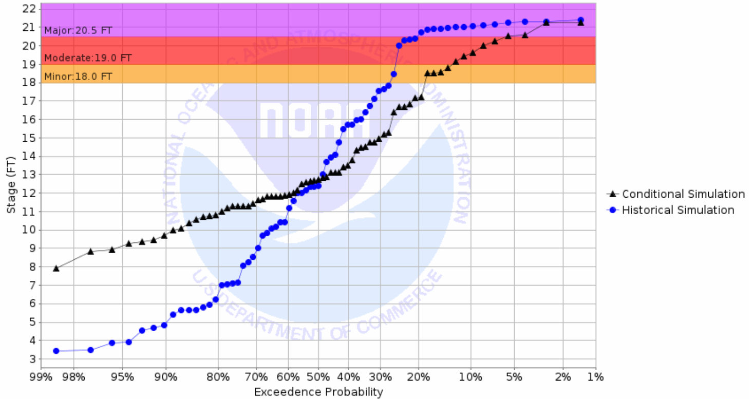
Chance of Exceeding River Stage at Pembina River at Neche (NCEN8) Forecast for the period 03/27/2023 - 06/25/2023 This is a conditional simulation based on the conditions as of 03/20/2023
