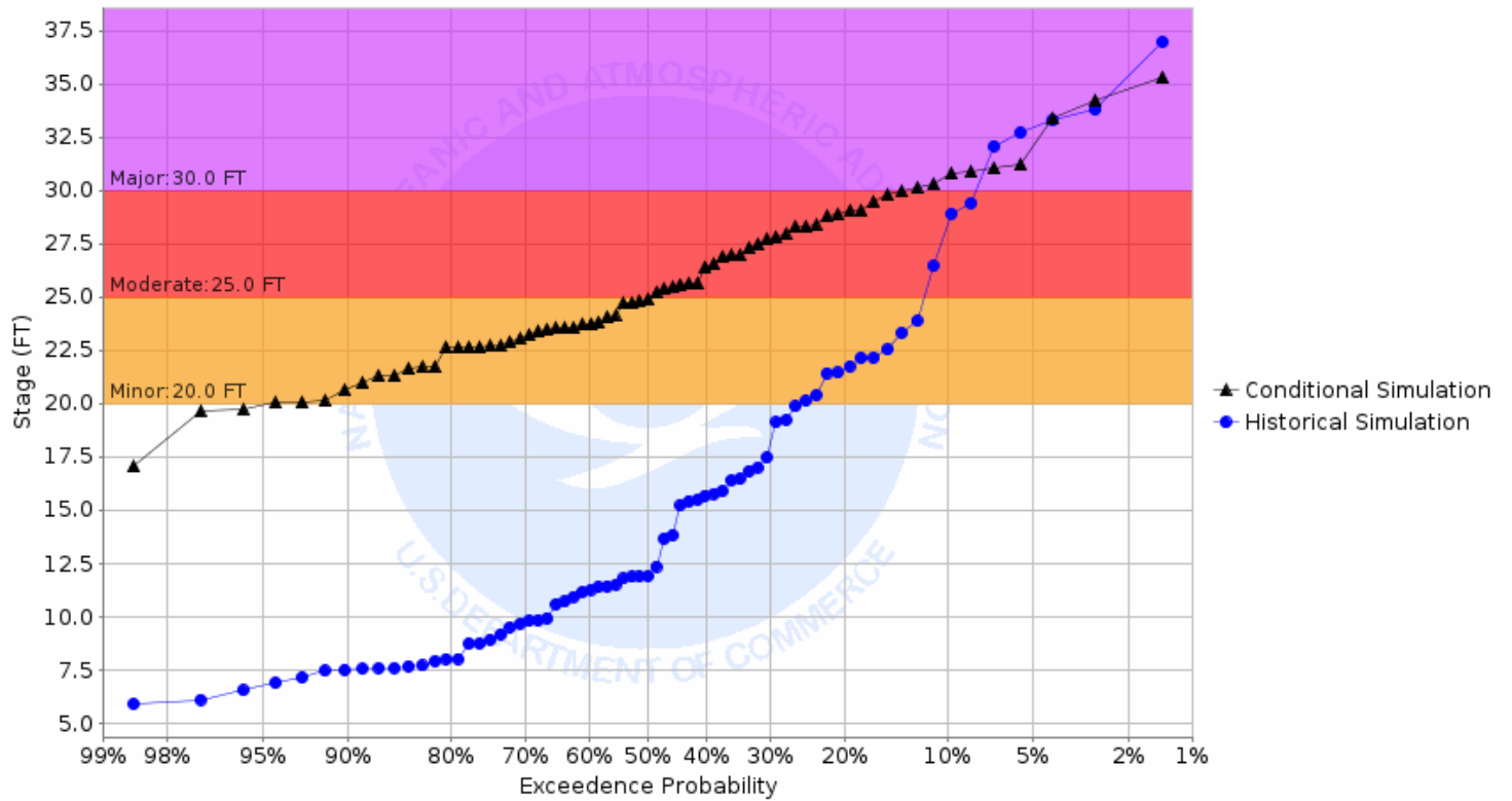
Chance of Exceeding River Stage at Sand Hill River at Climax (CLXM5) Forecast for the period 03/27/2023 - 06/25/2023 This is a conditional simulation based on the conditions as of 03/20/2023
