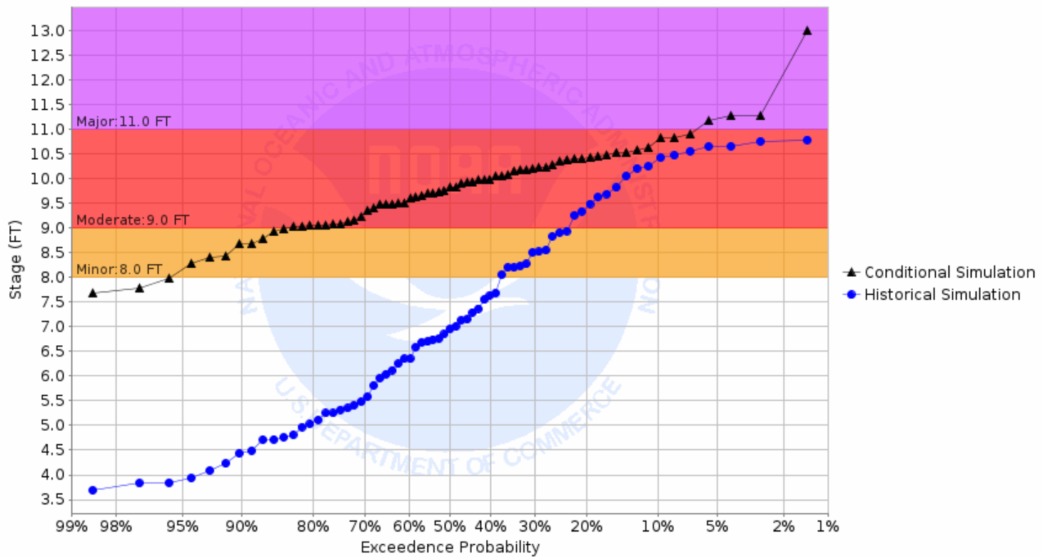
Chance of Exceeding River Stage at Buffalo River at Hawley 2SW (HWY5) Forecast for the period 03/27/2023 - 06/25/2023 This is a conditional simulation based on the conditions as of 03/20/2023
