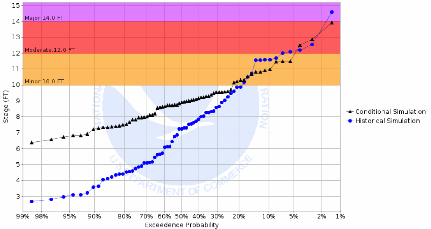
Chance of Exceeding River Stage at Wild Rice River at Twin Valley 1NE (TWVM5) Forecast for the period 03/27/2023 - 06/25/2023 This is a conditional simulation based on the conditions as of 03/20/2023
