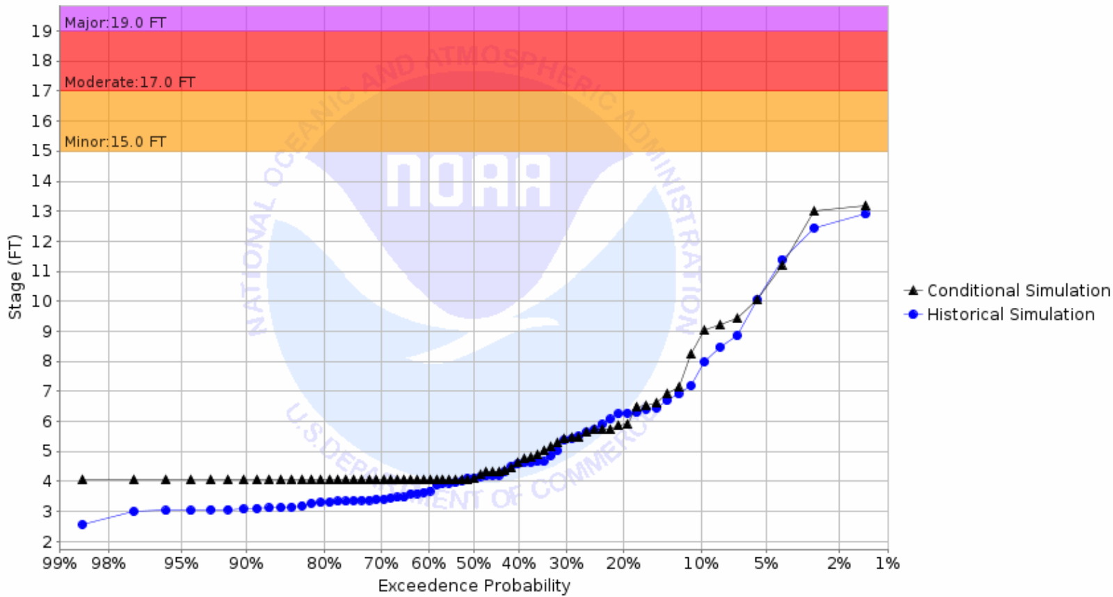
Chance of Exceeding River Stage at Sheyenne River at Lisbon (LBNN8) Forecast for the period 08/28/2023 - 11/26/2023 This is a conditional simulation based on the conditions as of 08/21/2023
