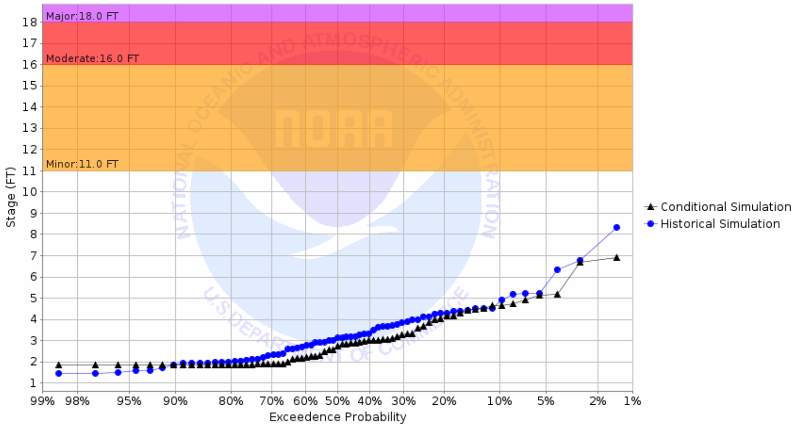
Chance of Exceeding River Stage at Pembina River at Walhalla (WLHN8) Forecast for the period 08/28/2023 - 11/26/2023 This is a conditional simulation based on the conditions as of 08/21/2023
