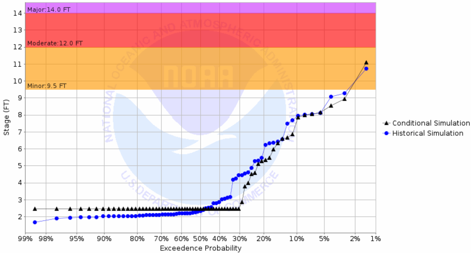
Chance of Exceeding River Stage at Maple River at Enderlin 1E (ENDN8) Forecast for the period 08/28/2023 - 11/26/2023 This is a conditional simulation based on the conditions as of 08/21/2023
