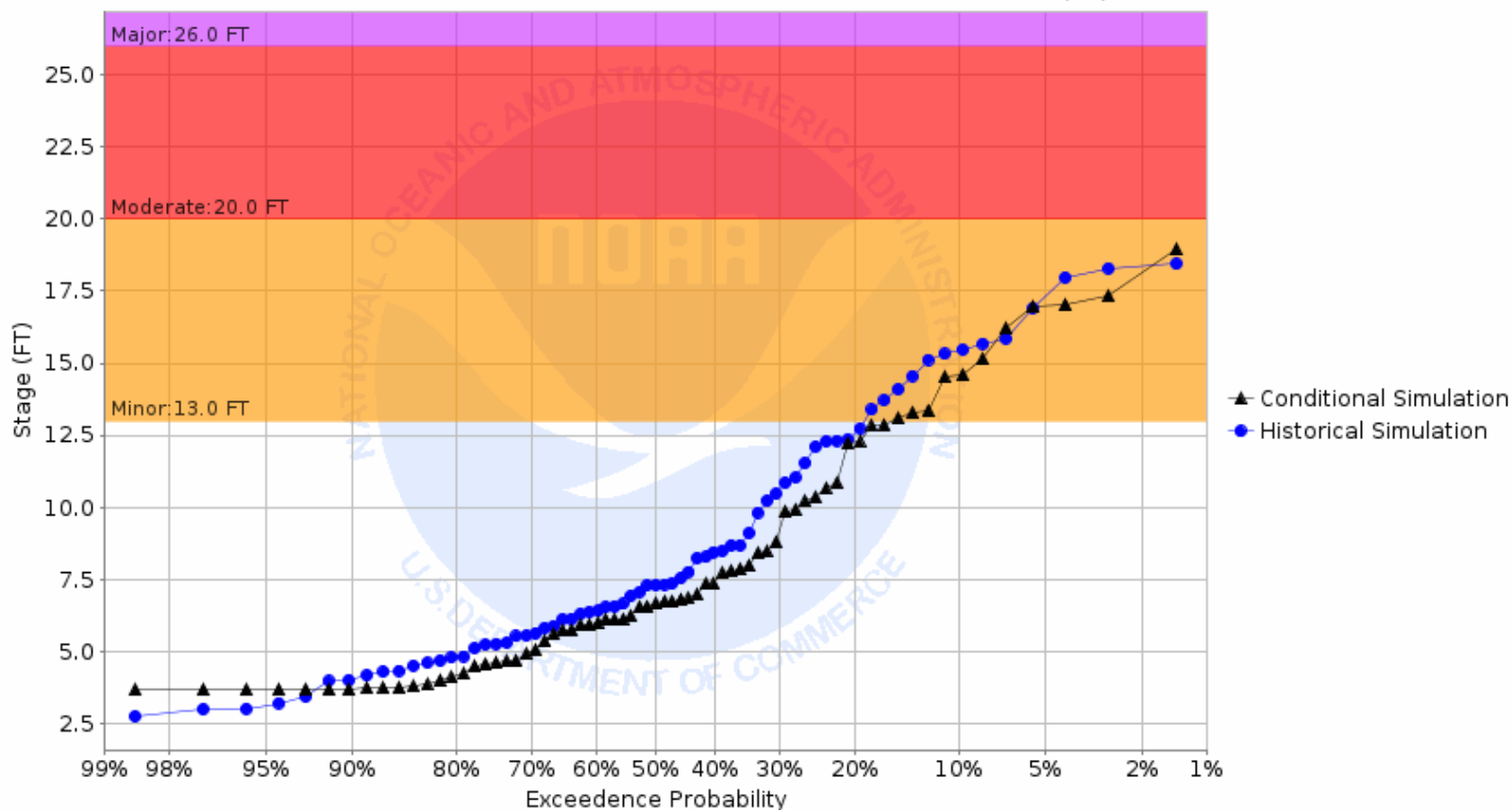
Chance of Exceeding River Stage at Buffalo River at Dilworth 7NE (DILM5) Forecast for the period 08/28/2023 - 11/26/2023 This is a conditional simulation based on the conditions as of 08/21/2023
