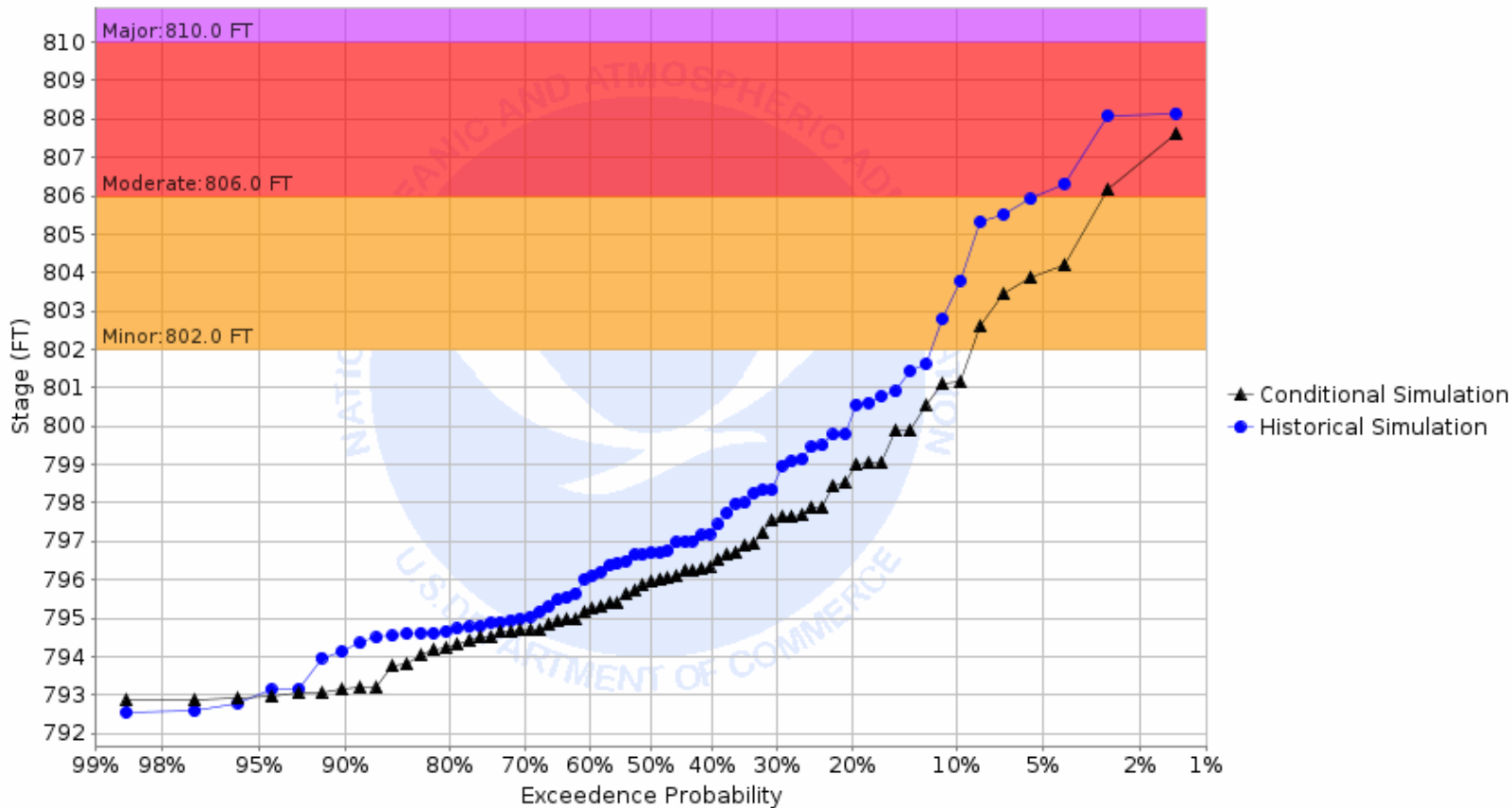
Chance of Exceeding River Stage at Two Rivers River at Hallock (HLLM5) Forecast for the period 08/28/2023 - 11/26/2023 This is a conditional simulation based on the conditions as of 08/21/2023
