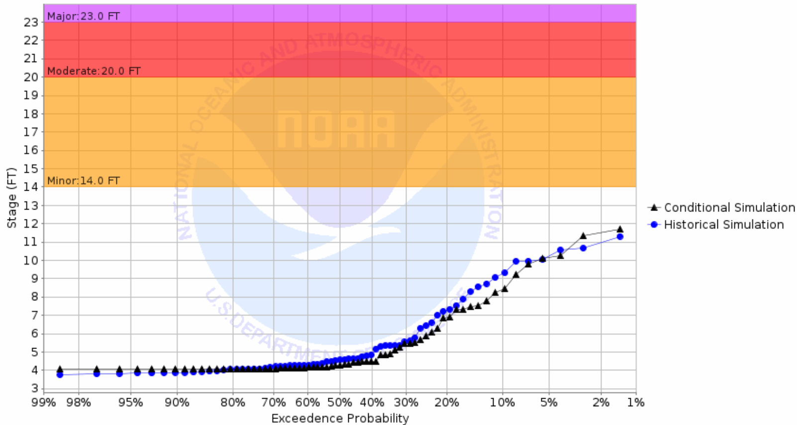
Chance of Exceeding River Stage at Marsh River at Shelly 4SE (SHYM5) Forecast for the period 08/28/2023 - 11/26/2023 This is a conditional simulation based on the conditions as of 08/21/2023
