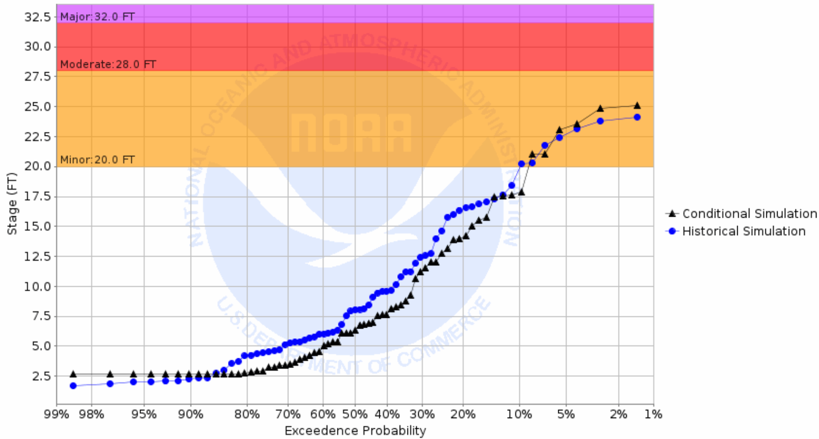
Chance of Exceeding River Stage at Wild Rice River at Hendrum (HNDM5) Forecast for the period 08/28/2023 - 11/26/2023 This is a conditional simulation based on the conditions as of 08/21/2023
