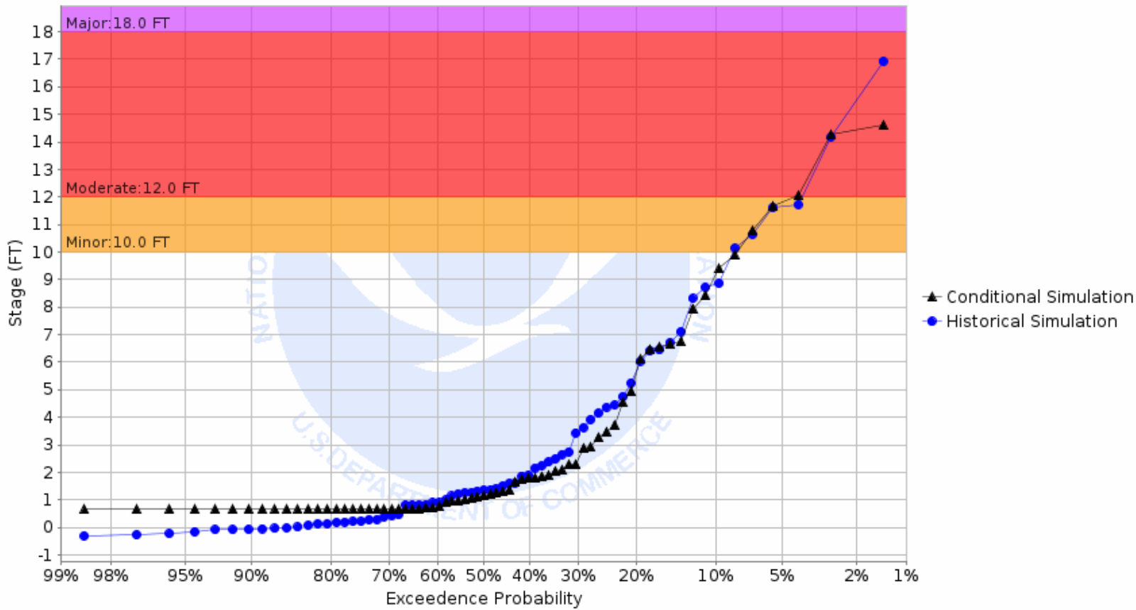
Chance of Exceeding River Stage at Wild Rice River at Abercrombie 2WNW (ABRN8) Forecast for the period 08/28/2023 - 11/26/2023 This is a conditional simulation based on the conditions as of 08/21/2023
