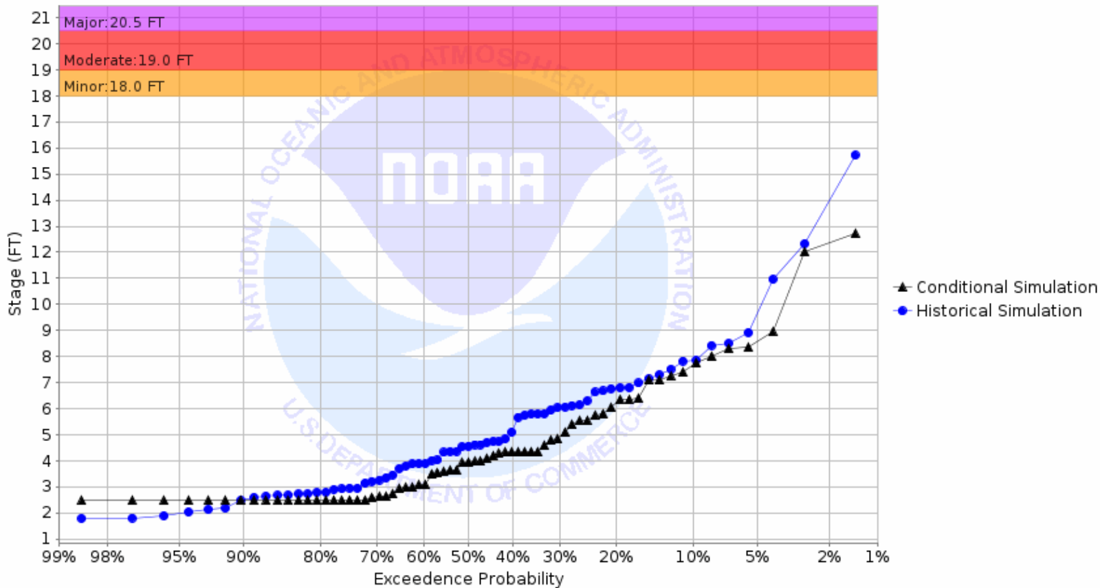
Chance of Exceeding River Stage at Pembina River at Neche (NCEN8) Forecast for the period 08/28/2023 - 11/26/2023 This is a conditional simulation based on the conditions as of 08/21/2023
