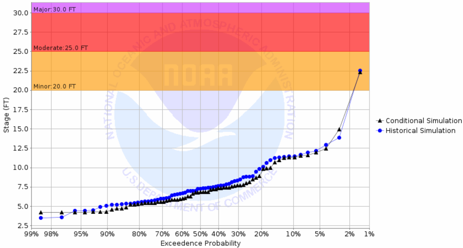
Chance of Exceeding River Stage at Sand Hill River at Climax (CLXM5) Forecast for the period 08/28/2023 - 11/26/2023 This is a conditional simulation based on the conditions as of 08/21/2023
