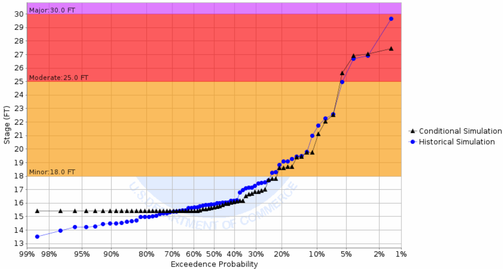
Chance of Exceeding River Stage at Red River of the North at Fargo WTP (FGON8) Forecast for the period 08/28/2023 - 11/26/2023 This is a conditional simulation based on the conditions as of 08/21/2023
