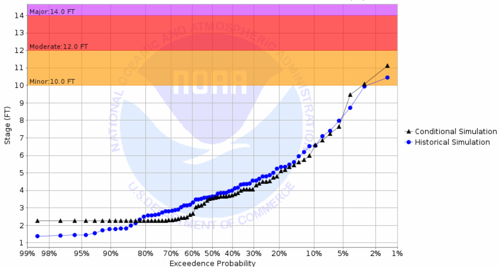
Chance of Exceeding River Stage at Wild Rice River at Twin Valley 1NE (TWVM5) Forecast for the period 08/28/2023 - 11/26/2023 This is a conditional simulation based on the conditions as of 08/21/2023
