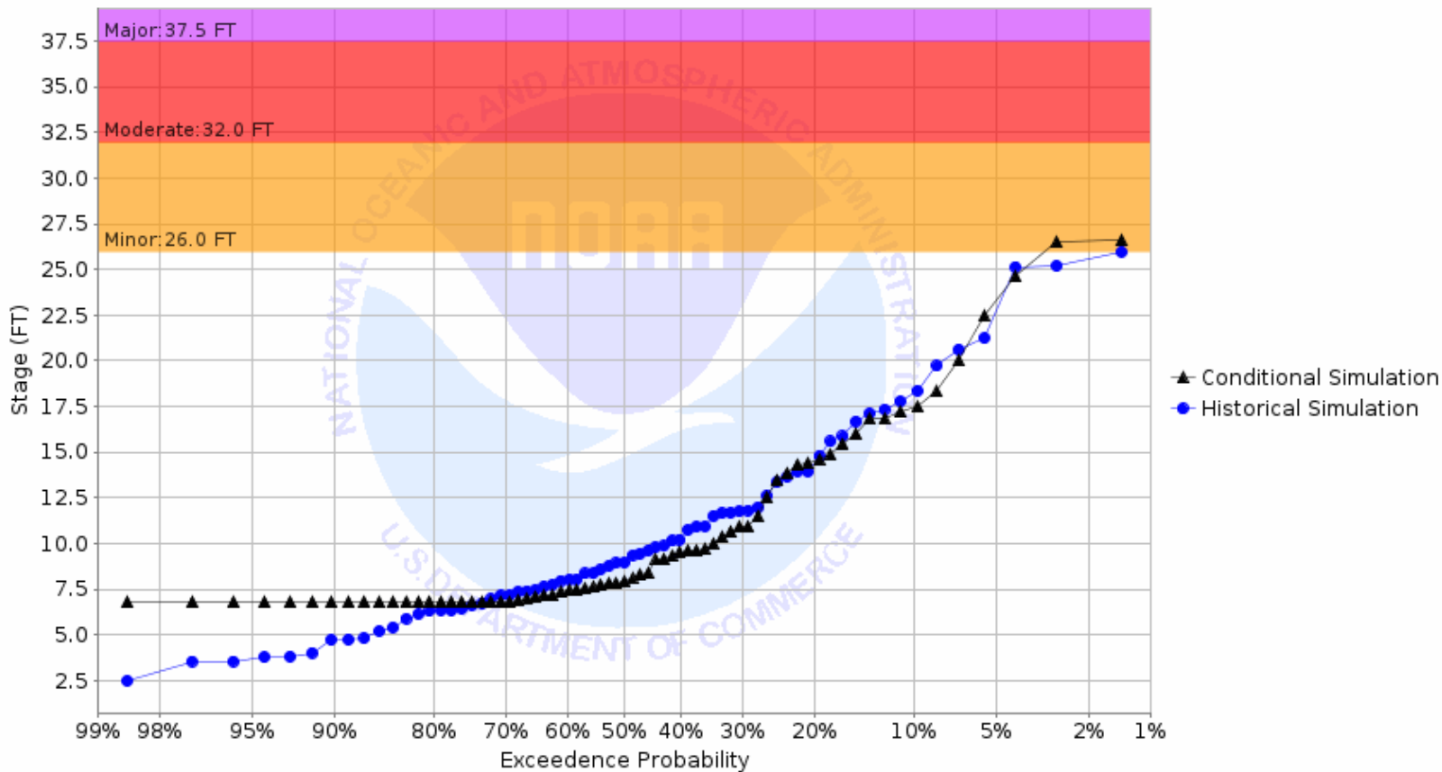
Chance of Exceeding River Stage at Red River of the North at Hillsboro 11ESE (Halstad MN) (HILN8) Forecast for the period 08/28/2023 - 11/26/2023 This is a conditional simulation based on the conditions as of 08/21/2023
