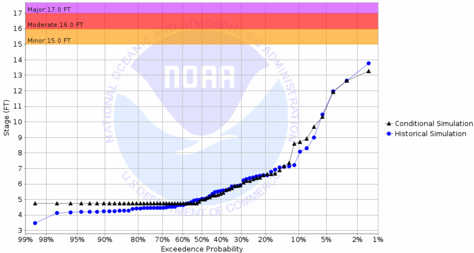
Chance of Exceeding River Stage at Sheyenne River at Valley City (VCRN8) Forecast for the period 08/28/2023 - 11/26/2023 This is a conditional simulation based on the conditions as of 08/21/2023
