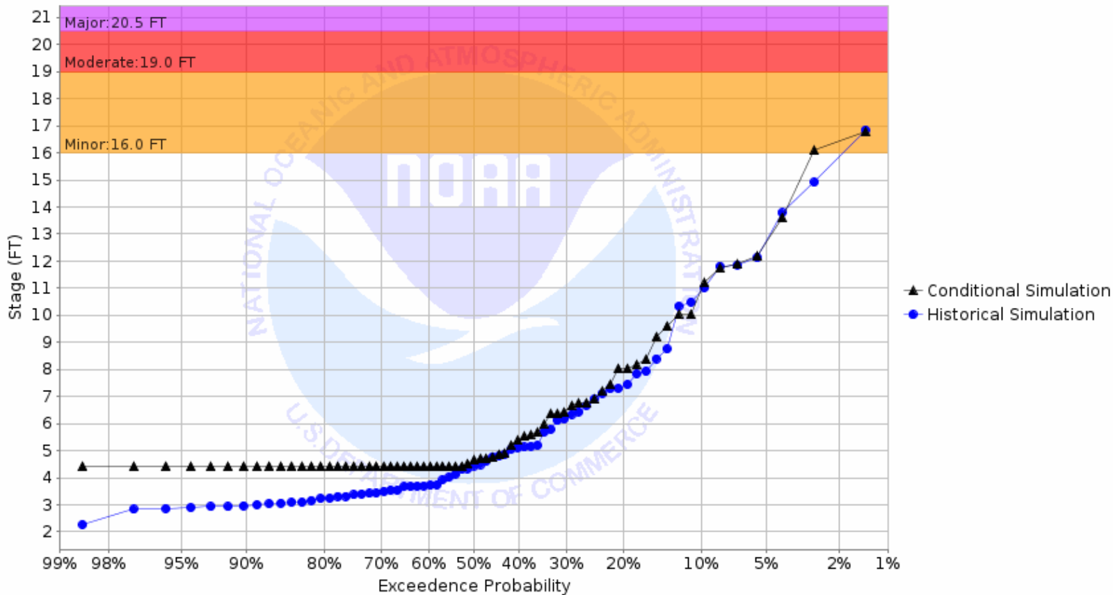
Chance of Exceeding River Stage at Sheyenne River at Kindred 2SE (KNDN8) Forecast for the period 08/28/2023 - 11/26/2023 This is a conditional simulation based on the conditions as of 08/21/2023
