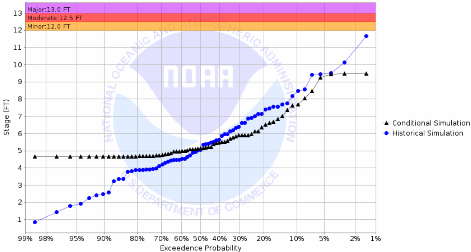
Chance of Exceeding River Stage at Red Lake River at High Landing (HIGM5) Forecast for the period 08/28/2023 - 11/26/2023 This is a conditional simulation based on the conditions as of 08/21/2023
