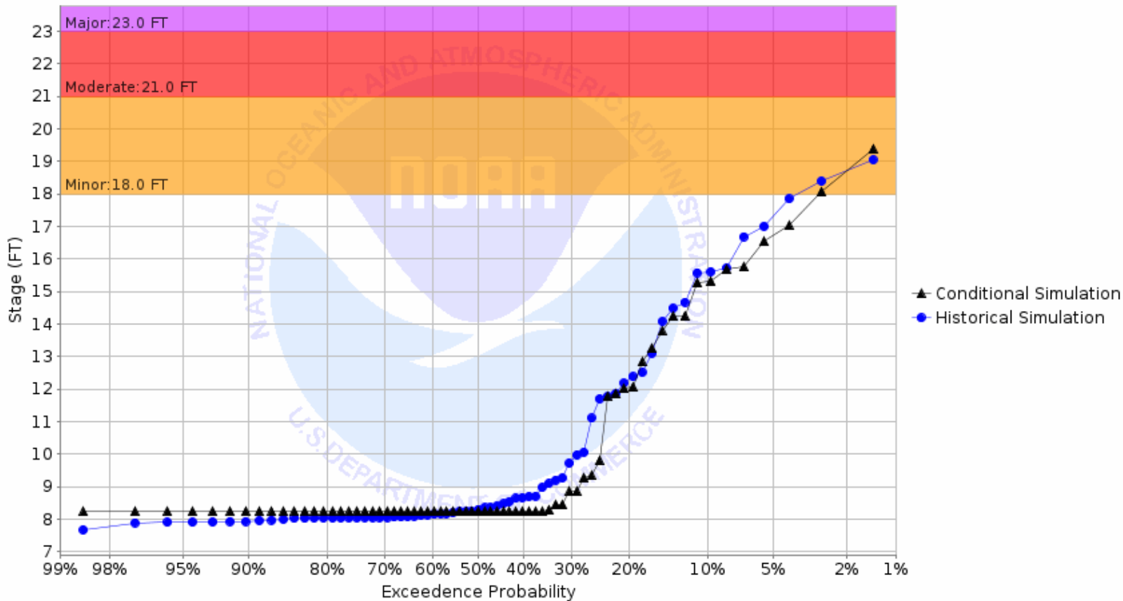
Chance of Exceeding River Stage at Maple River at Mapleton 3SW (MPLN8) Forecast for the period 08/28/2023 - 11/26/2023 This is a conditional simulation based on the conditions as of 08/21/2023
