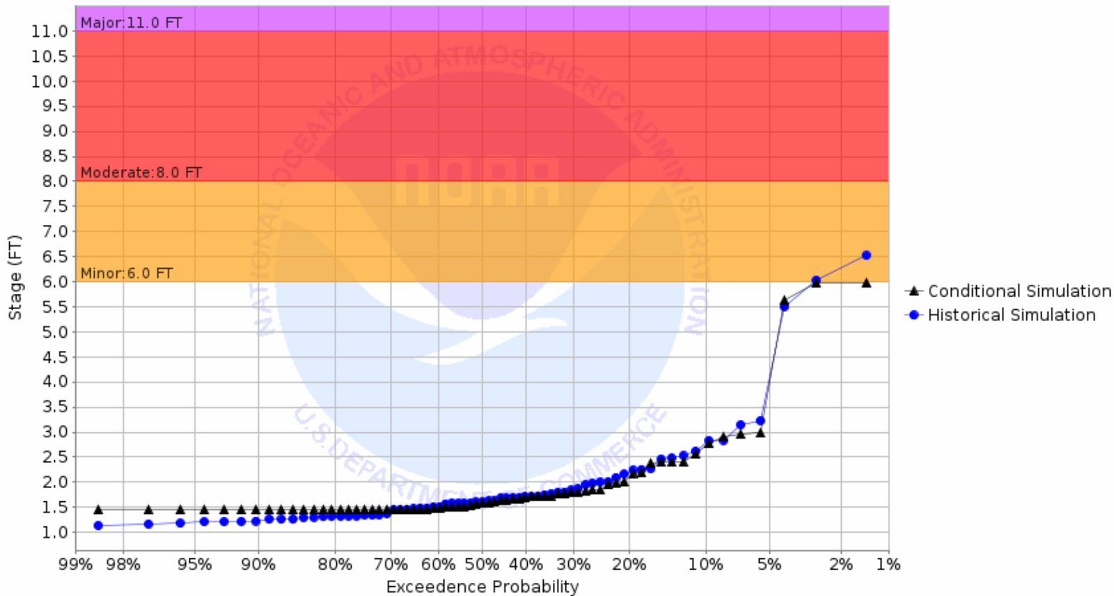
Chance of Exceeding River Stage at Forest River at Minto (MTON8) Forecast for the period 08/28/2023 - 11/26/2023 This is a conditional simulation based on the conditions as of 08/21/2023
