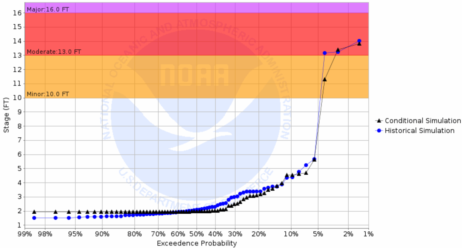
Chance of Exceeding River Stage at Goose River at Hillsboro (HGRN8) Forecast for the period 08/28/2023 - 11/26/2023 This is a conditional simulation based on the conditions as of 08/21/2023
