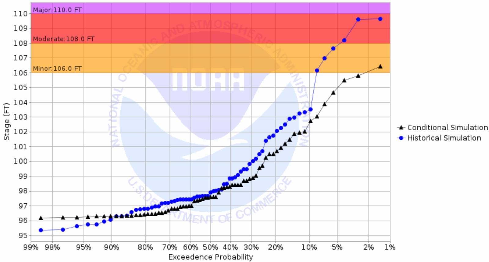
Chance of Exceeding River Stage at Snake River at Alvarado (ALVM5) Forecast for the period 08/28/2023 - 11/26/2023 This is a conditional simulation based on the conditions as of 08/21/2023
