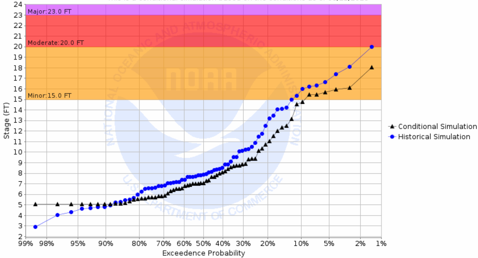
Chance of Exceeding River Stage at Red Lake River at Crookston (CRKM5) Forecast for the period 08/28/2023 - 11/26/2023 This is a conditional simulation based on the conditions as of 08/21/2023
