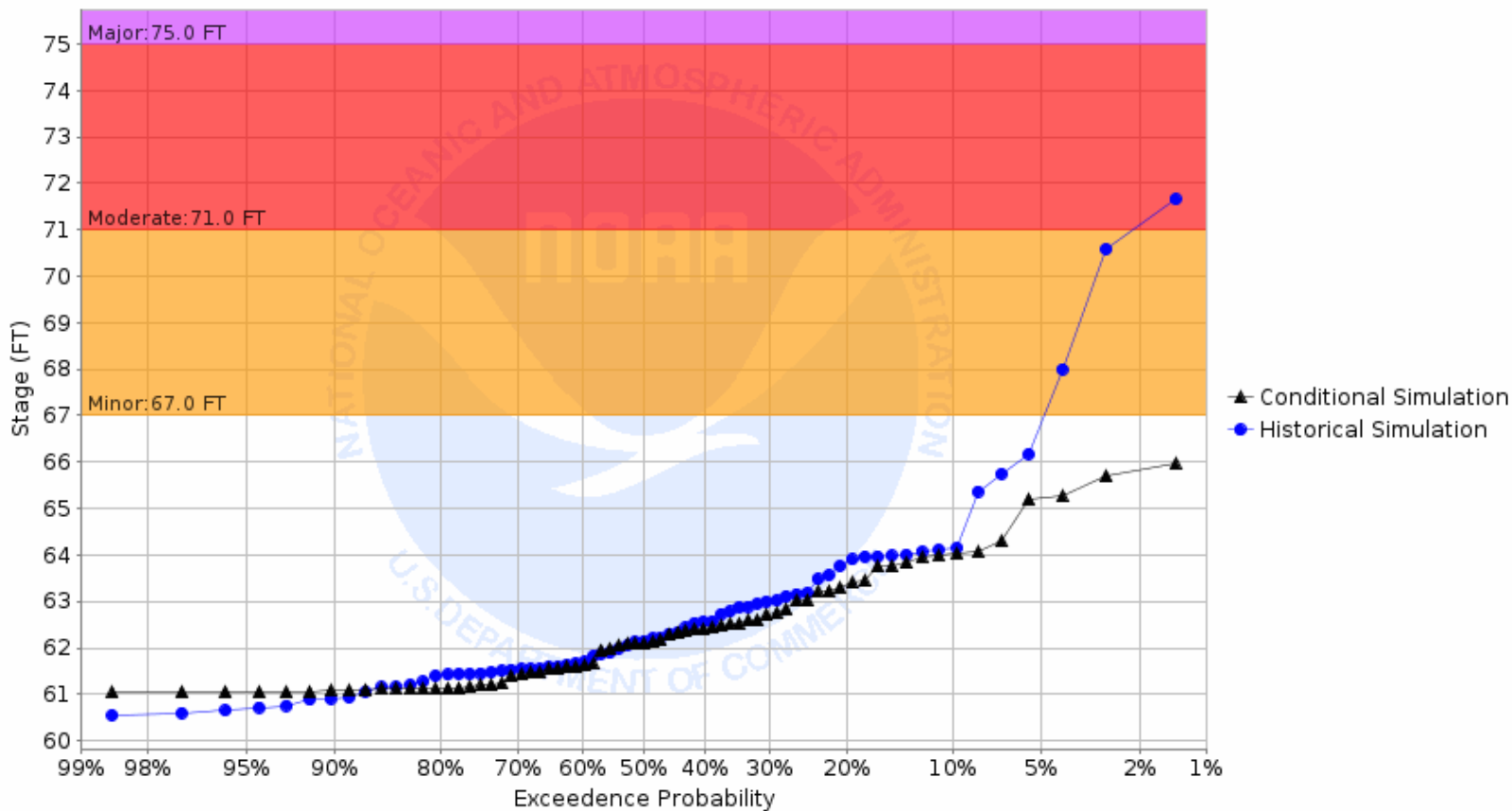
Chance of Exceeding River Stage at Snake River at Warren 3ENE-Morkassel Brdg (MKLM5) Forecast for the period 08/28/2023 - 11/26/2023 This is a conditional simulation based on the conditions as of 08/21/2023
