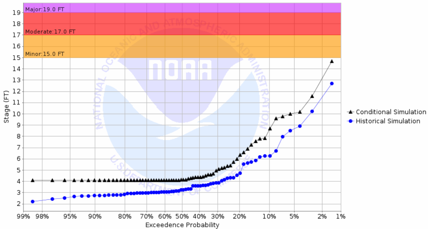
Chance of Exceeding River Stage at Sheyenne River at Lisbon (LBNN8) Forecast for the period 10/02/2023 - 12/31/2023 This is a conditional simulation based on the conditions as of 09/25/2023
