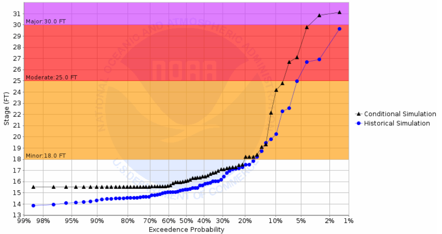
Chance of Exceeding River Stage at Red River of the North at Fargo WTP (FGON8) Forecast for the period 10/02/2023 - 12/31/2023 This is a conditional simulation based on the conditions as of 09/25/2023
