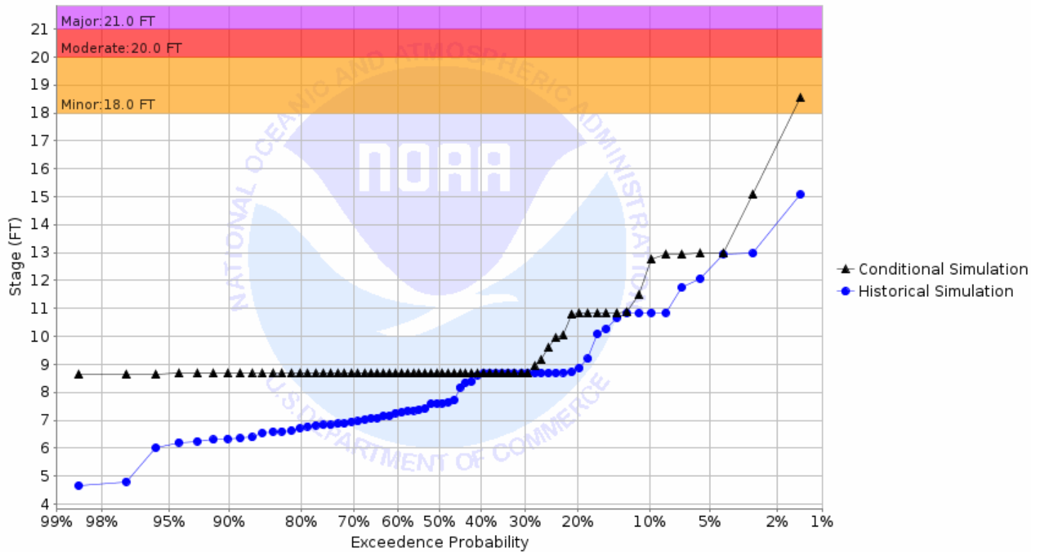
Chance of Exceeding River Stage at Sheyenne River Diversion at West Fargo (WFON8) Forecast for the period 10/02/2023 - 12/31/2023 This is a conditional simulation based on the conditions as of 09/25/2023
