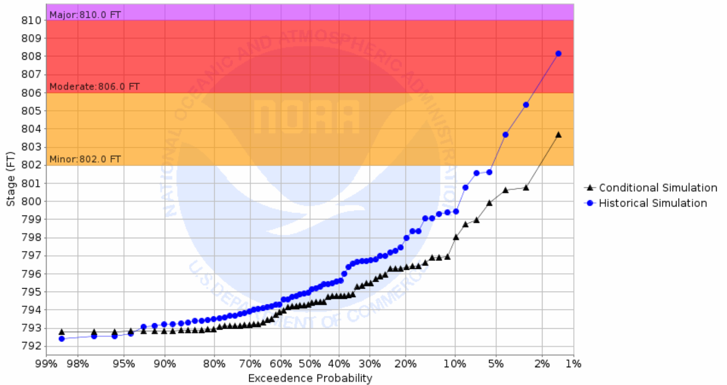
Chance of Exceeding River Stage at Two Rivers River at Hallock (HLLM5) Forecast for the period 10/02/2023 - 12/31/2023 This is a conditional simulation based on the conditions as of 09/25/2023
