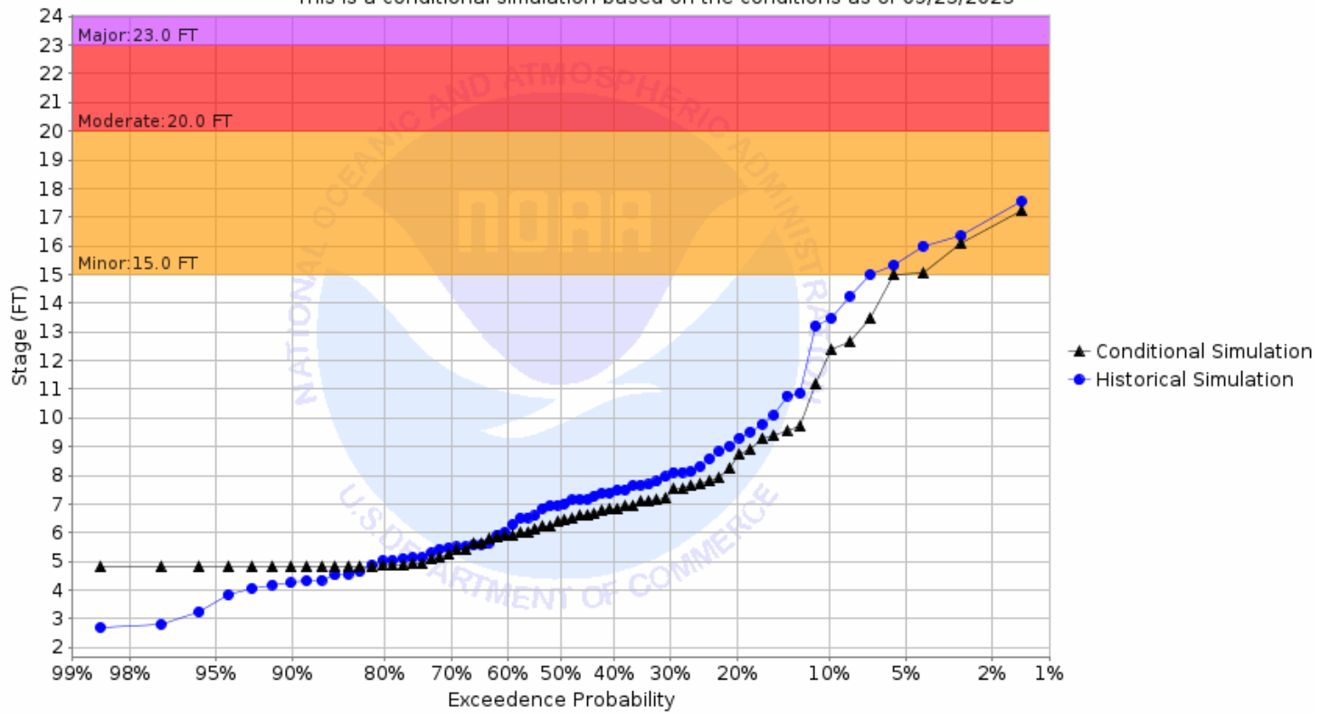
Chance of Exceeding River Stage at Snake River at Warren 3ENE-Morkassel Brdg (MKLM5) Forecast for the period 10/02/2023 - 12/31/2023 This is a conditional simulation based on the conditions as of 09/25/2023
