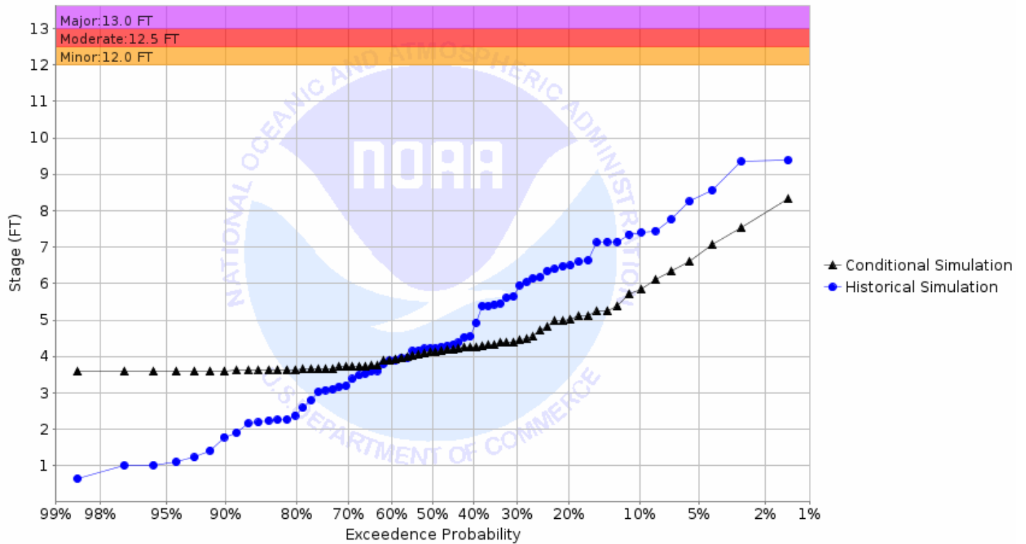
Chance of Exceeding River Stage at Red Lake River at High Landing (HIGM5) Forecast for the period 10/02/2023 - 12/31/2023 This is a conditional simulation based on the conditions as of 09/25/2023
