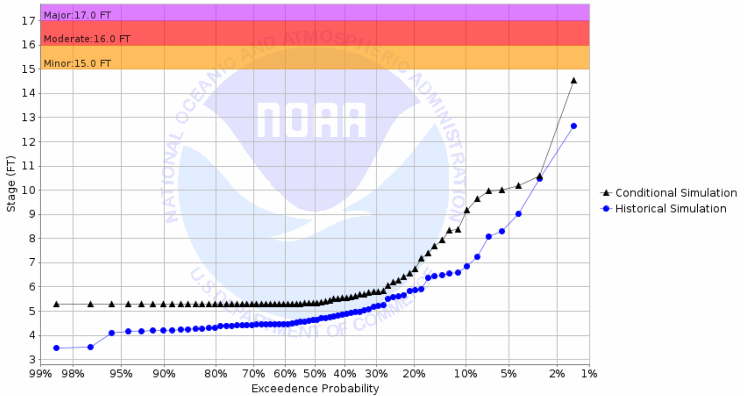
Chance of Exceeding River Stage at Sheyenne River at Valley City (VCRN8) Forecast for the period 10/02/2023 - 12/31/2023 This is a conditional simulation based on the conditions as of 09/25/2023
