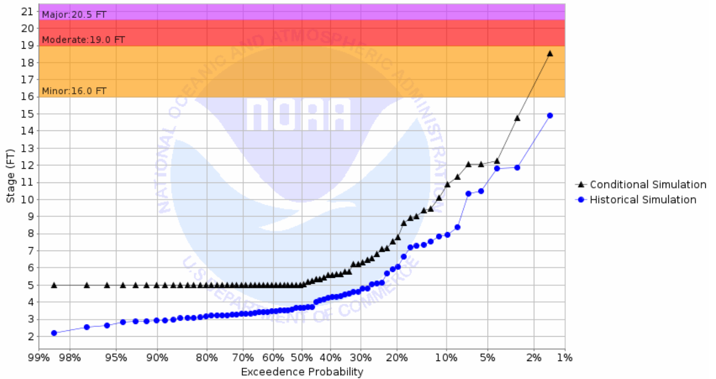
Chance of Exceeding River Stage at Sheyenne River at Kindred 2SE (KNDN8) Forecast for the period 10/02/2023 - 12/31/2023 This is a conditional simulation based on the conditions as of 09/25/2023
