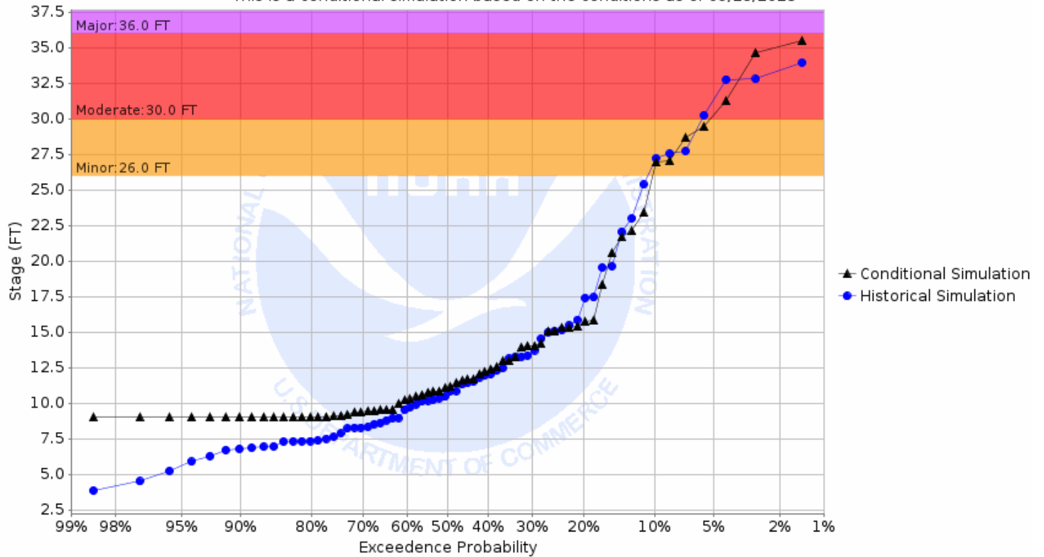
Chance of Exceeding River Stage at Red River of the North at Oslo (OSLM5) Forecast for the period 10/02/2023 - 12/31/2023 This is a conditional simulation based on the conditions as of 09/25/2023
