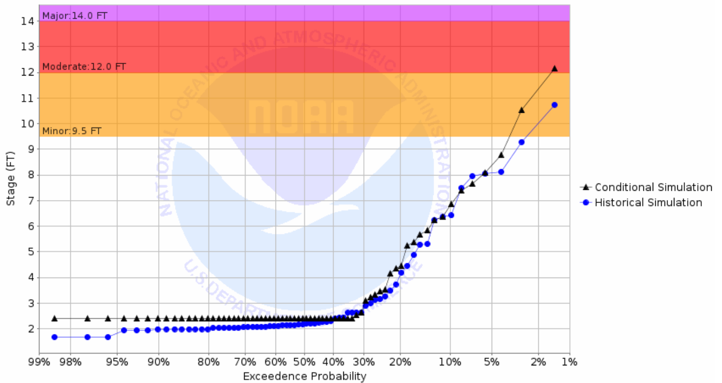
Chance of Exceeding River Stage at Maple River at Enderlin 1E (ENDN8) Forecast for the period 10/02/2023 - 12/31/2023 This is a conditional simulation based on the conditions as of 09/25/2023
