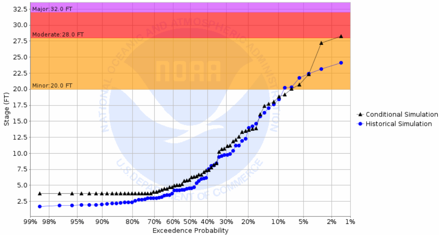
Chance of Exceeding River Stage at Wild Rice River at Hendrum (HNDM5) Forecast for the period 10/02/2023 - 12/31/2023 This is a conditional simulation based on the conditions as of 09/25/2023
