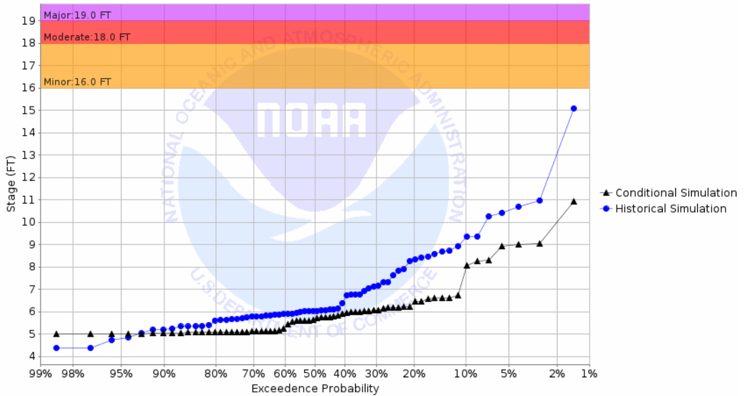
Chance of Exceeding River Stage at Roseau River at Roseau - Center St Brdg (ROSM5) Forecast for the period 10/02/2023 - 12/31/2023 This is a conditional simulation based on the conditions as of 09/25/2023
