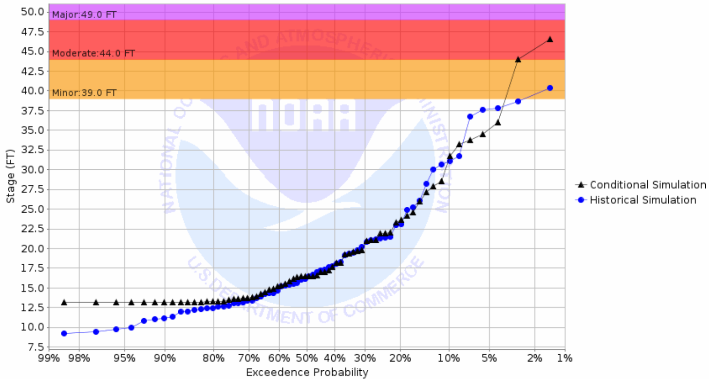
Chance of Exceeding River Stage at Red River of the North at Pembina (PBNN8) Forecast for the period 10/02/2023 - 12/31/2023 This is a conditional simulation based on the conditions as of 09/25/2023
