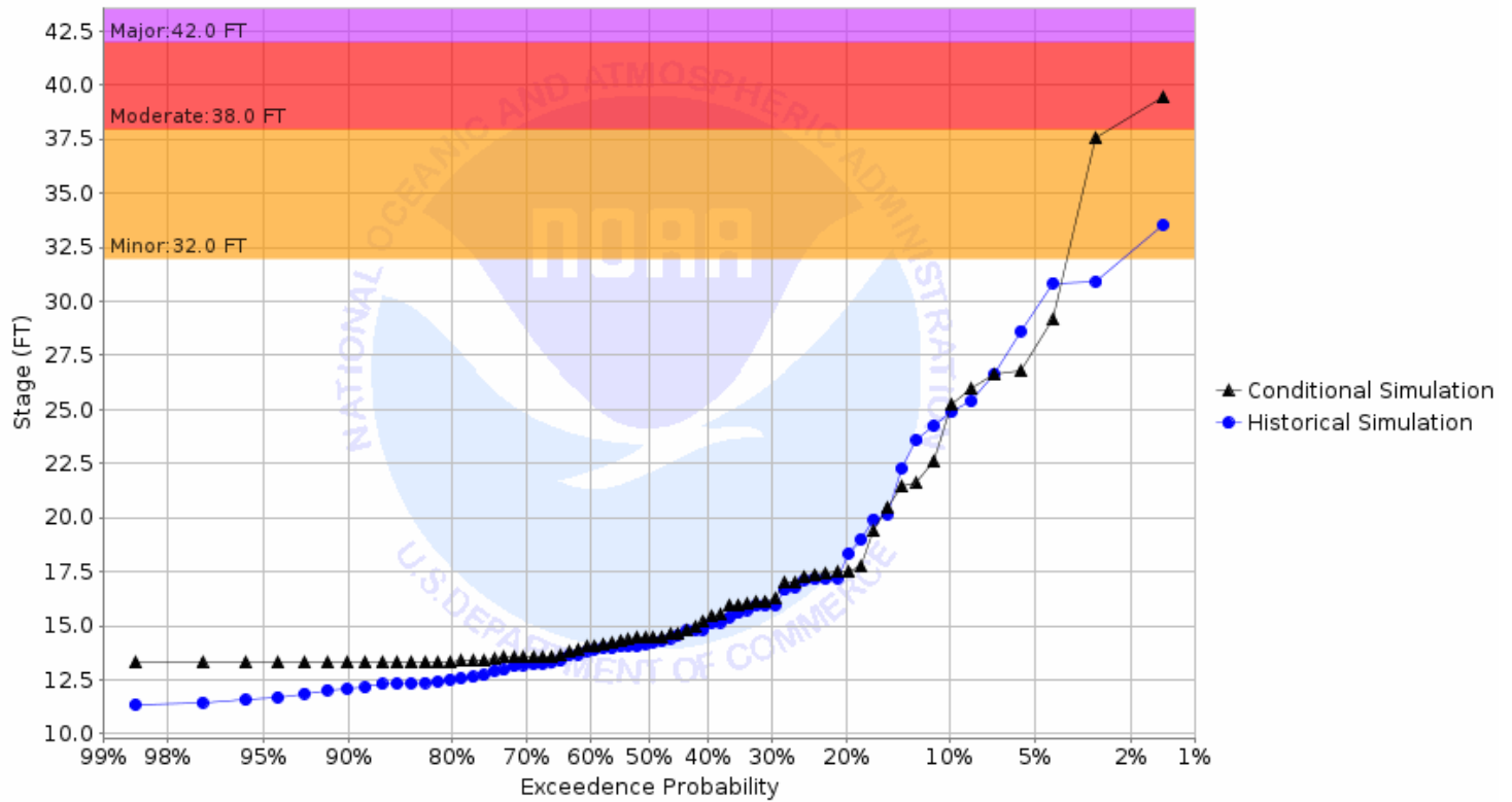
Chance of Exceeding River Stage at Red River of the North at Drayton 2NE - Hwy 66 Brdg (DRTN8) Forecast for the period 10/02/2023 - 12/31/2023 This is a conditional simulation based on the conditions as of 09/25/2023
