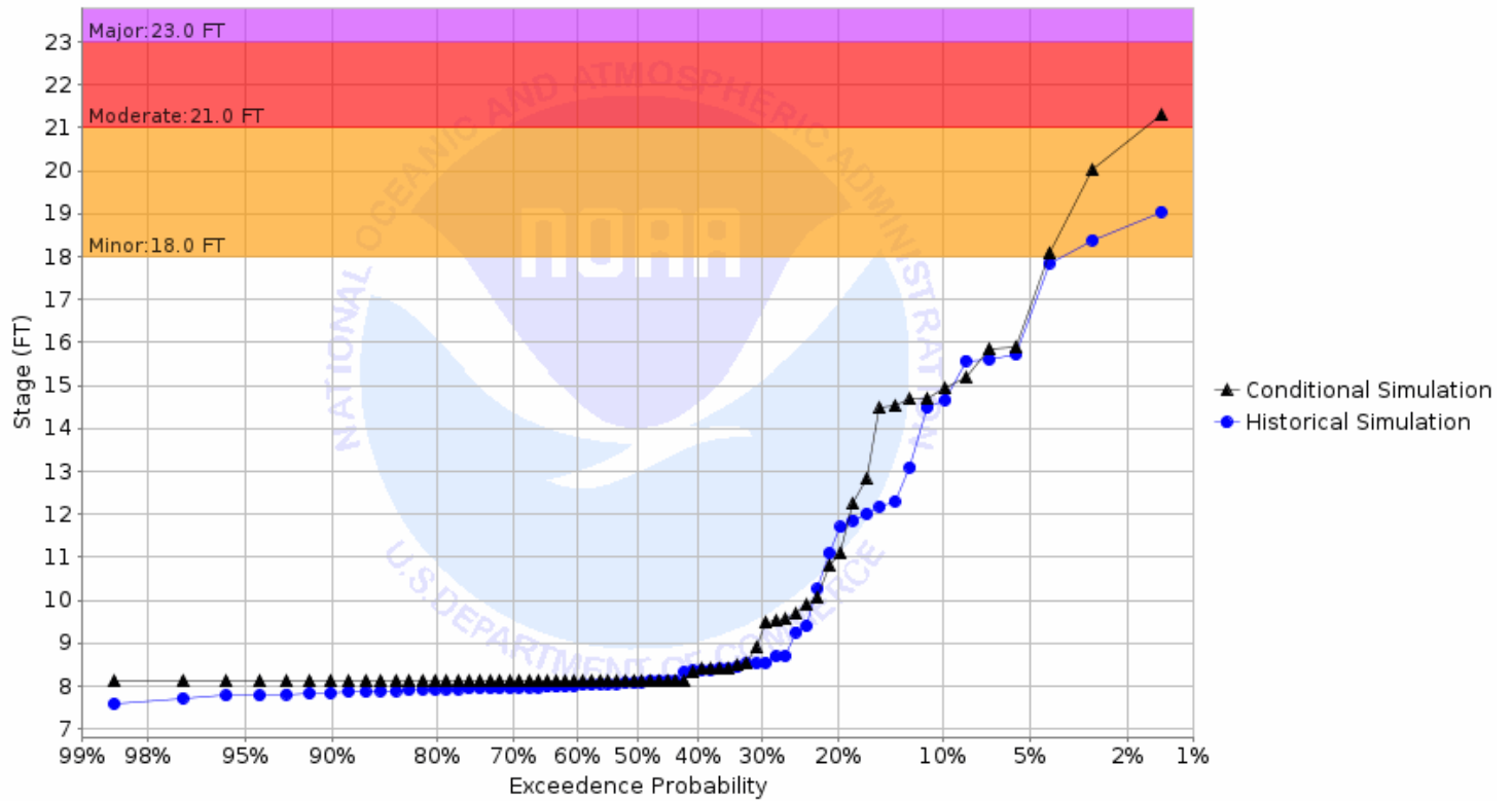
Chance of Exceeding River Stage at Maple River at Mapleton 3SW (MPLN8) Forecast for the period 10/02/2023 - 12/31/2023 This is a conditional simulation based on the conditions as of 09/25/2023
