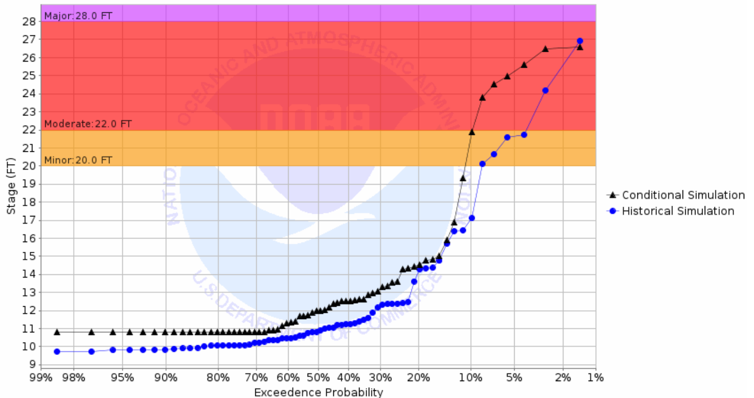
Chance of Exceeding River Stage at Wild Rice River at Abercrombie 2WNW (ABRN8) Forecast for the period 10/02/2023 - 12/31/2023 This is a conditional simulation based on the conditions as of 09/25/2023
