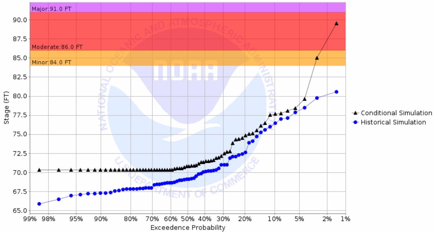
Chance of Exceeding River Stage at Sheyenne River at Harwood (HWDN8) Forecast for the period 10/02/2023 - 12/31/2023 This is a conditional simulation based on the conditions as of 09/25/2023
