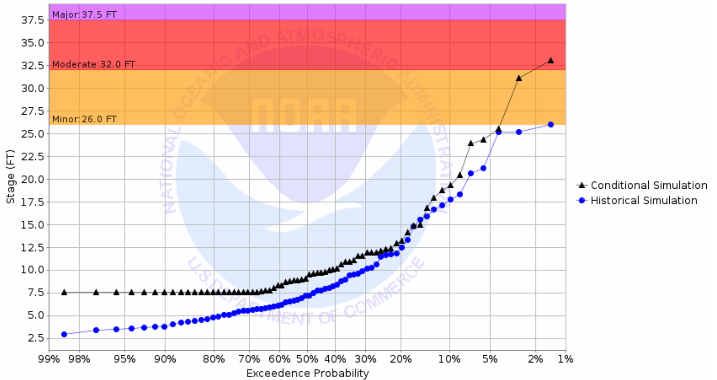
Chance of Exceeding River Stage at Red River of the North at Hillsboro 11ESE (Halstad MN) (HILN8) Forecast for the period 10/02/2023 - 12/31/2023 This is a conditional simulation based on the conditions as of 09/25/2023
