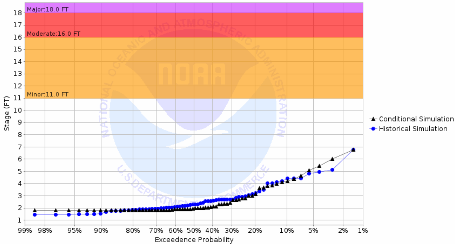
Chance of Exceeding River Stage at Pembina River at Walhalla (WLHN8) Forecast for the period 10/02/2023 - 12/31/2023 This is a conditional simulation based on the conditions as of 09/25/2023
