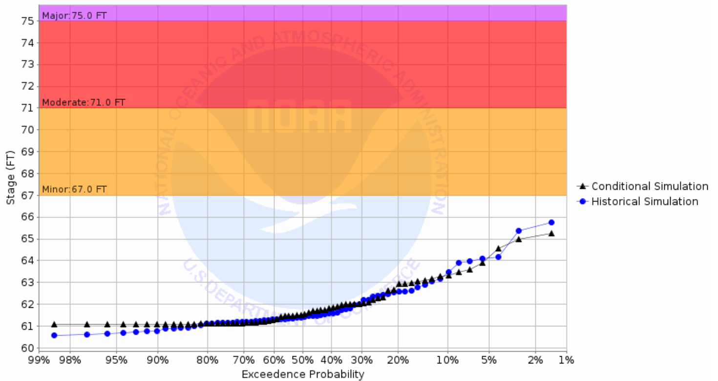
Chance of Exceeding River Stage at Snake River at Warren 3ENE-Morkassel Brdg (MKLM5) Forecast for the period 10/02/2023 - 12/31/2023 This is a conditional simulation based on the conditions as of 09/25/2023
