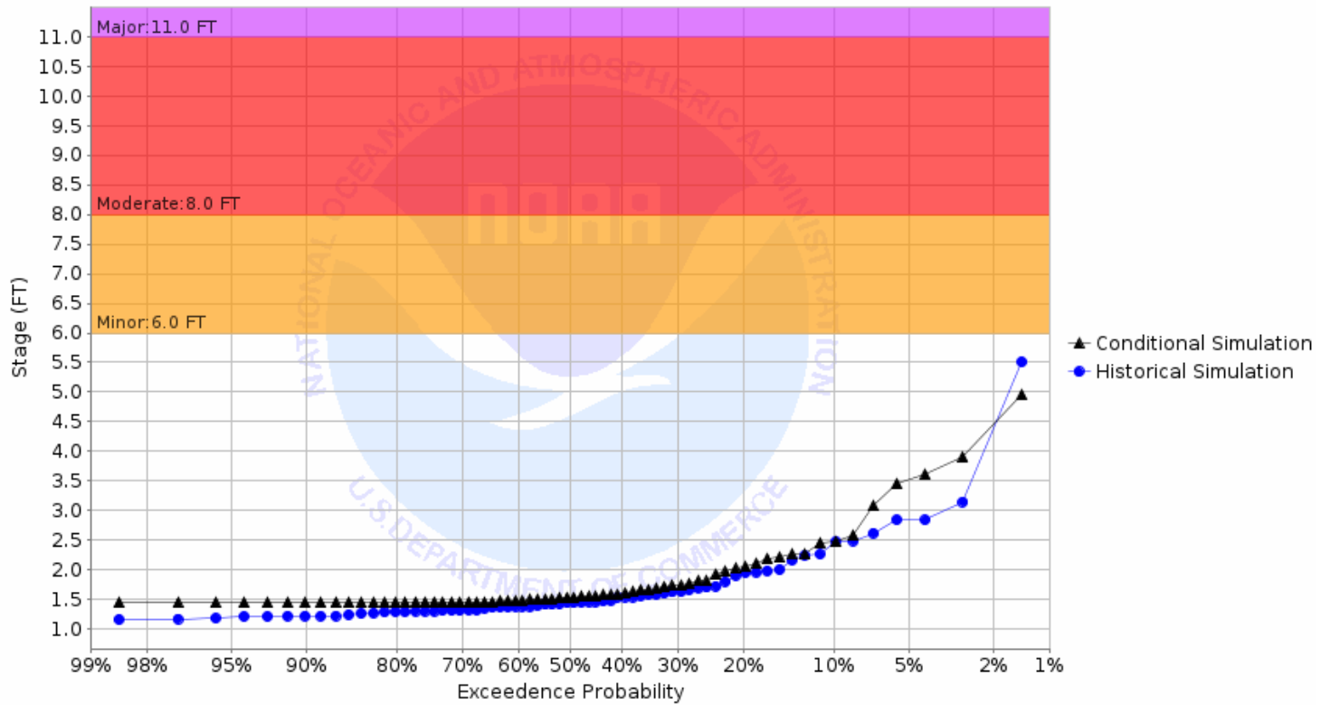
Chance of Exceeding River Stage at Forest River at Minto (MTON8) Forecast for the period 10/02/2023 - 12/31/2023 This is a conditional simulation based on the conditions as of 09/25/2023
