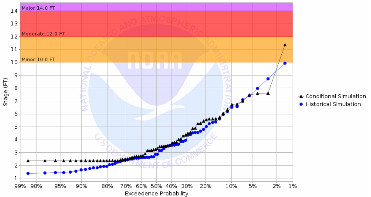
Chance of Exceeding River Stage at Wild Rice River at Twin Valley 1NE (TWVM5) Forecast for the period 10/02/2023 - 12/31/2023 This is a conditional simulation based on the conditions as of 09/25/2023
