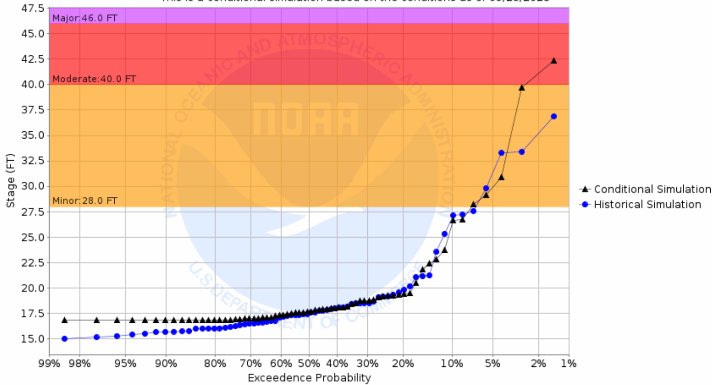
Chance of Exceeding River Stage at Red River of the North at East Grand Forks (EGFM5) Forecast for the period 10/02/2023 - 12/31/2023 This is a conditional simulation based on the conditions as of 09/25/2023
