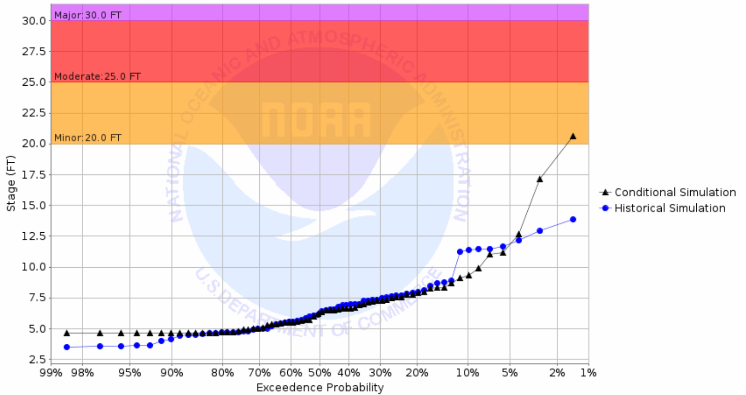
Chance of Exceeding River Stage at Sand Hill River at Climax (CLXM5) Forecast for the period 10/02/2023 - 12/31/2023 This is a conditional simulation based on the conditions as of 09/25/2023
