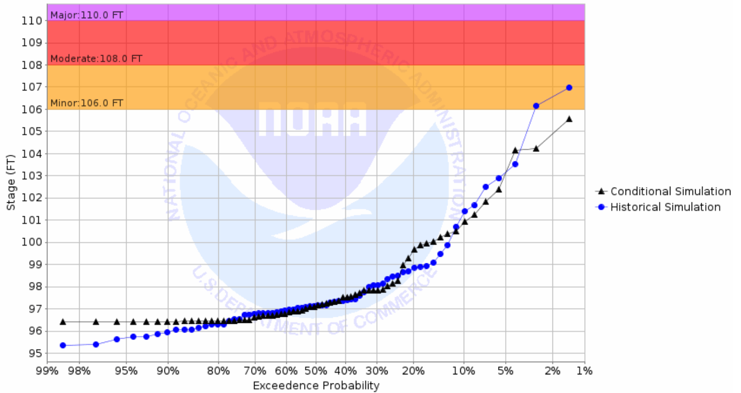
Chance of Exceeding River Stage at Snake River at Alvarado (ALVM5) Forecast for the period 10/02/2023 - 12/31/2023 This is a conditional simulation based on the conditions as of 09/25/2023
