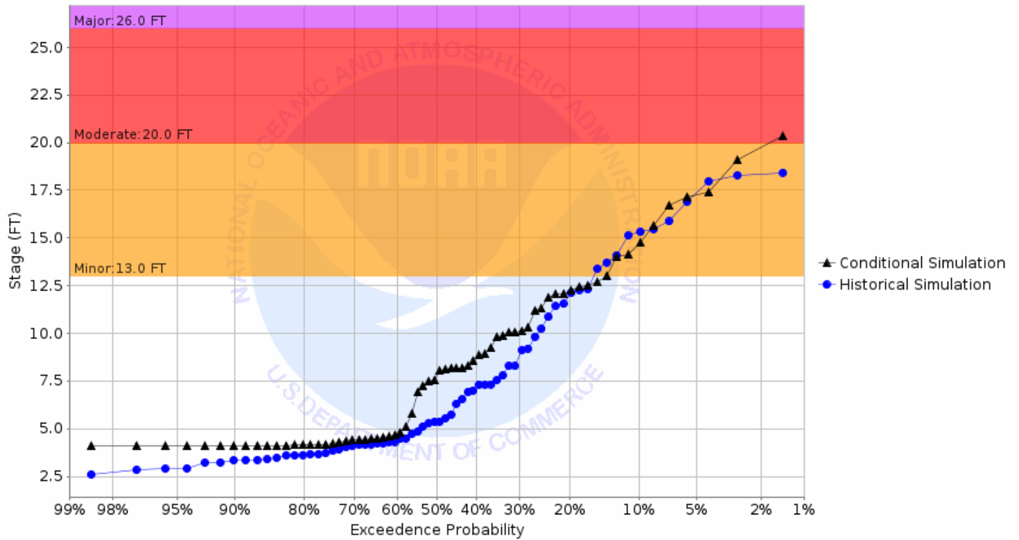
Chance of Exceeding River Stage at Buffalo River at Dilworth 7NE (DILM5) Forecast for the period 10/02/2023 - 12/31/2023 This is a conditional simulation based on the conditions as of 09/25/2023
