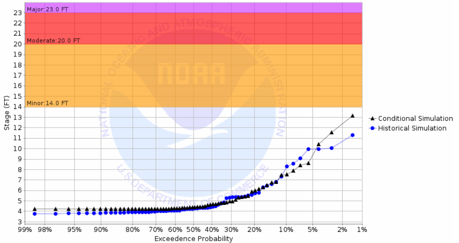
Chance of Exceeding River Stage at Marsh River at Shelly 4SE (SHYM5) Forecast for the period 10/02/2023 - 12/31/2023 This is a conditional simulation based on the conditions as of 09/25/2023
