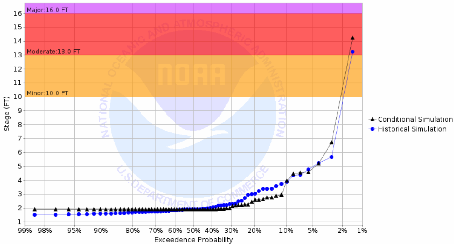
Chance of Exceeding River Stage at Goose River at Hillsboro (HGRN8) Forecast for the period 10/02/2023 - 12/31/2023 This is a conditional simulation based on the conditions as of 09/25/2023
