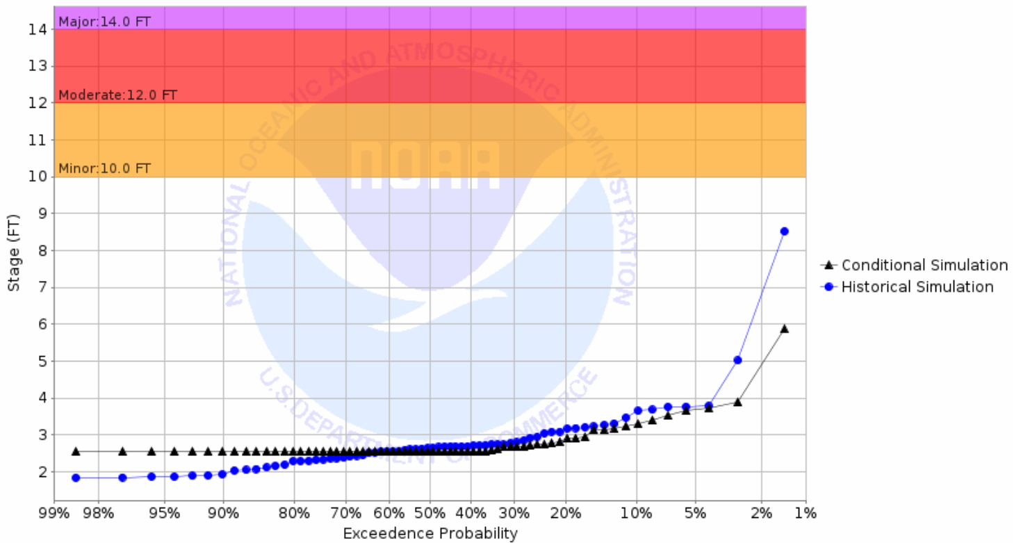
Chance of Exceeding River Stage at Wild Rice River at Twin Valley 1NE (TWVM5) Forecast for the period 11/27/2023 - 02/25/2024 This is a conditional simulation based on the conditions as of 11/20/2023
