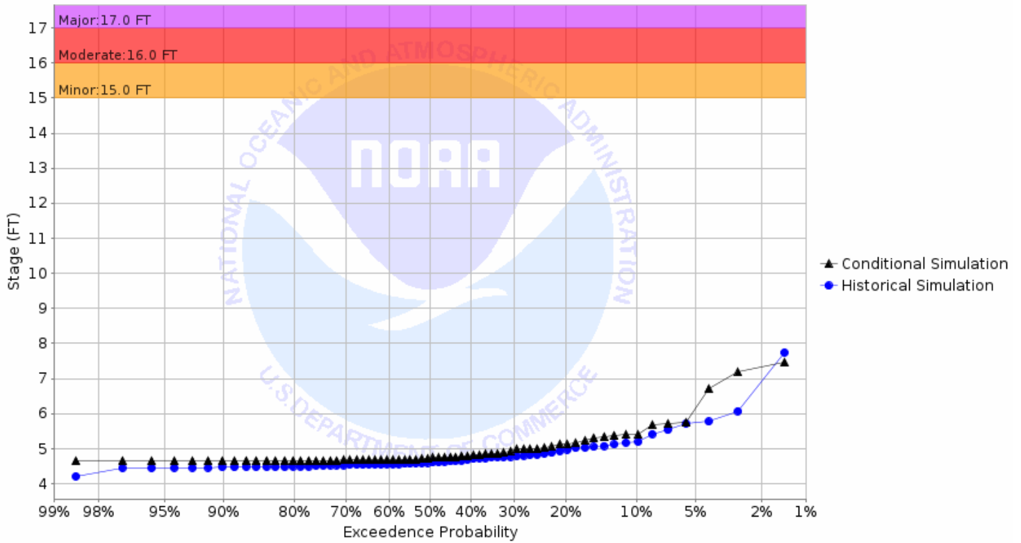
Chance of Exceeding River Stage at Sheyenne River at Valley City (VCRN8) Forecast for the period 11/27/2023 - 02/25/2024 This is a conditional simulation based on the conditions as of 11/20/2023
