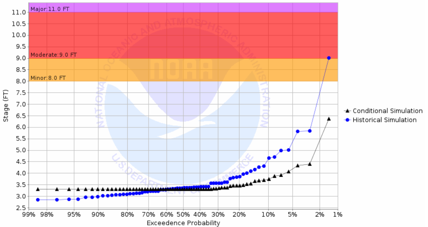
Chance of Exceeding River Stage at Buffalo River at Hawley 2SW (HWYM5) Forecast for the period 11/27/2023 - 02/25/2024
