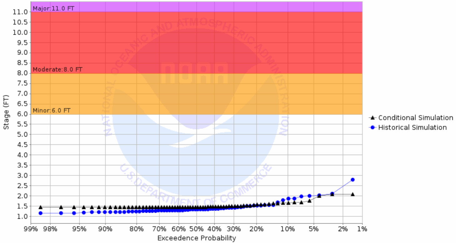
Chance of Exceeding River Stage at Forest River at Minto (MTON8) Forecast for the period 11/27/2023 - 02/25/2024 This is a conditional simulation based on the conditions as of 11/20/2023
