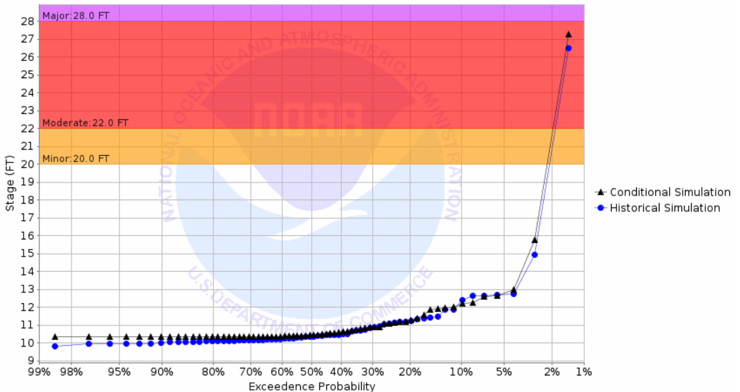
Chance of Exceeding River Stage at Wild Rice River at Abercrombie 2WNW (ABRN8) Forecast for the period 11/27/2023 - 02/25/2024 This is a conditional simulation based on the conditions as of 11/20/2023
