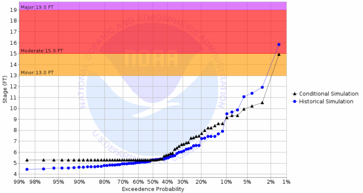
Chance of Exceeding River Stage at South Branch Buffalo River at Sabin 1E (SABM5) Forecast for the period 11/27/2023 - 02/25/2024
