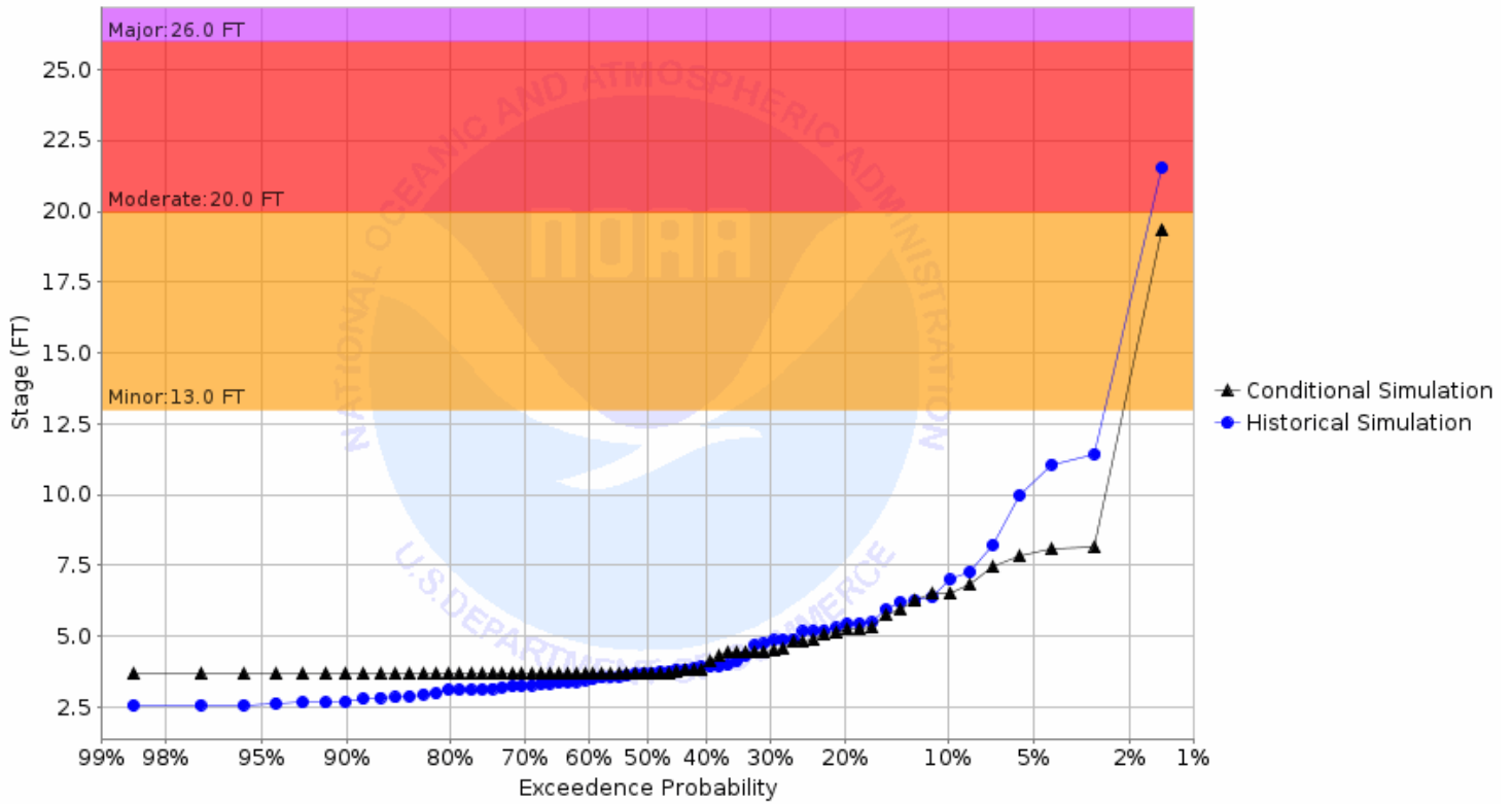
Chance of Exceeding River Stage at Buffalo River at Dilworth 7NE (DILM5) Forecast for the period 11/27/2023 - 02/25/2024 This is a conditional simulation based on the conditions as of 11/20/2023
