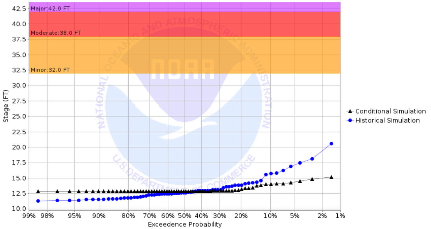
Chance of Exceeding River Stage at Red River of the North at Drayton 2NE - Hwy 66 Brdg (DRTN8) Forecast for the period 11/27/2023 - 02/25/2024 This is a conditional simulation based on the conditions as of 11/20/2023
