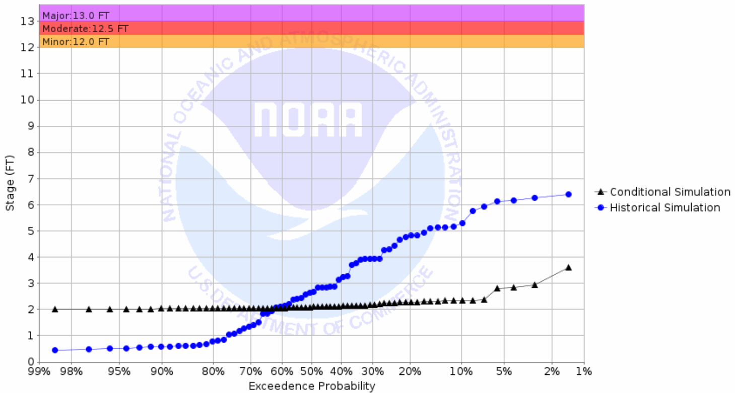
Chance of Exceeding River Stage at Red Lake River at High Landing (HIGM5) Forecast for the period 11/27/2023 - 02/25/2024 This is a conditional simulation based on the conditions as of 11/20/2023
