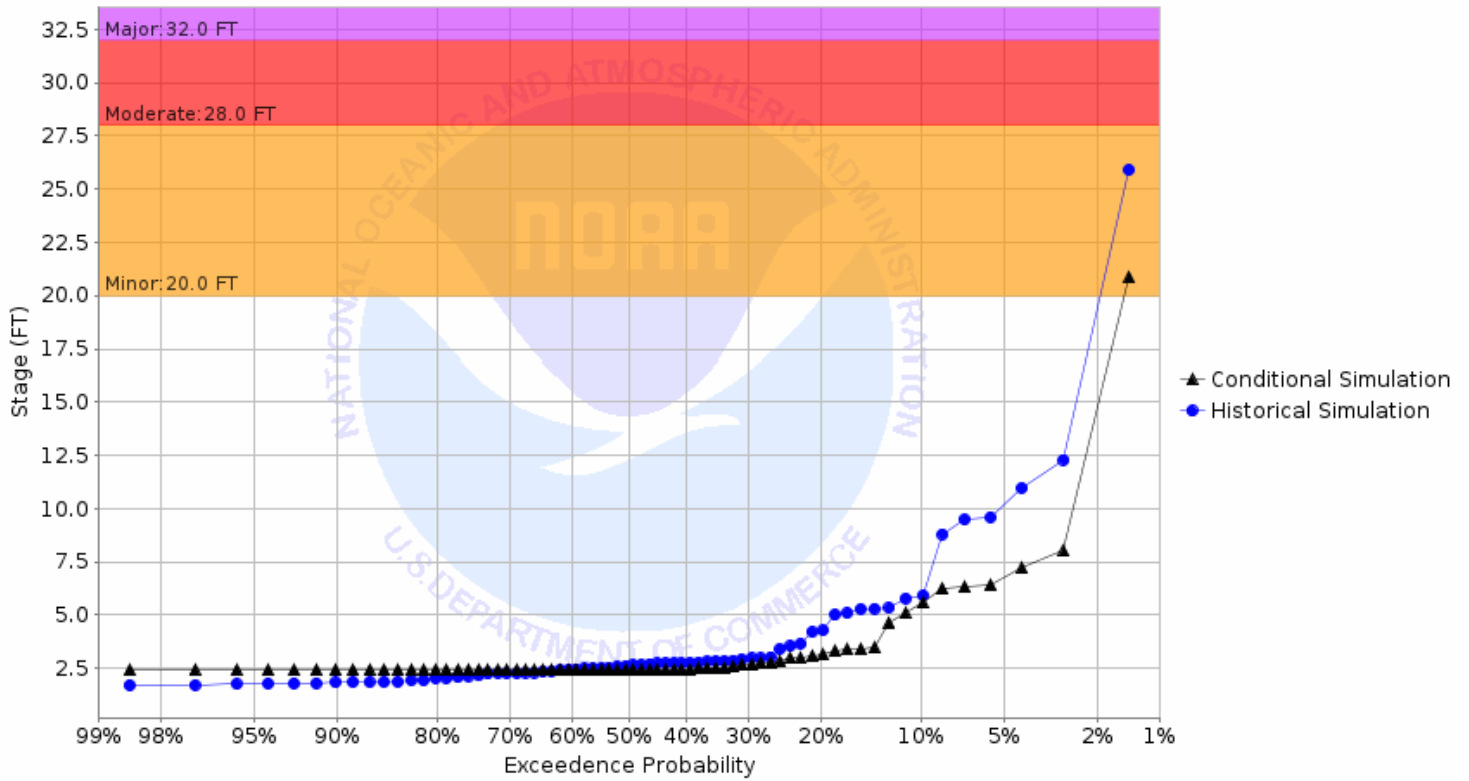
Chance of Exceeding River Stage at Wild Rice River at Hendrum (HNDM5) Forecast for the period 11/27/2023 - 02/25/2024 This is a conditional simulation based on the conditions as of 11/20/2023
