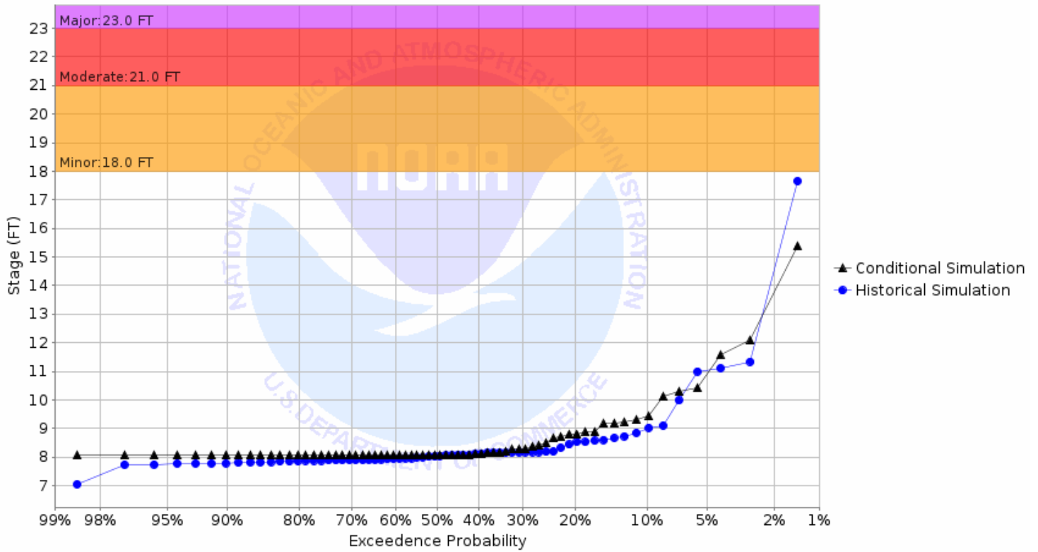
Chance of Exceeding River Stage at Maple River at Mapleton 3SW (MPLN8) Forecast for the period 11/27/2023 - 02/25/2024 This is a conditional simulation based on the conditions as of 11/20/2023
