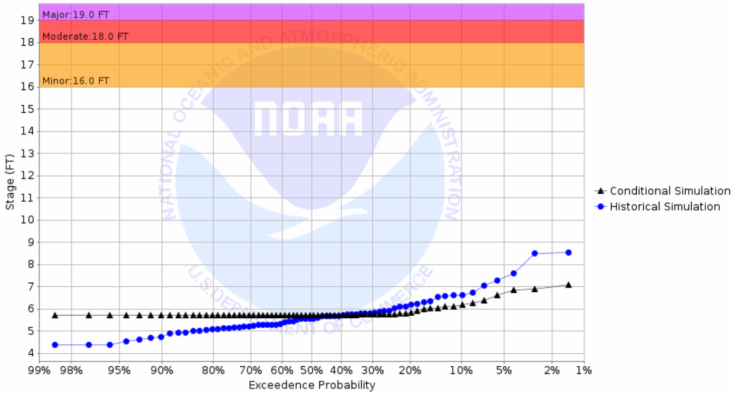
Chance of Exceeding River Stage at Roseau River at Roseau - Center St Brdg (ROSM5) Forecast for the period 11/27/2023 - 02/25/2024 This is a conditional simulation based on the conditions as of 11/20/2023
