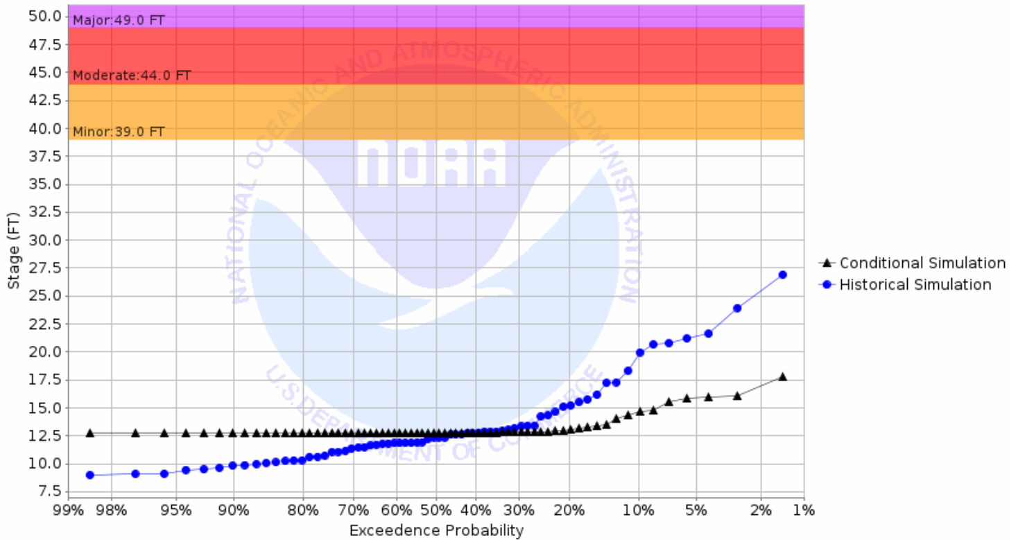
Chance of Exceeding River Stage at Red River of the North at Pembina (PBNN8) Forecast for the period 11/27/2023 - 02/25/2024 This is a conditional simulation based on the conditions as of 11/20/2023
