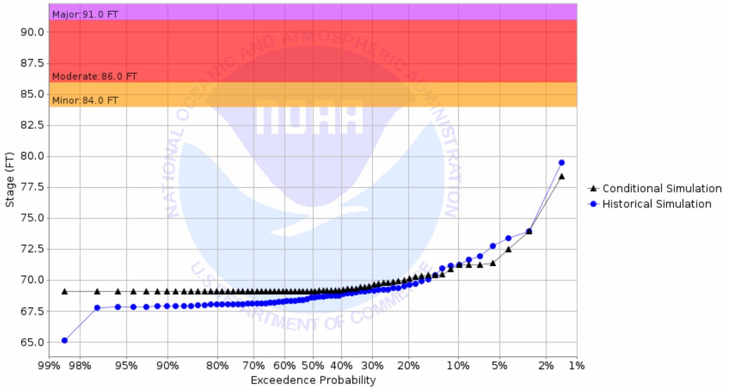
Chance of Exceeding River Stage at Sheyenne River at Harwood (HWDN8) Forecast for the period 11/27/2023 - 02/25/2024 This is a conditional simulation based on the conditions as of 11/20/2023
