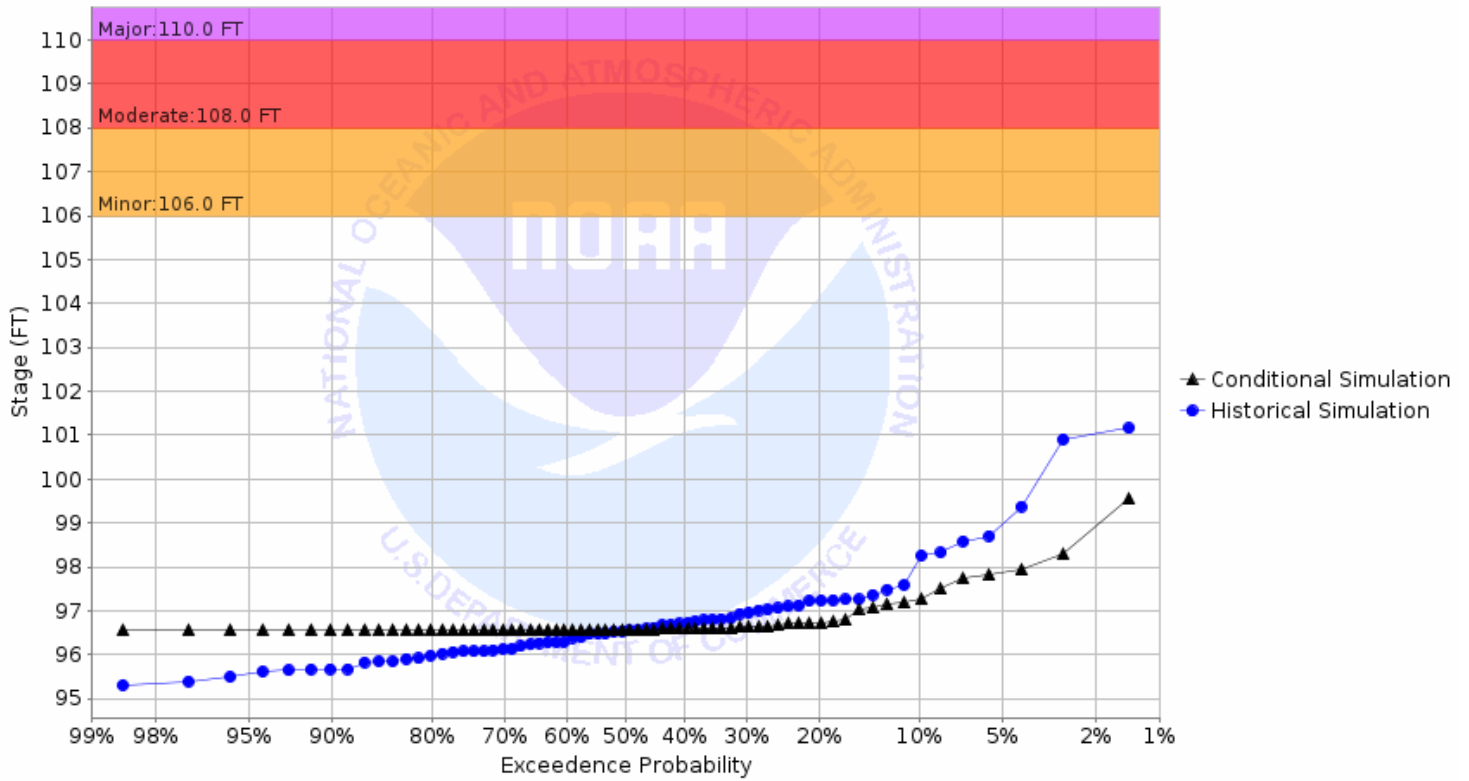
Chance of Exceeding River Stage at Snake River at Alvarado (ALVM5) Forecast for the period 11/27/2023 - 02/25/2024 This is a conditional simulation based on the conditions as of 11/20/2023
