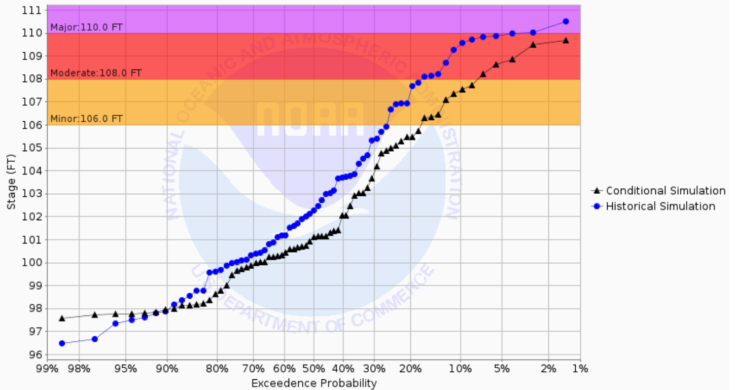
Chance of Exceeding River Stage at Snake River at Alvarado (ALVM5) Forecast for the period 03/04/2024 - 06/02/2024 This is a conditional simulation based on the conditions as of 02/26/2024
