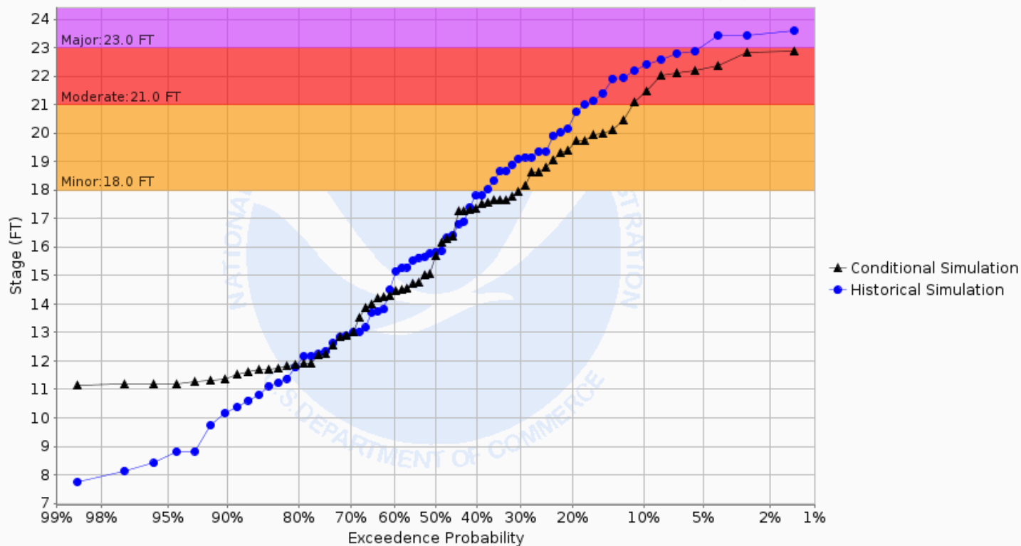
Chance of Exceeding River Stage at Maple River at Mapleton 3SW (MPLN8) Forecast for the period 03/04/2024 - 06/02/2024 This is a conditional simulation based on the conditions as of 02/26/2024
