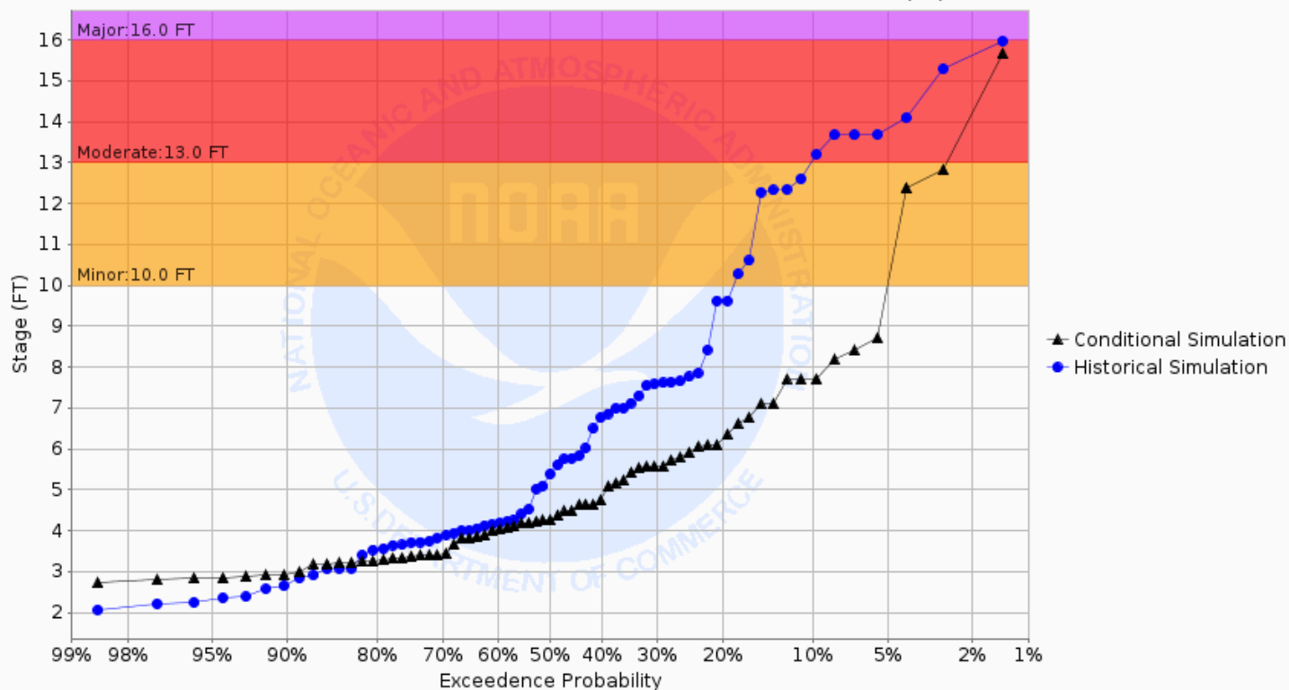
Chance of Exceeding River Stage at Goose River at Hillsboro (HGRN8) Forecast for the period 03/04/2024 - 06/02/2024 This is a conditional simulation based on the conditions as of 02/26/2024
