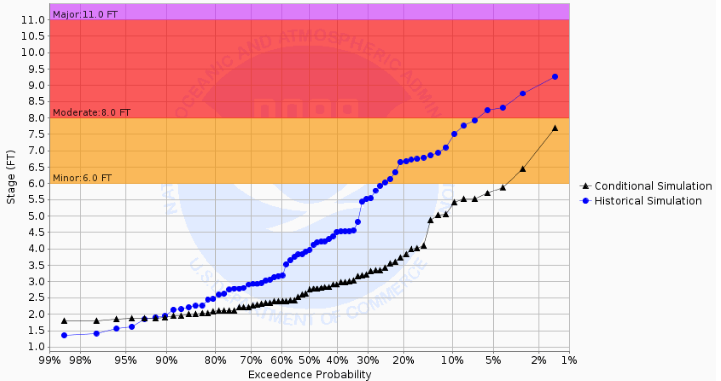
Chance of Exceeding River Stage at Forest River at Minto (MTON8) Forecast for the period 03/04/2024 - 06/02/2024 This is a conditional simulation based on the conditions as of 02/26/2024
