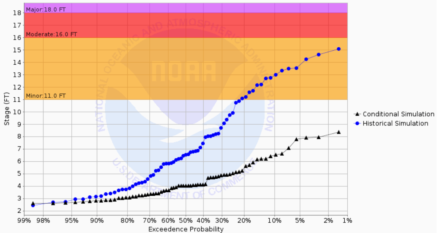
Chance of Exceeding River Stage at Pembina River at Walhalla (WLHN8) Forecast for the period 03/04/2024 - 06/02/2024 This is a conditional simulation based on the conditions as of 02/26/2024
