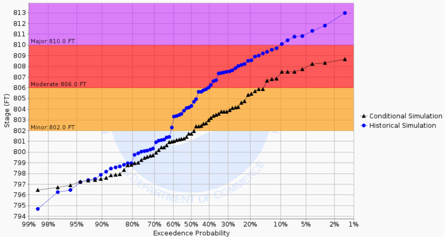
Chance of Exceeding River Stage at Two Rivers River at Hallock (HLLM5) Forecast for the period 03/04/2024 - 06/02/2024 This is a conditional simulation based on the conditions as of 02/26/2024
