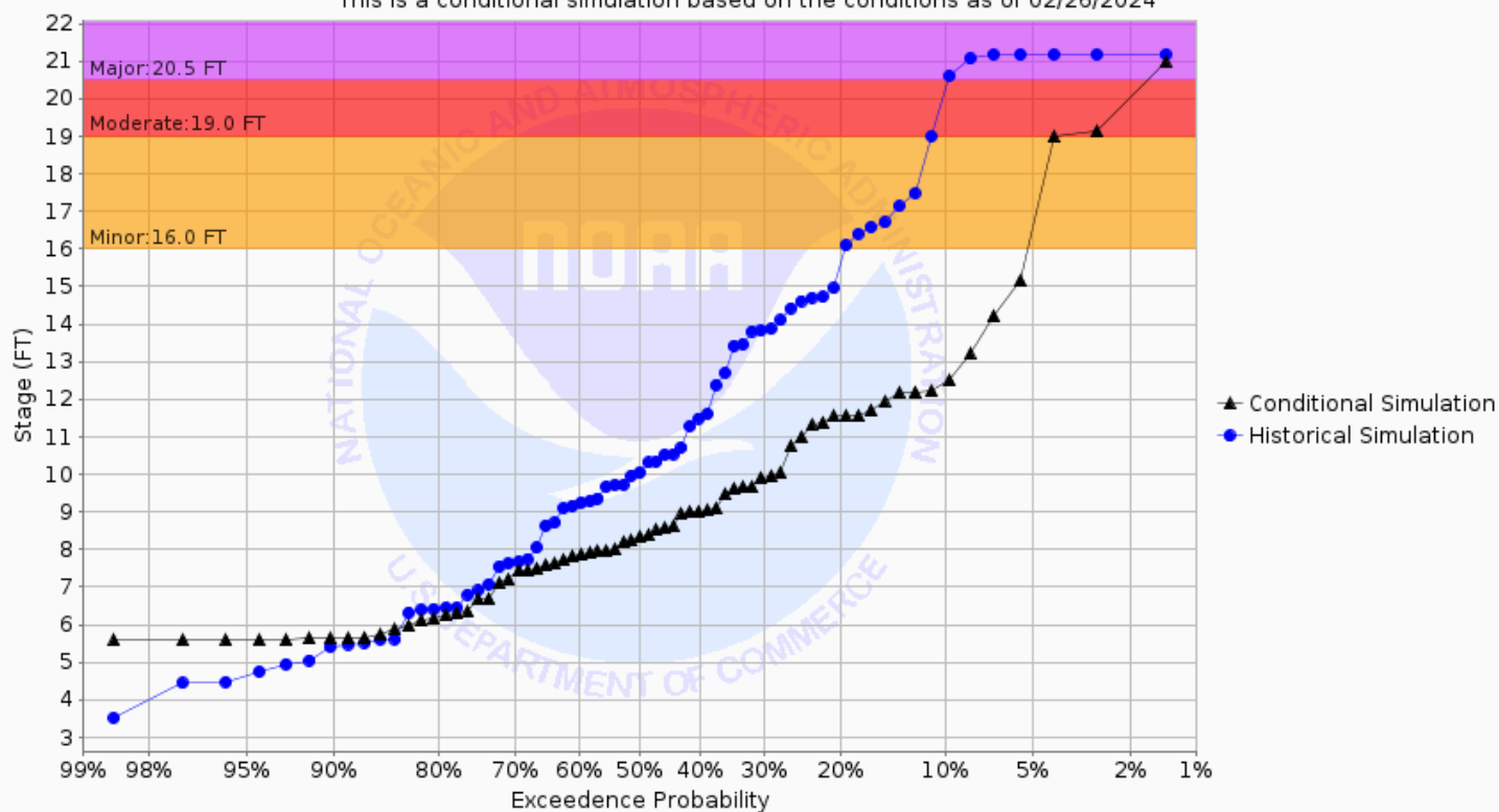
Chance of Exceeding River Stage at Sheyenne River at Kindred 2SE (KNDN8) Forecast for the period 03/04/2024 - 06/02/2024 This is a conditional simulation based on the conditions as of 02/26/2024
