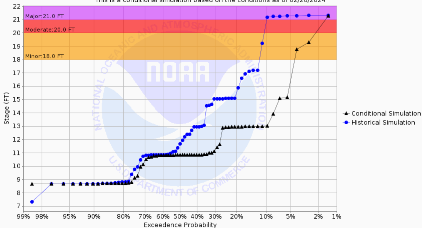
Chance of Exceeding River Stage at Sheyenne River Diversion at West Fargo (WFON8) Forecast for the period 03/04/2024 - 06/02/2024 This is a conditional simulation based on the conditions as of 02/26/2024
