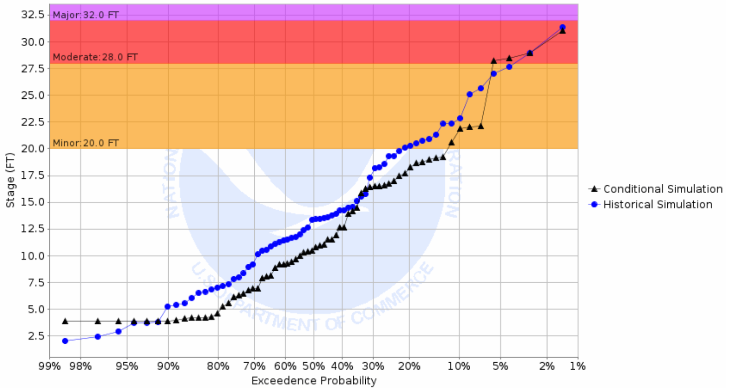
Chance of Exceeding River Stage at Wild Rice River at Hendrum (HNDM5) Forecast for the period 06/01/2026 - 08/30/2026 This is a conditional simulation based on the conditions as of 05/25/2026
