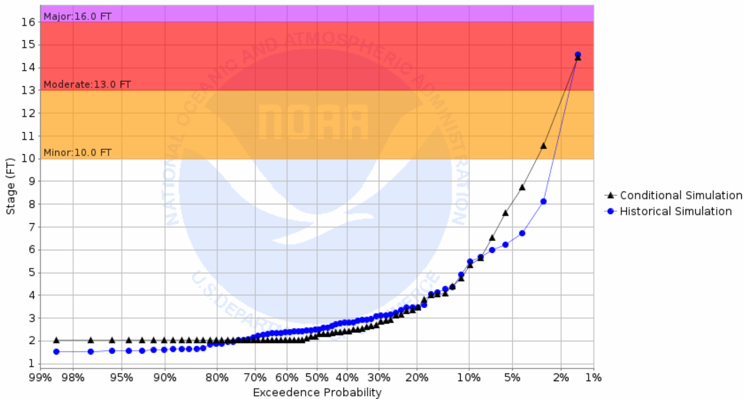
Chance of Exceeding River Stage at Goose River at Hillsboro (HGRN8) Forecast for the period 06/01/2026 - 08/30/2026 This is a conditional simulation based on the conditions as of 05/25/2026
