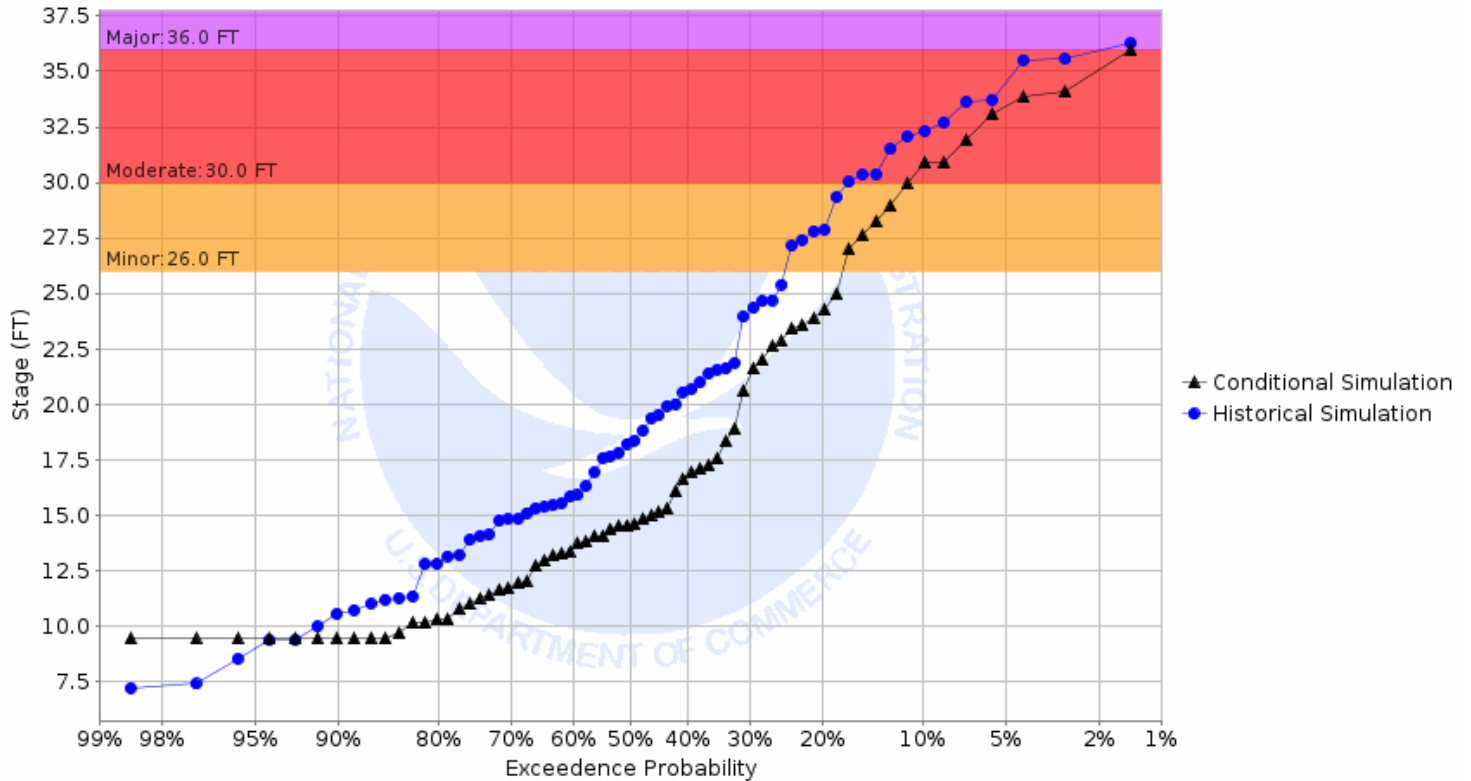
Chance of Exceeding River Stage at Red River of the North at Oslo (OSLM5) Forecast for the period 06/01/2026 - 08/30/2026 This is a conditional simulation based on the conditions as of 05/25/2026
