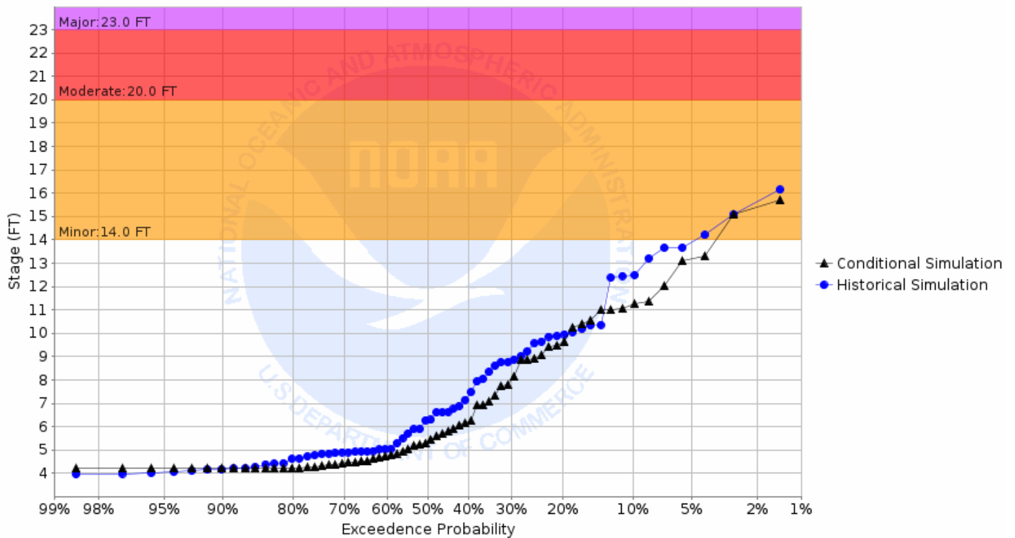
Chance of Exceeding River Stage at Marsh River at Shelly 4SE (SHYM5) Forecast for the period 06/01/2026 - 08/30/2026 This is a conditional simulation based on the conditions as of 05/25/2026
