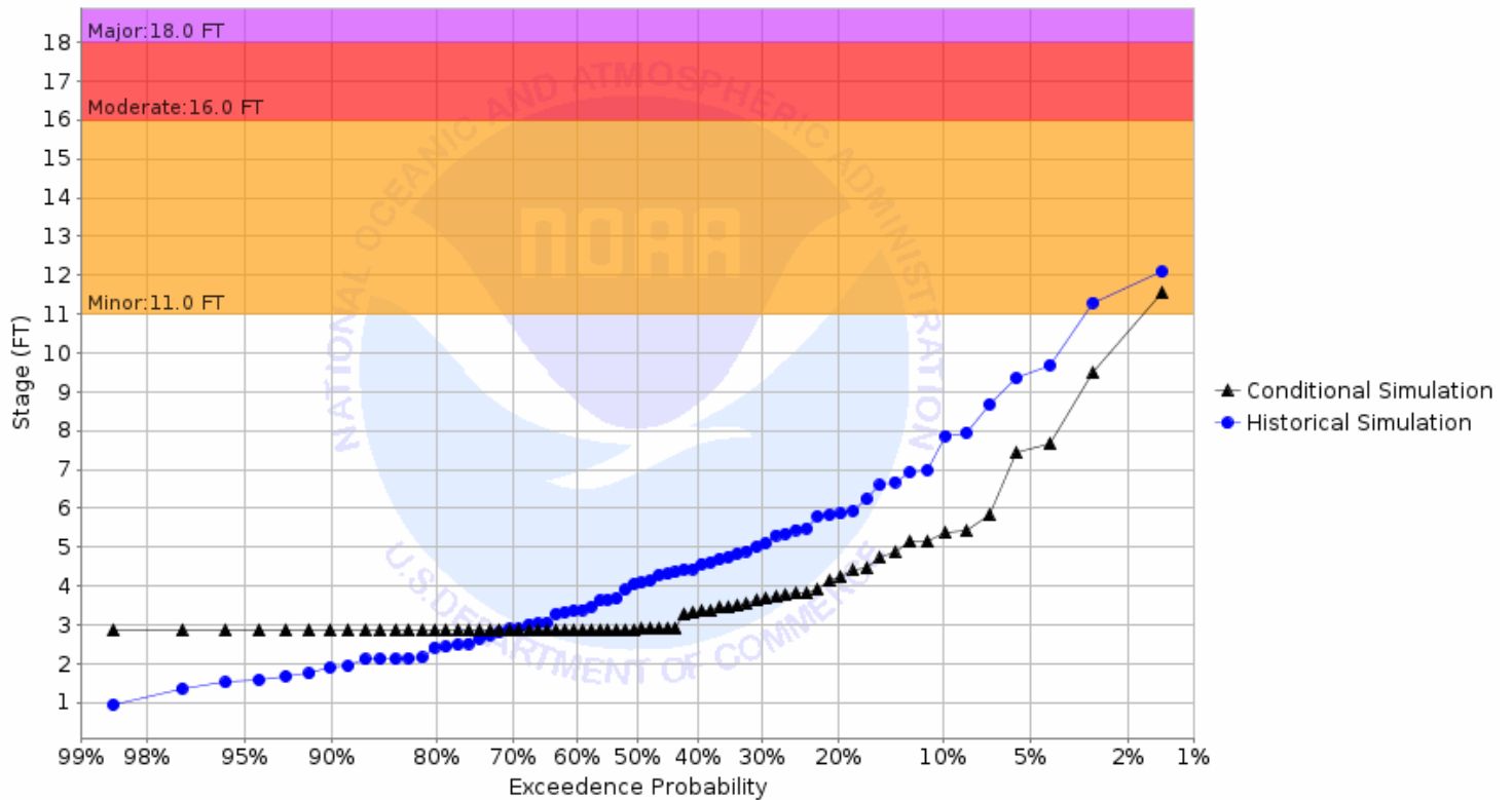
Chance of Exceeding River Stage at Pembina River at Walhalla (WLHN8) Forecast for the period 06/01/2026 - 08/30/2026 This is a conditional simulation based on the conditions as of 05/25/2026
