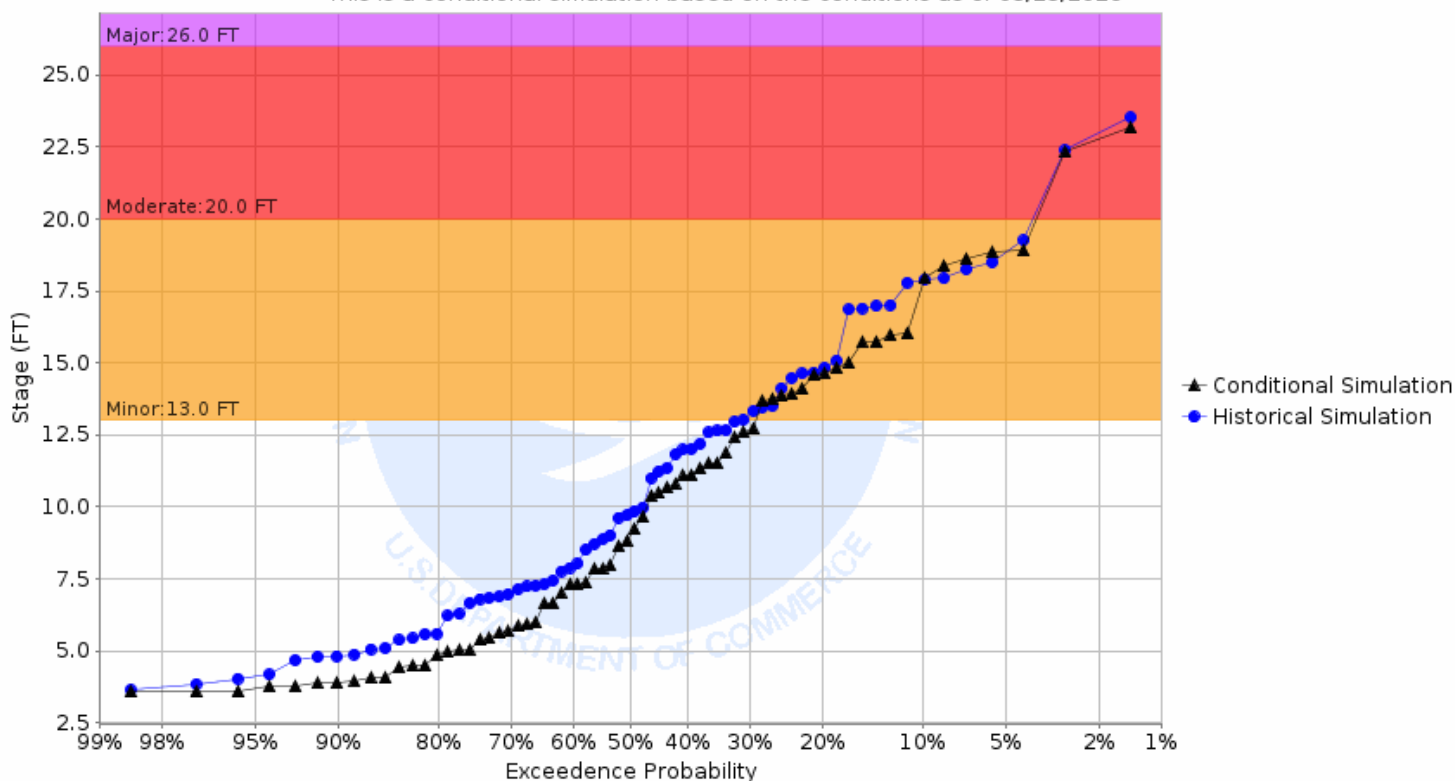
Chance of Exceeding River Stage at Buffalo River at Dilworth 7NE (DILM5) Forecast for the period 06/01/2026 - 08/30/2026 This is a conditional simulation based on the conditions as of 05/25/2026
