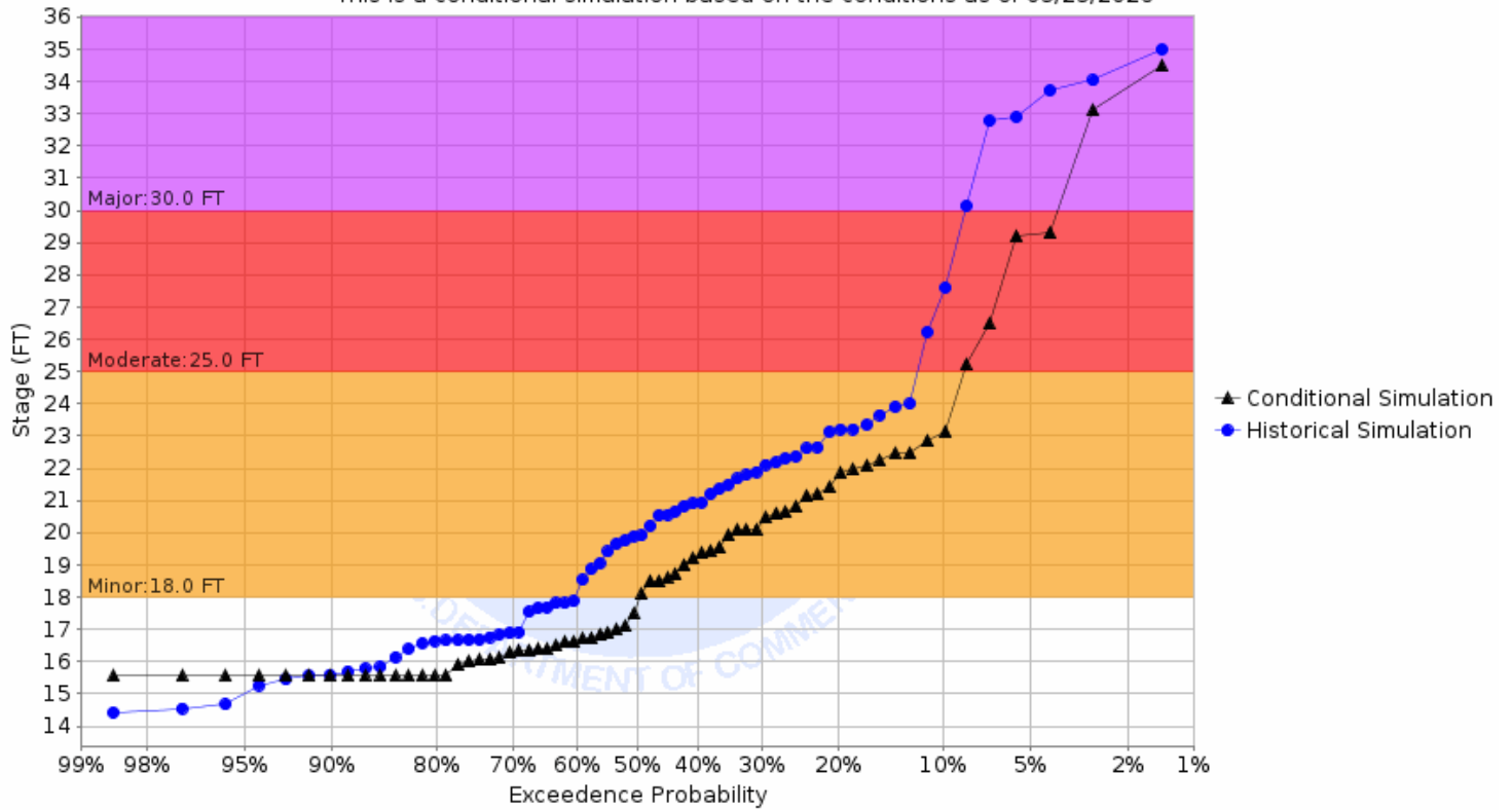
Chance of Exceeding River Stage at Red River of the North at Fargo WTP (FGON8) Forecast for the period 06/01/2026 - 08/30/2026 This is a conditional simulation based on the conditions as of 05/25/2026
