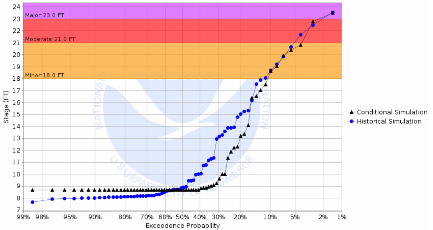
Chance of Exceeding River Stage at Maple River at Mapleton 3SW (MPLN8) Forecast for the period 06/01/2026 - 08/30/2026 This is a conditional simulation based on the conditions as of 05/25/2026
