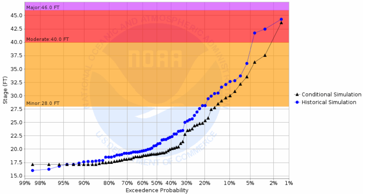
Chance of Exceeding River Stage at Red River of the North at East Grand Forks (EGFM5) Forecast for the period 06/01/2026 - 08/30/2026 This is a conditional simulation based on the conditions as of 05/25/2026
