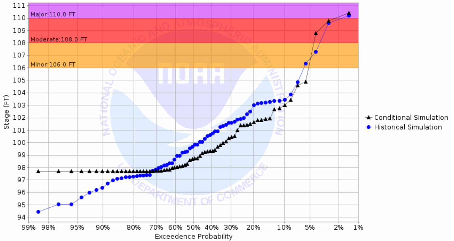
Chance of Exceeding River Stage at Snake River at Alvarado (ALVM5) Forecast for the period 06/01/2026 - 08/30/2026 This is a conditional simulation based on the conditions as of 05/25/2026
