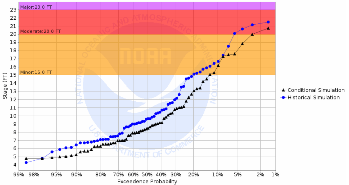
Chance of Exceeding River Stage at Red Lake River at Crookston (CRKM5) Forecast for the period 06/01/2026 - 08/30/2026 This is a conditional simulation based on the conditions as of 05/25/2026
