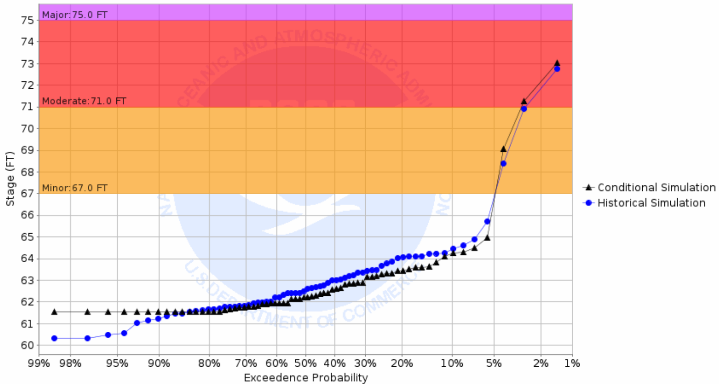
Chance of Exceeding River Stage at Snake River at Warren 3ENE-Morkassel Brdg (MKLM5) Forecast for the period 06/01/2026 - 08/30/2026 This is a conditional simulation based on the conditions as of 05/25/2026
