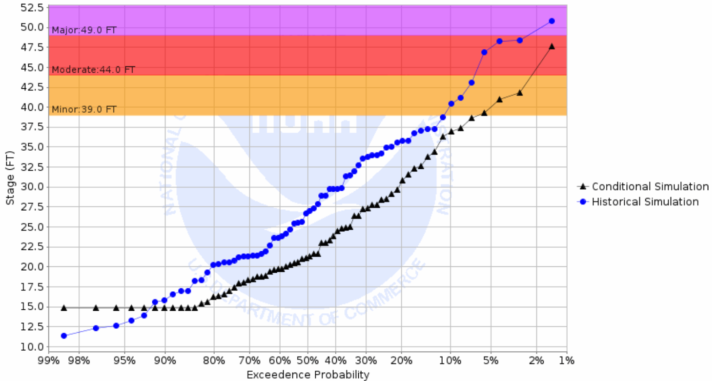
Chance of Exceeding River Stage at Red River of the North at Pembina (PBNN8) Forecast for the period 06/01/2026 - 08/30/2026 This is a conditional simulation based on the conditions as of 05/25/2026
