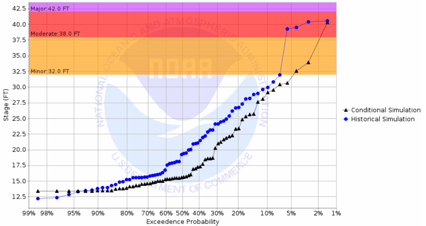
Chance of Exceeding River Stage at Red River of the North at Drayton 2NE - Hwy 66 Brdg (DRTN8) Forecast for the period 06/01/2026 - 08/30/2026 This is a conditional simulation based on the conditions as of 05/25/2026
