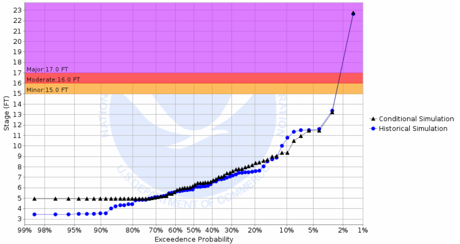
Chance of Exceeding River Stage at Sheyenne River at Valley City (VCRN8) Forecast for the period 06/01/2026 - 08/30/2026 This is a conditional simulation based on the conditions as of 05/25/2026
