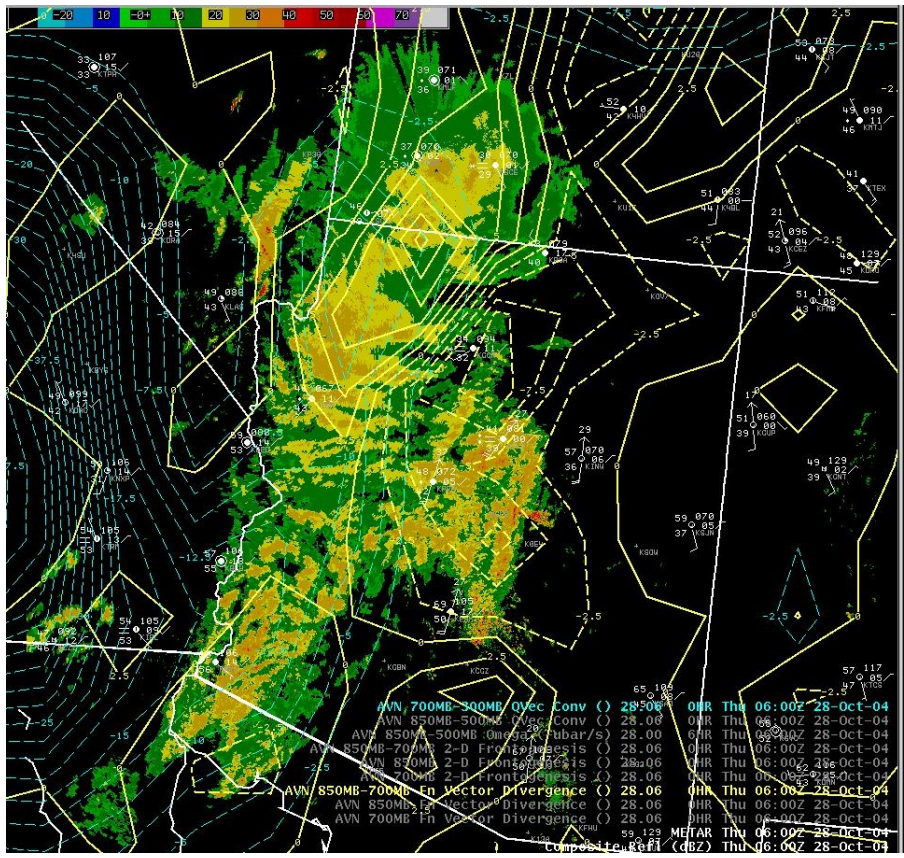
Figure 5: Radar imagery at 0600 UTC 28 October 2004, with METAR observations (white plots) and 850-700 mb Fv-divergence (yellow).
