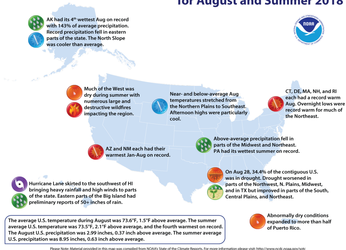
Figure 7: Climate Highlights for August of 2018.
