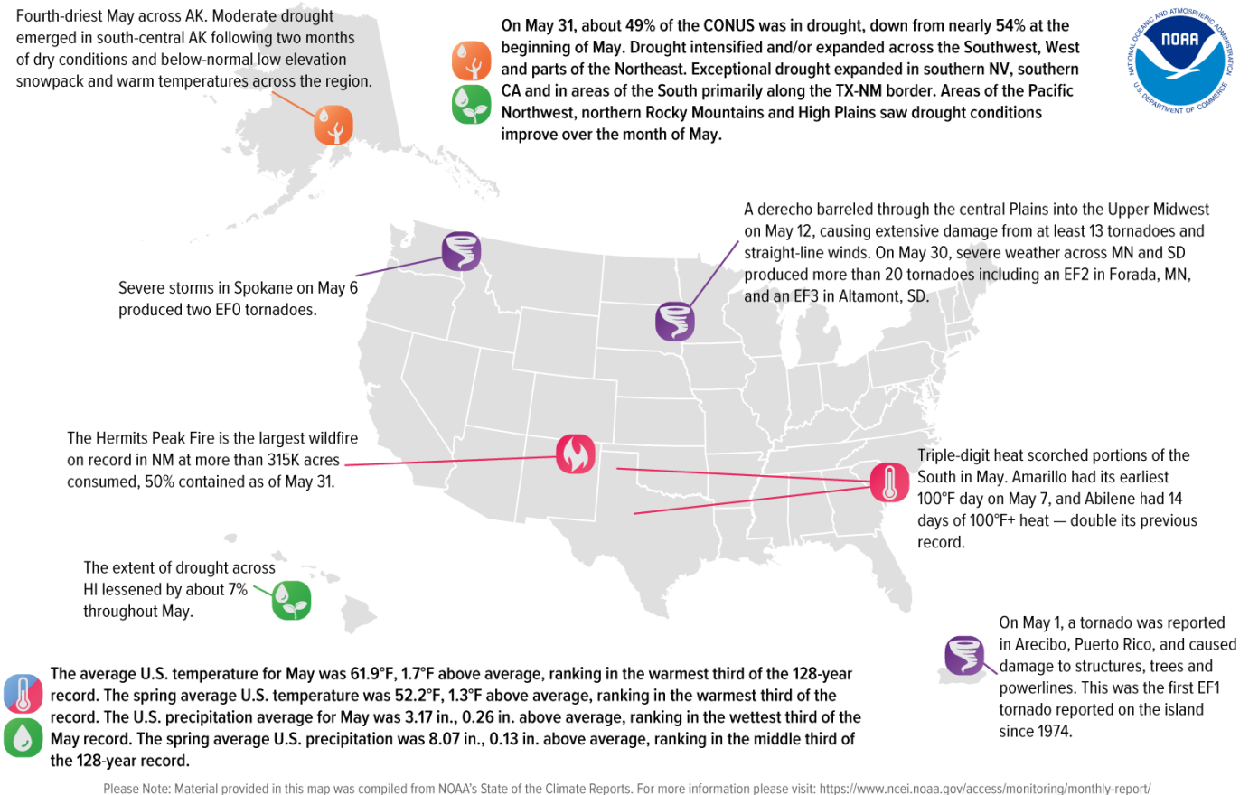
Figure 5: Significant Climate anomalies and events in May 2022
