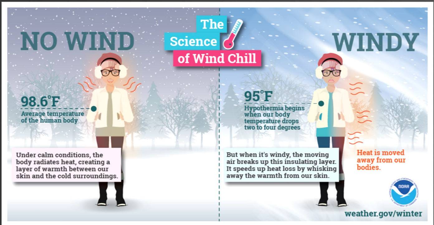
Figure 7: Graphic depicting the science of wind chill.
