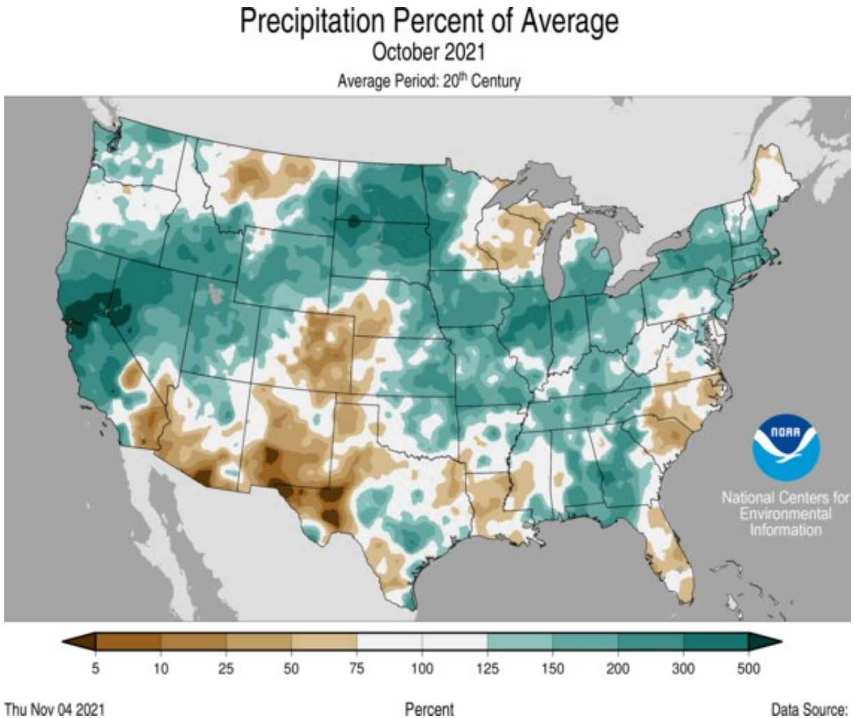
Figure 5: October 2021 Percent of Average Precipitation (U.S.).
