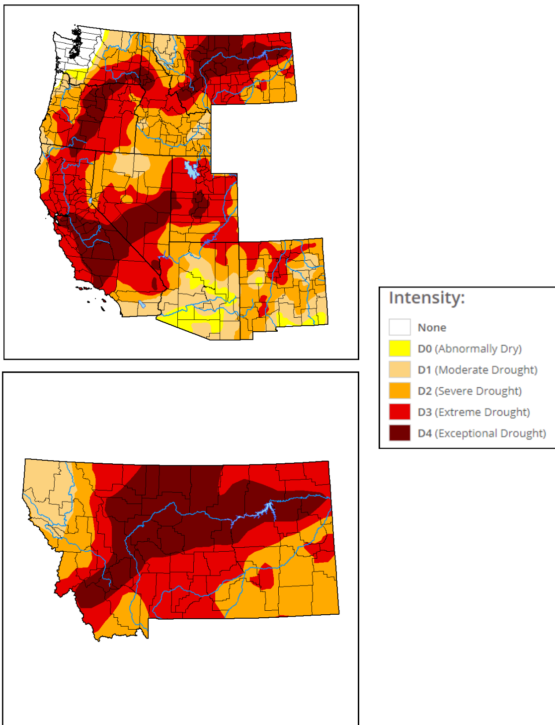
Figure 4: U.S. Drought Monitor updated December 2, 2021
