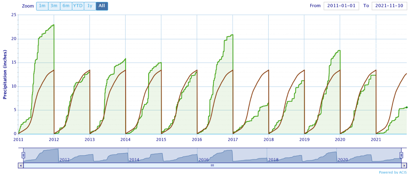
Accumulated Precipitation – Glasgow Area, MT (ThreadEx)
