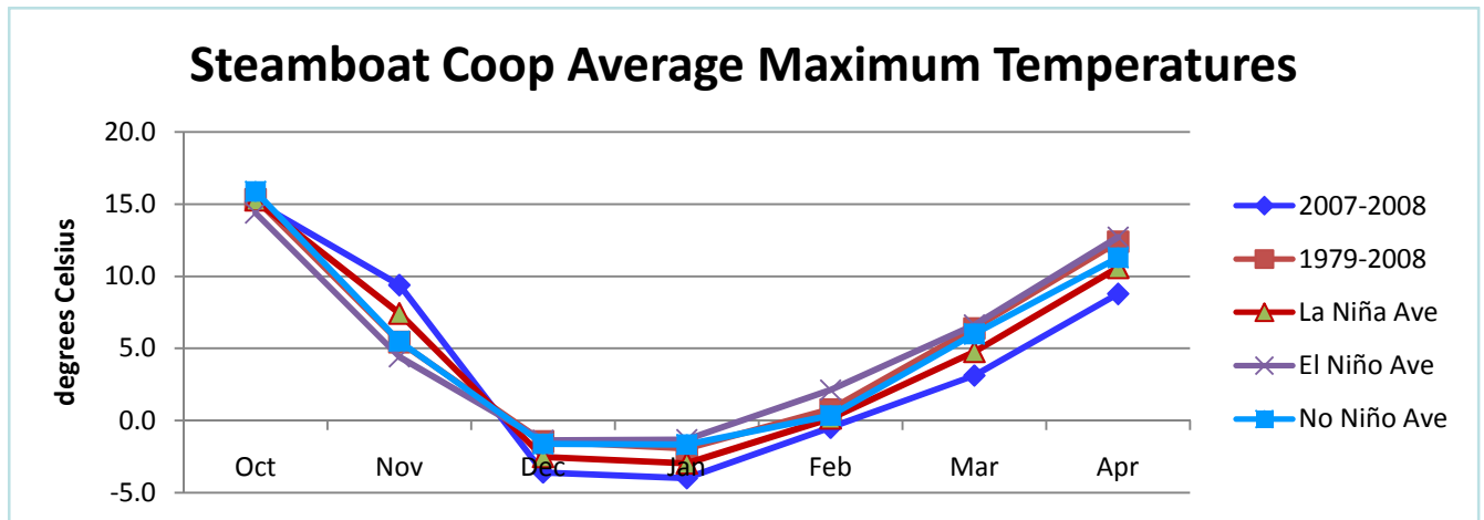
Figure 9: Graph of Maximum Temperature in degrees Celsius for the Steamboat Springs Cooperative Weather Observer site during different climate regimes. Note the colder than normal 2007-2008 winter.
