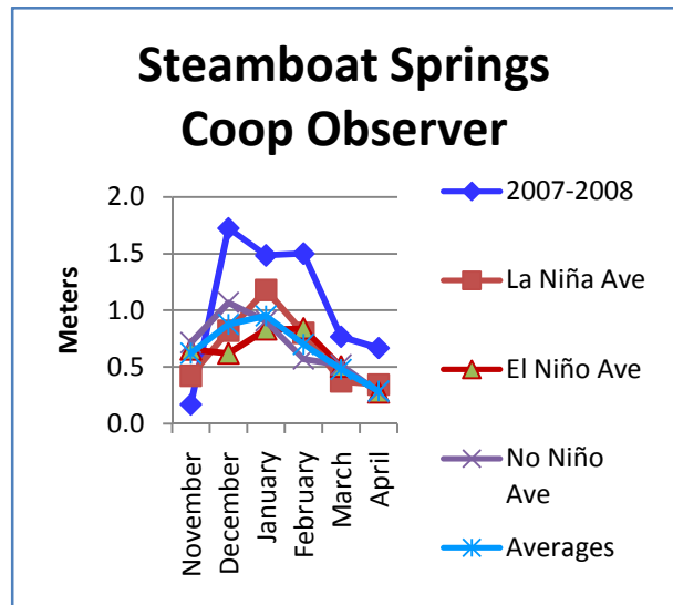
Figure 8: Graph represents seasonal snowfall in meters under different climate regimes for the Steamboat Springs Cooperative Weather Observer.
