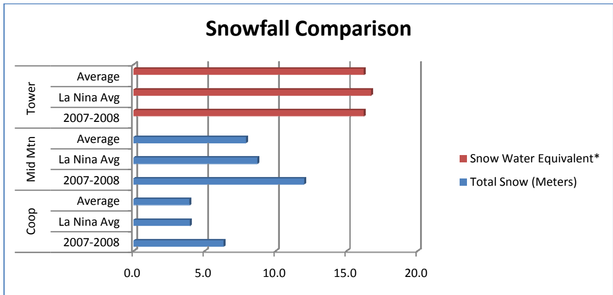
Figure 2: Graph of snowfall in meters comparing the 2007-08 winter to an average winter and to that of a typical La Niña Winter. *Note: The Tower SNOTEL data was converted from SWE using a 14:1 ratio (Judson and Doesken 2000)
