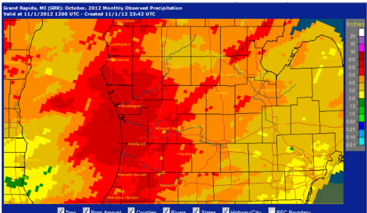
Figure 1. October 2012 Monthly Precipitation Totals
