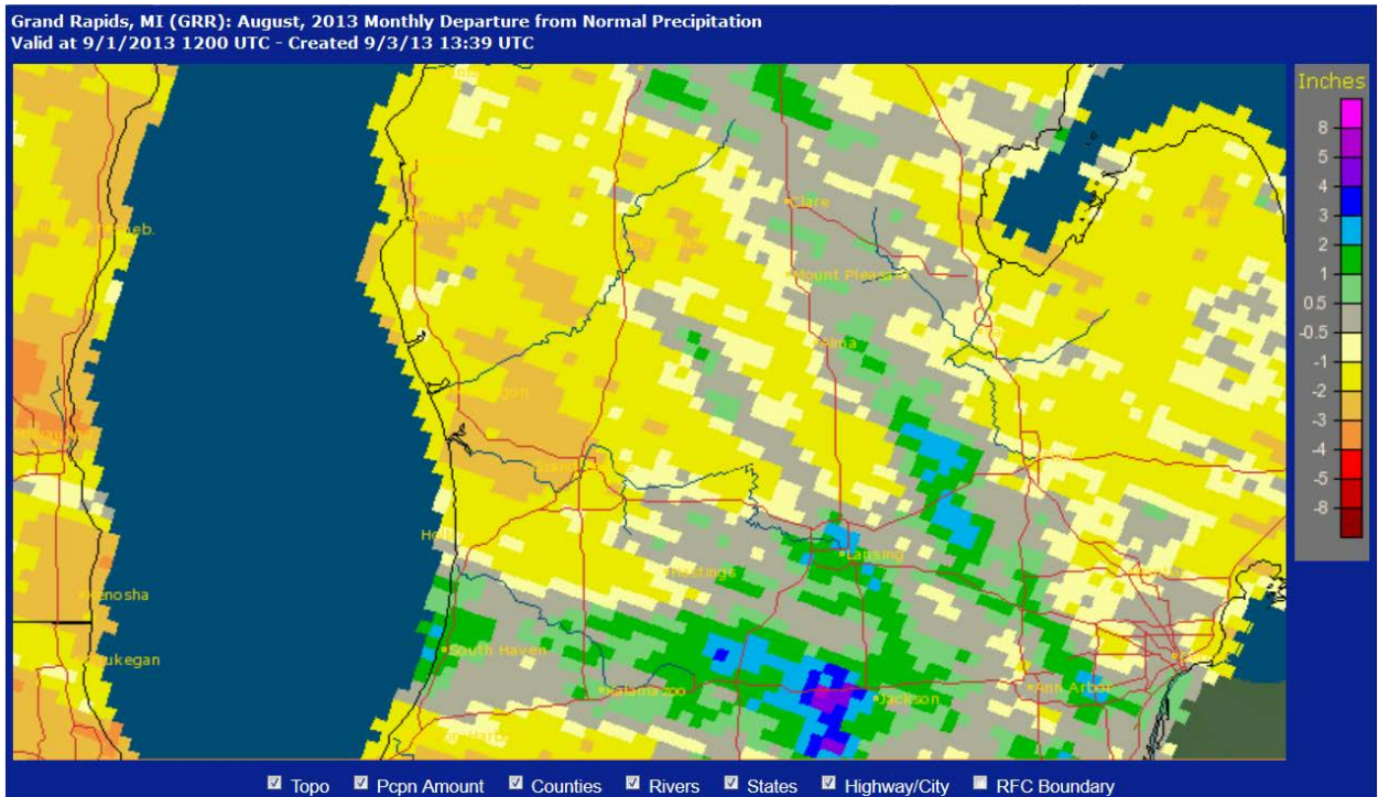
Figure 2. August Monthly Departure from Normal Precipitation Totals
