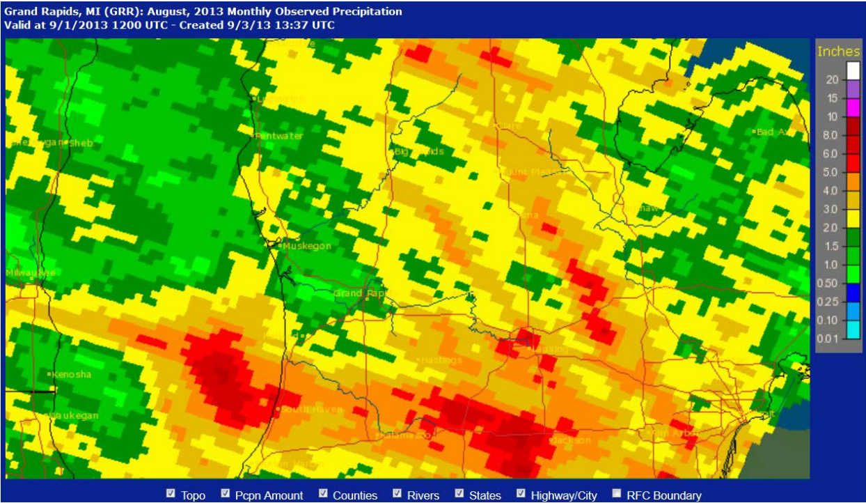
Figure 1. August Monthly Precipitation Totals
