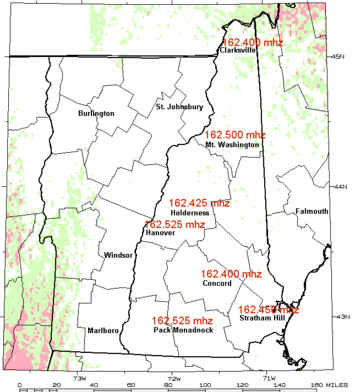
NWR transmitters across New Hampshire along with the frequency and signal level.
