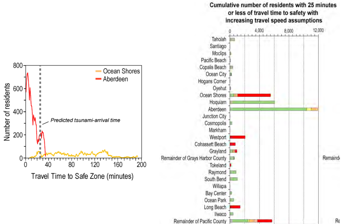
Figure S.56. Example of USGS Pedestrian Evacuation Analyst outputs summary graphs showing the number of residents who would be able to evacuate safely for towns in Washington ( Wood and Schmidtlein, 2013a ).
