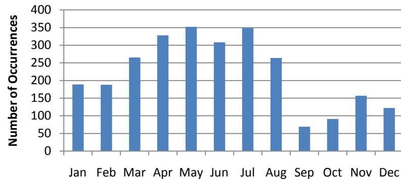
WFO LIX Severe Wind Events 1/1950 - 7/2009
