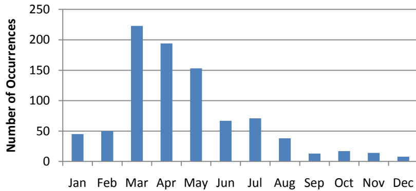
WFO LIX Severe Hail Events 1/1950 - 7/2009
