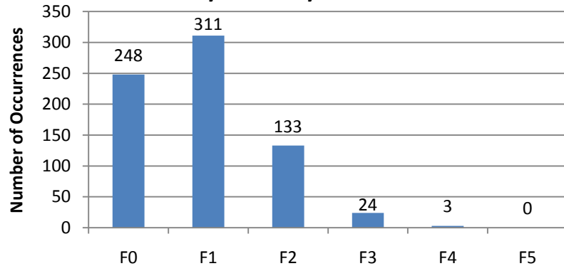
WFO LIX Tornadoes 1/1950 - 7/2009
