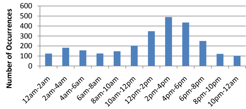
WFO LIX Severe Wind Events 1/1950 - 7/2009
