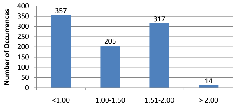
WFO LIX Severe Hail Events 1/1950 - 7/2009
