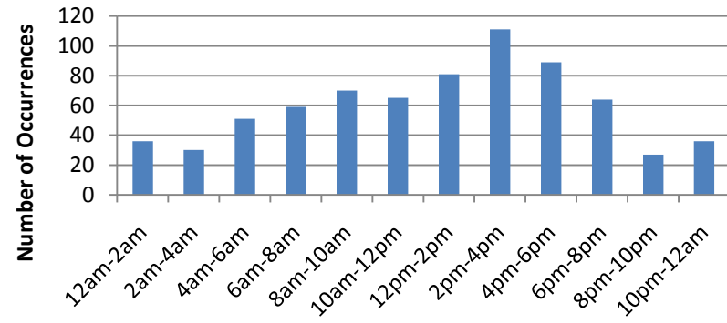
WFO LIX Tornadoes 1/1950 - 7/2009
