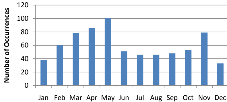
WFO LIX Tornadoes 1/1950 - 7/2009
