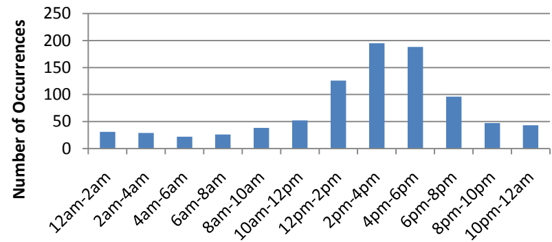
WFO LIX Severe Hail Events 1/1950 - 7/2009
