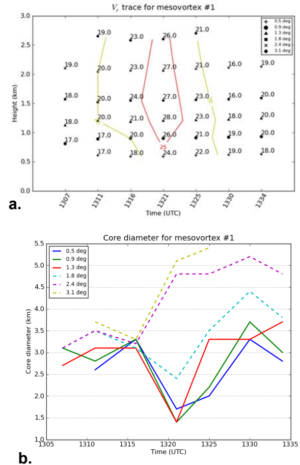
Fig. 12. (a) Rotational velocity trace for MV1. (b) Core diameter trace for MV1.
