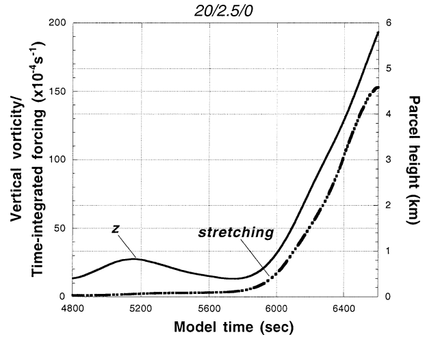
FIG. 9. Time series of parcel height ( z ) and time-integrated contribution to vertical vorticity from the relative vorticity-stretching term [ s^{-1} ; see Eq. (4.1)], along the forward trajectory denoted as “F” in Fig. 6.
