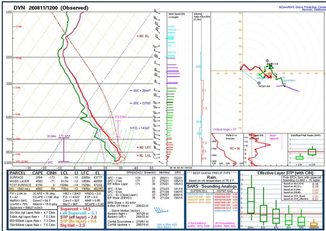
Figure 13. The 12:00 UTC / 7:00 AM CDT RAOB launched at KDVN the morning of 11 August 2026.
