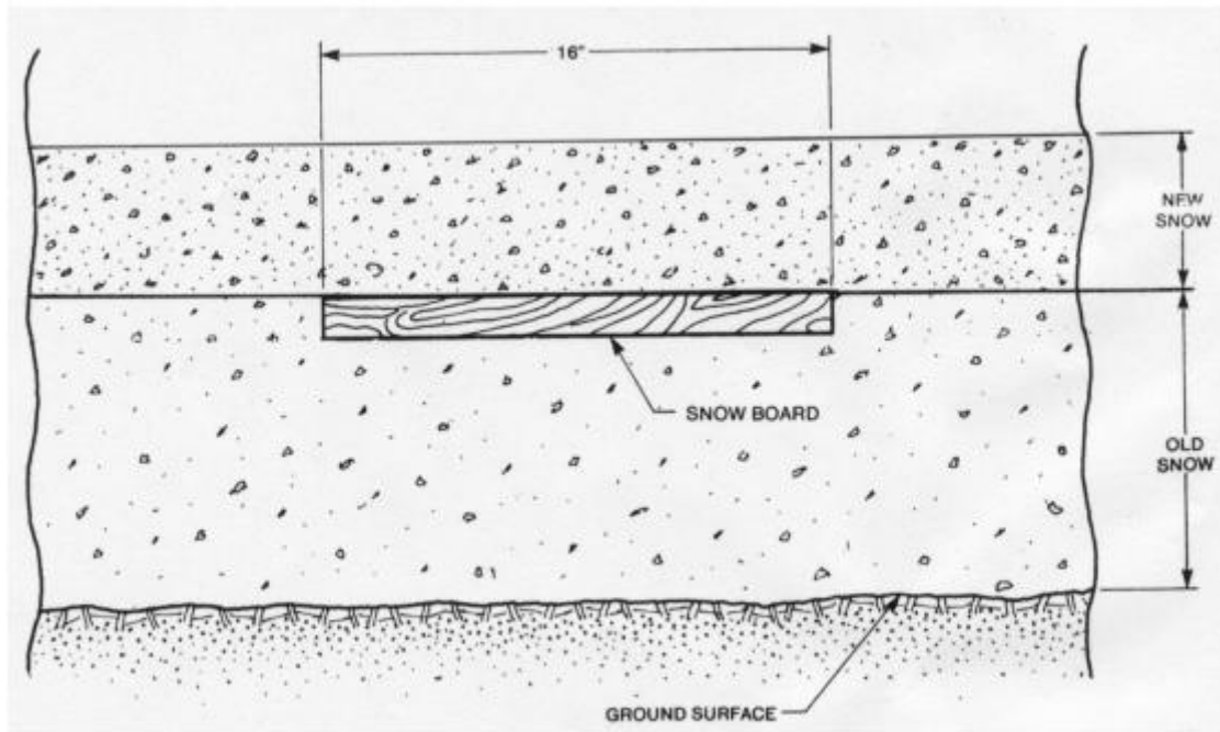
Figure A-34. Snow Measurement Board (size and material may vary)
