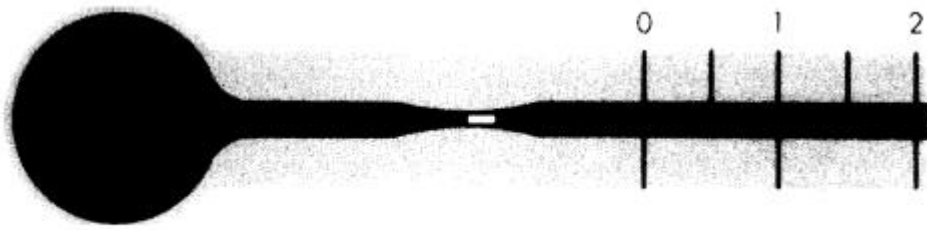
Figure B-4 - Liquid-in-Glass Maximum Thermometer
