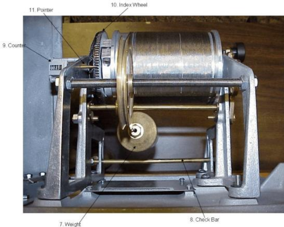
Figure C-3. Top View of Wire Weight Gauge Components
