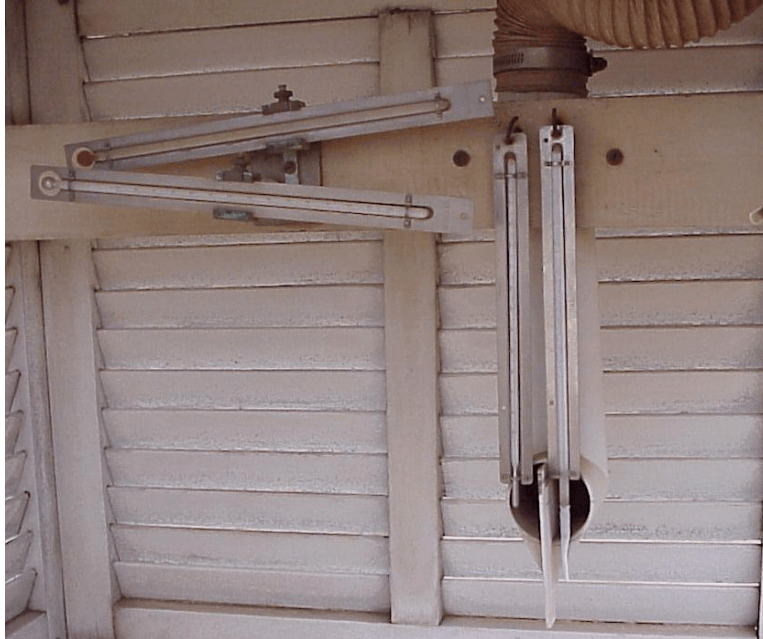
Figure D-9. CRS With Fan
