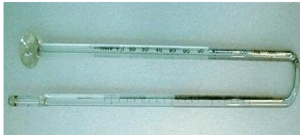
Figure D-12. Sixes Thermometer
