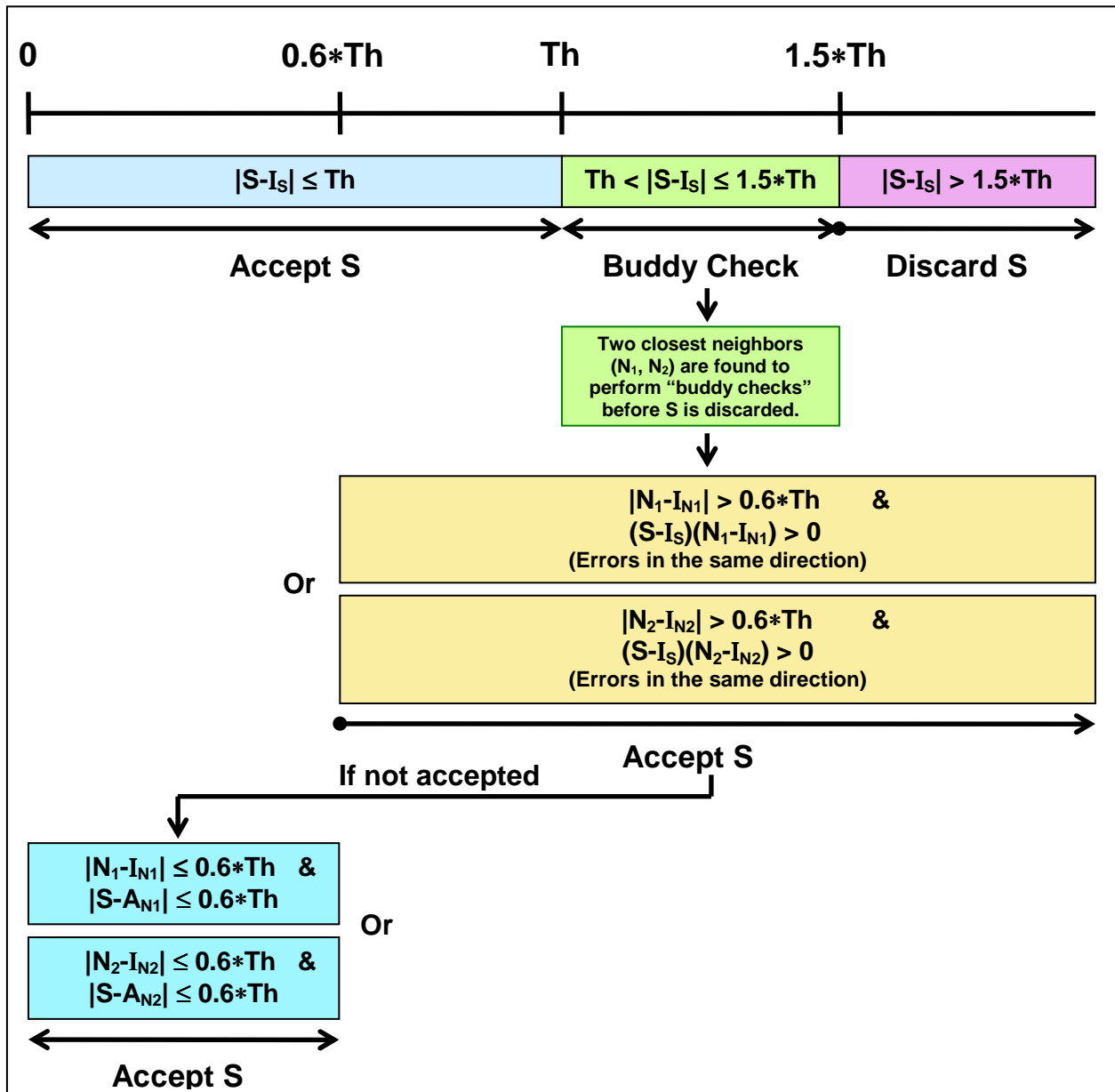
FIG. 1. BCDG's error checking procedures.
