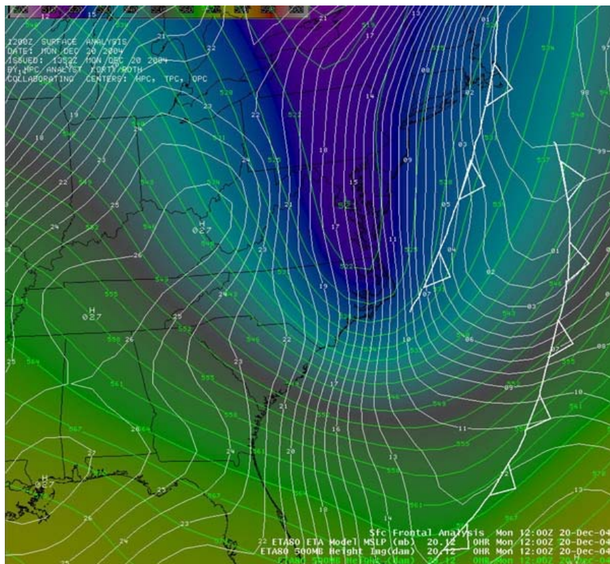
Figure 4. 12Z 12/20/2004 500 mb Heights (green lines), Mean Sea Level Pressure (white lines) and HPC Surface Frontal Analysis (thick white lines).
