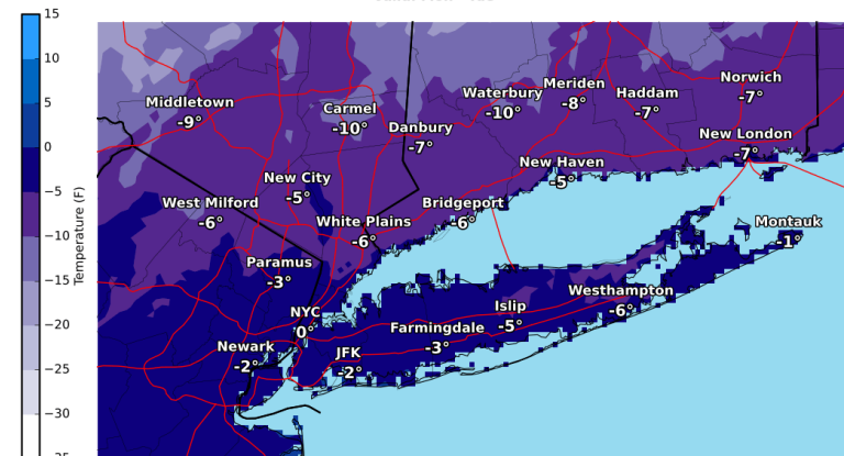
Coldest Wind Chill Temperatures for the Beginning of the Week Valid: Mon - Tue
